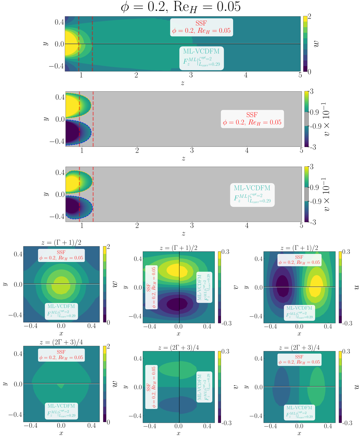
Figure D.110: Detailed comparison between the geometry-resolved small-scale flow (SSF) and ML-VCDFM using F_z^{ML} for the 1 \times 1 SRG at \phi = 0.2 and Re_H = 0.05 . The upper panels compare the streamwise velocity w and transverse velocity v in the central (z, y) -plane, restricted to the correction region. The lower panels compare the corresponding transverse (x, y) -plane distributions of w , v , and u , from left to right, at z = (\Gamma + 1)/2 in the first row and z = (2\Gamma + 3)/4 in the second row.
