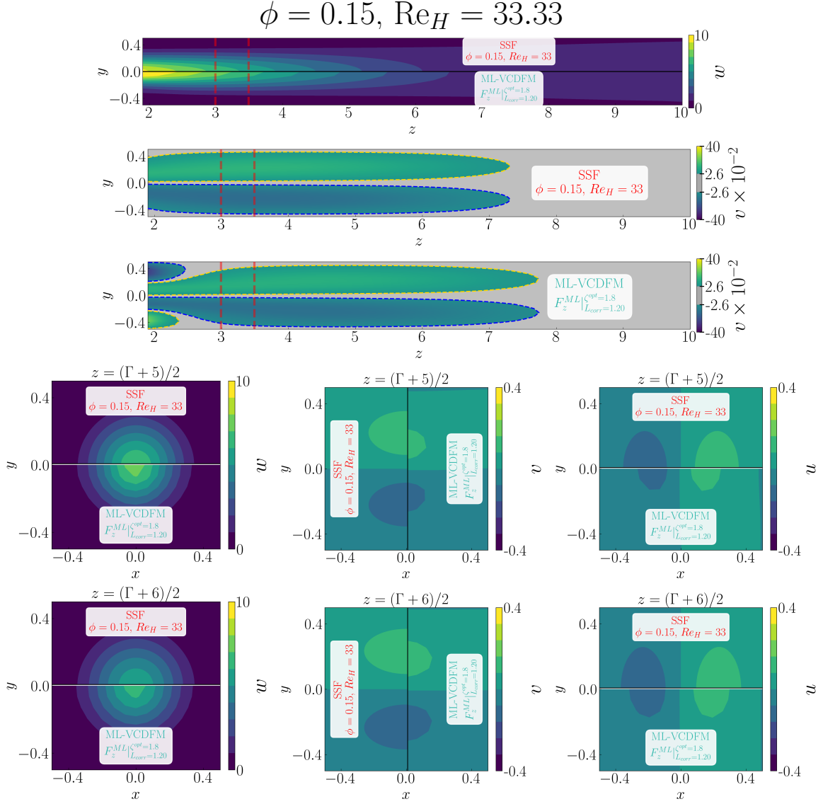
Figure D.104: Detailed comparison between the geometry-resolved small-scale flow (SSF) and ML-VCDFM using F_z^{ML} for the 1 \times 1 SRG at \phi = 0.15 and Re_H = 33.33 . The upper panels compare the streamwise velocity w and transverse velocity v in the central (z, y) -plane, restricted to the correction region. The lower panels compare the corresponding transverse (x, y) -plane distributions of w , v , and u , from left to right, at z = (\Gamma + 5)/2 in the first row and z = (\Gamma + 6)/2 in the second row.
