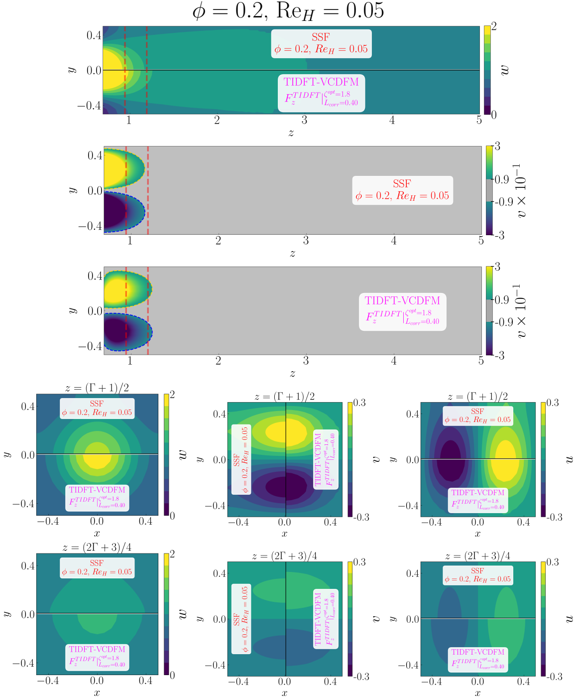
Figure D.109: Detailed comparison between the geometry-resolved small-scale flow (SSF) and TIDFT-VCDFM using F_z^{TIDFT} for the 1 \times 1 SRG at \phi = 0.2 and Re_H = 0.05 . The upper panels compare the streamwise velocity w and transverse velocity v in the central (z, y) -plane, restricted to the correction region. The lower panels compare the corresponding transverse (x, y) -plane distributions of w , v , and u , from left to right, at z = (\Gamma + 1)/2 in the first row and z = (2\Gamma + 3)/4 in the second row.
