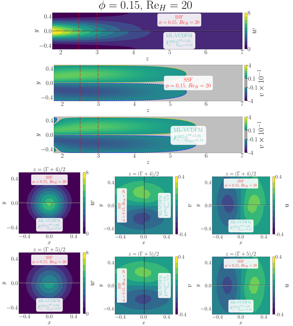
Figure D.98: Detailed comparison between the geometry-resolved small-scale flow (SSF) and ML-VCDFM using F_z^{ML} for the 1 \times 1 SRG at \phi = 0.15 and Re_H = 20 . The upper panels compare the streamwise velocity w and transverse velocity v in the central (z, y) -plane, restricted to the correction region. The lower panels compare the corresponding transverse (x, y) -plane distributions of w , v , and u , from left to right, at z = (\Gamma + 4)/2 in the first row and z = (\Gamma + 5)/2 in the second row.
