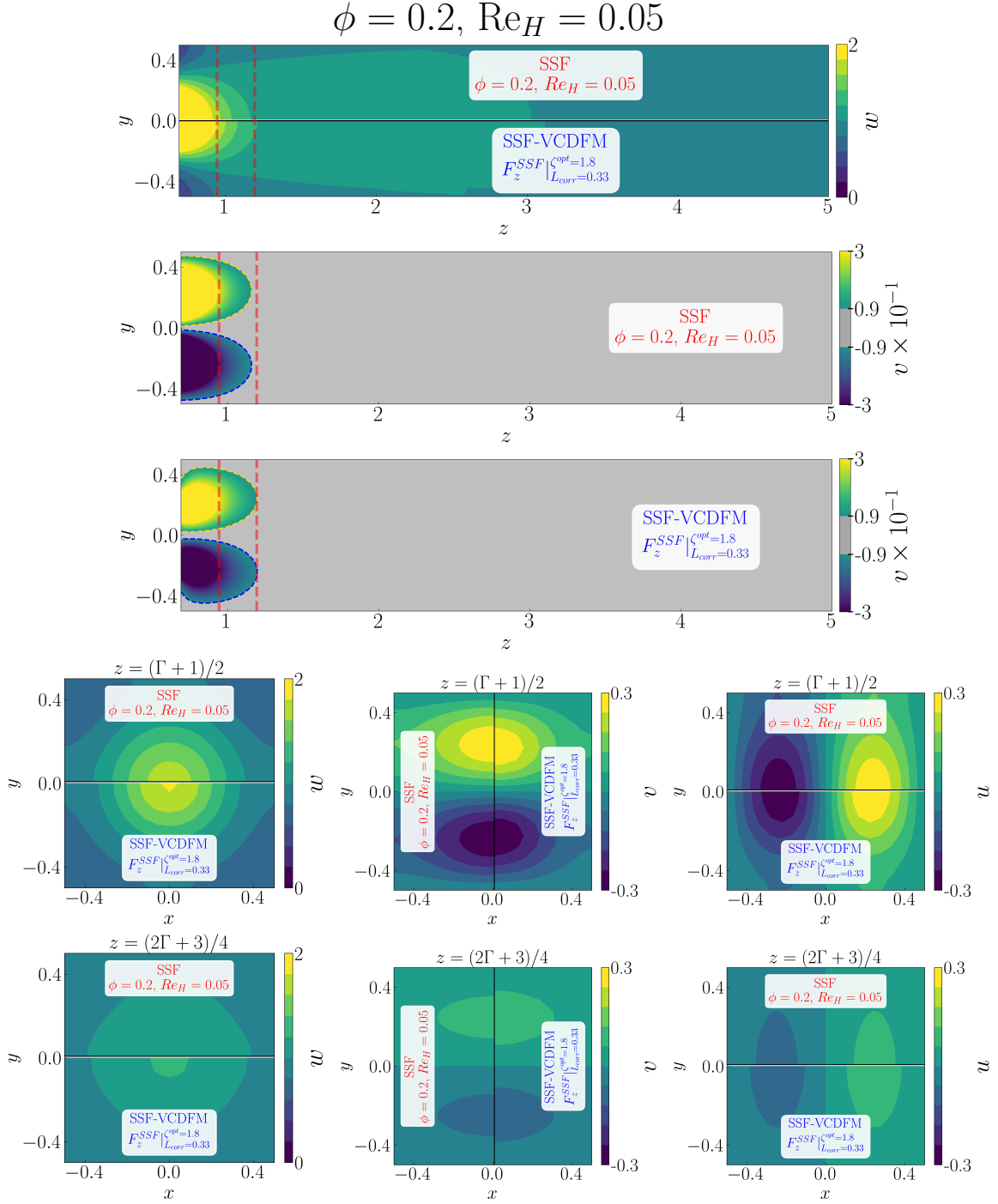
Figure D.108: Detailed comparison between the geometry-resolved small-scale flow (SSF) and SSF-VCDFM using F_z^{SSF} for the 1 \times 1 SRG at \phi = 0.2 and Re_H = 0.05 . The upper panels compare the streamwise velocity w and transverse velocity v in the central (z, y) -plane, restricted to the correction region. The lower panels compare the corresponding transverse (x, y) -plane distributions of w , v , and u , from left to right, at z = (\Gamma + 1)/2 in the first row and z = (2\Gamma + 3)/4 in the second row.
