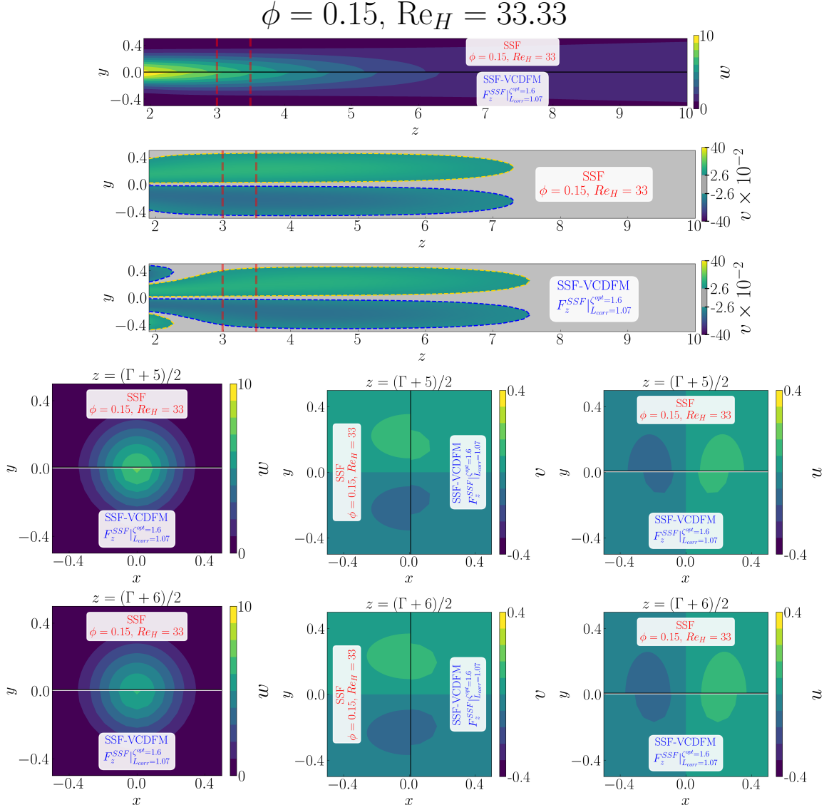
Figure D.102: Detailed comparison between the geometry-resolved small-scale flow (SSF) and SSF-VCDFM using F_z^{SSF} for the 1 × 1 SRG at \phi = 0.15 and Re_H = 33.33 . The upper panels compare the streamwise velocity w and transverse velocity v in the central (z, y) -plane, restricted to the correction region. The lower panels compare the corresponding transverse (x, y) -plane distributions of w , v , and u , from left to right, at z = (\Gamma + 5)/2 in the first row and z = (\Gamma + 6)/2 in the second row.
