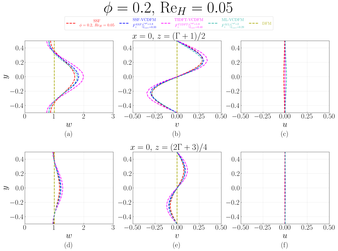
Figure D.107: Velocity profiles at x = 0 for the 1 \times 1 SRG at \phi = 0.2 and \text{Re}_H = 0.05 , comparing the SSF, DFM, SSF-VCDFM, TIDFT-VCDFM, and ML-VCDFM. Profiles of w(y) , v(y) , and u(y) are shown at z = (\Gamma + 1)/2 in (a–c) and z = (2\Gamma + 3)/4 in (d–f).
