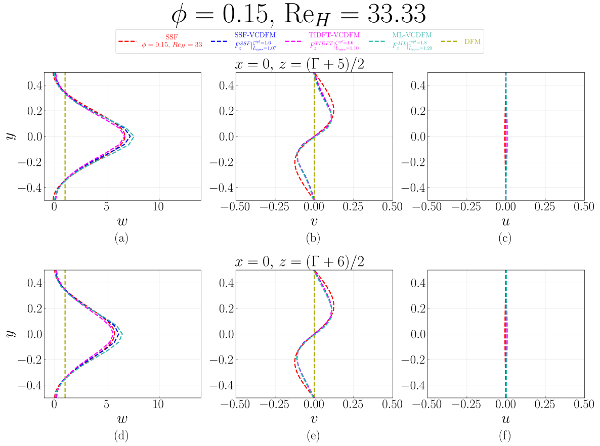
Figure D.101: Velocity profiles at x = 0 for the 1 \times 1 SRG at \phi = 0.15 and \text{Re}_H = 33.33 , comparing the SSF, DFM, SSF-VCDFM, TIDFT-VCDFM, and ML-VCDFM. Profiles of w(y) , v(y) , and u(y) are shown at z = (\Gamma + 5)/2 in (a–c) and z = (\Gamma + 6)/2 in (d–f).
