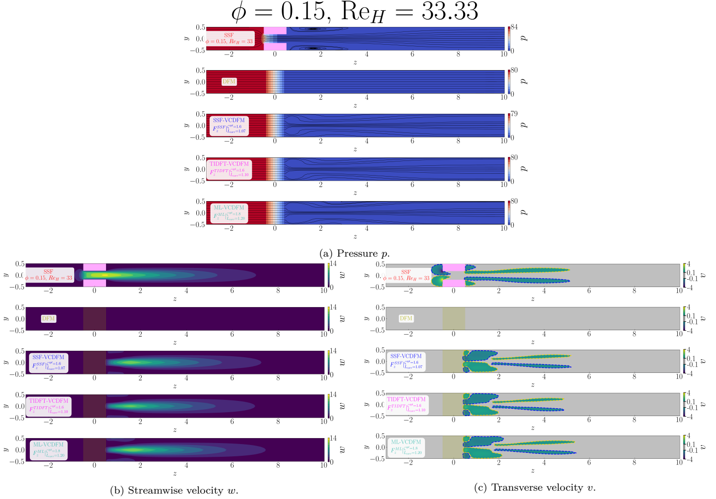
Figure D.100: Flow organization in the streamwise (z, y) -plane for the 1 \times 1 SRG at \phi = 0.15 , Re_H = 33.33 , and \alpha = 0^\circ . The blocks show (a) pressure p with streamlines, (b) streamwise velocity w , and (c) transverse velocity v . Within each block, the rows show, from top to bottom, the SSF, DFM, SSF-VCDFM, TIDFT-VCDFM, and ML-VCDFM. Pink shading marks the grid walls in the SSF; olive shading marks the equivalent porous zone in the model solutions.
