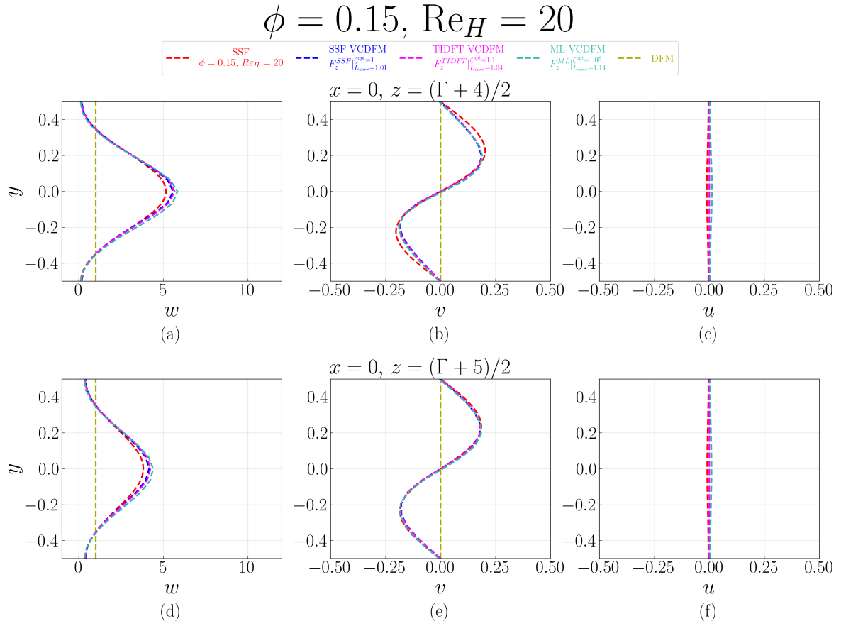
Figure D.95: Velocity profiles at x = 0 for the 1 \times 1 SRG at \phi = 0.15 and \text{Re}_H = 20 , comparing the SSF, DFM, SSF-VCDFM, TIDFT-VCDFM, and ML-VCDFM. Profiles of w(y) , v(y) , and u(y) are shown at z = (\Gamma + 4)/2 in (a–c) and z = (\Gamma + 5)/2 in (d–f).
