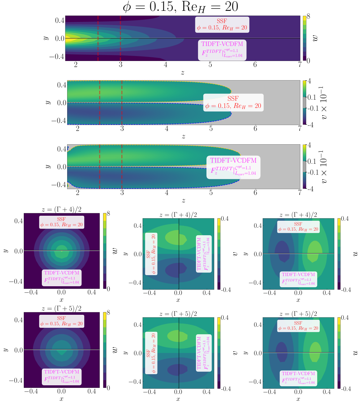
Figure D.97: Detailed comparison between the geometry-resolved small-scale flow (SSF) and TIDFT-VCDFM using F_z^{TIDFT} for the 1 \times 1 SRG at \phi = 0.15 and Re_H = 20 . The upper panels compare the streamwise velocity w and transverse velocity v in the central (z, y) -plane, restricted to the correction region. The lower panels compare the corresponding transverse (x, y) -plane distributions of w , v , and u , from left to right, at z = (\Gamma + 4)/2 in the first row and z = (\Gamma + 5)/2 in the second row.
