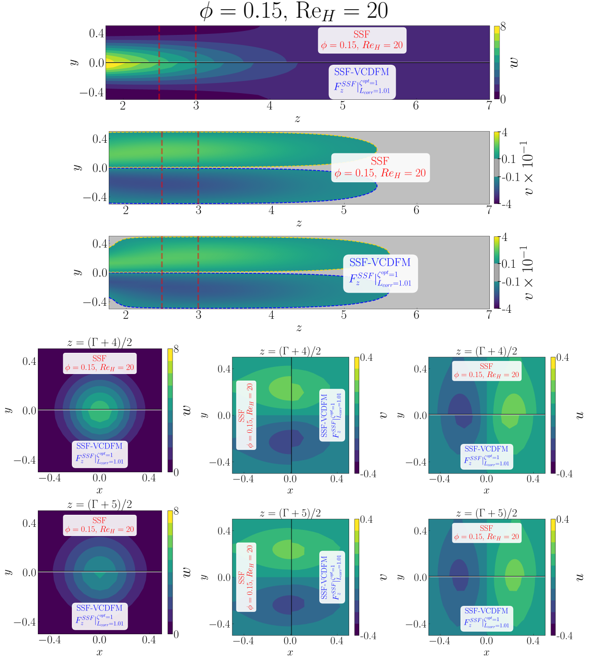
Figure D.96: Detailed comparison between the geometry-resolved small-scale flow (SSF) and SSF-VCDFM using F_z^{SSF} for the 1 \times 1 SRG at \phi = 0.15 and Re_H = 20 . The upper panels compare the streamwise velocity w and transverse velocity v in the central (z, y) -plane, restricted to the correction region. The lower panels compare the corresponding transverse (x, y) -plane distributions of w , v , and u , from left to right, at z = (\Gamma + 4)/2 in the first row and z = (\Gamma + 5)/2 in the second row.
