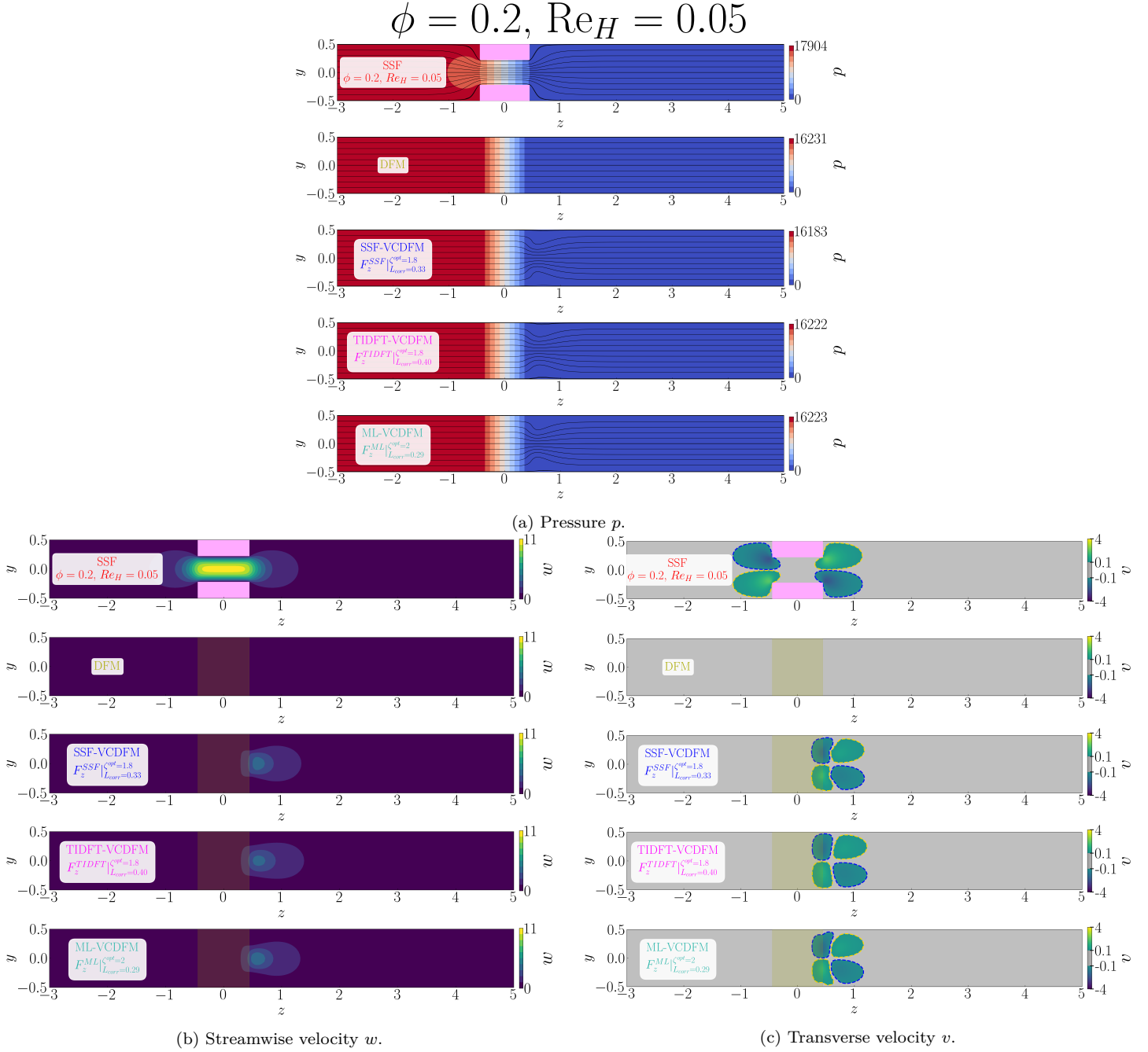
Figure D.106: Flow organization in the streamwise (z, y) -plane for the 1 \times 1 SRG at \phi = 0.2 , \text{Re}_H = 0.05 , and \alpha = 0^\circ . The blocks show (a) pressure p with streamlines, (b) streamwise velocity w , and (c) transverse velocity v . Within each block, the rows show, from top to bottom, the SSF, DFM, SSF-VCDFM, TIDFT-VCDFM, and ML-VCDFM. Pink shading marks the grid walls in the SSF; olive shading marks the equivalent porous zone in the model solutions.
