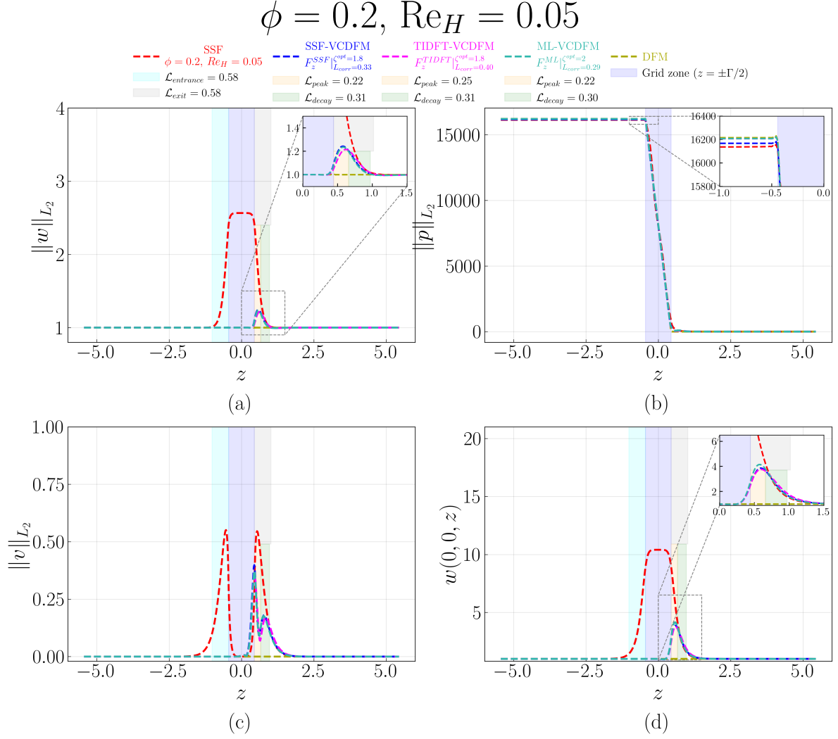
Figure D.105: Streamwise evolution of (a) \|w\|_{L_2} , (b) \|p\|_{L_2} , (c) \|v\|_{L_2} , and (d) centerline velocity w(0,0,z) for the 1 \times 1 SRG at \phi = 0.2 and \text{Re}_H = 0.05 . The figure compares the SSF, DFM, SSF-VCDFM, TIDFT-VCDFM, and ML-VCDFM. Shading marks the grid and the characteristic entrance, exit, peak, and decay regions. Only the SSF-based \mathcal{L}_{\text{peak}} and \mathcal{L}_{\text{decay}} are marked on the plot; the corresponding TIDFT-VCDFM and ML-VCDFM values appear in the legend.
