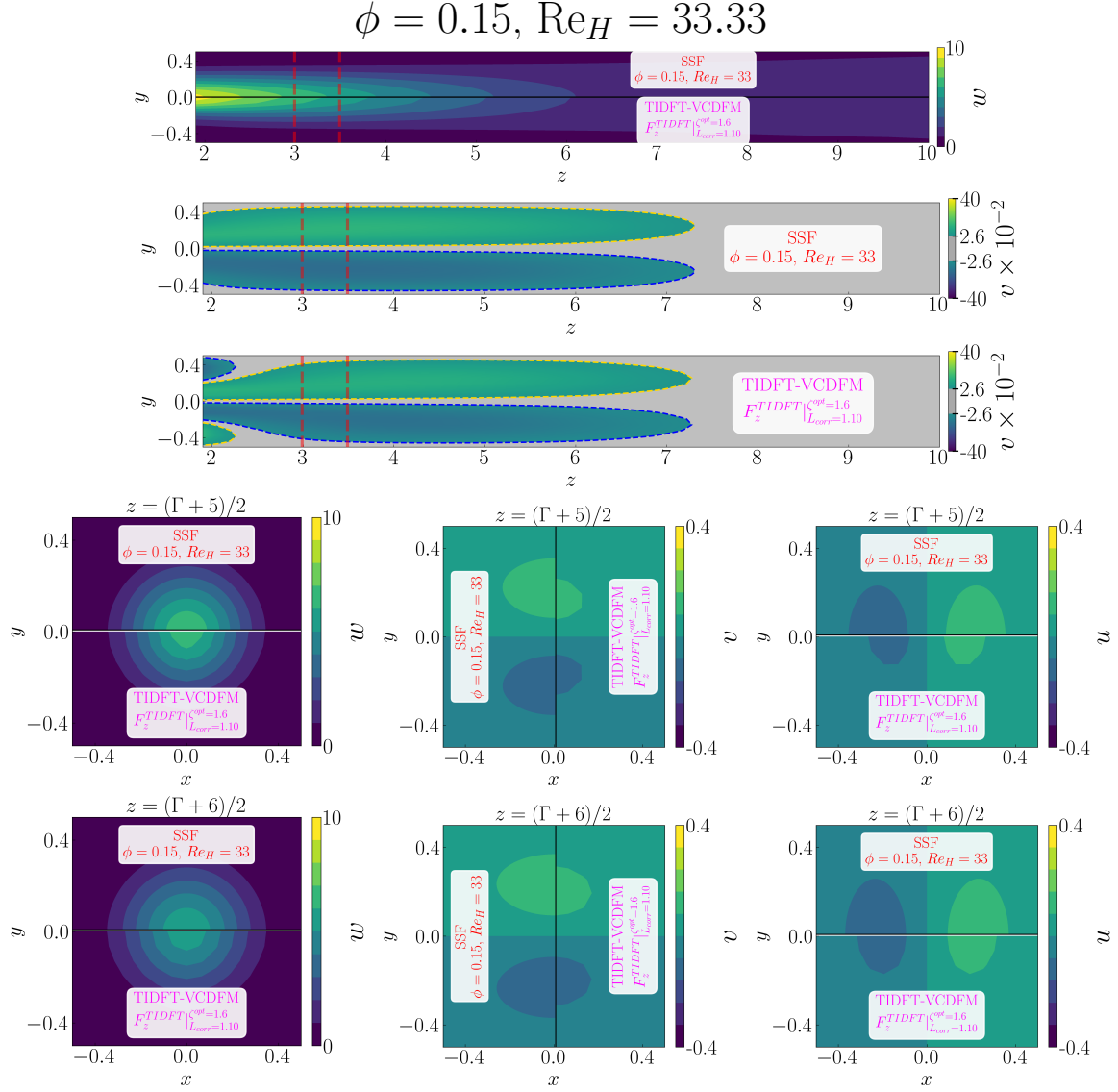
Figure D.103: Detailed comparison between the geometry-resolved small-scale flow (SSF) and TIDFT-VCDFM using F_z^{TIDFT} for the 1 \times 1 SRG at \phi = 0.15 and Re_H = 33.33 . The upper panels compare the streamwise velocity w and transverse velocity v in the central (z, y) -plane, restricted to the correction region. The lower panels compare the corresponding transverse (x, y) -plane distributions of w , v , and u , from left to right, at z = (\Gamma + 5)/2 in the first row and z = (\Gamma + 6)/2 in the second row.
