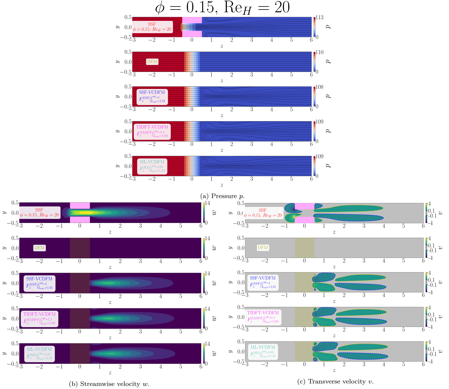
Figure D.94: Flow organization in the streamwise (z, y) -plane for the 1 \times 1 SRG at \phi = 0.15 , \text{Re}_H = 20 , and \alpha = 0^\circ . The blocks show (a) pressure p with streamlines, (b) streamwise velocity w , and (c) transverse velocity v . Within each block, the rows show, from top to bottom, the SSF, DFM, SSF-VCDFM, TIDFT-VCDFM, and ML-VCDFM. Pink shading marks the grid walls in the SSF; olive shading marks the equivalent porous zone in the model solutions.
