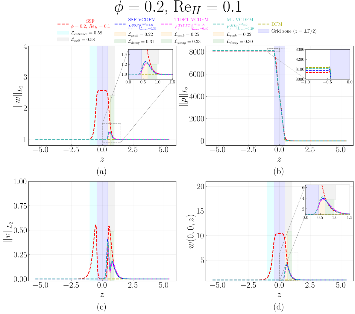
Figure D.111: Streamwise evolution of (a) \|w\|_{L_2} , (b) \|p\|_{L_2} , (c) \|v\|_{L_2} , and (d) centerline velocity w(0,0,z) for the 1 \times 1 SRG at \phi = 0.2 and \text{Re}_H = 0.1 . The figure compares the SSF, DFM, SSF-VCDFM, TIDFT-VCDFM, and ML-VCDFM. Shading marks the grid and the characteristic entrance, exit, peak, and decay regions. Only the SSF-based \mathcal{L}_{\text{peak}} and \mathcal{L}_{\text{decay}} are marked on the plot; the corresponding TIDFT-VCDFM and ML-VCDFM values appear in the legend.
