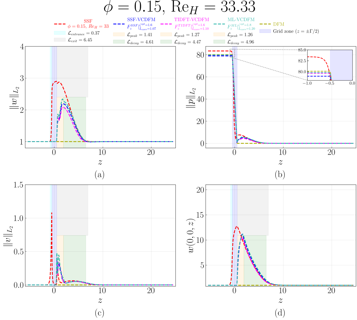
Figure D.99: Streamwise evolution of (a) \|w\|_{L_2} , (b) \|p\|_{L_2} , (c) \|v\|_{L_2} , and (d) centerline velocity w(0,0,z) for the 1 \times 1 SRG at \phi = 0.15 and \text{Re}_H = 33.33 . The figure compares the SSF, DFM, SSF-VCDFM, TIDFT-VCDFM, and ML-VCDFM. Shading marks the grid and the characteristic entrance, exit, peak, and decay regions. Only the SSF-based \mathcal{L}_{\text{peak}} and \mathcal{L}_{\text{decay}} are marked on the plot; the corresponding TIDFT-VCDFM and ML-VCDFM values appear in the legend.
