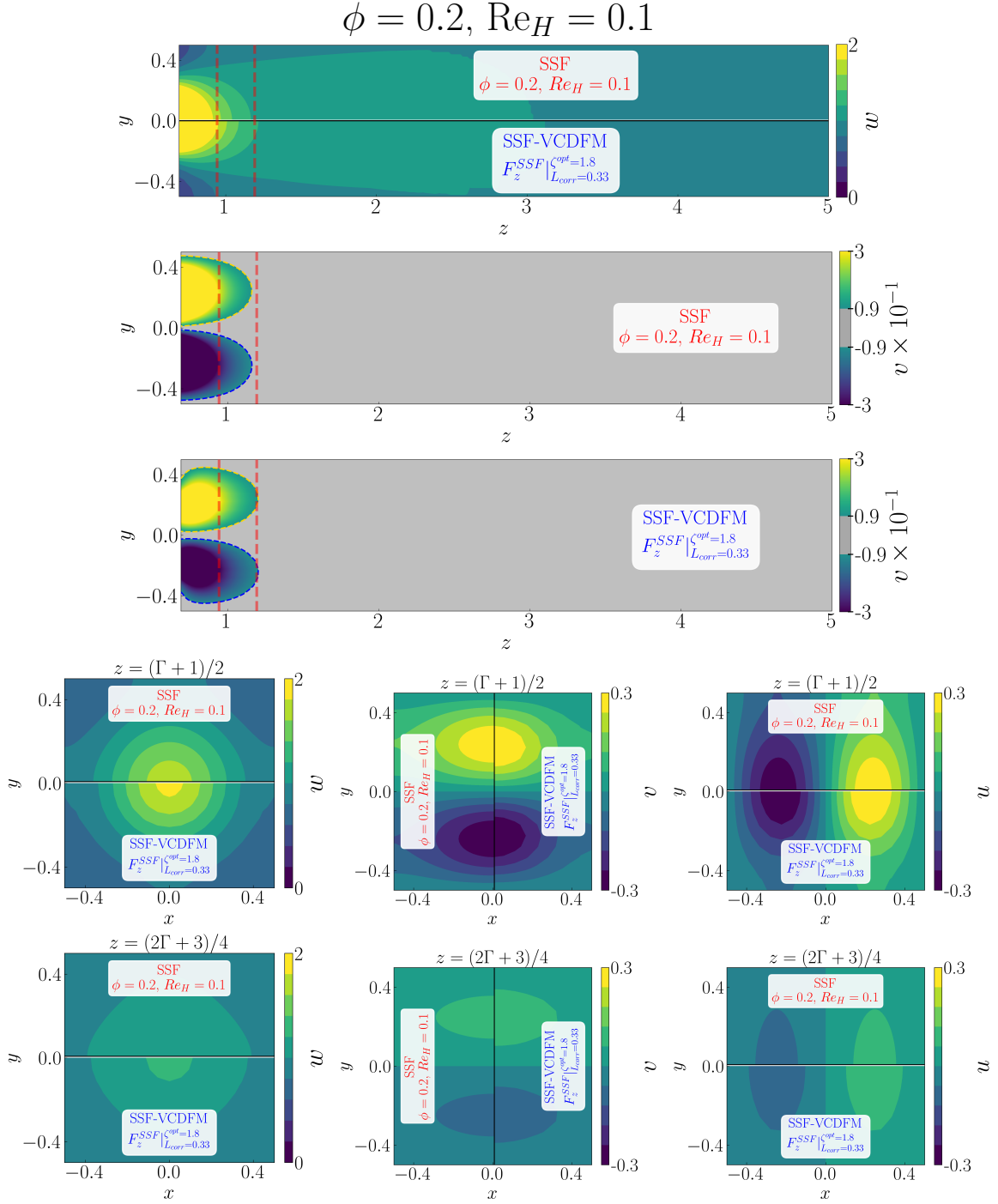
Figure D.114: Detailed comparison between the geometry-resolved small-scale flow (SSF) and SSF-VCDFM using F_z^{SSF} for the 1 \times 1 SRG at \phi = 0.2 and Re_H = 0.1 . The upper panels compare the streamwise velocity w and transverse velocity v in the central (z, y) -plane, restricted to the correction region. The lower panels compare the corresponding transverse (x, y) -plane distributions of w , v , and u , from left to right, at z = (\Gamma + 1)/2 in the first row and z = (2\Gamma + 3)/4 in the second row.
