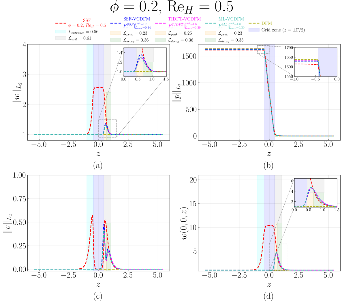
Figure D.117: Streamwise evolution of (a) \|w\|_{L_2} , (b) \|p\|_{L_2} , (c) \|v\|_{L_2} , and (d) centerline velocity w(0,0,z) for the 1 \times 1 SRG at \phi = 0.2 and \text{Re}_H = 0.5 . The figure compares the SSF, DFM, SSF-VCDFM, TIDFT-VCDFM, and ML-VCDFM. Shading marks the grid and the characteristic entrance, exit, peak, and decay regions. Only the SSF-based \mathcal{L}_{\text{peak}} and \mathcal{L}_{\text{decay}} are marked on the plot; the corresponding TIDFT-VCDFM and ML-VCDFM values appear in the legend.
