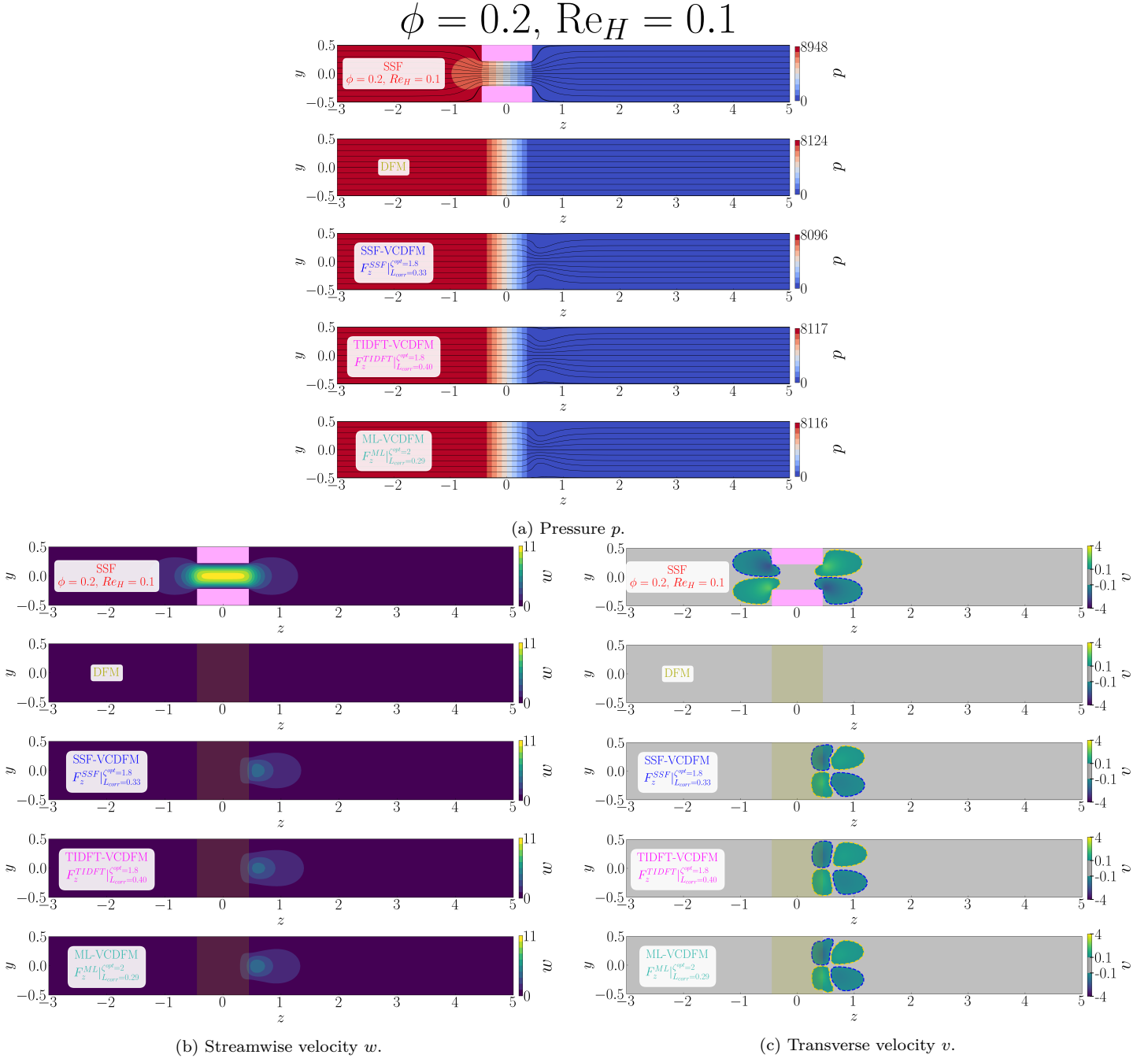
Figure D.112: Flow organization in the streamwise (z, y) -plane for the 1 \times 1 SRG at \phi = 0.2 , \text{Re}_H = 0.1 , and \alpha = 0^\circ . The blocks show (a) pressure p with streamlines, (b) streamwise velocity w , and (c) transverse velocity v . Within each block, the rows show, from top to bottom, the SSF, DFM, SSF-VCDFM, TIDFT-VCDFM, and ML-VCDFM. Pink shading marks the grid walls in the SSF; olive shading marks the equivalent porous zone in the model solutions.
