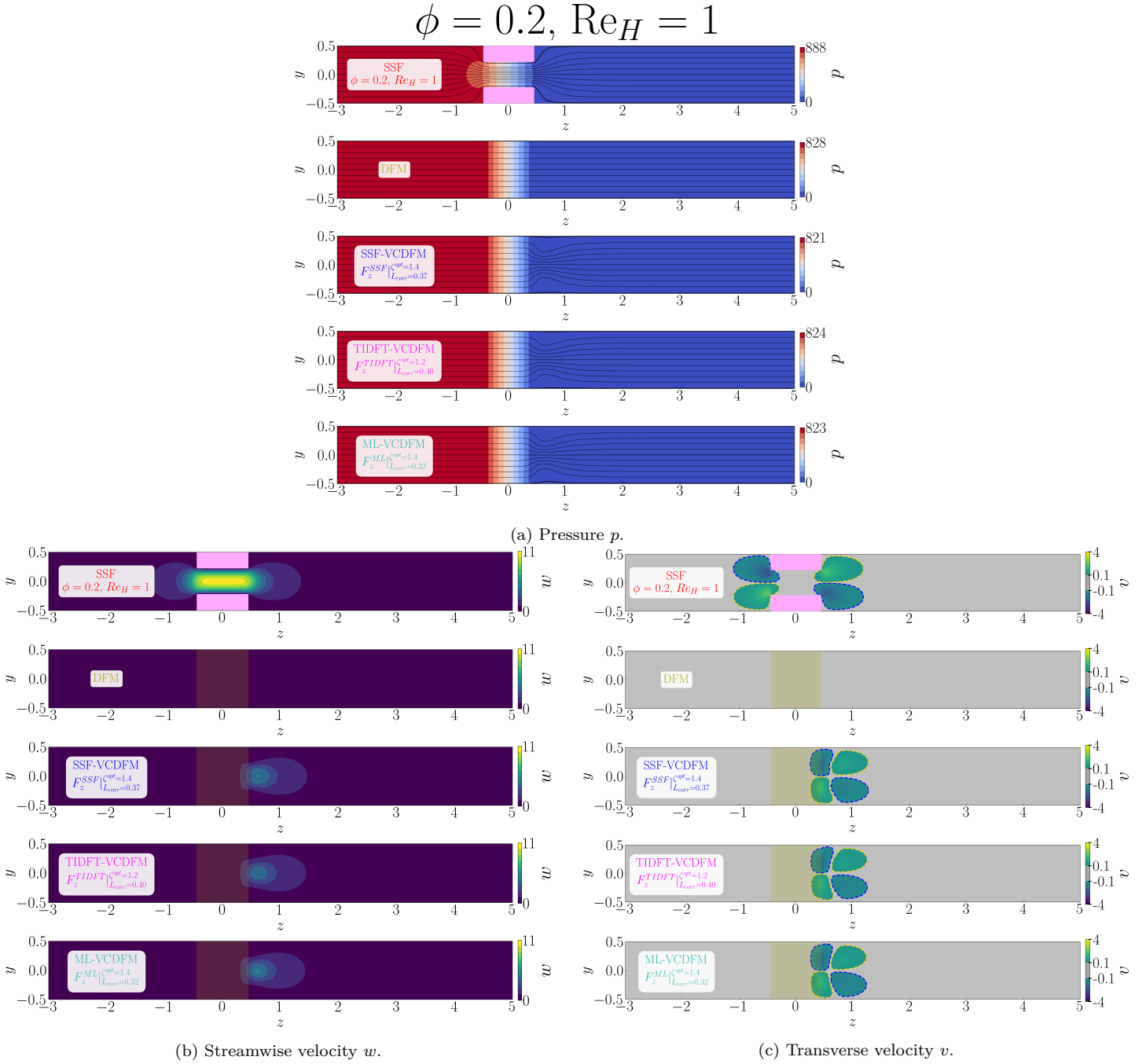
Figure D.124: Flow organization in the streamwise (z, y) -plane for the 1 \times 1 SRG at \phi = 0.2 , Re_H = 1 , and \alpha = 0^\circ . The blocks show (a) pressure p with streamlines, (b) streamwise velocity w , and (c) transverse velocity v . Within each block, the rows show, from top to bottom, the SSF, DFM, SSF-VCDFM, TIDFT-VCDFM, and ML-VCDFM. Pink shading marks the grid walls in the SSF; olive shading marks the equivalent porous zone in the model solutions.
