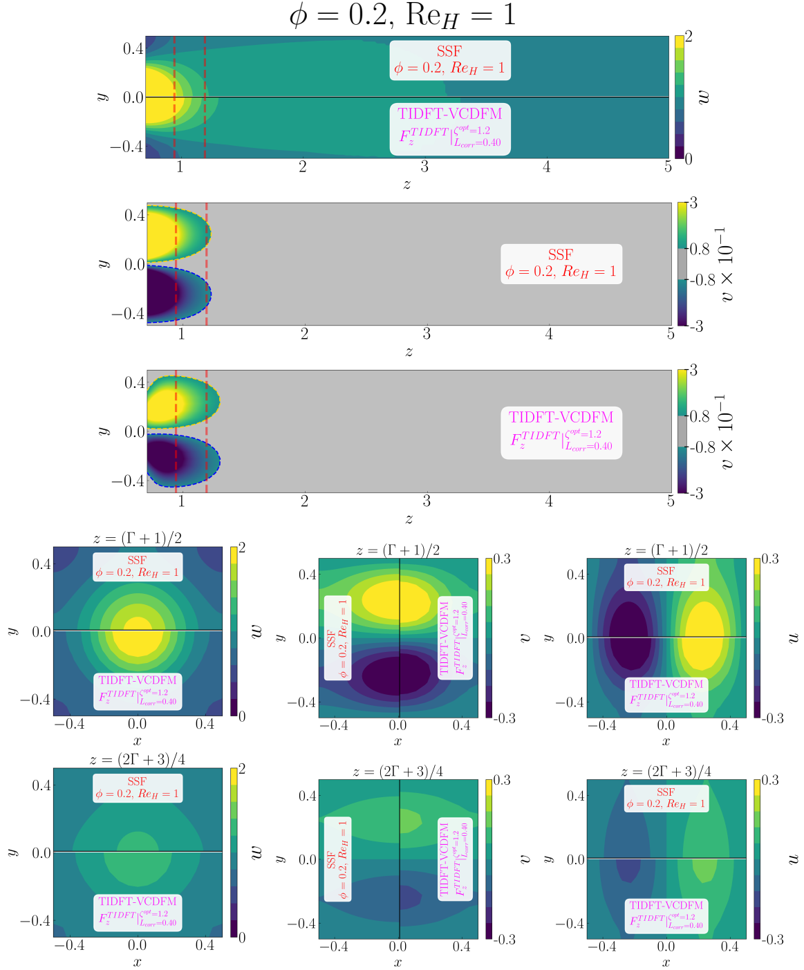
Figure D.127: Detailed comparison between the geometry-resolved small-scale flow (SSF) and TIDFT-VCDFM using F_z^{\text{TIDFT}} for the 1 \times 1 SRG at \phi = 0.2 and \text{Re}_H = 1 . The upper panels compare the streamwise velocity w and transverse velocity v in the central (z, y) -plane, restricted to the correction region. The lower panels compare the corresponding transverse (x, y) -plane distributions of w , v , and u , from left to right, at z = (\Gamma + 1)/2 in the first row and z = (2\Gamma + 3)/4 in the second row.
