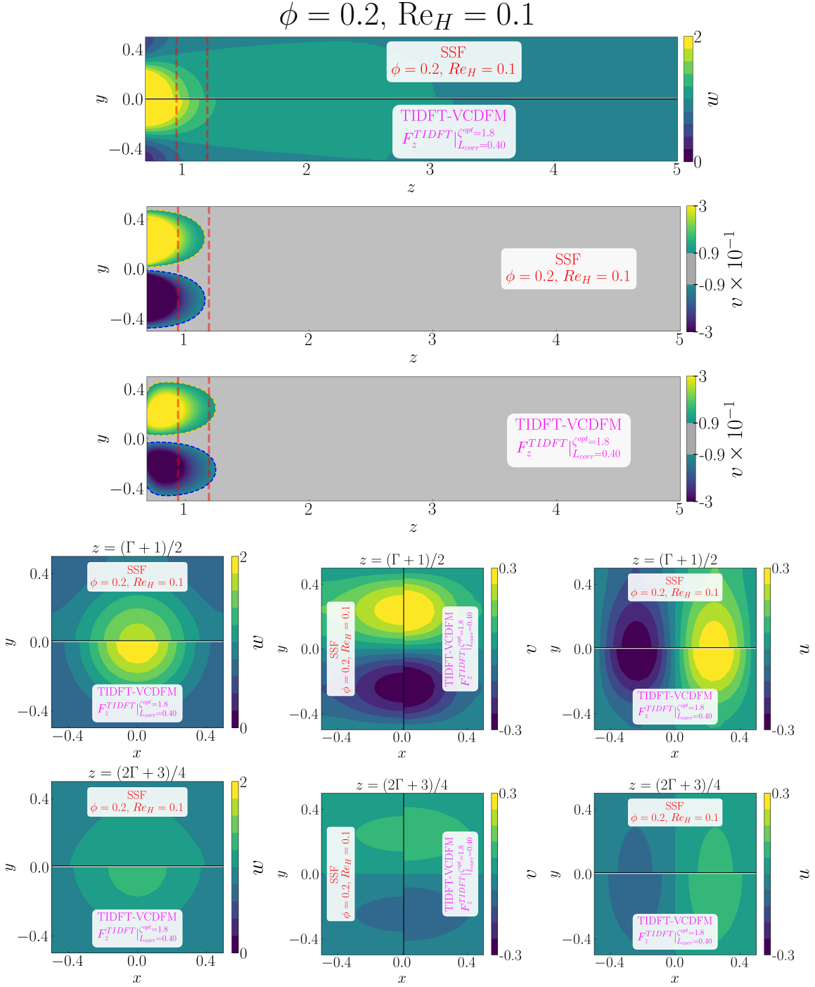
Figure D.115: Detailed comparison between the geometry-resolved small-scale flow (SSF) and TIDFT-VCDFM using F_z^{\text{TIDFT}} for the 1 \times 1 SRG at \phi = 0.2 and \text{Re}_H = 0.1 . The upper panels compare the streamwise velocity w and transverse velocity v in the central (z, y) -plane, restricted to the correction region. The lower panels compare the corresponding transverse (x, y) -plane distributions of w , v , and u , from left to right, at z = (\Gamma + 1)/2 in the first row and z = (2\Gamma + 3)/4 in the second row.
