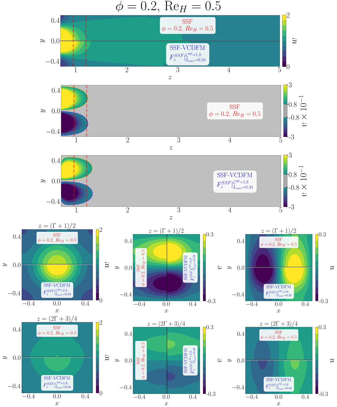
Figure D.120: Detailed comparison between the geometry-resolved small-scale flow (SSF) and SSF-VCDFM using F_z^{SSF} for the 1 \times 1 SRG at \phi = 0.2 and Re_H = 0.5 . The upper panels compare the streamwise velocity w and transverse velocity v in the central (z, y) -plane, restricted to the correction region. The lower panels compare the corresponding transverse (x, y) -plane distributions of w , v , and u , from left to right, at z = (\Gamma + 1)/2 in the first row and z = (2\Gamma + 3)/4 in the second row.
