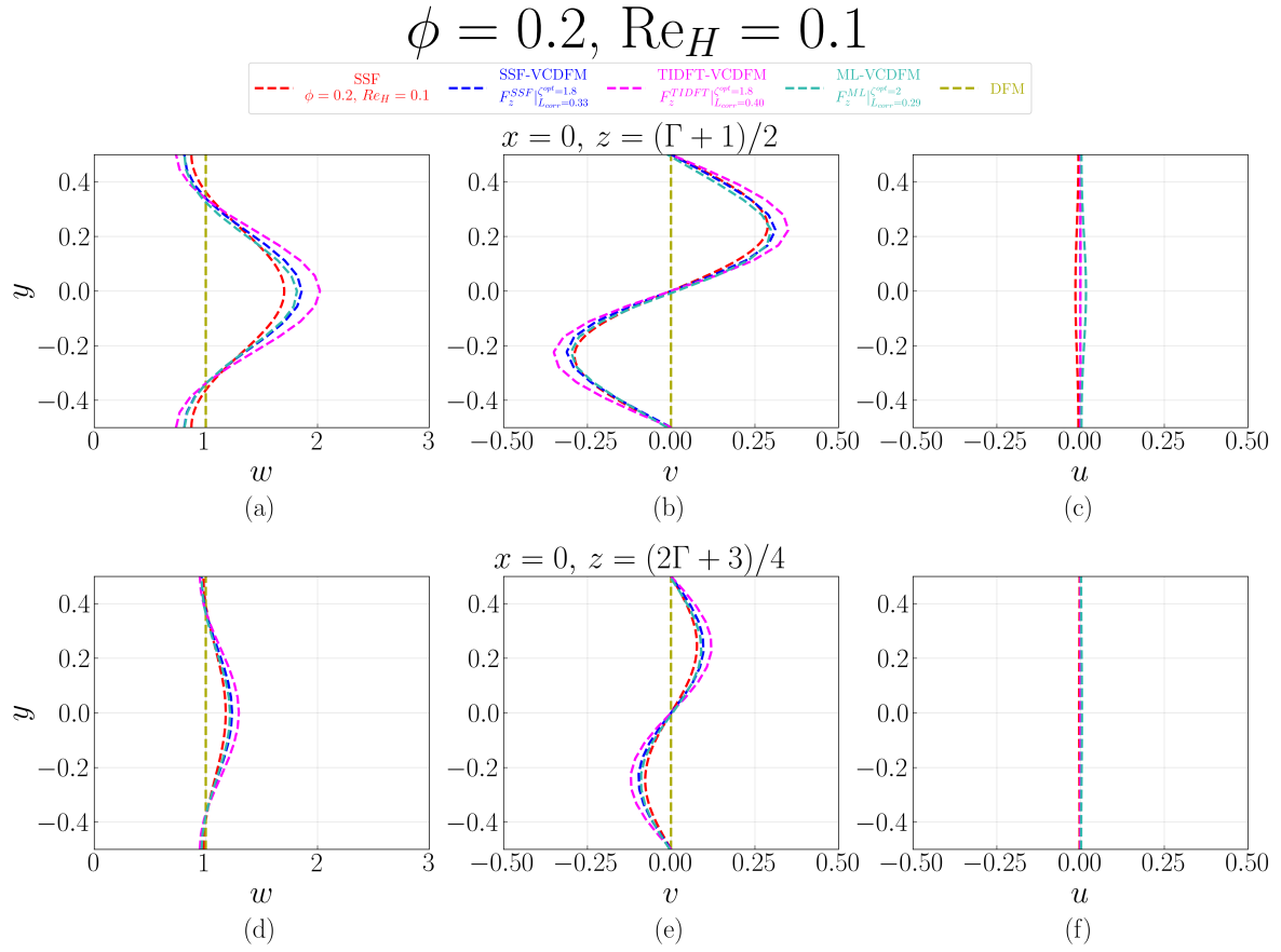
Figure D.113: Velocity profiles at x = 0 for the 1 \times 1 SRG at \phi = 0.2 and \text{Re}_H = 0.1 , comparing the SSF, DFM, SSF-VCDFM, TIDFT-VCDFM, and ML-VCDFM. Profiles of w(y) , v(y) , and u(y) are shown at z = (\Gamma + 1)/2 in (a–c) and z = (2\Gamma + 3)/4 in (d–f).
