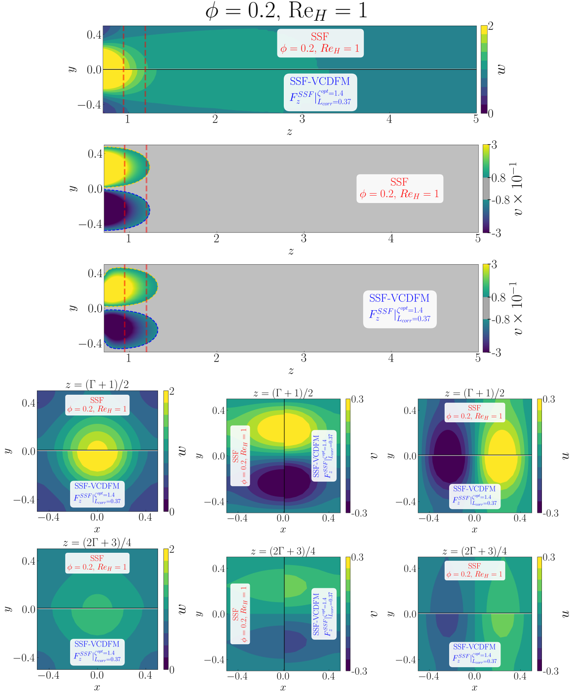
Figure D.126: Detailed comparison between the geometry-resolved small-scale flow (SSF) and SSF-VCDFM using F_z^{\text{SSF}} for the 1 \times 1 SRG at \phi = 0.2 and \text{Re}_H = 1 . The upper panels compare the streamwise velocity w and transverse velocity v in the central (z, y) -plane, restricted to the correction region. The lower panels compare the corresponding transverse (x, y) -plane distributions of w , v , and u , from left to right, at z = (\Gamma + 1)/2 in the first row and z = (2\Gamma + 3)/4 in the second row.
