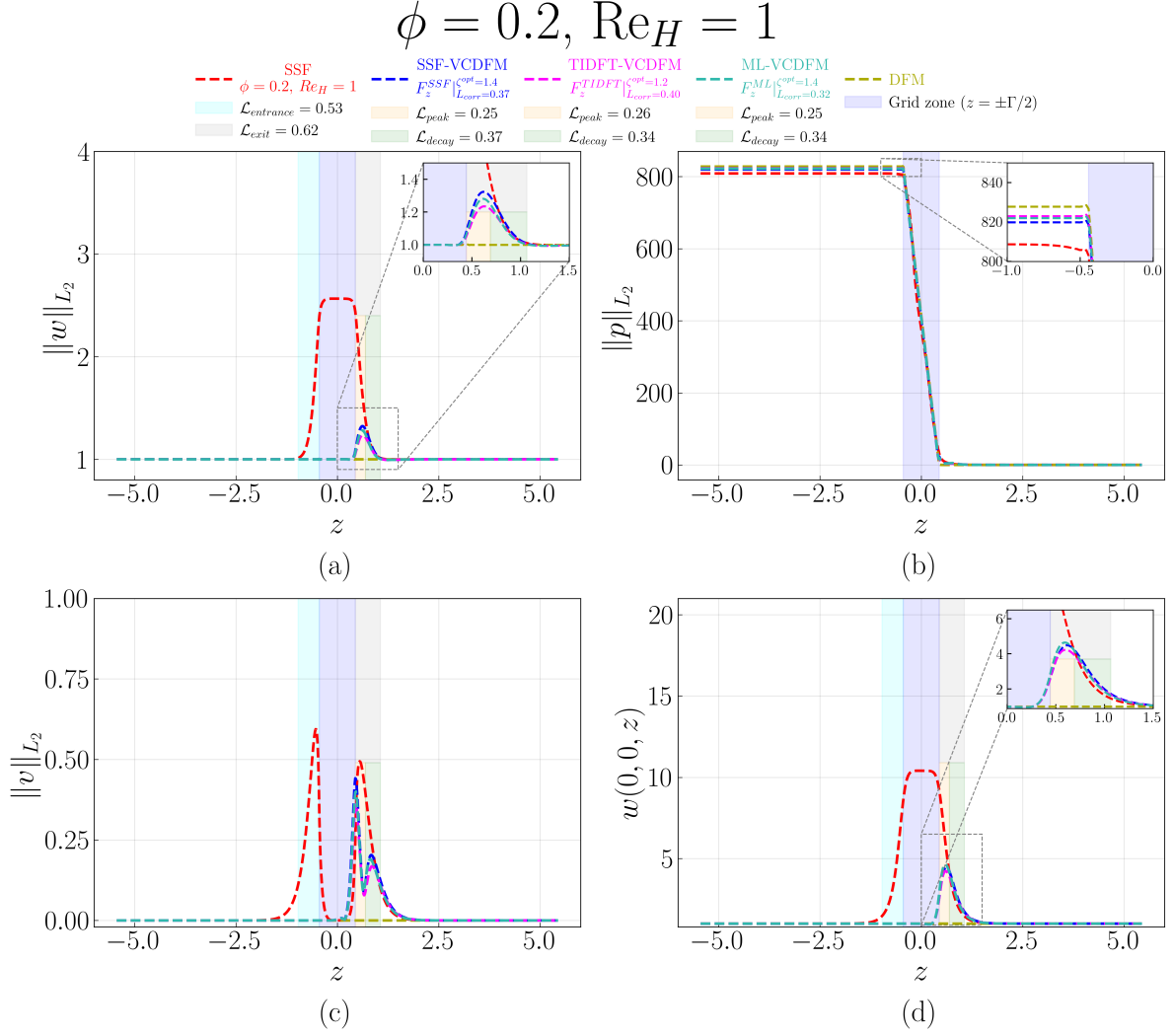
Figure D.123: Streamwise evolution of (a) \|w\|_{L_2} , (b) \|p\|_{L_2} , (c) \|v\|_{L_2} , and (d) centerline velocity w(0,0,z) for the 1 \times 1 SRG at \phi = 0.2 and \text{Re}_H = 1 . The figure compares the SSF, DFM, SSF-VCDFM, TIDFT-VCDFM, and ML-VCDFM. Shading marks the grid and the characteristic entrance, exit, peak, and decay regions. Only the SSF-based \mathcal{L}_{\text{peak}} and \mathcal{L}_{\text{decay}} are marked on the plot; the corresponding TIDFT-VCDFM and ML-VCDFM values appear in the legend.
