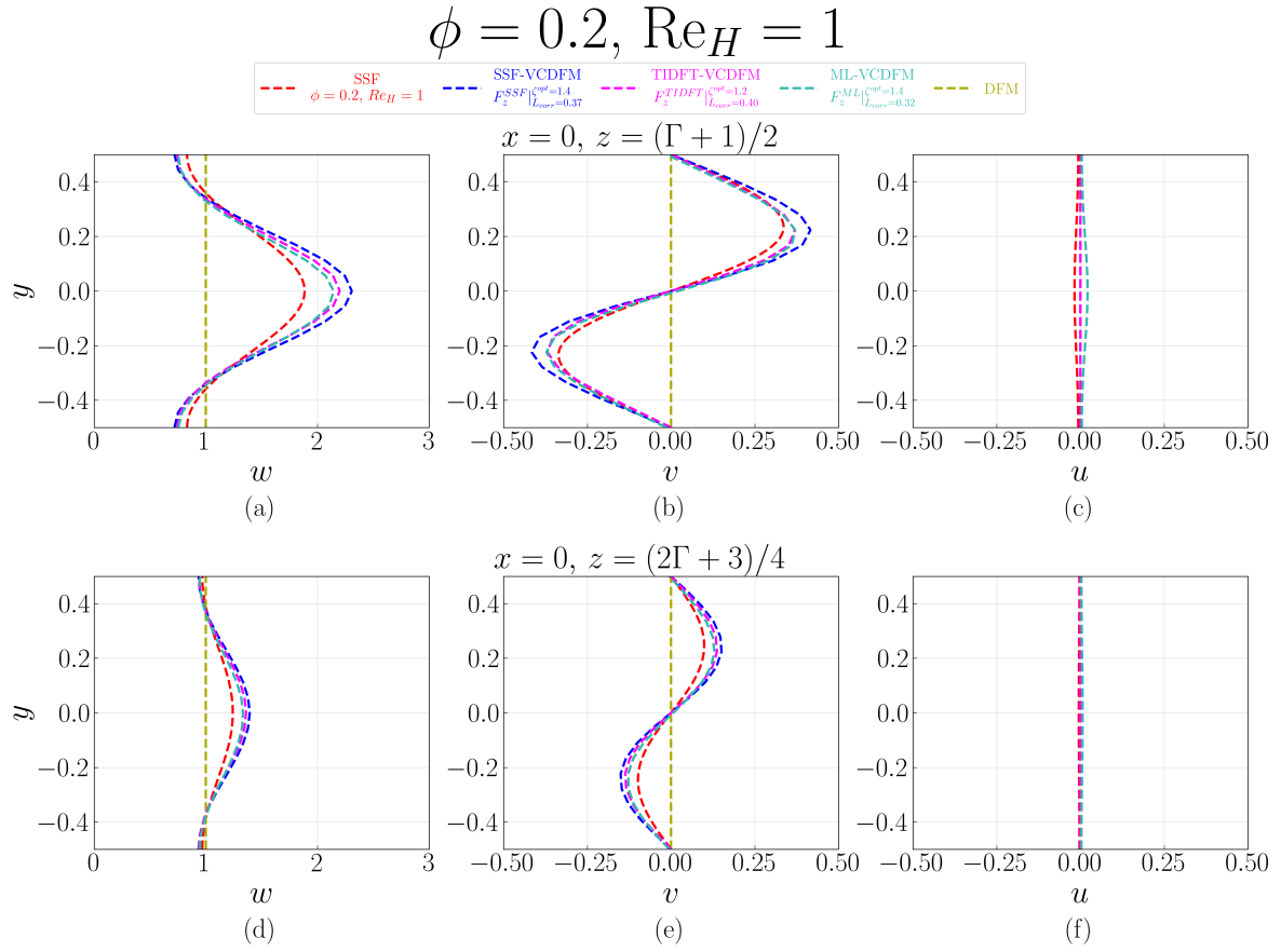
Figure D.125: Velocity profiles at x = 0 for the 1 \times 1 SRG at \phi = 0.2 and \text{Re}_H = 1 , comparing the SSF, DFM, SSF-VCDFM, TIDFT-VCDFM, and ML-VCDFM. Profiles of w(y) , v(y) , and u(y) are shown at z = (\Gamma + 1)/2 in (a–c) and z = (2\Gamma + 3)/4 in (d–f).
