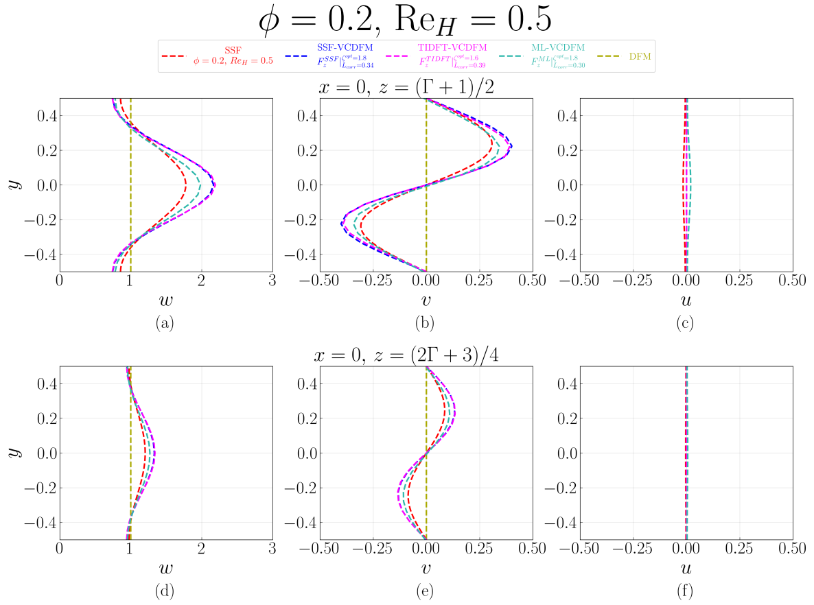
Figure D.119: Velocity profiles at x = 0 for the 1 \times 1 SRG at \phi = 0.2 and \text{Re}_H = 0.5 , comparing the SSF, DFM, SSF-VCDFM, TIDFT-VCDFM, and ML-VCDFM. Profiles of w(y) , v(y) , and u(y) are shown at z = (\Gamma + 1)/2 in (a–c) and z = (2\Gamma + 3)/4 in (d–f).
