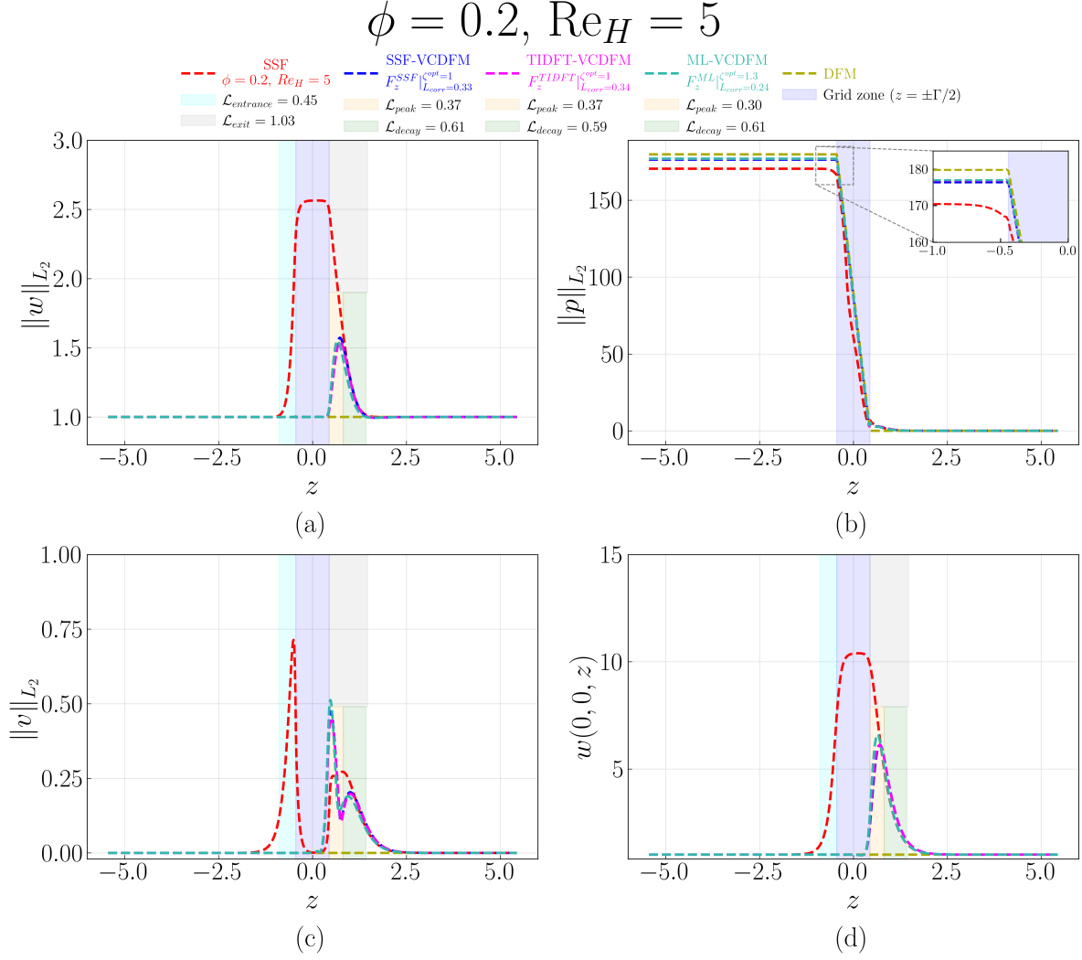
Figure D.129: Streamwise evolution of (a) \|w\|_{L_2} , (b) \|p\|_{L_2} , (c) \|v\|_{L_2} , and (d) centerline velocity w(0,0,z) for the 1 \times 1 SRG at \phi = 0.2 and \text{Re}_H = 5 . The figure compares the SSF, DFM, SSF-VCDFM, TIDFT-VCDFM, and ML-VCDFM. Shading marks the grid and the characteristic entrance, exit, peak, and decay regions. Only the SSF-based \mathcal{L}_{\text{peak}} and \mathcal{L}_{\text{decay}} are marked on the plot; the corresponding TIDFT-VCDFM and ML-VCDFM values appear in the legend.
