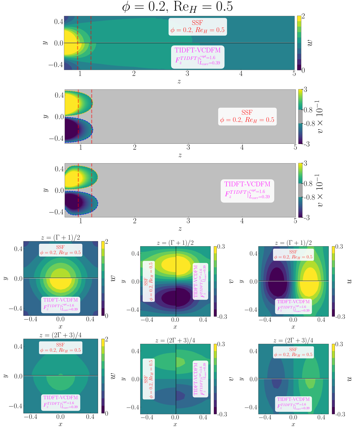
Figure D.121: Detailed comparison between the geometry-resolved small-scale flow (SSF) and TIDFT-VCDFM using F_z^{\text{TIDFT}} for the 1 \times 1 SRG at \phi = 0.2 and \text{Re}_H = 0.5 . The upper panels compare the streamwise velocity w and transverse velocity v in the central (z, y) -plane, restricted to the correction region. The lower panels compare the corresponding transverse (x, y) -plane distributions of w , v , and u , from left to right, at z = (\Gamma + 1)/2 in the first row and z = (2\Gamma + 3)/4 in the second row.
