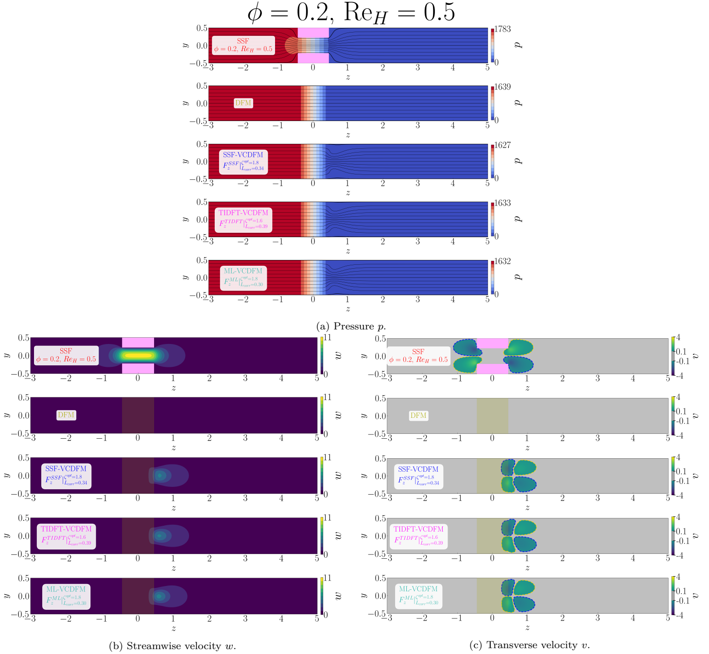
Figure D.118: Flow organization in the streamwise (z, y) -plane for the 1 \times 1 SRG at \phi = 0.2 , \text{Re}_H = 0.5 , and \alpha = 0^\circ . The blocks show (a) pressure p with streamlines, (b) streamwise velocity w , and (c) transverse velocity v . Within each block, the rows show, from top to bottom, the SSF, DFM, SSF-VCDFM, TIDFT-VCDFM, and ML-VCDFM. Pink shading marks the grid walls in the SSF; olive shading marks the equivalent porous zone in the model solutions.
