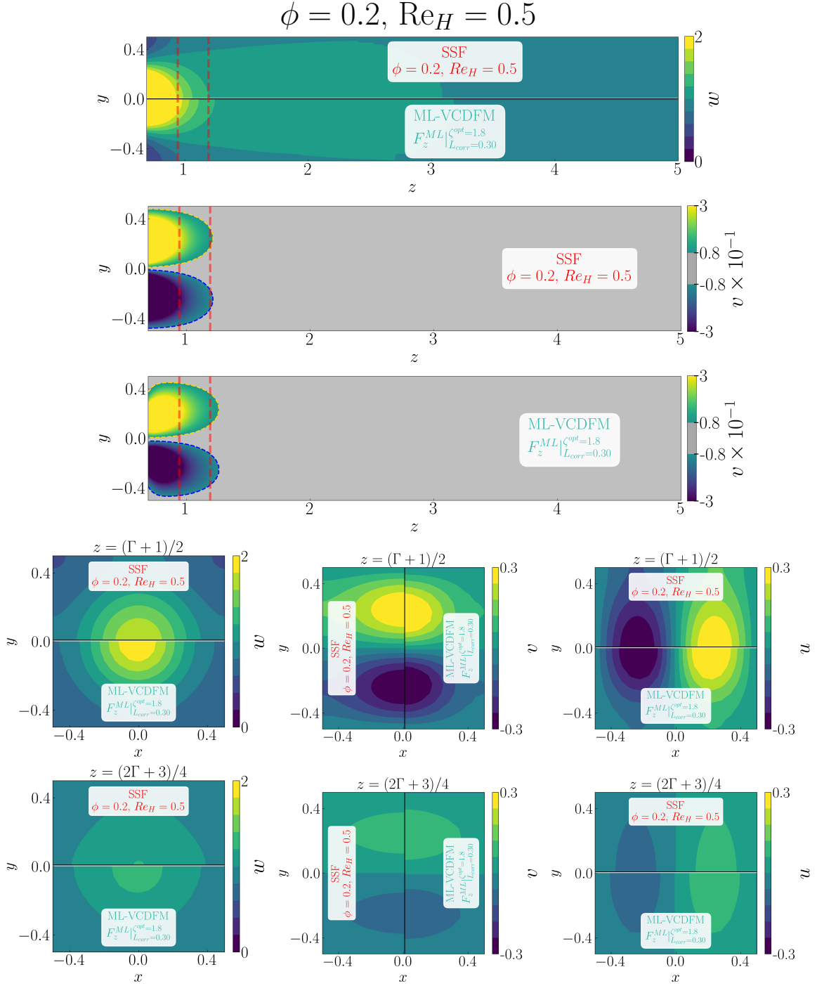
Figure D.122: Detailed comparison between the geometry-resolved small-scale flow (SSF) and ML-VCDM using F_z^{ML} for the 1 \times 1 SRG at \phi = 0.2 and Re_H = 0.5 . The upper panels compare the streamwise velocity w and transverse velocity v in the central (z, y) -plane, restricted to the correction region. The lower panels compare the corresponding transverse (x, y) -plane distributions of w , v , and u , from left to right, at z = (\Gamma + 1)/2 in the first row and z = (2\Gamma + 3)/4 in the second row.
