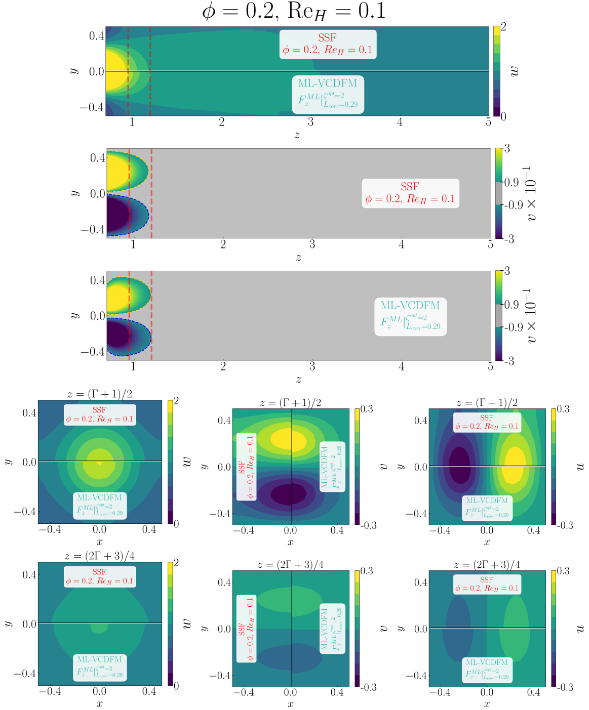
Figure D.116: Detailed comparison between the geometry-resolved small-scale flow (SSF) and ML-VCDFM using F_z^{\text{ML}} for the 1 \times 1 SRG at \phi = 0.2 and Re_H = 0.1 . The upper panels compare the streamwise velocity w and transverse velocity v in the central (z, y) -plane, restricted to the correction region. The lower panels compare the corresponding transverse (x, y) -plane distributions of w , v , and u , from left to right, at z = (\Gamma + 1)/2 in the first row and z = (2\Gamma + 3)/4 in the second row.
