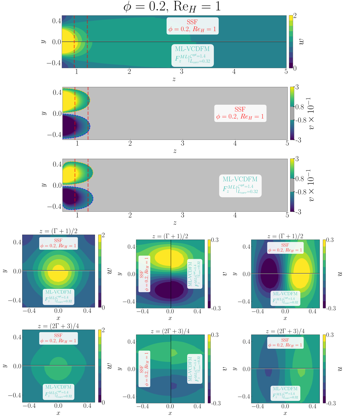
Figure D.128: Detailed comparison between the geometry-resolved small-scale flow (SSF) and ML-VCDFM using F_z^{\text{ML}} for the 1 \times 1 SRG at \phi = 0.2 and \text{Re}_H = 1 . The upper panels compare the streamwise velocity w and transverse velocity v in the central (z, y) -plane, restricted to the correction region. The lower panels compare the corresponding transverse (x, y) -plane distributions of w , v , and u , from left to right, at z = (\Gamma + 1)/2 in the first row and z = (2\Gamma + 3)/4 in the second row.
