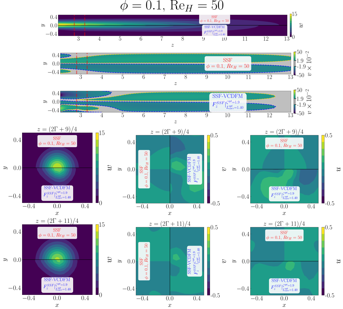
Figure D.227: Detailed comparison between the geometry-resolved small-scale flow (SSF) and SSF-VCDFM using F_z^{SSF} for the 1 \times 1 SRG at \phi = 0.1 and Re_H = 50 . The upper panels compare the streamwise velocity w and transverse velocity v in the central (z, y) -plane, restricted to the correction region. The lower panels compare the corresponding transverse (x, y) -plane distributions of w , v , and u , from left to right, at z = (2\Gamma + 9)/4 in the first row and z = (2\Gamma + 11)/4 in the second row.
