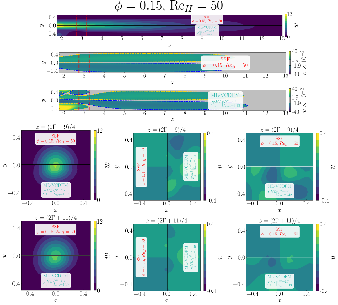
Figure D.240: Detailed comparison between the geometry-resolved small-scale flow (SSF) and ML-VCDFM using F_z^{\text{ML}} for the 1 \times 1 SRG at \phi = 0.15 and Re_H = 50 . The upper panels compare the streamwise velocity w and transverse velocity v in the central (z, y) -plane, restricted to the correction region. The lower panels compare the corresponding transverse (x, y) -plane distributions of w , v , and u , from left to right, at z = (2\Gamma + 9)/4 in the first row and z = (2\Gamma + 11)/4 in the second row.
