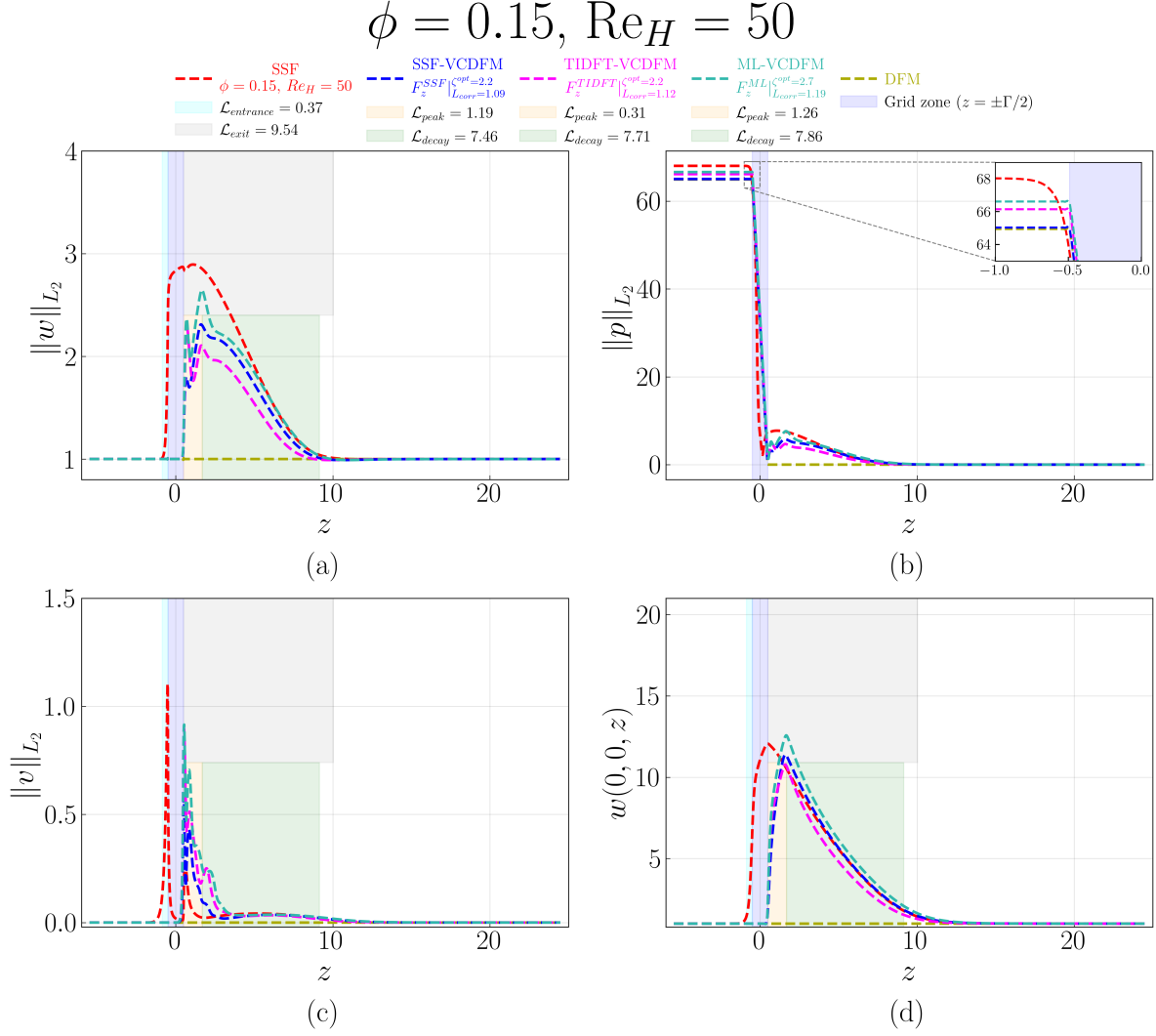
Figure D.235: Streamwise evolution of (a) \|w\|_{L_2} , (b) \|p\|_{L_2} , (c) \|v\|_{L_2} , and (d) centerline velocity w(0,0,z) for the 1 \times 1 SRG at \phi = 0.15 and \text{Re}_H = 50 . The figure compares the SSF, DFM, SSF-VCDFM, TIDFT-VCDFM, and ML-VCDFM. Shading marks the grid and the characteristic entrance, exit, peak, and decay regions. Only the SSF-based \mathcal{L}_{\text{peak}} and \mathcal{L}_{\text{decay}} are marked on the plot; the corresponding TIDFT-VCDFM and ML-VCDFM values appear in the legend.
