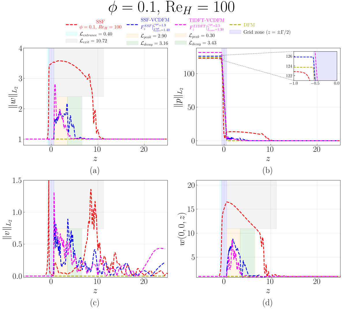
Figure D.230: Streamwise evolution of (a) \|w\|_{L_2} , (b) \|p\|_{L_2} , (c) \|v\|_{L_2} , and (d) centerline velocity w(0, 0, z) for the 1 \times 1 SRG at \phi = 0.1 and \text{Re}_H = 100 . The figure compares the SSF, DFM, SSF-VCDFM, and TIDFT-VCDFM. Shading marks the grid and the characteristic entrance, exit, peak, and decay regions. Only the SSF-based L_{\text{peak}} and L_{\text{decay}} are marked on the plot; the corresponding TIDFT-VCDFM values appear in the legend.
