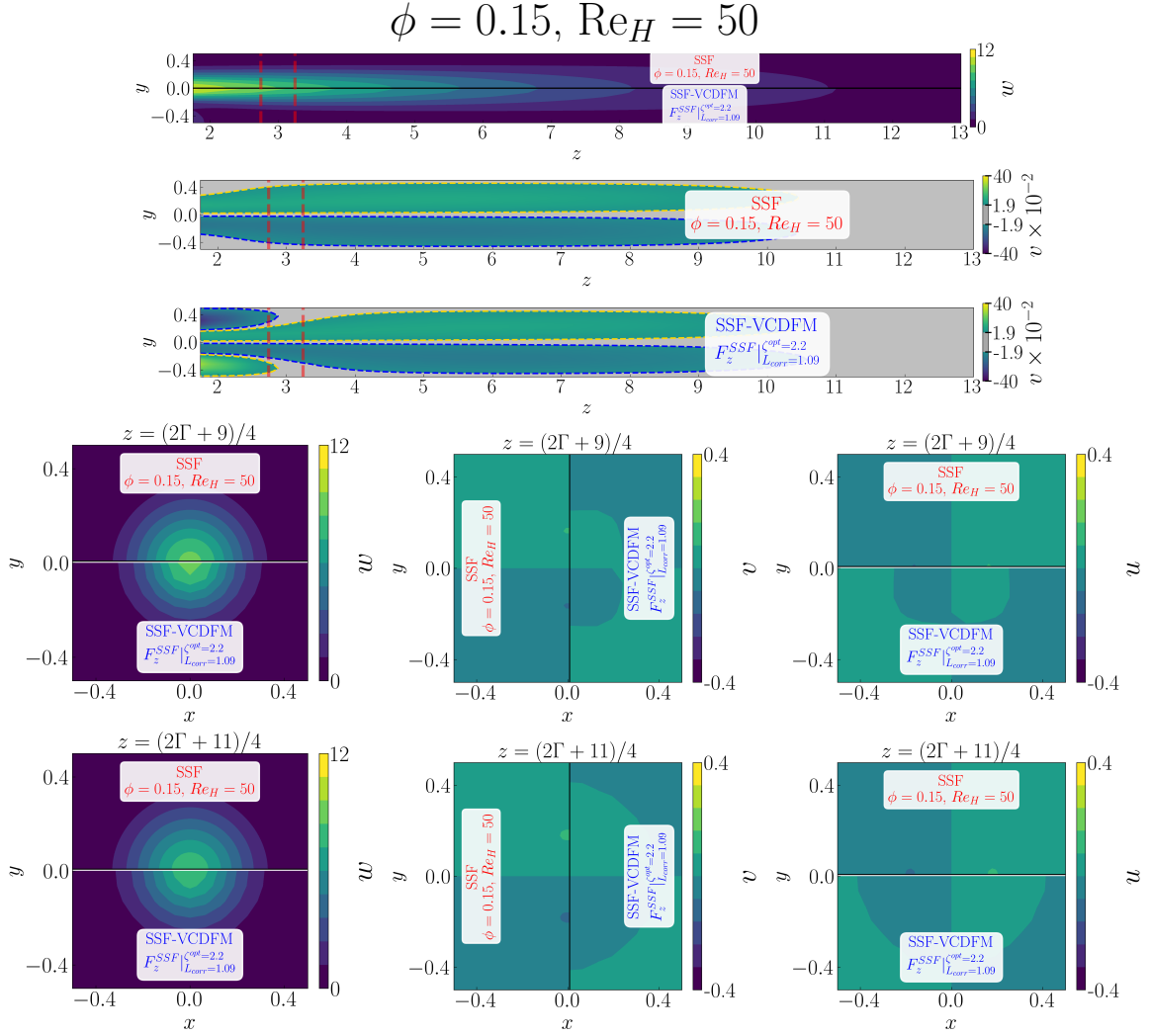
Figure D.238: Detailed comparison between the geometry-resolved small-scale flow (SSF) and SSF-VCDFM using F_z^{SSF} for the 1 \times 1 SRG at \phi = 0.15 and Re_H = 50 . The upper panels compare the streamwise velocity w and transverse velocity v in the central (z, y) -plane, restricted to the correction region. The lower panels compare the corresponding transverse (x, y) -plane distributions of w , v , and u , from left to right, at z = (2\Gamma + 9)/4 in the first row and z = (2\Gamma + 11)/4 in the second row.
