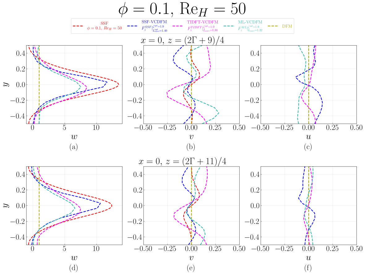
Figure D.226: Velocity profiles at x = 0 for the 1 \times 1 SRG at \phi = 0.1 and \text{Re}_H = 50 , comparing the SSF, DFM, SSF-VCDFM, TIDFT-VCDFM, and ML-VCDFM. Profiles of w(y) , v(y) , and u(y) are shown at z = (2\Gamma + 9)/4 in (a–c) and z = (2\Gamma + 11)/4 in (d–f).
