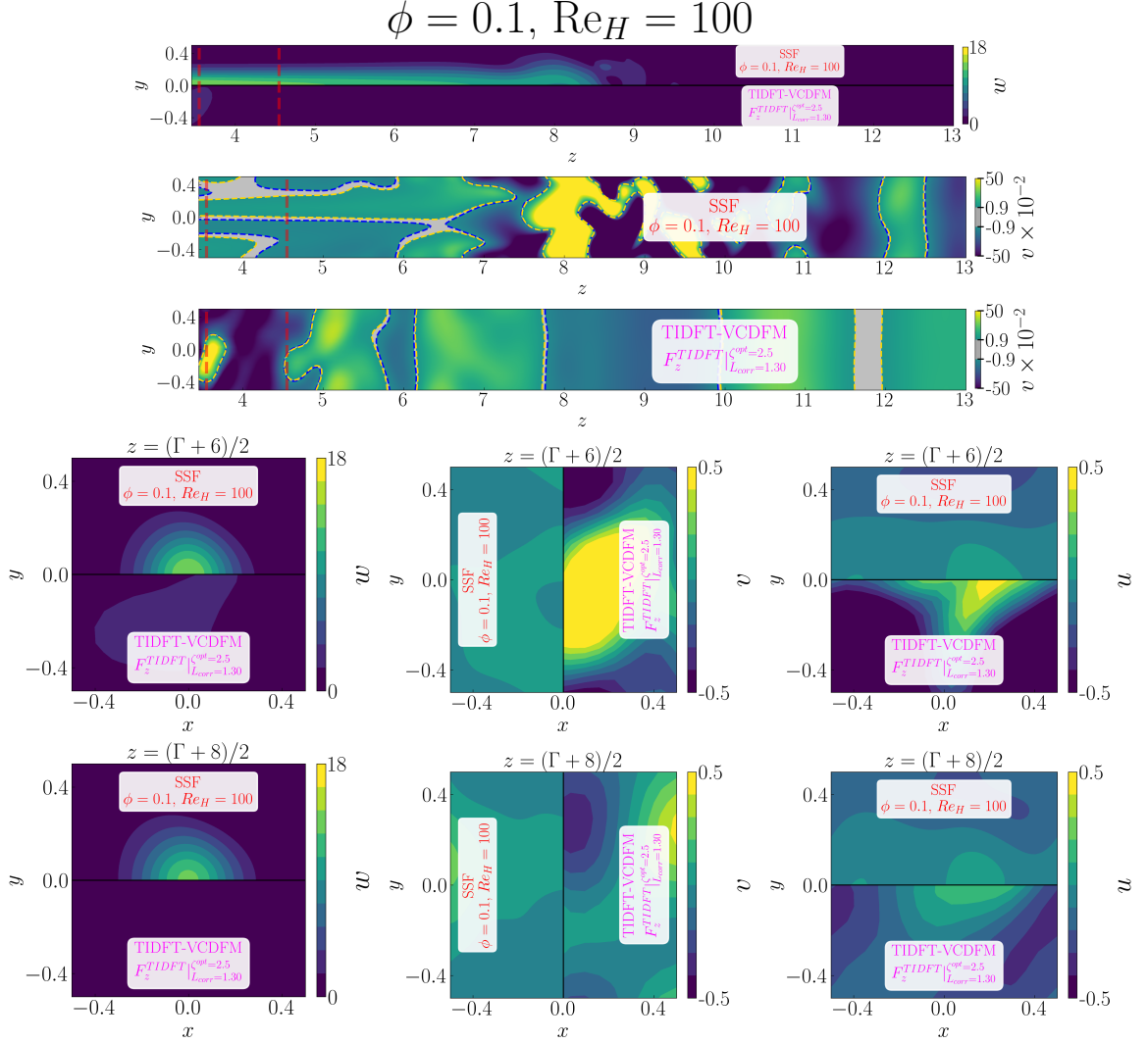
Figure D.234: Detailed comparison between the geometry-resolved small-scale flow (SSF) and TIDFT-VCDFM using F_z^{\text{TIDFT}} for the 1 \times 1 SRG at \phi = 0.1 and Re_H = 100 . The upper panels compare the downstream flow in the central (z, y) -plane, restricted to the correction region. The lower panels compare the corresponding transverse (x, y) -plane distributions at z = (\Gamma + 6)/2 and z = (\Gamma + 8)/2 .
