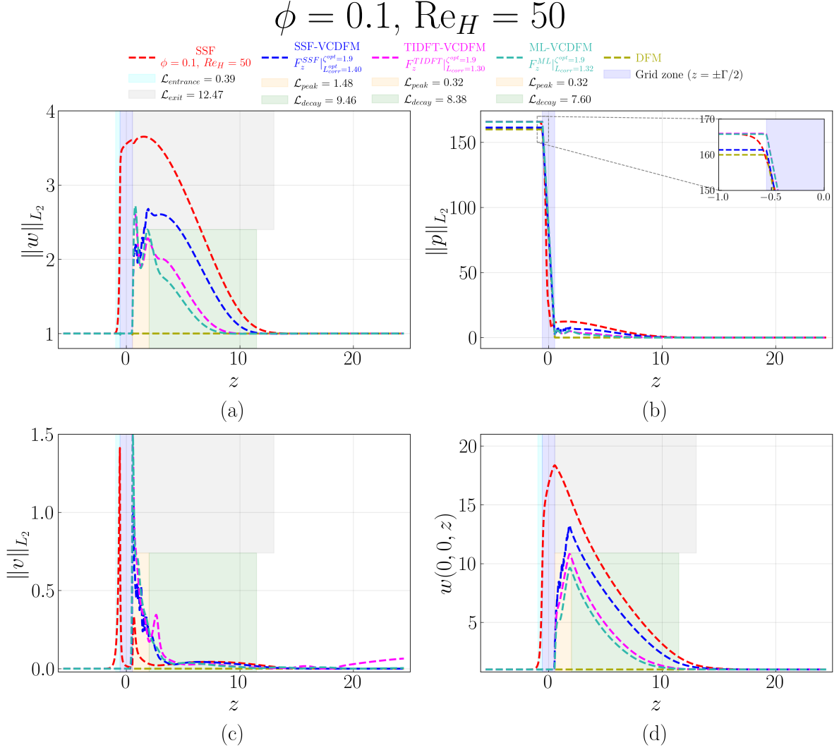
Figure D.224: Streamwise evolution of (a) \|w\|_{L_2} , (b) \|p\|_{L_2} , (c) \|v\|_{L_2} , and (d) centerline velocity w(0,0,z) for the 1 \times 1 SRG at \phi = 0.1 and \text{Re}_H = 50 . The figure compares the SSF, DFM, SSF-VCDFM, TIDFT-VCDFM, and ML-VCDFM. Shading marks the grid and the characteristic entrance, exit, peak, and decay regions. Only the SSF-based \mathcal{L}_{\text{peak}} and \mathcal{L}_{\text{decay}} are marked on the plot; the corresponding TIDFT-VCDFM and ML-VCDFM values appear in the legend.
