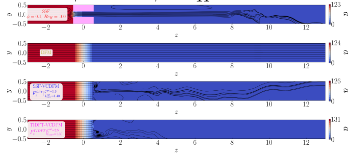
(a) Pressure p .
