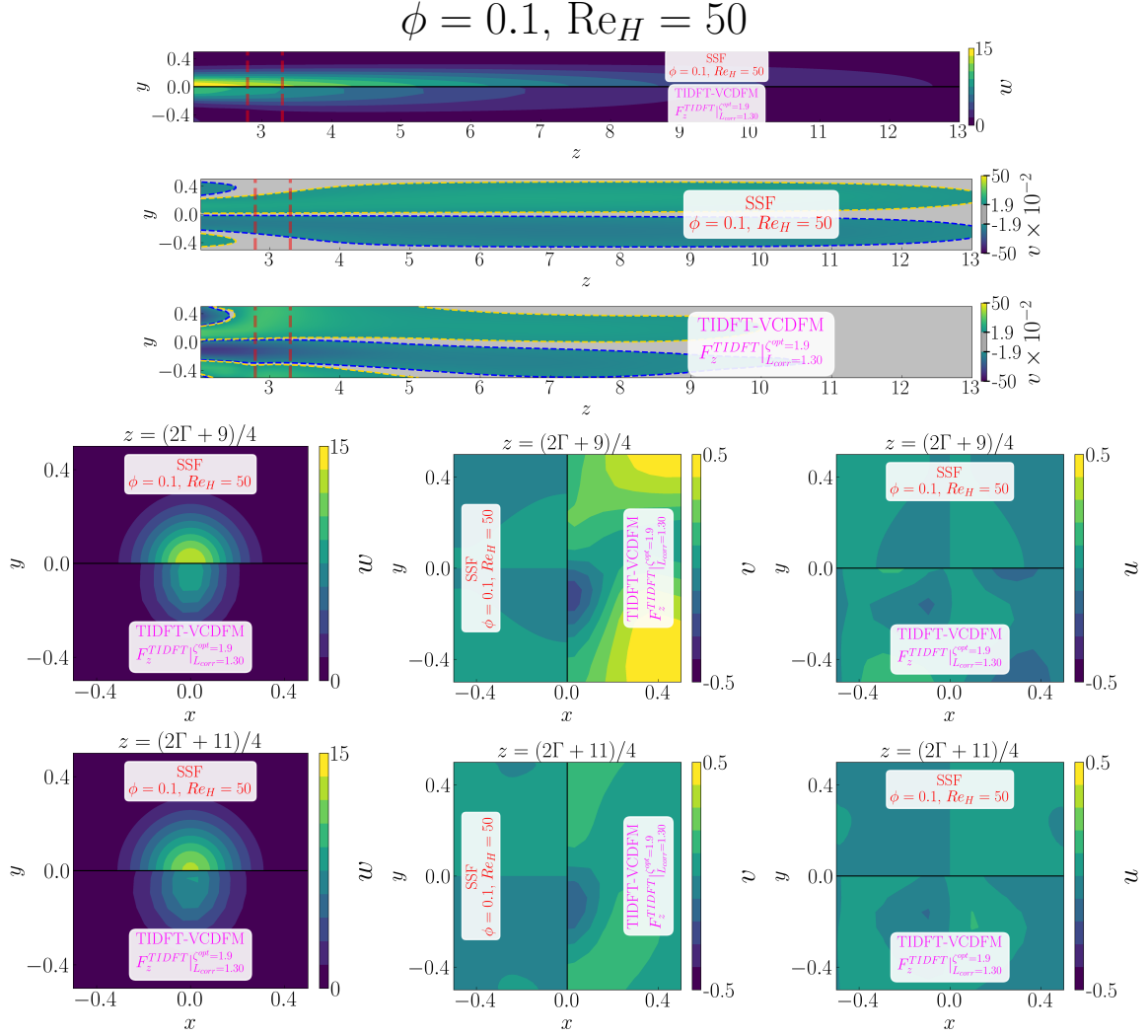
Figure D.228: Detailed comparison between the geometry-resolved small-scale flow (SSF) and TIDFT-VCDFM using F_z^{\text{TIDFT}} for the 1 \times 1 SRG at \phi = 0.1 and Re_H = 50 . The upper panels compare the streamwise velocity w and transverse velocity v in the central (z, y) -plane, restricted to the correction region. The lower panels compare the corresponding transverse (x, y) -plane distributions of w , v , and u , from left to right, at z = (2\Gamma + 9)/4 in the first row and z = (2\Gamma + 11)/4 in the second row.
