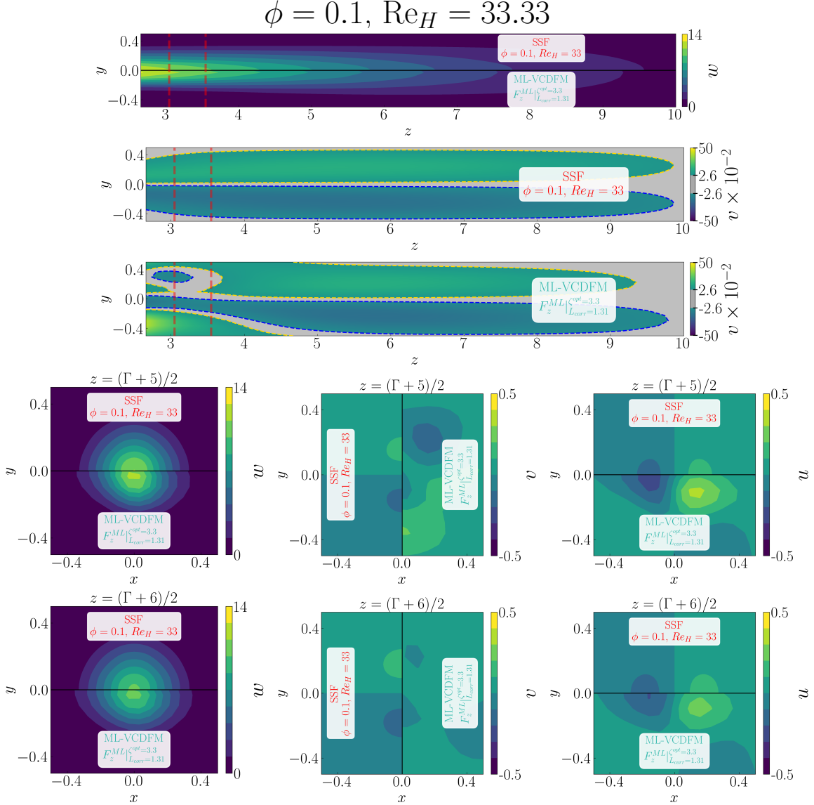
Figure D.223: Detailed comparison between the geometry-resolved small-scale flow (SSF) and ML-VCDFM using F_z^{\text{ML}} for the 1 \times 1 SRG at \phi = 0.1 and Re_H = 33.33 . The upper panels compare the streamwise velocity w and transverse velocity v in the central (z, y) -plane, restricted to the correction region. The lower panels compare the corresponding transverse (x, y) -plane distributions of w , v , and u , from left to right, at z = (\Gamma + 5)/2 in the first row and z = (\Gamma + 6)/2 in the second row.
