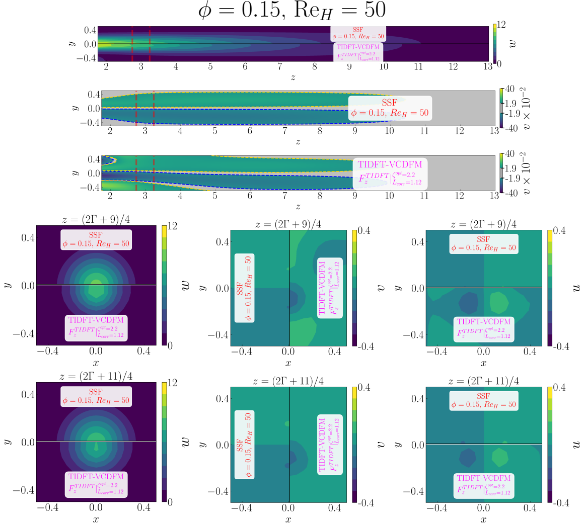
Figure D.239: Detailed comparison between the geometry-resolved small-scale flow (SSF) and TIDFT-VCDFM using F_z^{TIDFT} for the 1 \times 1 SRG at \phi = 0.15 and Re_H = 50 . The upper panels compare the streamwise velocity w and transverse velocity v in the central (z, y) -plane, restricted to the correction region. The lower panels compare the corresponding transverse (x, y) -plane distributions of w , v , and u , from left to right, at z = (2\Gamma + 9)/4 in the first row and z = (2\Gamma + 11)/4 in the second row.
