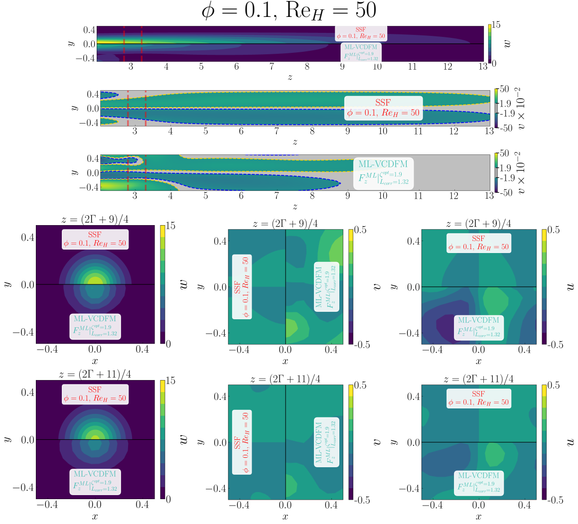
Figure D.229: Detailed comparison between the geometry-resolved small-scale flow (SSF) and ML-VCDFM using F_z^{\text{ML}} for the 1 \times 1 SRG at \phi = 0.1 and \text{Re}_H = 50 . The upper panels compare the streamwise velocity w and transverse velocity v in the central (z, y) -plane, restricted to the correction region. The lower panels compare the corresponding transverse (x, y) -plane distributions of w , v , and u , from left to right, at z = (2\Gamma + 9)/4 in the first row and z = (2\Gamma + 11)/4 in the second row.
