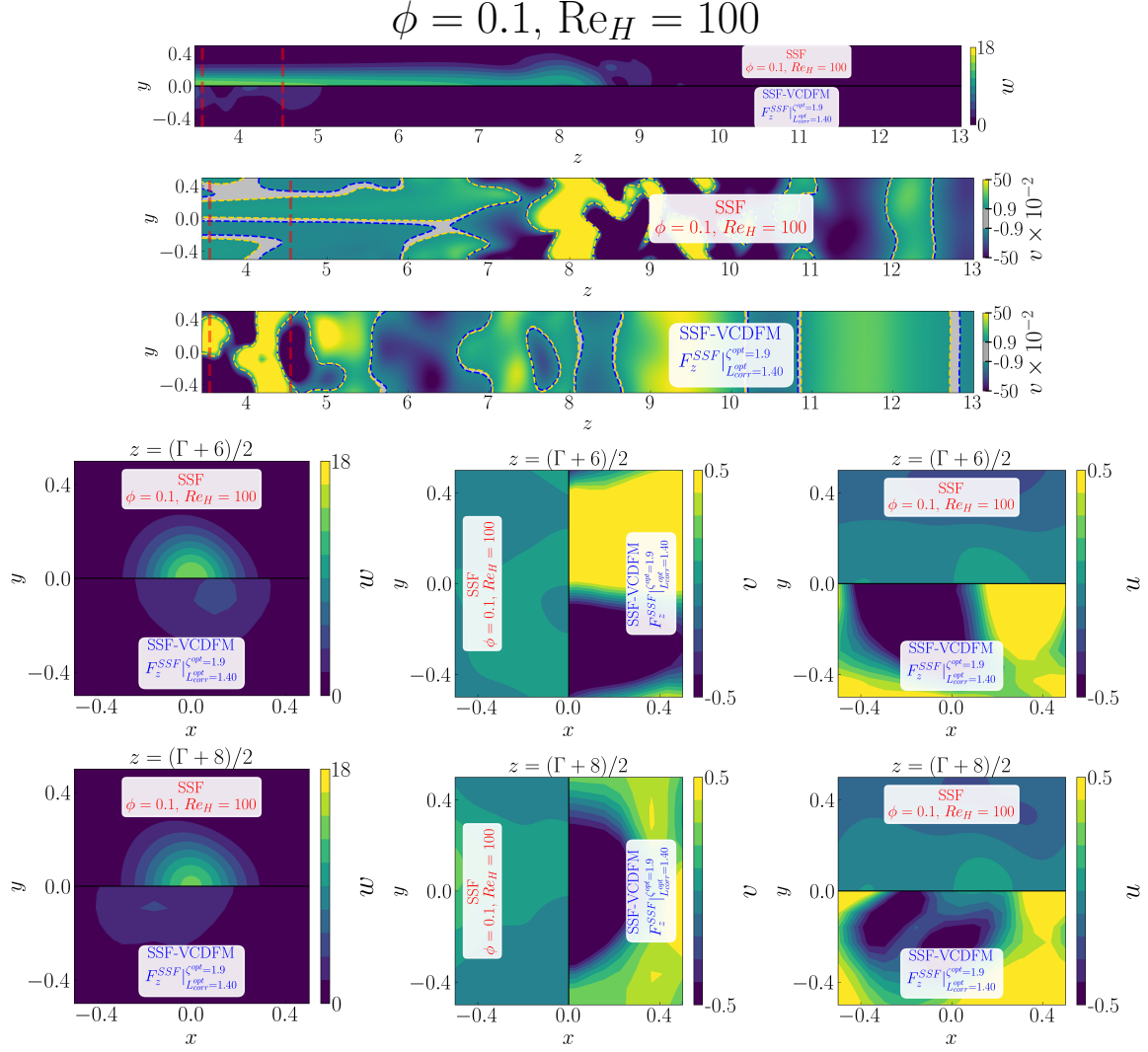
Figure D.233: Detailed comparison between the geometry-resolved small-scale flow (SSF) and SSF-VCDFM using F_z^{\text{SSF}} for the 1 \times 1 SRG at \phi = 0.1 and \text{Re}_H = 100 . The upper panels show the downstream flow in the streamwise (z, y) -plane, restricted to the correction region. The lower panels show the corresponding transverse (x, y) -plane distributions at z = (\Gamma + 6)/2 and z = (\Gamma + 8)/2 .
