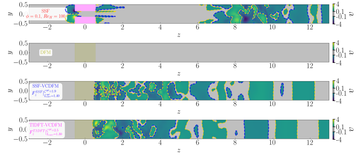
(c) Transverse velocity v .
