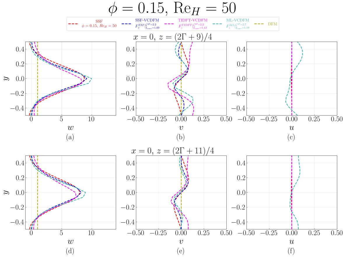
Figure D.237: Velocity profiles at x = 0 for the 1 \times 1 SRG at \phi = 0.15 and \text{Re}_H = 50 , comparing the SSF, DFM, SSF-VCDFM, TIDFT-VCDFM, and ML-VCDFM. Profiles of w(y) , v(y) , and u(y) are shown at z = (2\Gamma + 9)/4 in (a–c) and z = (2\Gamma + 11)/4 in (d–f).
