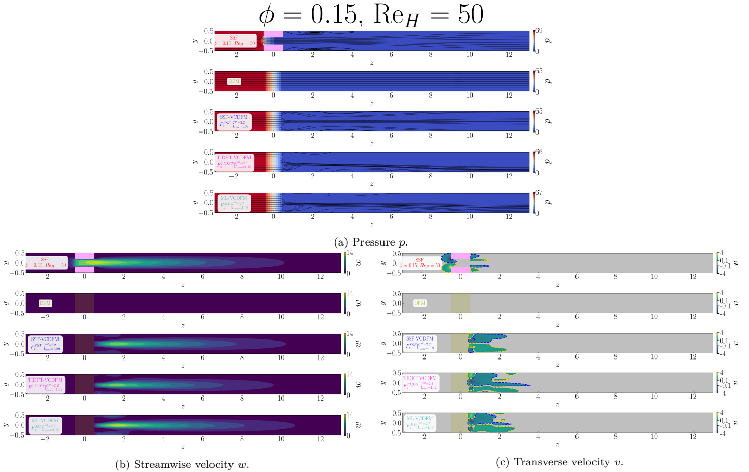
Figure D.236: Flow organization in the streamwise (z, y) -plane for the 1 \times 1 SRG at \phi = 0.15 , \text{Re}_H = 50 , and \alpha = 0^\circ . The blocks show (a) pressure p with streamlines, (b) streamwise velocity w , and (c) transverse velocity v . Within each block, the rows show, from top to bottom, the SSF, DFM, SSF-VCDFM, TIDFT-VCDFM, and ML-VCDFM. Pink shading marks the grid walls in the SSF; olive shading marks the equivalent porous zone in the model solutions.
