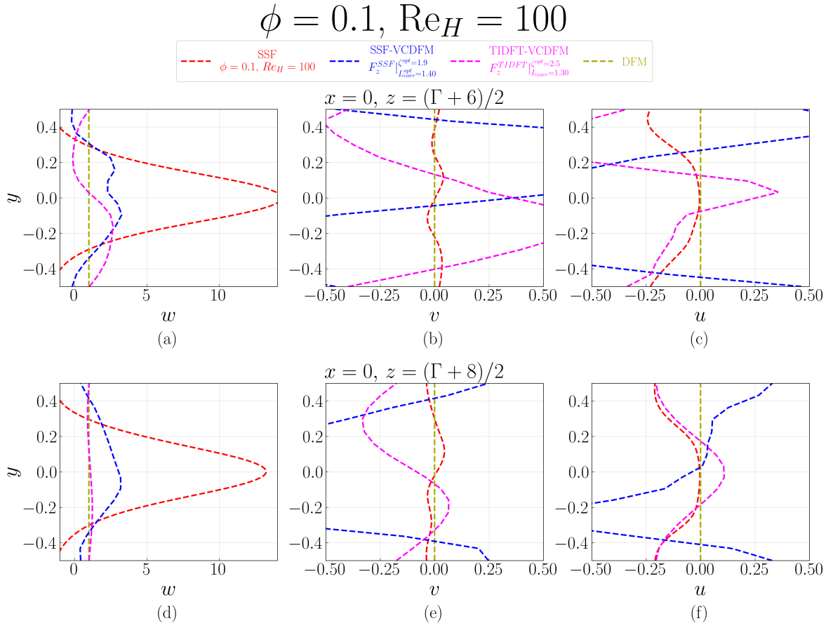
Figure D.232: Velocity profiles at x = 0 for the 1 \times 1 SRG at \phi = 0.1 and \text{Re}_H = 100 , comparing the SSF, DFM, SSF-VCDFM, and TIDFT-VCDFM. Profiles of w(y) , v(y) , and u(y) are shown at z = (\Gamma + 6)/2 in (a-c) and z = (\Gamma + 8)/2 in (d-f).
