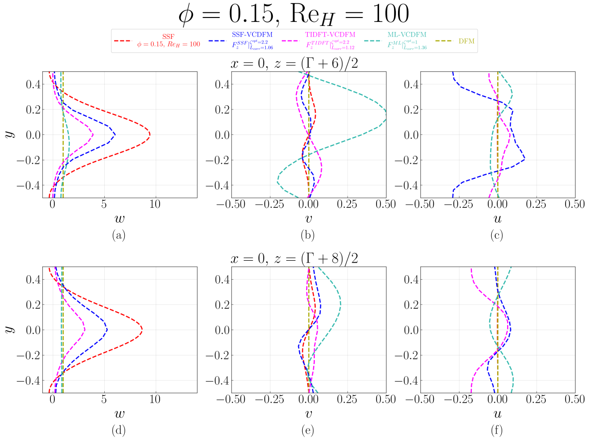
Figure D.259: Velocity profiles at x = 0 for the 1 \times 1 SRG at \phi = 0.15 and \text{Re}_H = 100 , comparing the SSF, DFM, SSF-VCDFM, TIDFT-VCDFM, and ML-VCDFM. Profiles of w(y) , v(y) , and u(y) are shown at z = (\Gamma + 6)/2 in (a–c) and z = (\Gamma + 8)/2 in (d–f). ML-VCDFM is evaluated outside the Reynolds-number range used for training.
