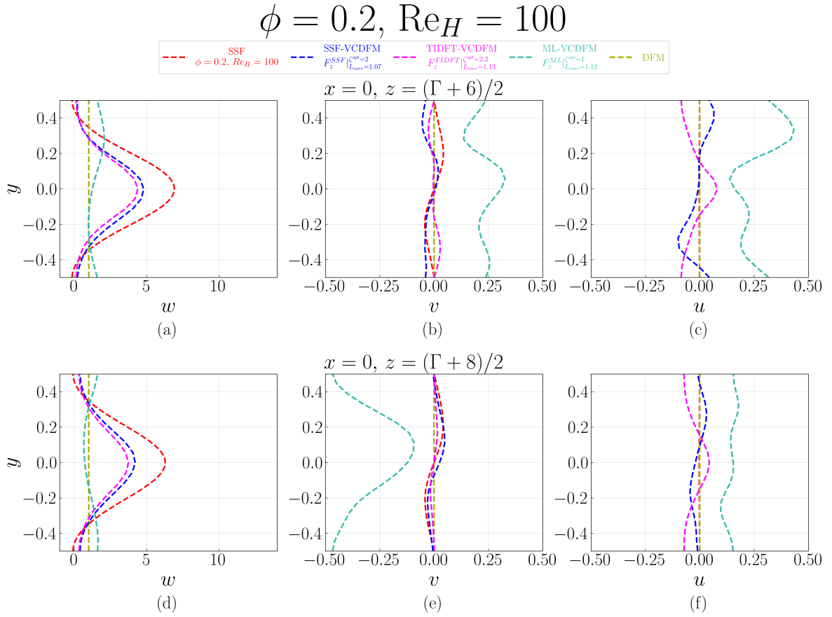
Figure D.265: Velocity profiles at x = 0 for the 1 \times 1 SRG at \phi = 0.2 and \text{Re}_H = 100 , comparing the SSF, DFM, SSF-VCDFM, TIDFT-VCDFM, and ML-VCDFM. Profiles of w(y) , v(y) , and u(y) are shown at z = (\Gamma + 6)/2 in (a–c) and z = (\Gamma + 8)/2 in (d–f). ML-VCDFM is evaluated outside the Reynolds-number range used for training.
