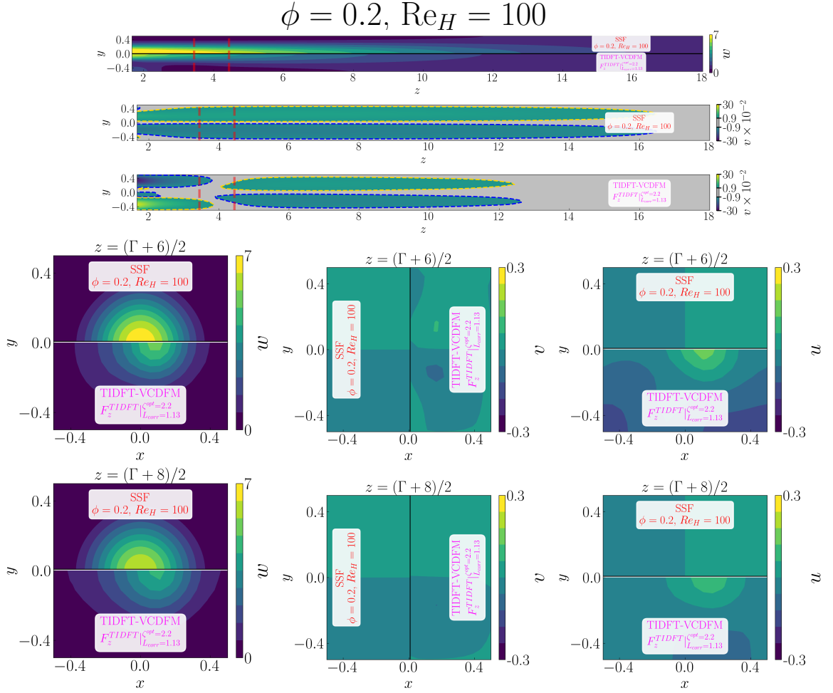
Figure D.267: Detailed comparison between the geometry-resolved small-scale flow (SSF) and TIDFT-VCDFM using F_z^{\text{TIDFT}} for the 1 \times 1 SRG at \phi = 0.2 and \text{Re}_H = 100 . The upper panels compare streamwise velocity w and transverse velocity v in the central (z, y) -plane, restricted to the correction region. The lower panels compare the corresponding transverse (x, y) -plane distributions of w , v , and u , from left to right, at z = (\Gamma + 6)/2 in the first row and z = (\Gamma + 8)/2 in the second row.
