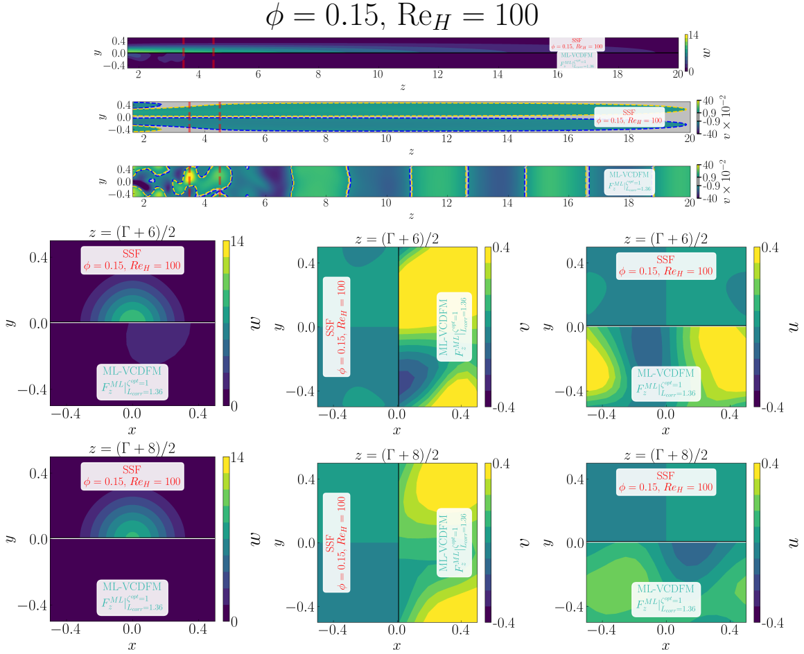
Figure D.262: Detailed comparison between the geometry-resolved small-scale flow (SSF) and ML-VCDFM using F_z^{\text{ML}} for the 1 \times 1 SRG at \phi = 0.15 and Re_H = 100 . The upper panels compare streamwise velocity w and transverse velocity v in the central (z, y) -plane, restricted to the correction region. The lower panels compare the corresponding transverse (x, y) -plane distributions of w , v , and u , from left to right, at z = (\Gamma + 6)/2 in the first row and z = (\Gamma + 8)/2 in the second row. This case tests extrapolation beyond the Reynolds-number range used for training; deviations from the SSF appear in the velocity fields.
