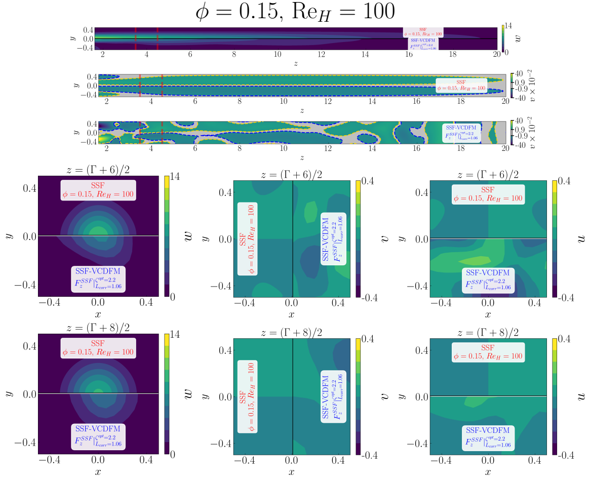
Figure D.260: Detailed comparison between the geometry-resolved small-scale flow (SSF) and SSF-VCDFM using F_z^{\text{SSF}} for the 1 \times 1 SRG at \phi = 0.15 and Re_H = 100 . The upper panels compare streamwise velocity w and transverse velocity v in the central (z, y) -plane, restricted to the correction region. The lower panels compare the corresponding transverse (x, y) -plane distributions of w , v , and u , from left to right, at z = (\Gamma + 6)/2 in the first row and z = (\Gamma + 8)/2 in the second row.
