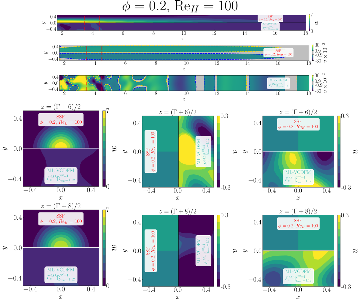
Figure D.268: Detailed comparison between the geometry-resolved small-scale flow (SSF) and ML-VCDFM using F_z^{\text{ML}} for the 1 \times 1 SRG at \phi = 0.2 and \text{Re}_H = 100 . The upper panels compare streamwise velocity w and transverse velocity v in the central (z, y) -plane, restricted to the correction region. The lower panels compare the corresponding transverse (x, y) -plane distributions of w , v , and u , from left to right, at z = (\Gamma + 6)/2 in the first row and z = (\Gamma + 8)/2 in the second row. This case tests extrapolation beyond the Reynolds-number range used for training; deviations from the SSF appear in the velocity fields.
