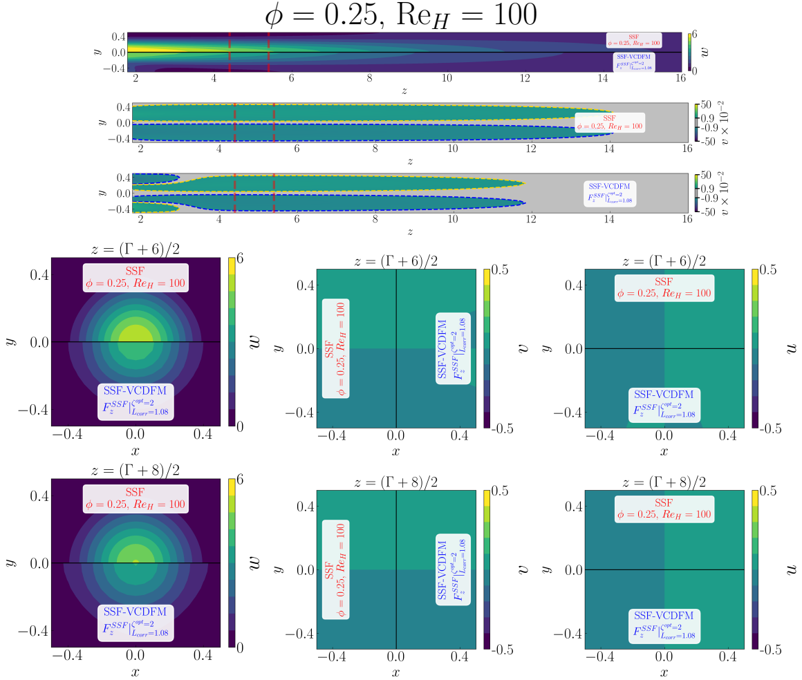
Figure D.272: Detailed comparison between the geometry-resolved small-scale flow (SSF) and SSF-VCDFM using F_z^{\text{SSF}} for the 1 × 1 SRG at \phi = 0.25 and \text{Re}_H = 100 . The upper panels compare streamwise velocity w and transverse velocity v in the central (z, y) -plane, restricted to the correction region. The lower panels compare the corresponding transverse (x, y) -plane distributions of w , v , and u , from left to right, at z = (\Gamma + 6)/2 in the first row and z = (\Gamma + 8)/2 in the second row.
