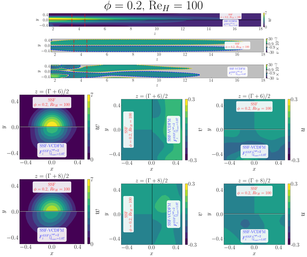
Figure D.266: Detailed comparison between the geometry-resolved small-scale flow (SSF) and SSF-VCDFM using F_z^{\text{SSF}} for the 1 \times 1 SRG at \phi = 0.2 and \text{Re}_H = 100 . The upper panels compare streamwise velocity w and transverse velocity v in the central (z, y) -plane, restricted to the correction region. The lower panels compare the corresponding transverse (x, y) -plane distributions of w , v , and u , from left to right, at z = (\Gamma + 6)/2 in the first row and z = (\Gamma + 8)/2 in the second row.
