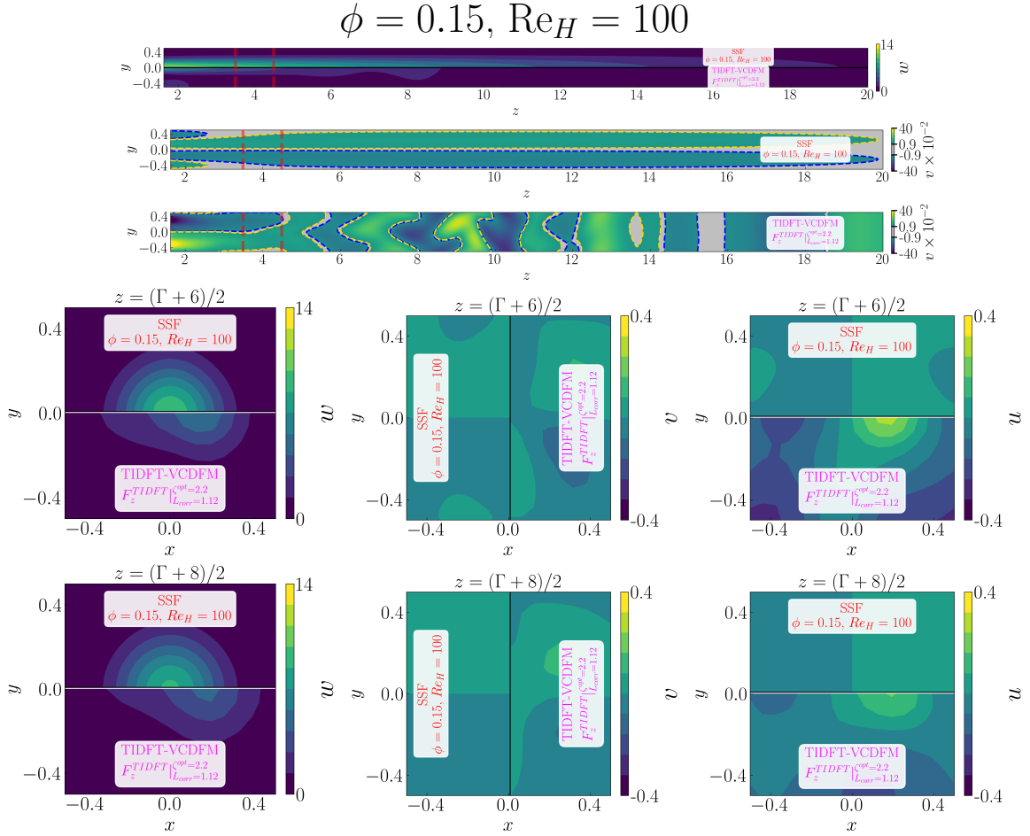
Figure D.261: Detailed comparison between the geometry-resolved small-scale flow (SSF) and TIDFT-VCDFM using F_z^{\text{TIDFT}} for the 1 \times 1 SRG at \phi = 0.15 and \text{Re}_H = 100 . The upper panels compare streamwise velocity w and transverse velocity v in the central (z, y) -plane, restricted to the correction region. The lower panels compare the corresponding transverse (x, y) -plane distributions of w , v , and u , from left to right, at z = (\Gamma + 6)/2 in the first row and z = (\Gamma + 8)/2 in the second row.
