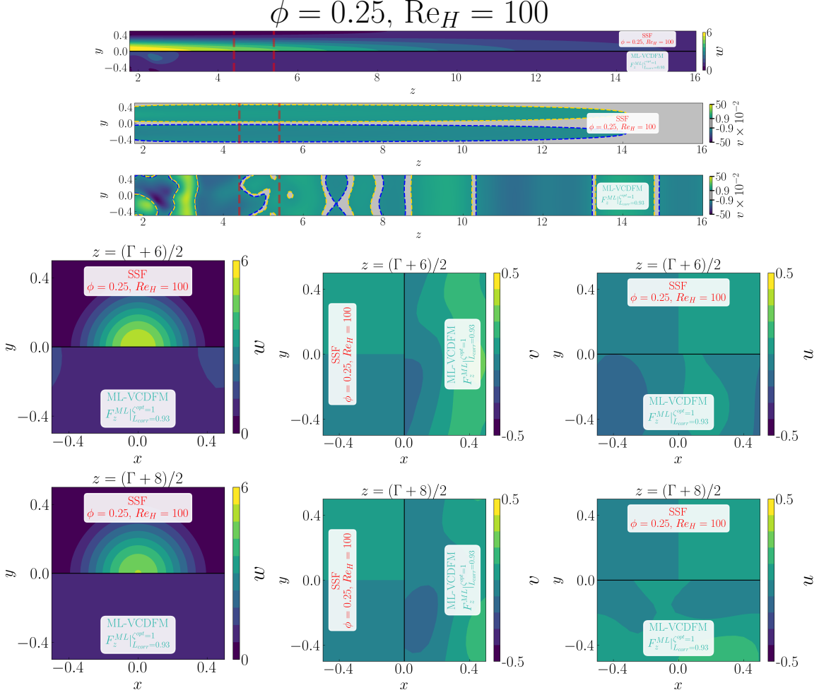
Figure D.274: Detailed comparison between the geometry-resolved small-scale flow (SSF) and ML-VCDFM using F_z^{\text{ML}} for the 1 \times 1 SRG at \phi = 0.25 and \text{Re}_H = 100 . The upper panels compare streamwise velocity w and transverse velocity v in the central (z, y) -plane, restricted to the correction region. The lower panels compare the corresponding transverse (x, y) -plane distributions of w , v , and u , from left to right, at z = (\Gamma + 6)/2 in the first row and z = (\Gamma + 8)/2 in the second row. This case tests extrapolation beyond the Reynolds-number range used for training; deviations from the SSF appear in the velocity fields.
