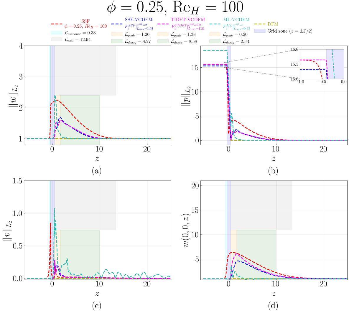
Figure D.269: Streamwise evolution of (a) \|w\|_{L_2} , (b) \|p\|_{L_2} , (c) \|v\|_{L_2} , and (d) centerline velocity w(0,0,z) for the 1 \times 1 SRG at \phi = 0.25 and \text{Re}_H = 100 . The figure compares the SSF, DFM, SSF-VCDFM, TIDFT-VCDFM, and ML-VCDFM. Shading marks the grid and the characteristic entrance, exit, peak, and decay regions. Only the SSF-based \mathcal{L}_{peak} and \mathcal{L}_{decay} are marked on the plot; the corresponding TIDFT-VCDFM and ML-VCDFM values appear in the legend. The ML-VCDFM result tests extrapolation beyond the Reynolds-number range used for training and deviates from the reference SSF solution.
