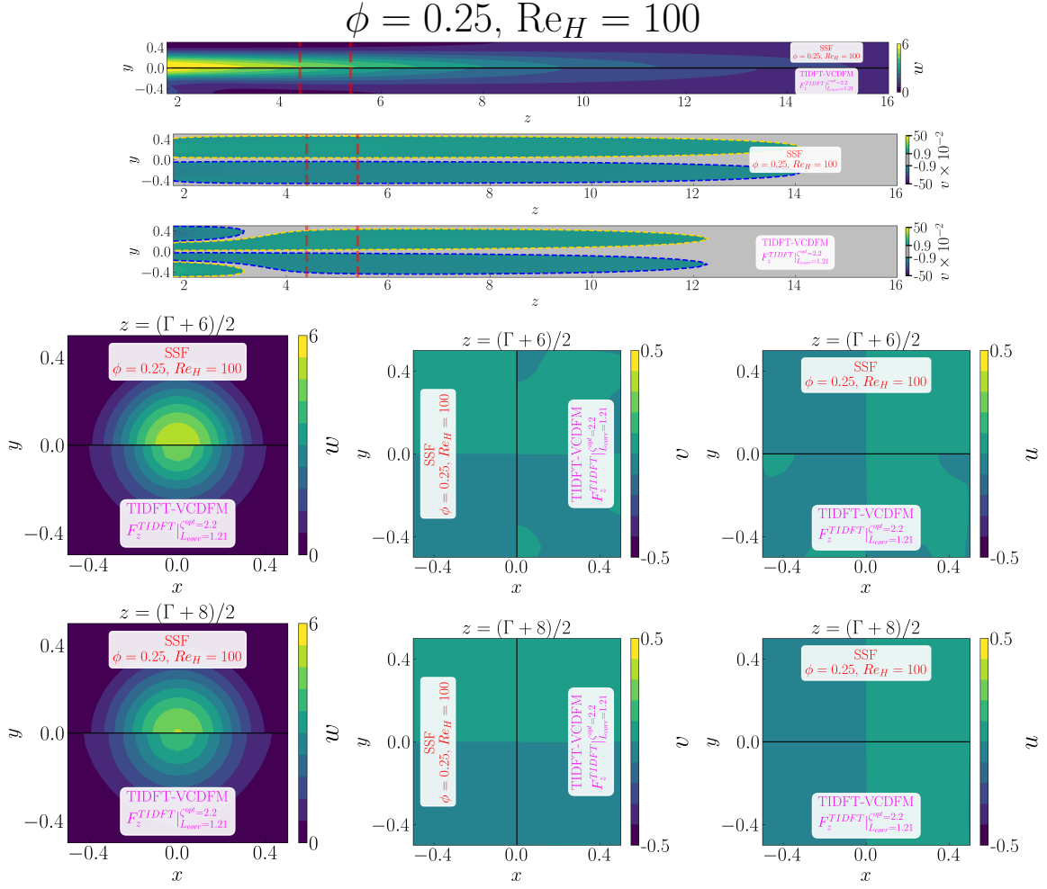
Figure D.273: Detailed comparison between the geometry-resolved small-scale flow (SSF) and TIDFT-VCDFM using F_z^{\text{TIDFT}} for the 1 \times 1 SRG at \phi = 0.25 and Re_H = 100 . The upper panels compare streamwise velocity w and transverse velocity v in the central (z, y) -plane, restricted to the correction region. The lower panels compare the corresponding transverse (x, y) -plane distributions of w , v , and u , from left to right, at z = (\Gamma + 6)/2 in the first row and z = (\Gamma + 8)/2 in the second row.
