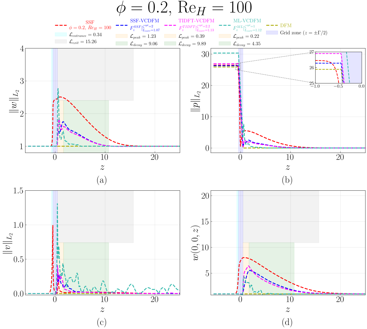
Figure D.263: Streamwise evolution of (a) \|w\|_{L_2} , (b) \|p\|_{L_2} , (c) \|v\|_{L_2} , and (d) centerline velocity w(0,0,z) for the 1 \times 1 SRG at \phi = 0.2 and \text{Re}_H = 100 . The figure compares the SSF, DFM, SSF-VCDFM, TIDFT-VCDFM, and ML-VCDFM. Shading marks the grid and the characteristic entrance, exit, peak, and decay regions. Only the SSF-based \mathcal{L}_{peak} and \mathcal{L}_{decay} are marked on the plot; the corresponding TIDFT-VCDFM and ML-VCDFM values appear in the legend. The ML-VCDFM result tests extrapolation beyond the Reynolds-number range used for training and deviates from the reference SSF solution.
