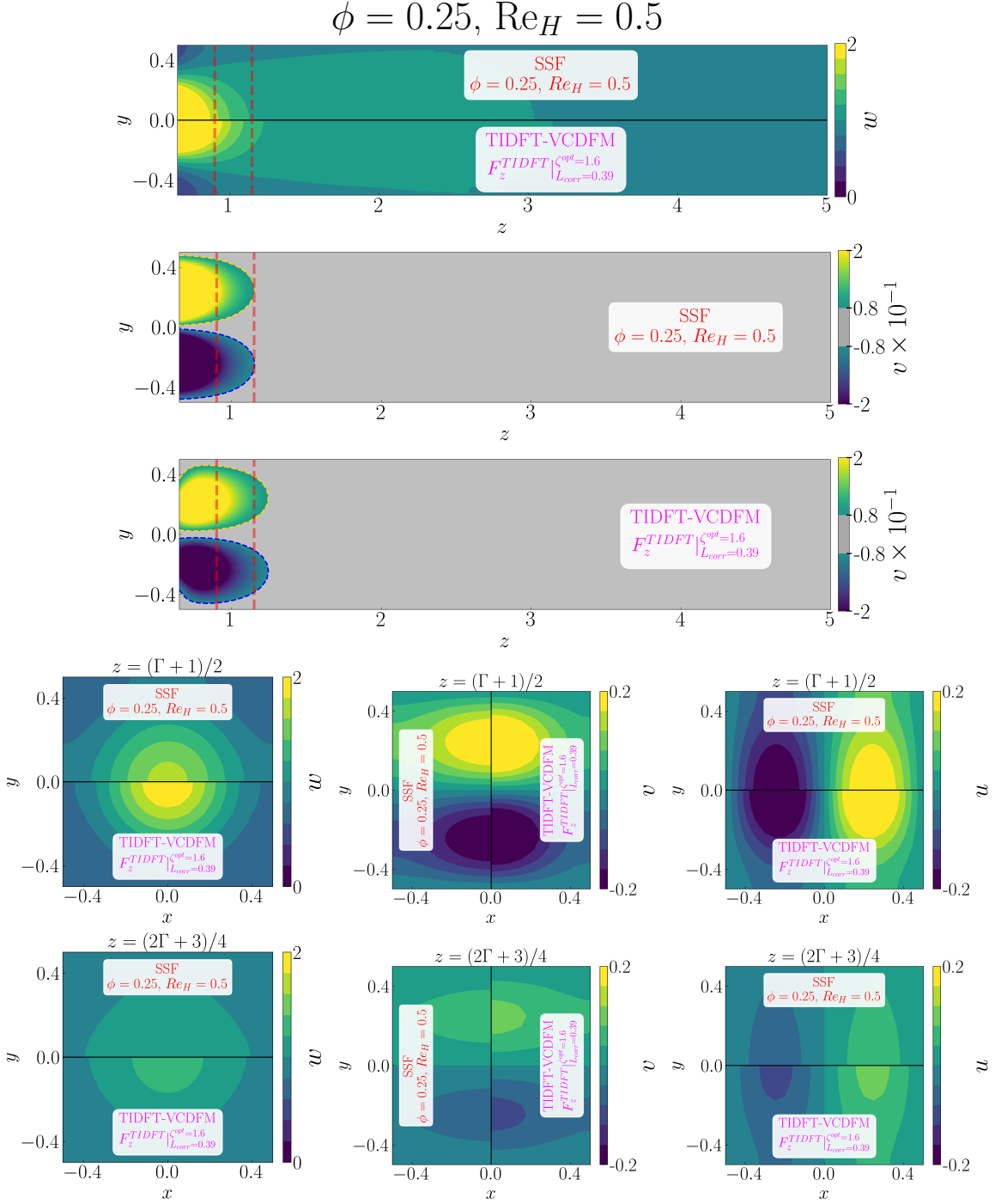
Figure D.175: Detailed comparison between the geometry-resolved small-scale flow (SSF) and TIDFT-VCDFM using F_z^{\text{TIDFT}} for the 1 \times 1 SRG at \phi = 0.25 and \text{Re}_H = 0.5 . The upper panels compare the streamwise velocity w and transverse velocity v in the central (z, y) -plane, restricted to the correction region. The lower panels compare the corresponding transverse (x, y) -plane distributions of w , v , and u , from left to right, at z = (\Gamma + 1)/2 in the first row and z = (2\Gamma + 3)/4 in the second row.
