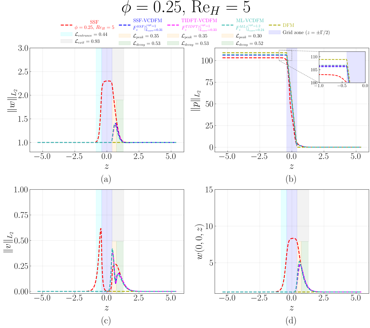
Figure D.183: Streamwise evolution of (a) \|w\|_{L_2} , (b) \|p\|_{L_2} , (c) \|v\|_{L_2} , and (d) centerline velocity w(0,0,z) for the 1 \times 1 SRG at \phi = 0.25 and \text{Re}_H = 5 . The figure compares the SSF, DFM, SSF-VCDFM, TIDFT-VCDFM, and ML-VCDFM. Shading marks the grid and the characteristic entrance, exit, peak, and decay regions. Only the SSF-based \mathcal{L}_{\text{peak}} and \mathcal{L}_{\text{decay}} are marked on the plot; the corresponding TIDFT-VCDFM and ML-VCDFM values appear in the legend.
