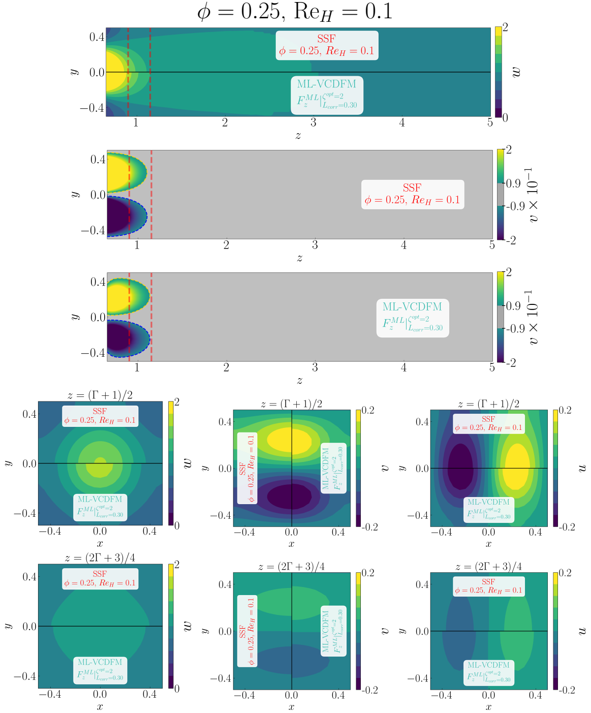
Figure D.170: Detailed comparison between the geometry-resolved small-scale flow (SSF) and ML-VCDFM using F_z^{\text{ML}} for the 1 \times 1 SRG at \phi = 0.25 and \text{Re}_H = 0.1 . The upper panels compare the streamwise velocity w and transverse velocity v in the central (z, y) -plane, restricted to the correction region. The lower panels compare the corresponding transverse (x, y) -plane distributions of w , v , and u , from left to right, at z = (\Gamma + 1)/2 in the first row and z = (2\Gamma + 3)/4 in the second row.
