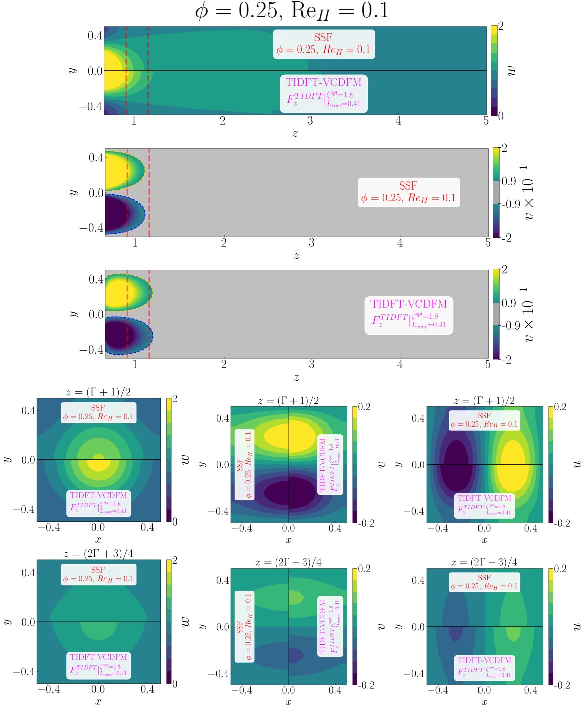
Figure D.169: Detailed comparison between the geometry-resolved small-scale flow (SSF) and TIDFT-VCDFM using F_z^{\text{TIDFT}} for the 1 \times 1 SRG at \phi = 0.25 and \text{Re}_H = 0.1 . The upper panels compare the streamwise velocity w and transverse velocity v in the central (z, y) -plane, restricted to the correction region. The lower panels compare the corresponding transverse (x, y) -plane distributions of w , v , and u , from left to right, at z = (\Gamma + 1)/2 in the first row and z = (2\Gamma + 3)/4 in the second row.
