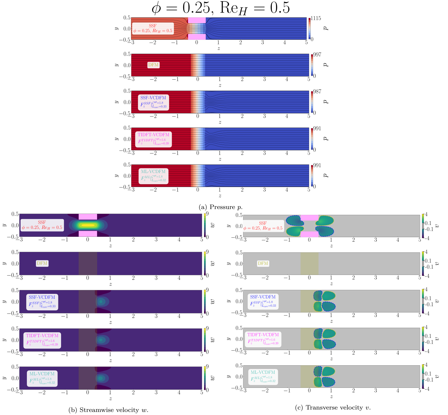
Figure D.172: Flow organization in the streamwise (z, y) -plane for the 1 \times 1 SRG at \phi = 0.25 , \text{Re}_H = 0.5 , and \alpha = 0^\circ . The blocks show (a) pressure p with streamlines, (b) streamwise velocity w , and (c) transverse velocity v . Within each block, the rows show, from top to bottom, the SSF, DFM, SSF-VCDFM, TIDFT-VCDFM, and ML-VCDFM. Pink shading marks the grid walls in the SSF; olive shading marks the equivalent porous zone in the model solutions.
