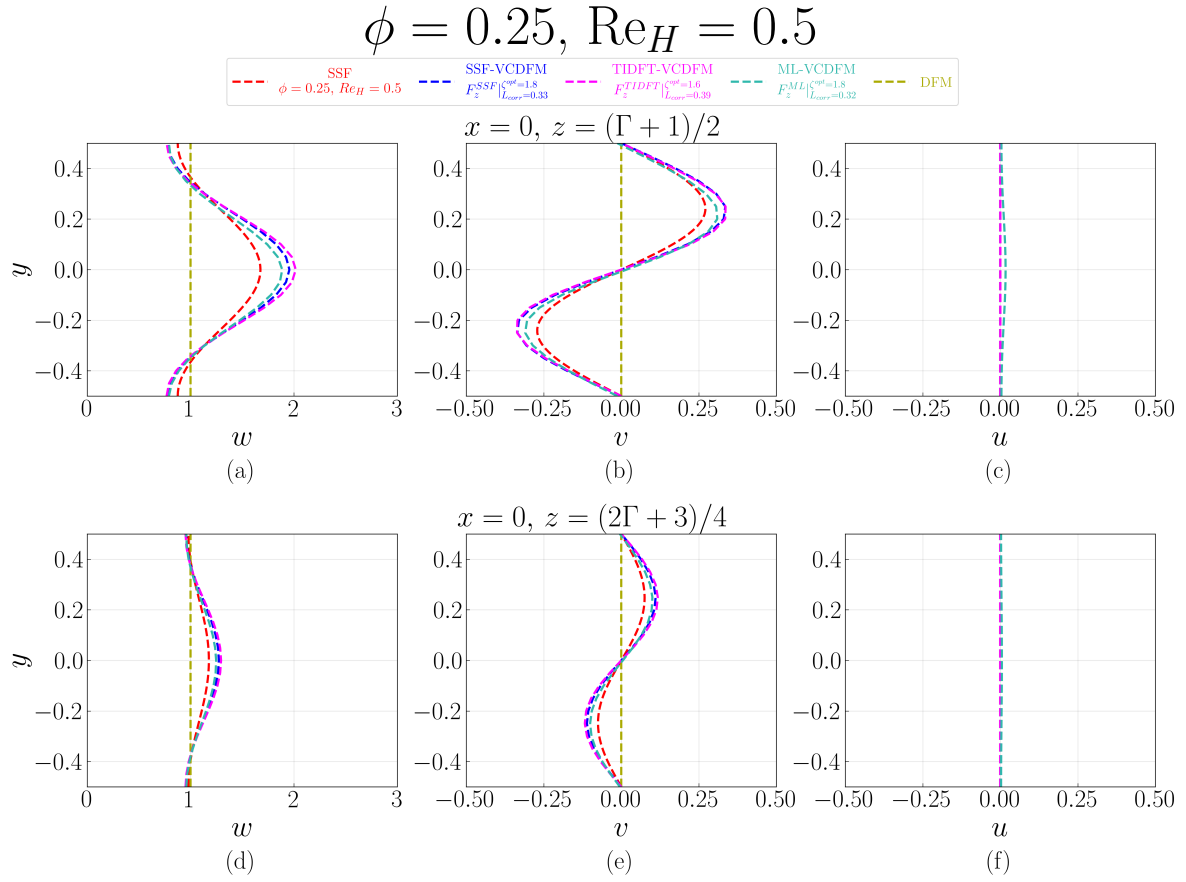
Figure D.173: Velocity profiles at x = 0 for the 1 \times 1 SRG at \phi = 0.25 and \text{Re}_H = 0.5 , comparing the SSF, DFM, SSF-VCDFM, TIDFT-VCDFM, and ML-VCDFM. Profiles of w(y) , v(y) , and u(y) are shown at z = (\Gamma + 1)/2 in (a–c) and z = (2\Gamma + 3)/4 in (d–f).
