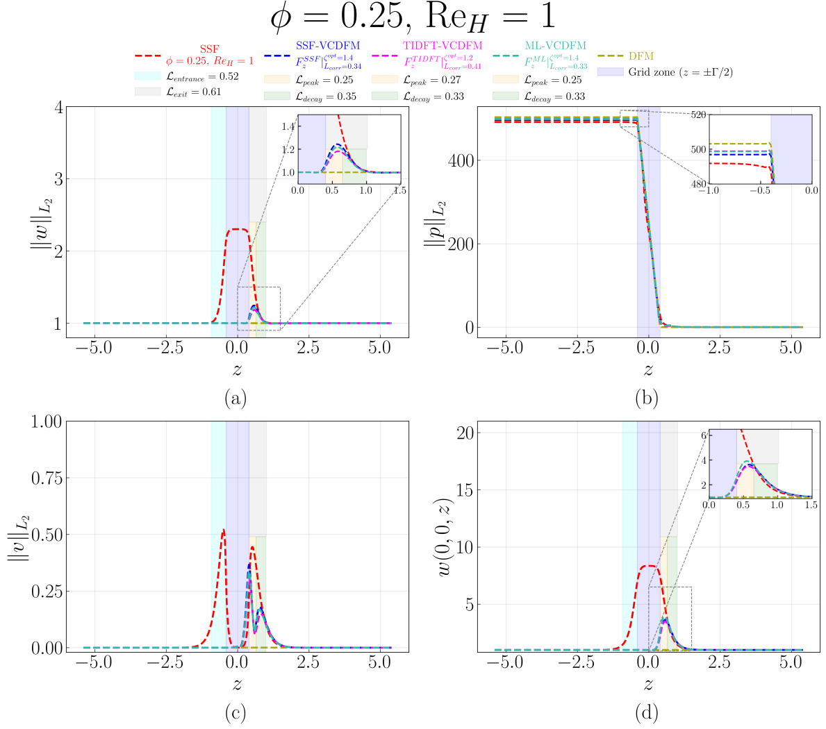
Figure D.177: Streamwise evolution of (a) \|w\|_{L_2} , (b) \|p\|_{L_2} , (c) \|v\|_{L_2} , and (d) centerline velocity w(0,0,z) for the 1 \times 1 SRG at \phi = 0.25 and \text{Re}_H = 1 . The figure compares the SSF, DFM, SSF-VCDFM, TIDFT-VCDFM, and ML-VCDFM. Shading marks the grid and the characteristic entrance, exit, peak, and decay regions. Only the SSF-based \mathcal{L}_{\text{peak}} and \mathcal{L}_{\text{decay}} are marked on the plot; the corresponding TIDFT-VCDFM and ML-VCDFM values appear in the legend.
