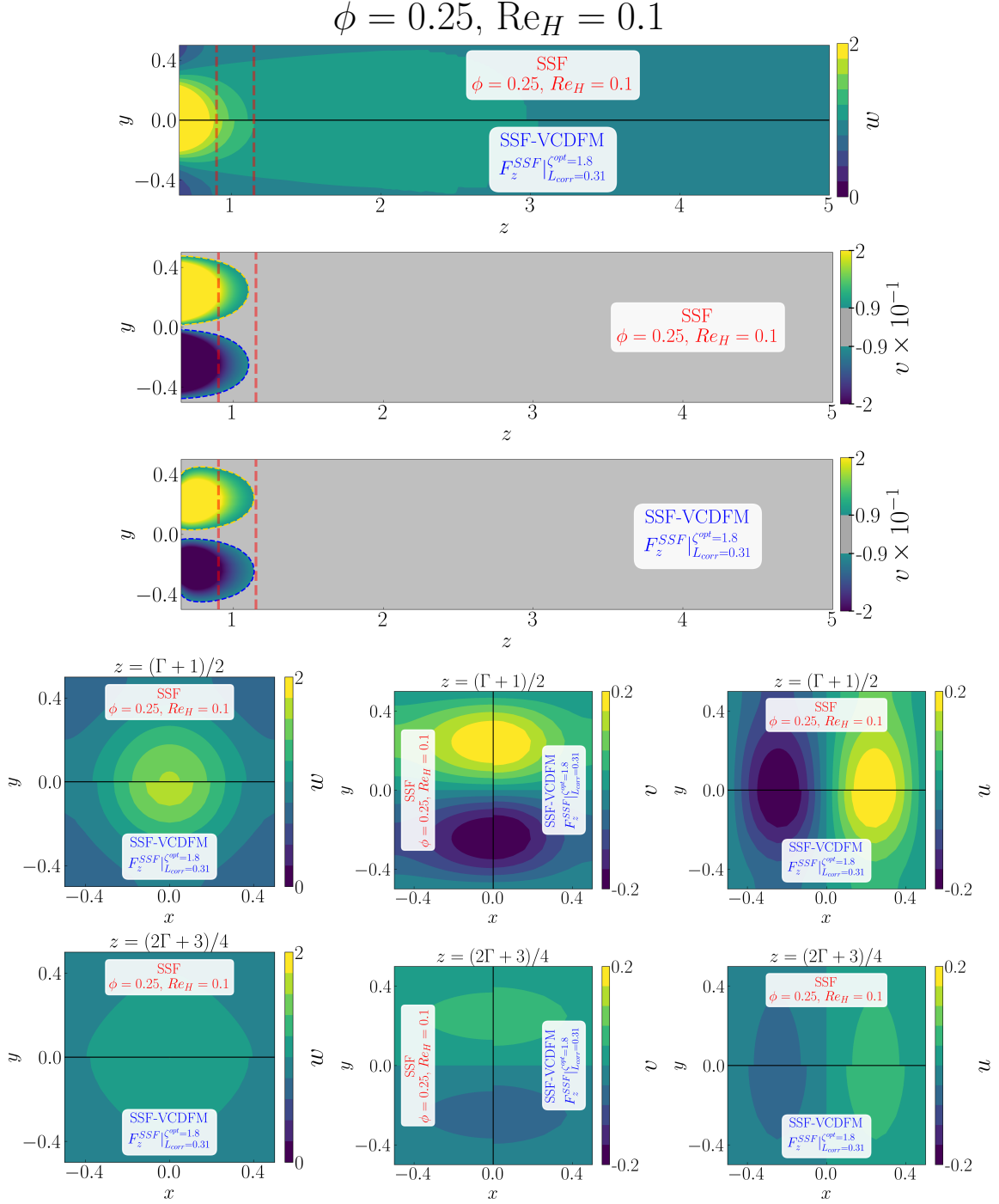
Figure D.168: Detailed comparison between the geometry-resolved small-scale flow (SSF) and SSF-VCDFM using F_z^{\text{SSF}} for the 1 \times 1 SRG at \phi = 0.25 and Re_H = 0.1 . The upper panels compare the streamwise velocity w and transverse velocity v in the central (z, y) -plane, restricted to the correction region. The lower panels compare the corresponding transverse (x, y) -plane distributions of w , v , and u , from left to right, at z = (\Gamma + 1)/2 in the first row and z = (2\Gamma + 3)/4 in the second row.
