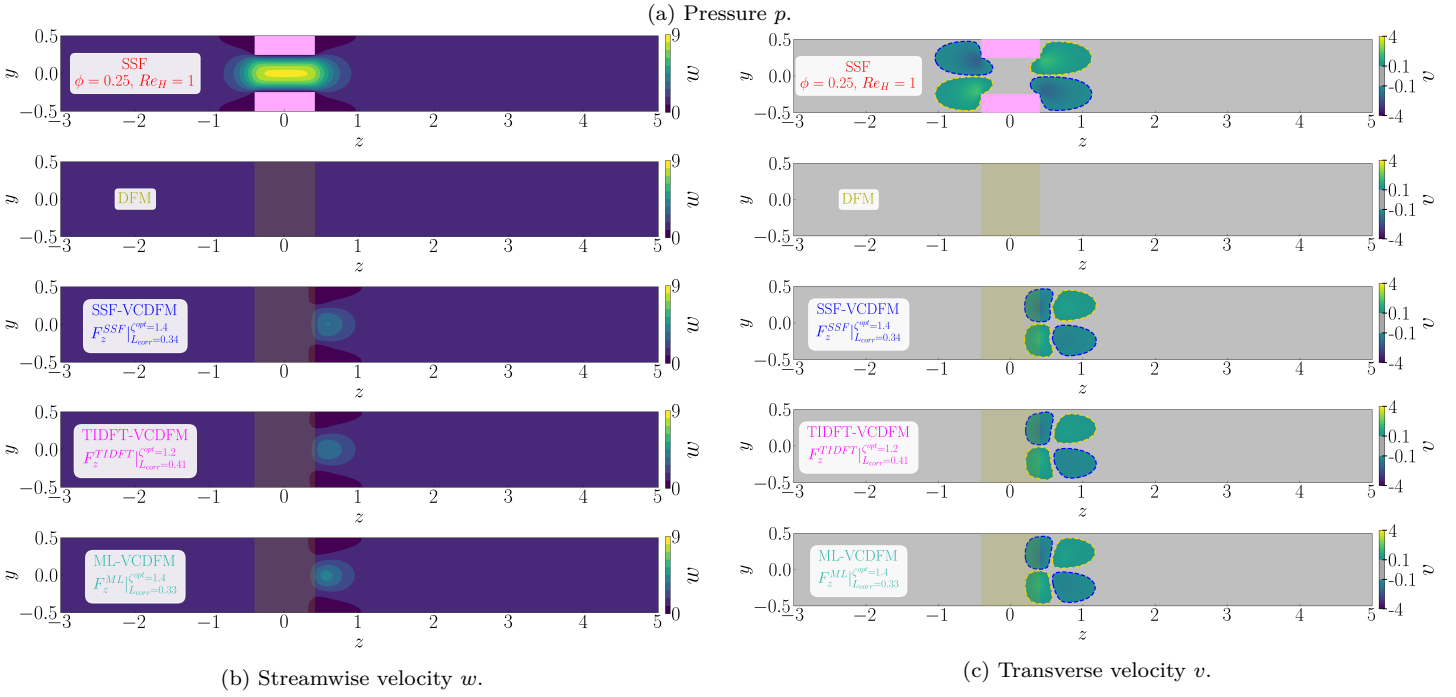
Figure D.178: Flow organization in the streamwise ( z, y )-plane for the 1 \times 1 SRG at \phi = 0.25 , \text{Re}_H = 1 , and \alpha = 0^\circ . The blocks show (a) pressure p with streamlines, (b) streamwise velocity w , and (c) transverse velocity v . Within each block, the rows show, from top to bottom, the SSF, DFM, SSF-VCDFM, TIDFT-VCDFM, and ML-VCDFM. Pink shading marks the grid walls in the SSF; olive shading marks the equivalent porous zone in the model solutions.
