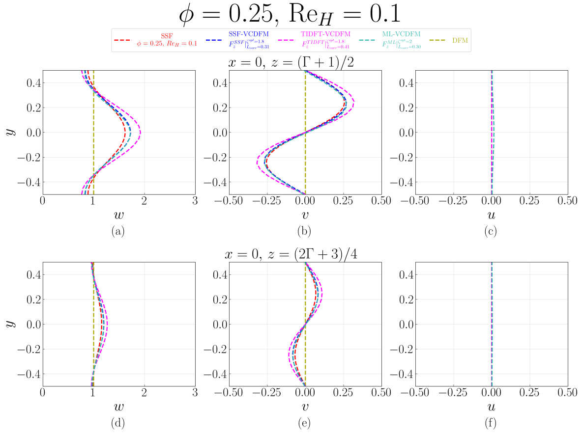
Figure D.167: Velocity profiles at x = 0 for the 1 \times 1 SRG at \phi = 0.25 and \text{Re}_H = 0.1 , comparing the SSF, DFM, SSF-VCDFM, TIDFT-VCDFM, and ML-VCDFM. Profiles of w(y) , v(y) , and u(y) are shown at z = (\Gamma + 1)/2 in (a–c) and z = (2\Gamma + 3)/4 in (d–f).
