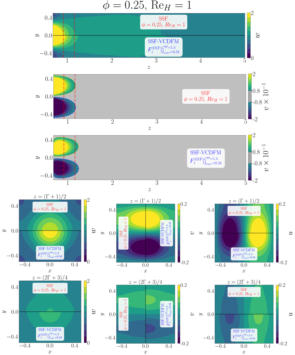
Figure D.180: Detailed comparison between the geometry-resolved small-scale flow (SSF) and SSF-VCDFM using F_z^{\text{SSF}} for the 1 \times 1 SRG at \phi = 0.25 and \text{Re}_H = 1 . The upper panels compare the streamwise velocity w and transverse velocity v in the central (z, y) -plane, restricted to the correction region. The lower panels compare the corresponding transverse (x, y) -plane distributions of w , v , and u , from left to right, at z = (\Gamma + 1)/2 in the first row and z = (2\Gamma + 3)/4 in the second row.
