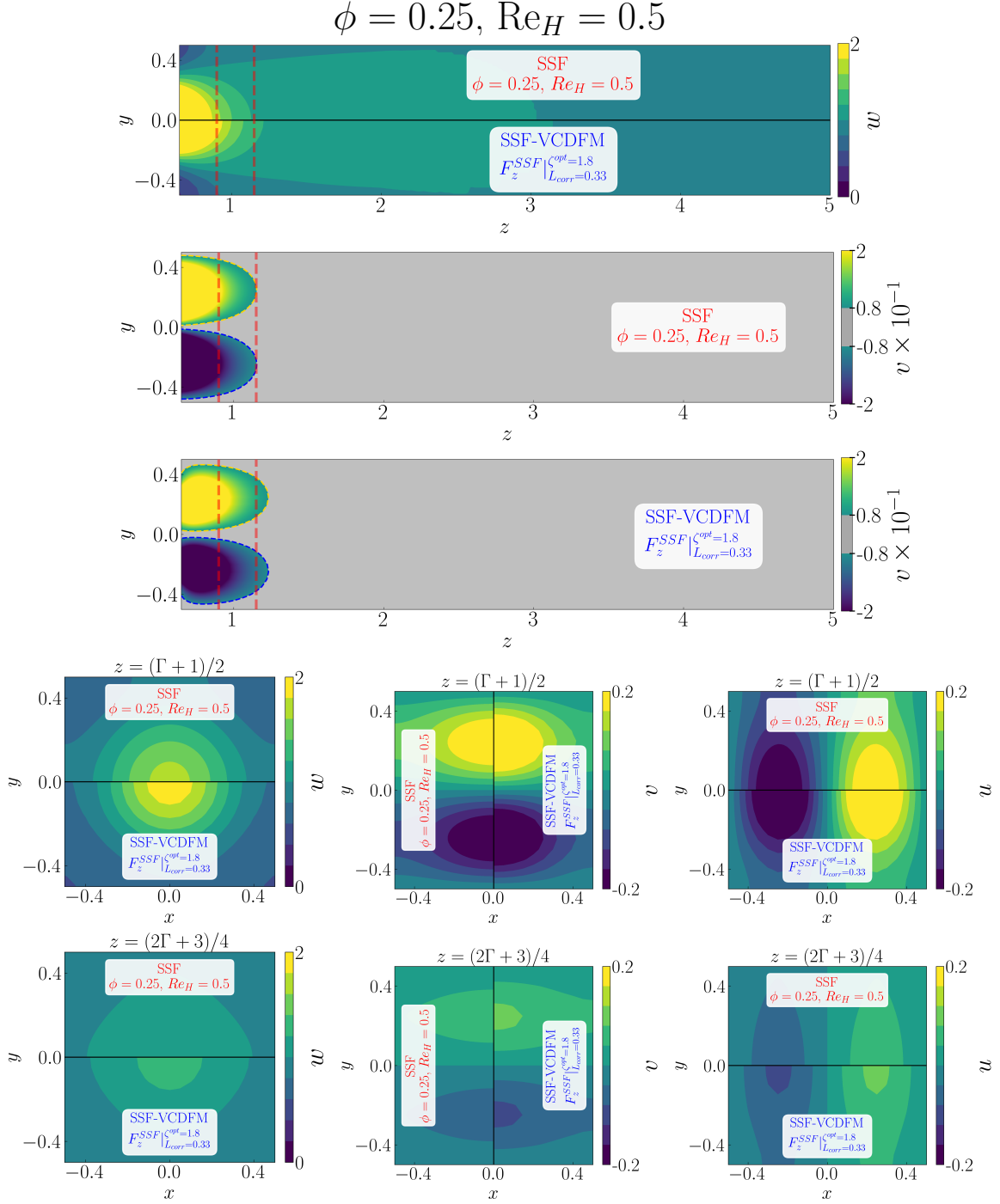
Figure D.174: Detailed comparison between the geometry-resolved small-scale flow (SSF) and SSF-VCDFM using F_z^{\text{SSF}} for the 1 \times 1 SRG at \phi = 0.25 and \text{Re}_H = 0.5 . The upper panels compare the streamwise velocity w and transverse velocity v in the central (z, y) -plane, restricted to the correction region. The lower panels compare the corresponding transverse (x, y) -plane distributions of w , v , and u , from left to right, at z = (\Gamma + 1)/2 in the first row and z = (2\Gamma + 3)/4 in the second row.
