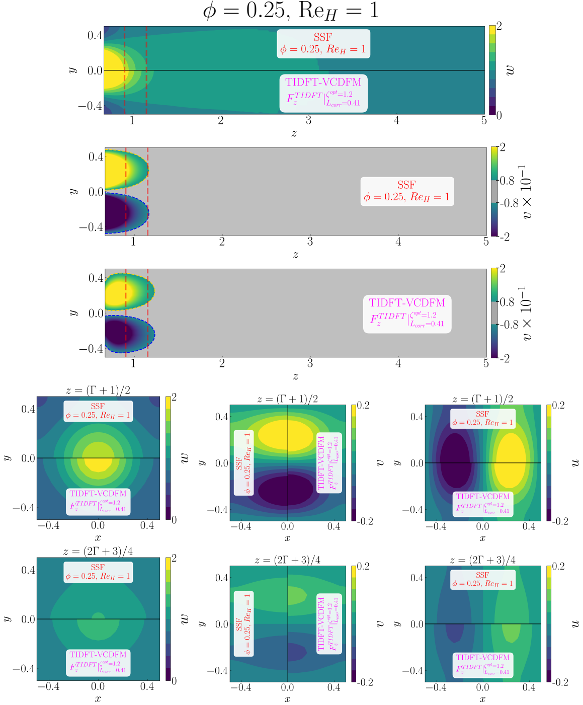
Figure D.181: Detailed comparison between the geometry-resolved small-scale flow (SSF) and TIDFT-VCDFM using F_z^{\text{TIDFT}} for the 1 \times 1 SRG at \phi = 0.25 and \text{Re}_H = 1 . The upper panels compare the streamwise velocity w and transverse velocity v in the central (z, y) -plane, restricted to the correction region. The lower panels compare the corresponding transverse (x, y) -plane distributions of w , v , and u , from left to right, at z = (\Gamma + 1)/2 in the first row and z = (2\Gamma + 3)/4 in the second row.
