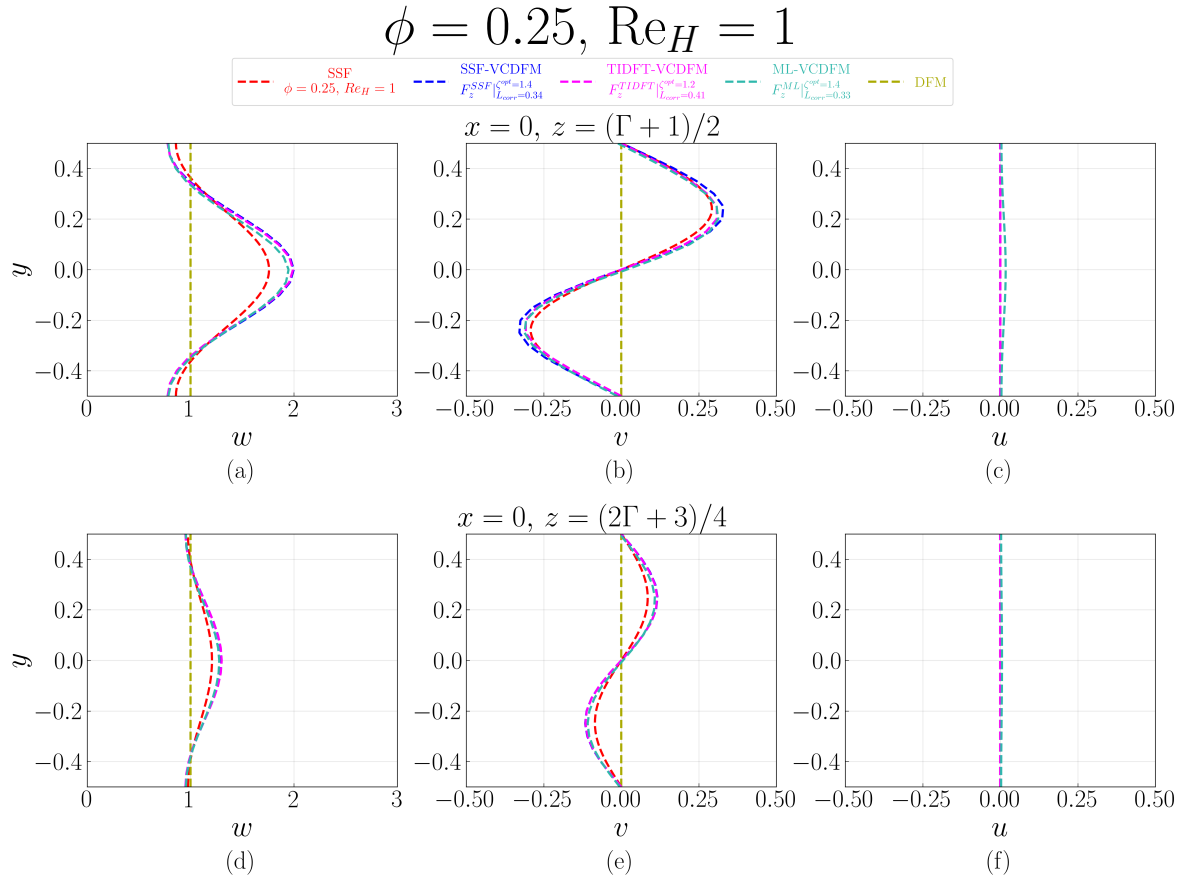
Figure D.179: Velocity profiles at x = 0 for the 1 \times 1 SRG at \phi = 0.25 and \text{Re}_H = 1 , comparing the SSF, DFM, SSF-VCDFM, TIDFT-VCDFM, and ML-VCDFM. Profiles of w(y) , v(y) , and u(y) are shown at z = (\Gamma + 1)/2 in (a–c) and z = (2\Gamma + 3)/4 in (d–f).
