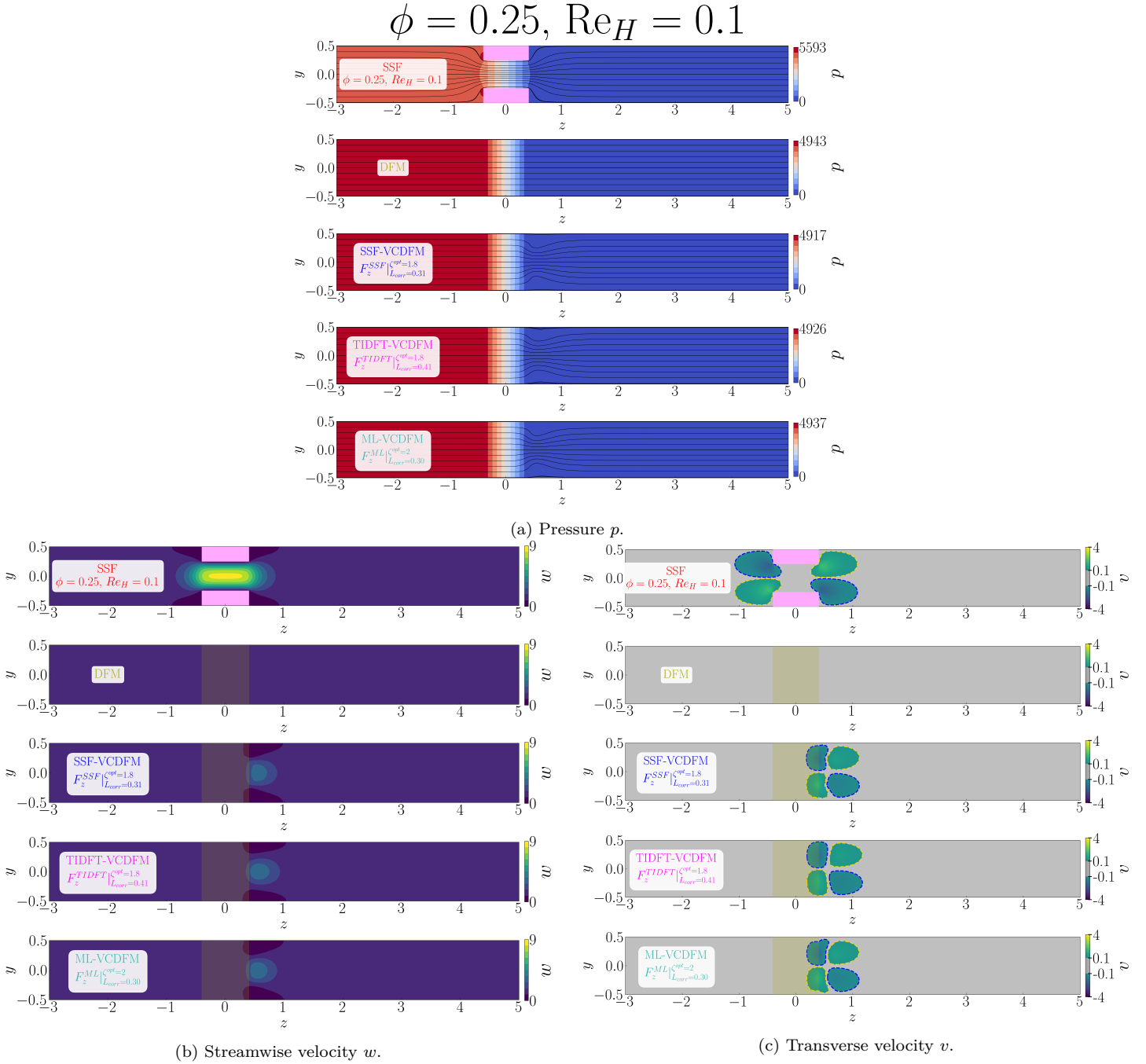
Figure D.166: Flow organization in the streamwise (z, y) -plane for the 1 \times 1 SRG at \phi = 0.25 , \text{Re}_H = 0.1 , and \alpha = 0^\circ . The blocks show (a) pressure p with streamlines, (b) streamwise velocity w , and (c) transverse velocity v . Within each block, the rows show, from top to bottom, the SSF, DFM, SSF-VCDFM, TIDFT-VCDFM, and ML-VCDFM. Pink shading marks the grid walls in the SSF; olive shading marks the equivalent porous zone in the model solutions.
