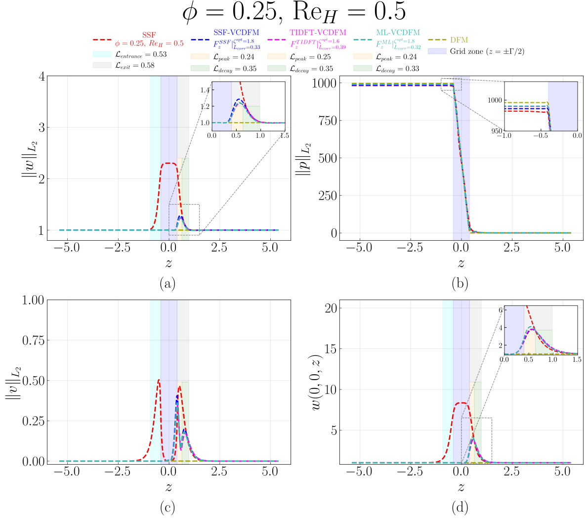
Figure D.171: Streamwise evolution of (a) \|w\|_{L_2} , (b) \|p\|_{L_2} , (c) \|v\|_{L_2} , and (d) centerline velocity w(0,0,z) for the 1 \times 1 SRG at \phi = 0.25 and \text{Re}_H = 0.5 . The figure compares the SSF, DFM, SSF-VCDFM, TIDFT-VCDFM, and ML-VCDFM. Shading marks the grid and the characteristic entrance, exit, peak, and decay regions. Only the SSF-based \mathcal{L}_{\text{peak}} and \mathcal{L}_{\text{decay}} are marked on the plot; the corresponding TIDFT-VCDFM and ML-VCDFM values appear in the legend.
