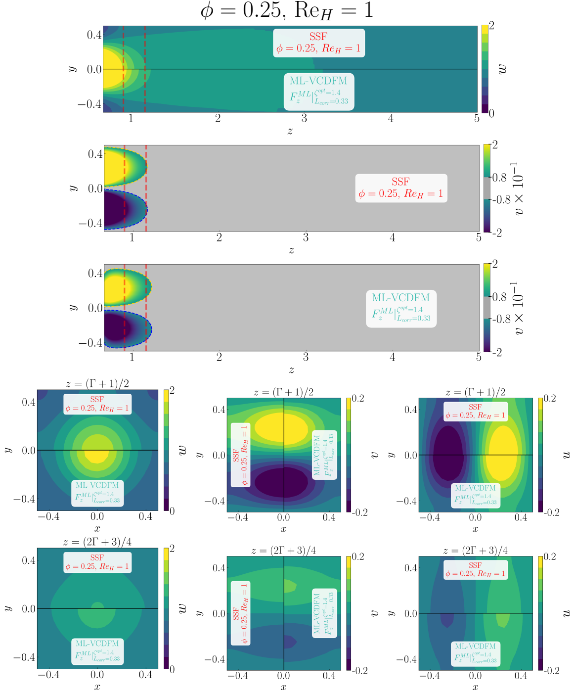
Figure D.182: Detailed comparison between the geometry-resolved small-scale flow (SSF) and ML-VCDFM using F_z^{\text{ML}} for the 1 \times 1 SRG at \phi = 0.25 and \text{Re}_H = 1 . The upper panels compare the streamwise velocity w and transverse velocity v in the central (z, y) -plane, restricted to the correction region. The lower panels compare the corresponding transverse (x, y) -plane distributions of w , v , and u , from left to right, at z = (\Gamma + 1)/2 in the first row and z = (2\Gamma + 3)/4 in the second row.
