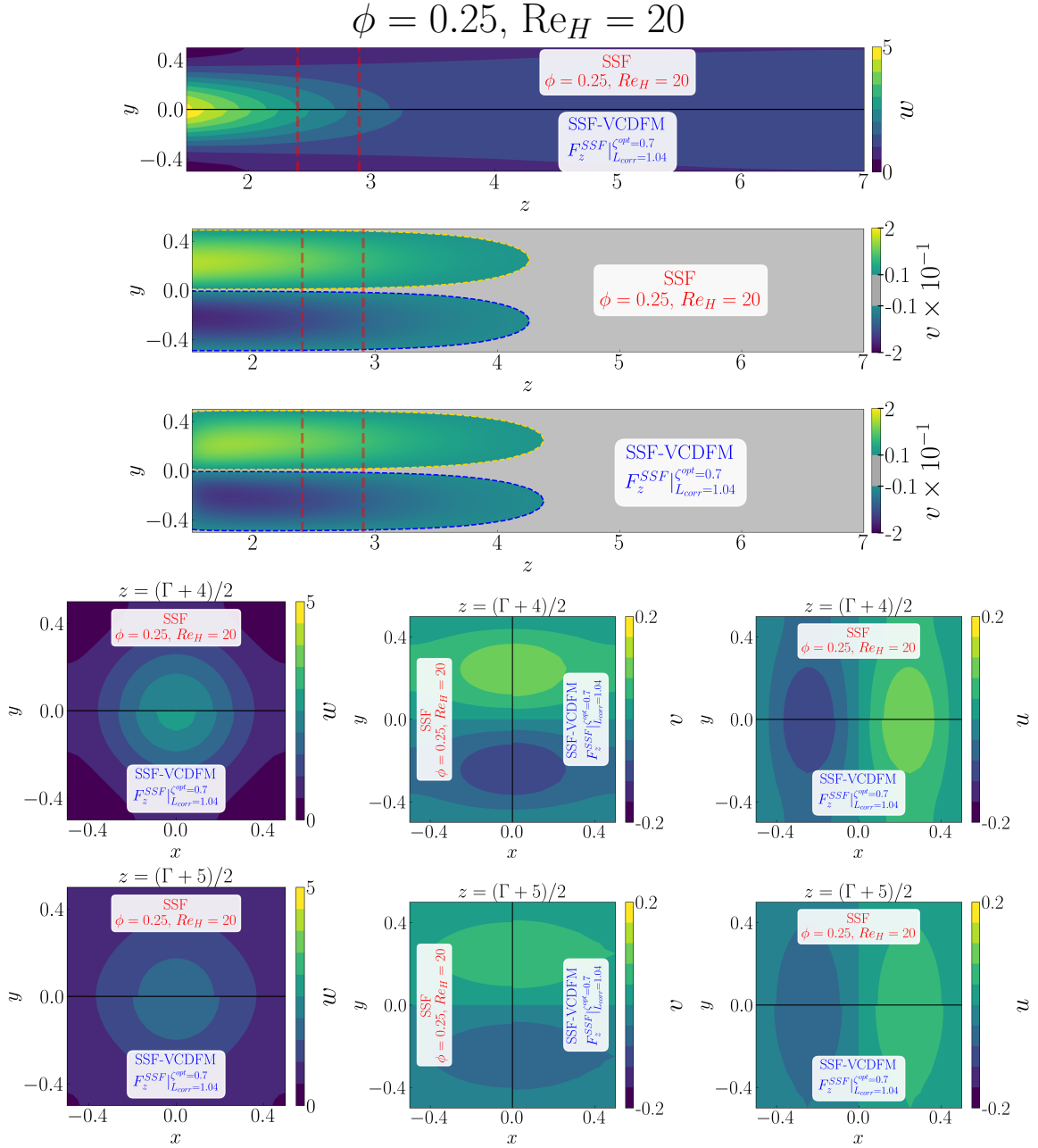
Figure D.198: Detailed comparison between the geometry-resolved small-scale flow (SSF) and SSF-VCDFM using F_z^{\text{SSF}} for the 1 \times 1 SRG at \phi = 0.25 and \text{Re}_H = 20 . The upper panels compare the streamwise velocity w and transverse velocity v in the central (z, y) -plane, restricted to the correction region. The lower panels compare the corresponding transverse (x, y) -plane distributions of w , v , and u , from left to right, at z = (\Gamma + 4)/2 in the first row and z = (\Gamma + 5)/2 in the second row.
