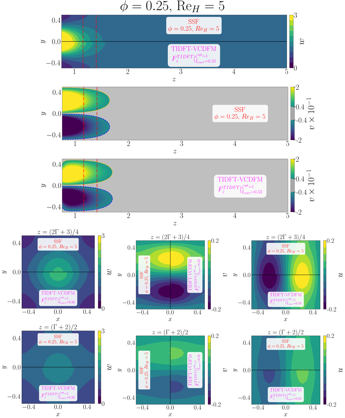
Figure D.187: Detailed comparison between the geometry-resolved small-scale flow (SSF) and TIDFT-VCDFM using F_z^{\text{TIDFT}} for the 1 \times 1 SRG at \phi = 0.25 and Re_H = 5 . The upper panels compare the streamwise velocity w and transverse velocity v in the central (z, y) -plane, restricted to the correction region. The lower panels compare the corresponding transverse (x, y) -plane distributions of w , v , and u , from left to right, at z = (2\Gamma + 3)/4 in the first row and z = (\Gamma + 2)/2 in the second row.
