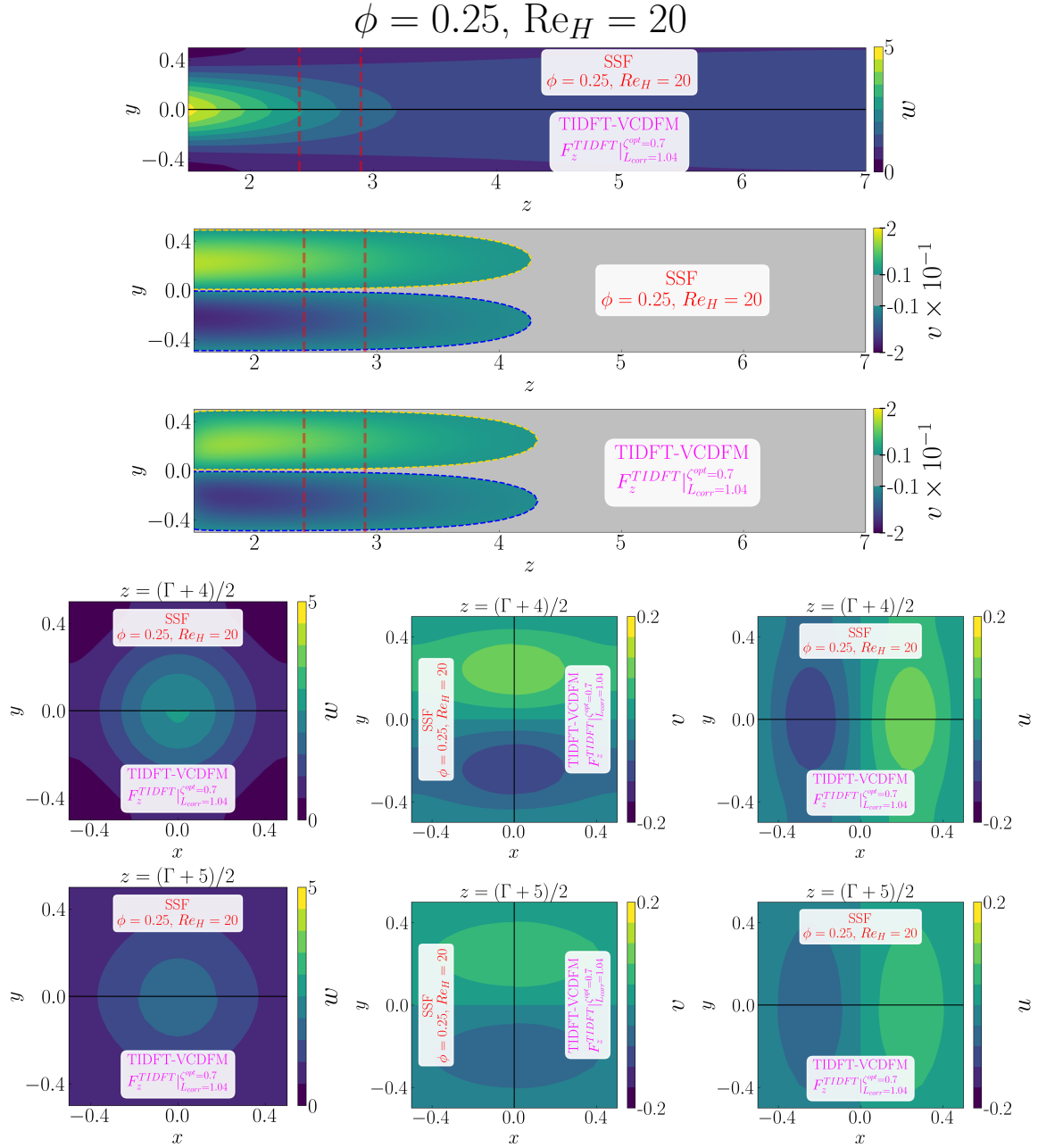
Figure D.199: Detailed comparison between the geometry-resolved small-scale flow (SSF) and TIDFT-VCDFM using F_z^{\text{TIDFT}} for the 1 \times 1 SRG at \phi = 0.25 and \text{Re}_H = 20 . The upper panels compare the streamwise velocity w and transverse velocity v in the central (z, y) -plane, restricted to the correction region. The lower panels compare the corresponding transverse (x, y) -plane distributions of w , v , and u , from left to right, at z = (\Gamma + 4)/2 in the first row and z = (\Gamma + 5)/2 in the second row.
