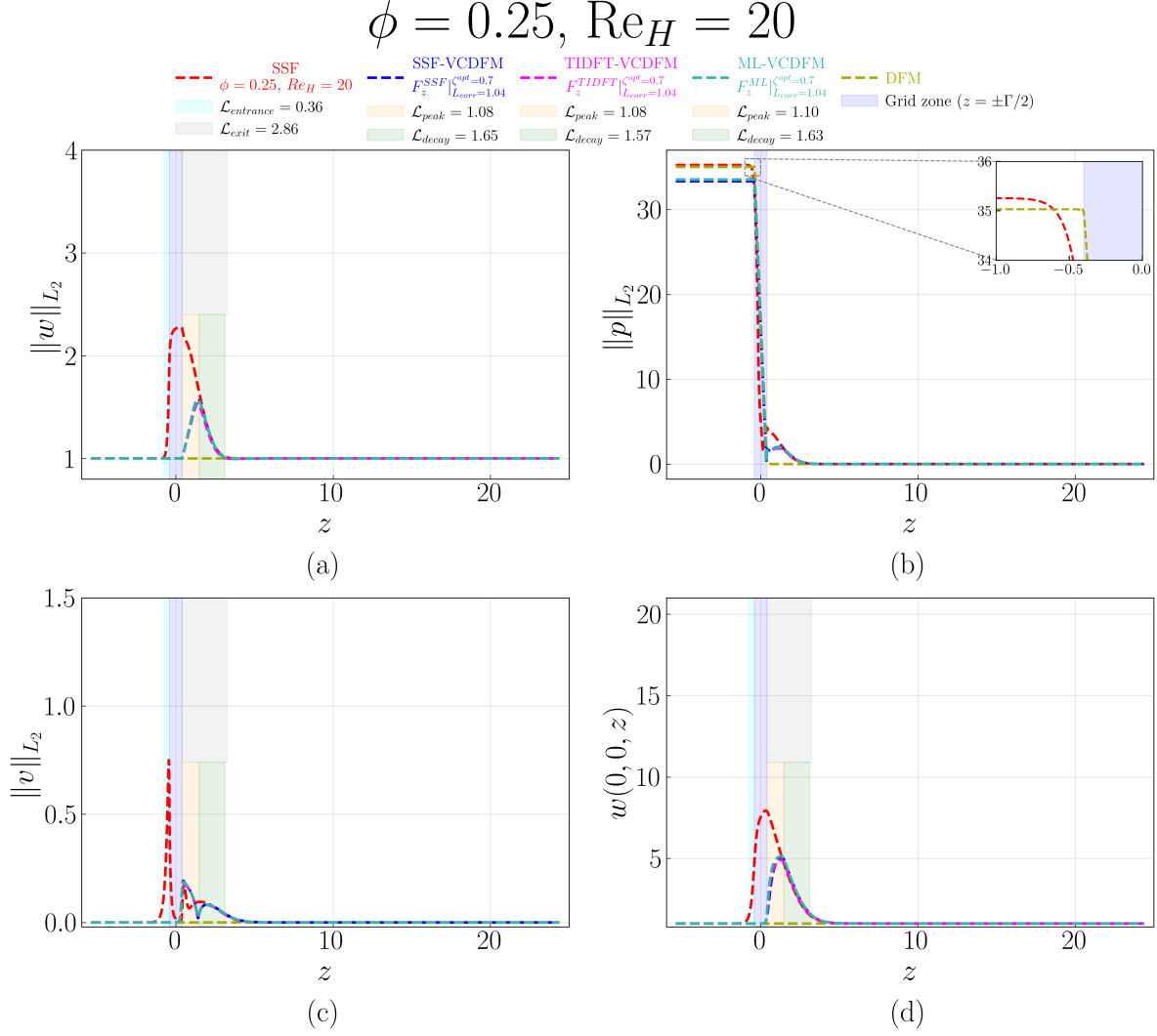
Figure D.195: Streamwise evolution of (a) \|w\|_{L_2} , (b) \|p\|_{L_2} , (c) \|v\|_{L_2} , and (d) centerline velocity w(0,0,z) for the 1 \times 1 SRG at \phi = 0.25 and \text{Re}_H = 20 . The figure compares the SSF, DFM, SSF-VCDFM, TIDFT-VCDFM, and ML-VCDFM. Shading marks the grid and the characteristic entrance, exit, peak, and decay regions. Only the SSF-based \mathcal{L}_{\text{peak}} and \mathcal{L}_{\text{decay}} are marked on the plot; the corresponding TIDFT-VCDFM and ML-VCDFM values appear in the legend.
