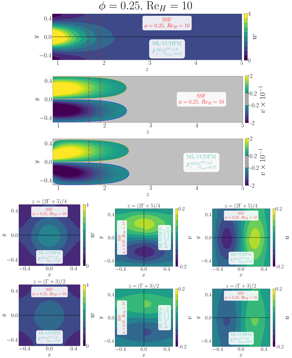
Figure D.194: Detailed comparison between the geometry-resolved small-scale flow (SSF) and ML-VCDFM using F_z^{ML} for the 1 \times 1 SRG at \phi = 0.25 and Re_H = 10 . The upper panels compare the streamwise velocity w and transverse velocity v in the central (z, y) -plane, restricted to the correction region. The lower panels compare the corresponding transverse (x, y) -plane distributions of w , v , and u , from left to right, at z = (2\Gamma + 5)/4 in the first row and z = (\Gamma + 3)/2 in the second row.
