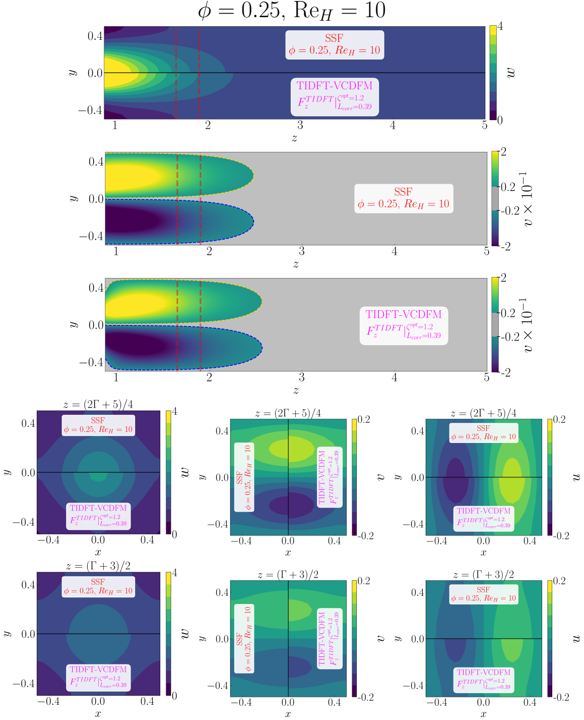
Figure D.193: Detailed comparison between the geometry-resolved small-scale flow (SSF) and TIDFT-VCDFM using F_z^{TIDFT} for the 1 \times 1 SRG at \phi = 0.25 and Re_H = 10 . The upper panels compare the streamwise velocity w and transverse velocity v in the central (z, y) -plane, restricted to the correction region. The lower panels compare the corresponding transverse (x, y) -plane distributions of w , v , and u , from left to right, at z = (2\Gamma + 5)/4 in the first row and z = (\Gamma + 3)/2 in the second row.
