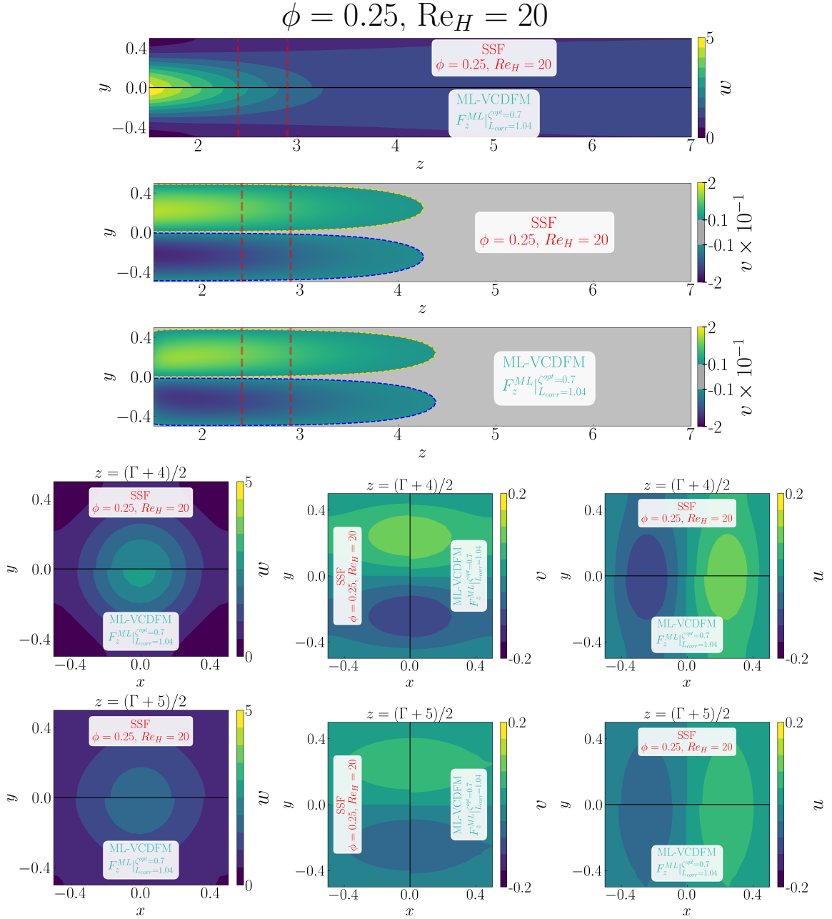
Figure D.200: Detailed comparison between the geometry-resolved small-scale flow (SSF) and ML-VCDFM using F_z^{\text{ML}} for the 1 \times 1 SRG at \phi = 0.25 and \text{Re}_H = 20 . The upper panels compare the streamwise velocity w and transverse velocity v in the central (z, y) -plane, restricted to the correction region. The lower panels compare the corresponding transverse (x, y) -plane distributions of w , v , and u , from left to right, at z = (\Gamma + 4)/2 in the first row and z = (\Gamma + 5)/2 in the second row.
