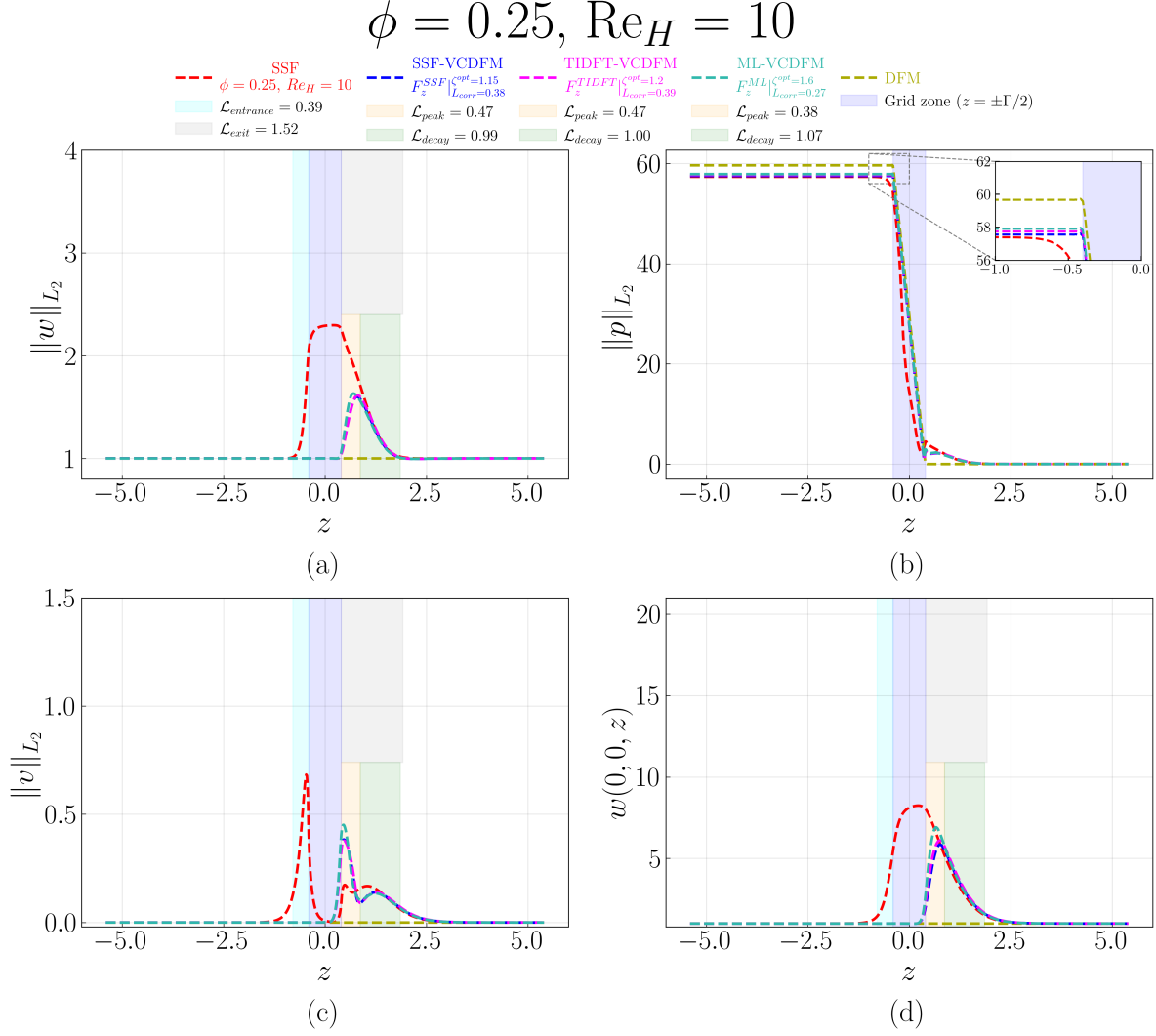
Figure D.189: Streamwise evolution of (a) \|w\|_{L_2} , (b) \|p\|_{L_2} , (c) \|v\|_{L_2} , and (d) centerline velocity w(0,0,z) for the 1 \times 1 SRG at \phi = 0.25 and \text{Re}_H = 10 . The figure compares the SSF, DFM, SSF-VCDFM, TIDFT-VCDFM, and ML-VCDFM. Shading marks the grid and the characteristic entrance, exit, peak, and decay regions. Only the SSF-based \mathcal{L}_{\text{peak}} and \mathcal{L}_{\text{decay}} are marked on the plot; the corresponding TIDFT-VCDFM and ML-VCDFM values appear in the legend.
