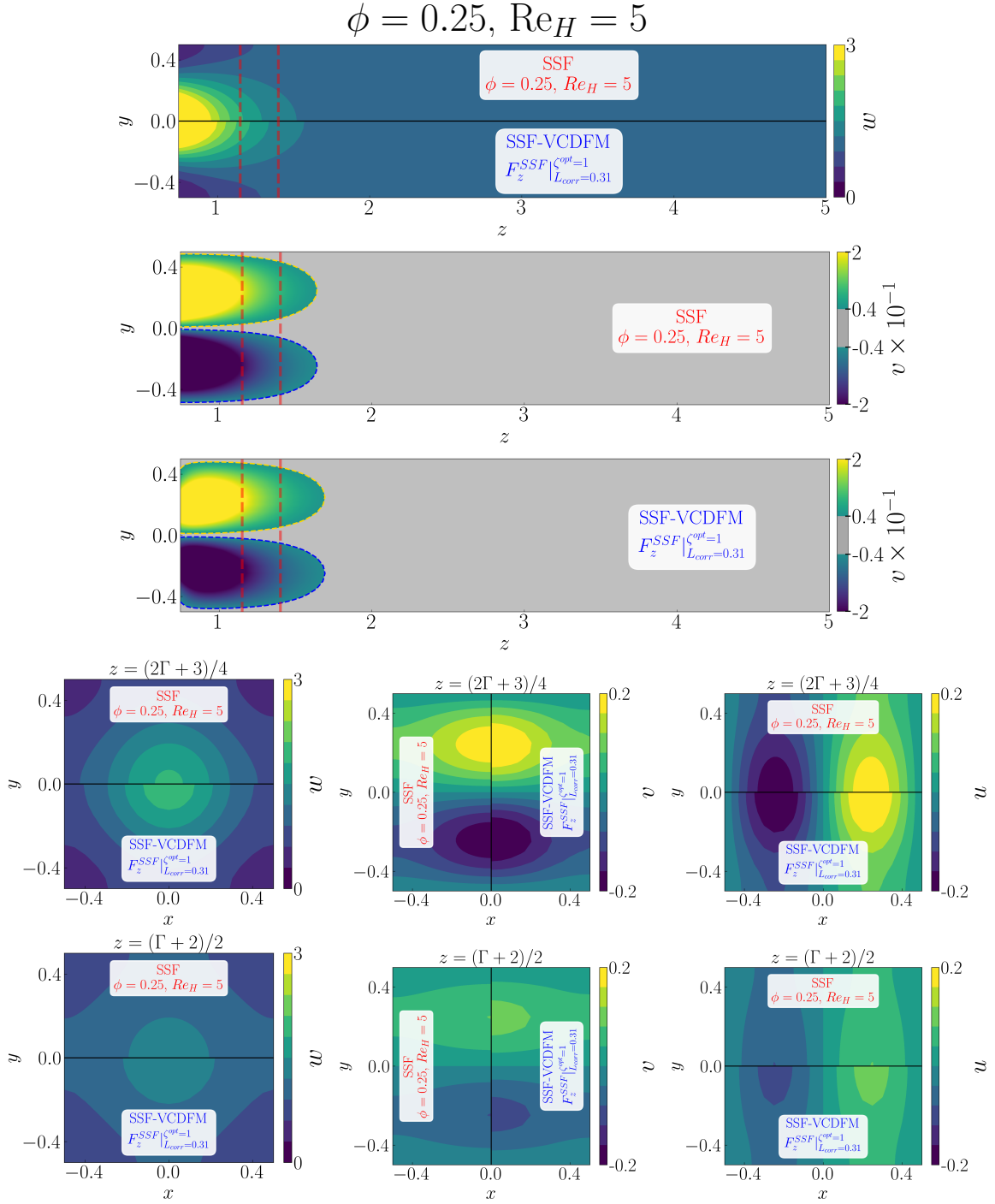
Figure D.186: Detailed comparison between the geometry-resolved small-scale flow (SSF) and SSF-VCDFM using F_z^{SSF} for the 1 \times 1 SRG at \phi = 0.25 and Re_H = 5 . The upper panels compare the streamwise velocity w and transverse velocity v in the central (z, y) -plane, restricted to the correction region. The lower panels compare the corresponding transverse (x, y) -plane distributions of w , v , and u , from left to right, at z = (2\Gamma + 3)/4 in the first row and z = (\Gamma + 2)/2 in the second row.
