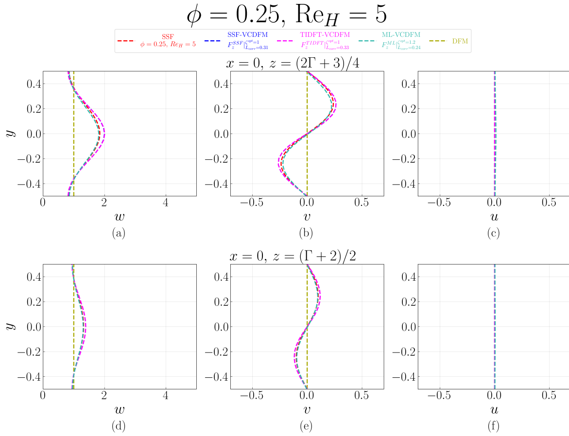
Figure D.185: Velocity profiles at x = 0 for the 1 \times 1 SRG at \phi = 0.25 and \text{Re}_H = 5 , comparing the SSF, DFM, SSF-VCDFM, TIDFT-VCDFM, and ML-VCDFM. Profiles of w(y) , v(y) , and u(y) are shown at z = (2\Gamma + 3)/4 in (a–c) and z = (\Gamma + 2)/2 in (d–f).
