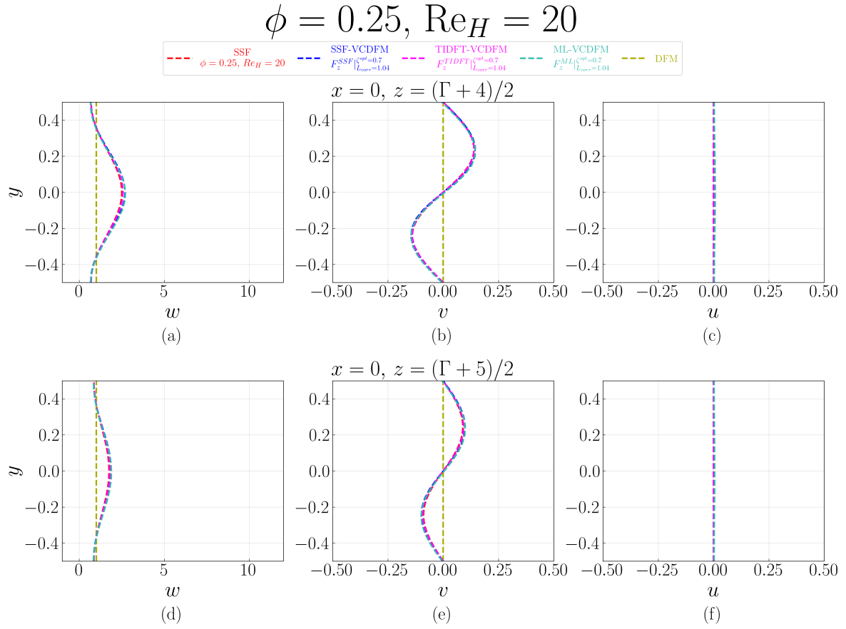
Figure D.197: Velocity profiles at x = 0 for the 1 \times 1 SRG at \phi = 0.25 and \text{Re}_H = 20 , comparing the SSF, DFM, SSF-VCDFM, TIDFT-VCDFM, and ML-VCDFM. Profiles of w(y) , v(y) , and u(y) are shown at z = (\Gamma + 4)/2 in (a–c) and z = (\Gamma + 5)/2 in (d–f).
