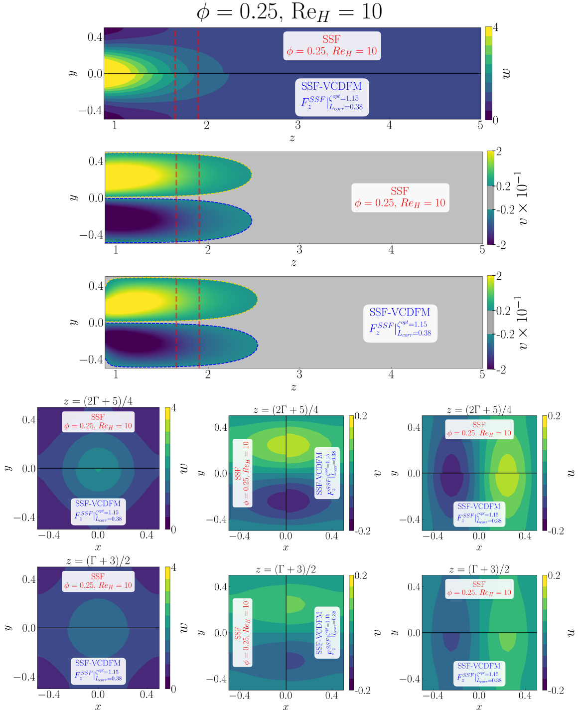
Figure D.192: Detailed comparison between the geometry-resolved small-scale flow (SSF) and SSF-VCDFM using F_z^{SSF} for the 1 \times 1 SRG at \phi = 0.25 and Re_H = 10 . The upper panels compare the streamwise velocity w and transverse velocity v in the central (z, y) -plane, restricted to the correction region. The lower panels compare the corresponding transverse (x, y) -plane distributions of w , v , and u , from left to right, at z = (2\Gamma + 5)/4 in the first row and z = (\Gamma + 3)/2 in the second row.
