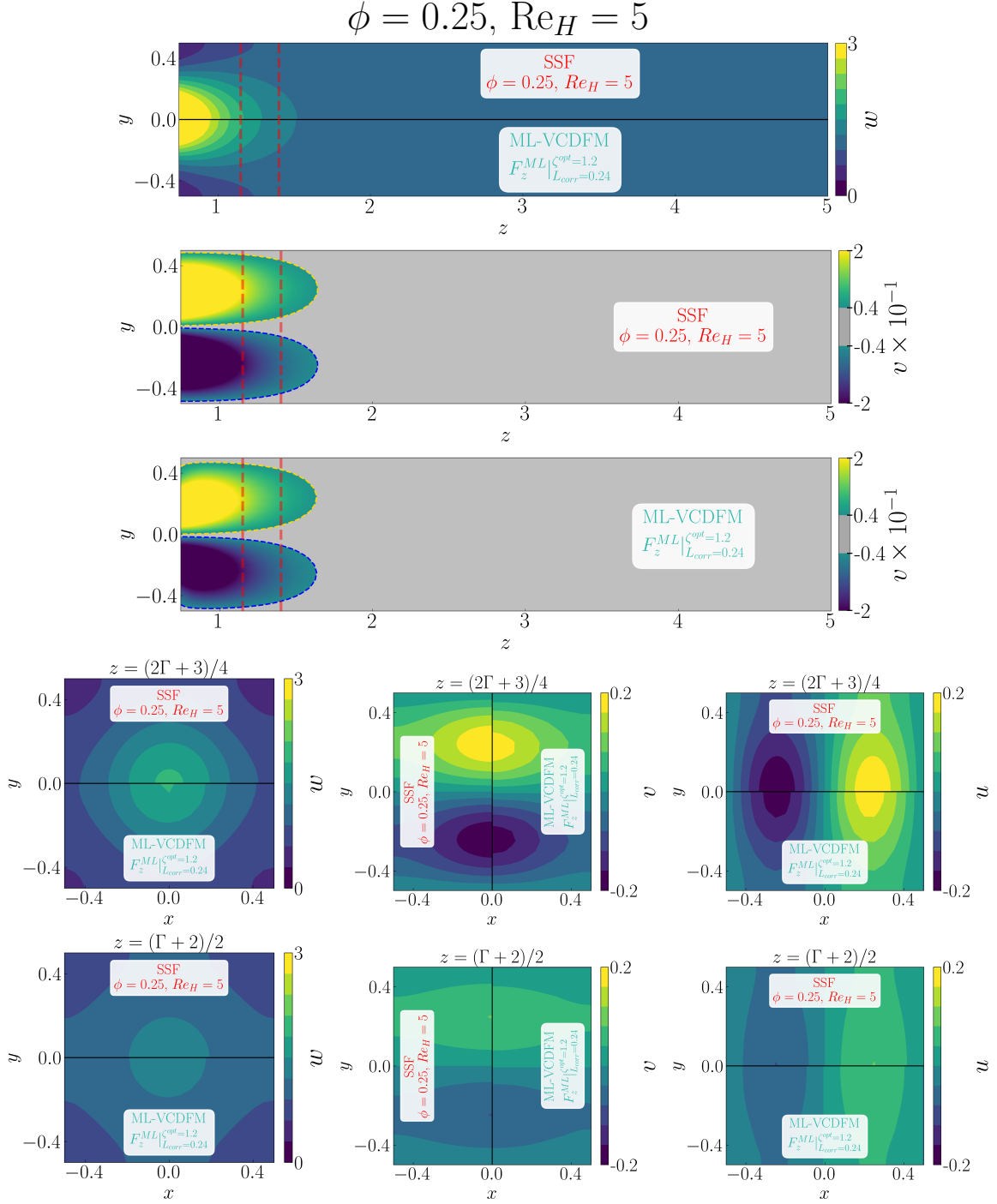
Figure D.188: Detailed comparison between the geometry-resolved small-scale flow (SSF) and ML-VCDFM using F_z^{\text{ML}} for the 1 \times 1 SRG at \phi = 0.25 and \text{Re}_H = 5 . The upper panels compare the streamwise velocity w and transverse velocity v in the central (z, y) -plane, restricted to the correction region. The lower panels compare the corresponding transverse (x, y) -plane distributions of w , v , and u , from left to right, at z = (2\Gamma + 3)/4 in the first row and z = (\Gamma + 2)/2 in the second row.
