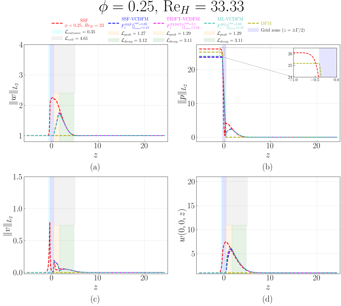
Figure D.201: Streamwise evolution of (a) \|w\|_{L_2} , (b) \|p\|_{L_2} , (c) \|v\|_{L_2} , and (d) centerline velocity w(0,0,z) for the 1 \times 1 SRG at \phi = 0.25 and \text{Re}_H = 33.33 . The figure compares the SSF, DFM, SSF-VCDFM, TIDFT-VCDFM, and ML-VCDFM. Shading marks the grid and the characteristic entrance, exit, peak, and decay regions. Only the SSF-based \mathcal{L}_{\text{peak}} and \mathcal{L}_{\text{decay}} are marked on the plot; the corresponding TIDFT-VCDFM and ML-VCDFM values appear in the legend.
