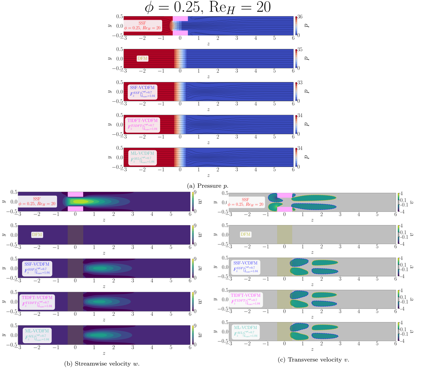
Figure D.196: Flow organization in the streamwise (z, y) -plane for the 1 \times 1 SRG at \phi = 0.25 , Re_H = 20 , and \alpha = 0^\circ . The blocks show (a) pressure p with streamlines, (b) streamwise velocity w , and (c) transverse velocity v . Within each block, the rows show, from top to bottom, the SSF, DFM, SSF-VCDFM, TIDFT-VCDFM, and ML-VCDFM. Pink shading marks the grid walls in the SSF; olive shading marks the equivalent porous zone in the model solutions.
