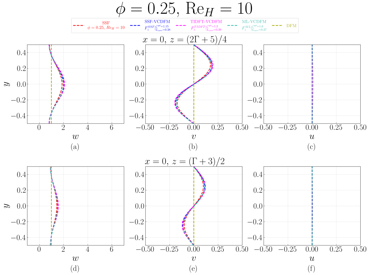
Figure D.191: Velocity profiles at x = 0 for the 1 \times 1 SRG at \phi = 0.25 and \text{Re}_H = 10 , comparing the SSF, DFM, SSF-VCDFM, TIDFT-VCDFM, and ML-VCDFM. Profiles of w(y) , v(y) , and u(y) are shown at z = (2\Gamma + 5)/4 in (a–c) and z = (\Gamma + 3)/2 in (d–f).
