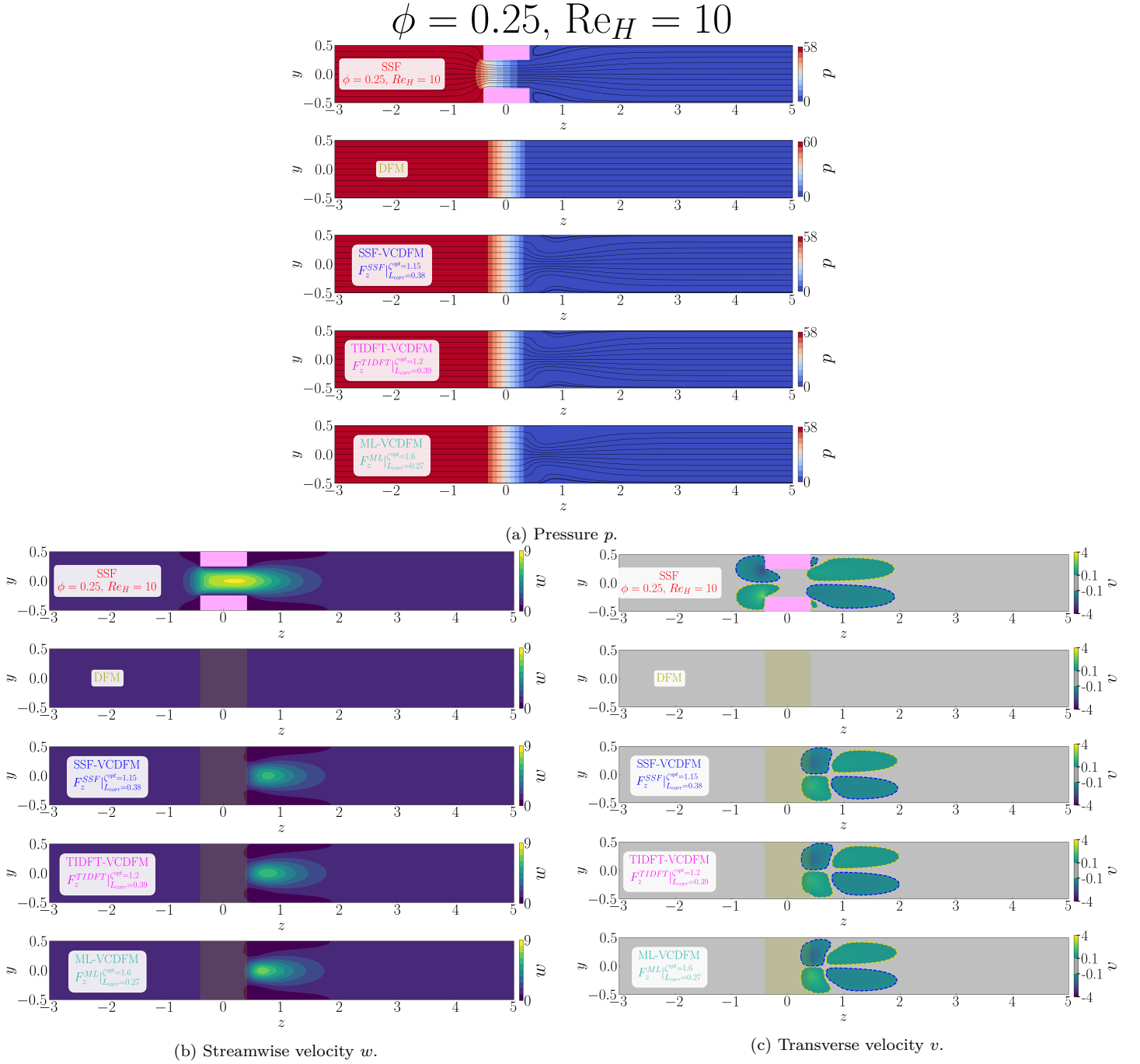
Figure D.190: Flow organization in the streamwise (z, y) -plane for the 1 \times 1 SRG at \phi = 0.25 , \text{Re}_H = 10 , and \alpha = 0^\circ . The blocks show (a) pressure p with streamlines, (b) streamwise velocity w , and (c) transverse velocity v . Within each block, the rows show, from top to bottom, the SSF, DFM, SSF-VCDFM, TIDFT-VCDFM, and ML-VCDFM. Pink shading marks the grid walls in the SSF; olive shading marks the equivalent porous zone in the model solutions.
