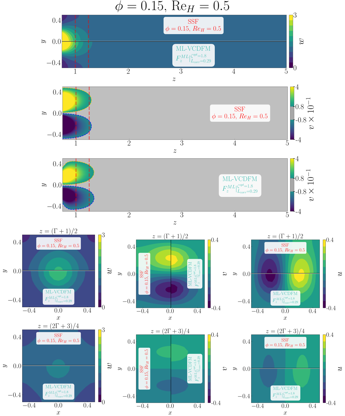
Figure D.74: Detailed comparison between the geometry-resolved small-scale flow (SSF) and ML-VCDFM using F_z^{\text{ML}} for the 1 \times 1 SRG at \phi = 0.15 and \text{Re}_H = 0.5 . The upper panels compare the streamwise velocity w and transverse velocity v in the central (z, y) -plane, restricted to the correction region. The lower panels compare the corresponding transverse (x, y) -plane distributions of w , v , and u , from left to right, at z = (\Gamma + 1)/2 in the first row and z = (2\Gamma + 3)/4 in the second row.
