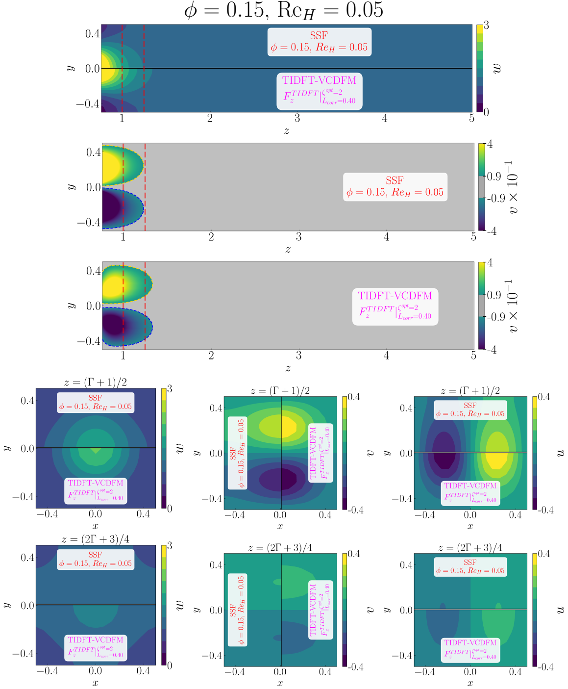
Figure D.61: Detailed comparison between the geometry-resolved small-scale flow (SSF) and TIDFT-VCDFM using F_z^{\text{TIDFT}} for the 1 \times 1 SRG at \phi = 0.15 and Re_H = 0.05 . The upper panels compare the streamwise velocity w and transverse velocity v in the central (z, y) -plane, restricted to the correction region. The lower panels compare the corresponding transverse (x, y) -plane distributions of w , v , and u , from left to right, at z = (\Gamma + 1)/2 in the first row and z = (2\Gamma + 3)/4 in the second row.
