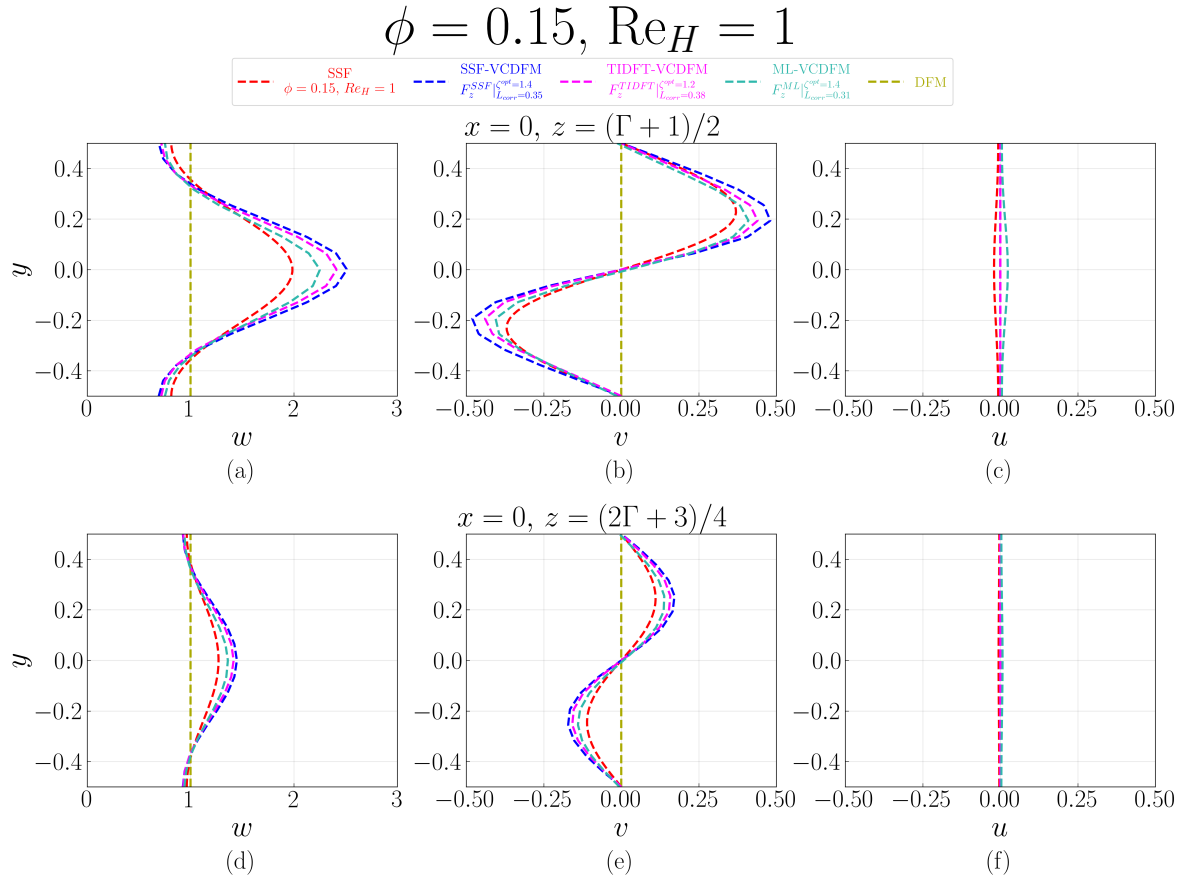
Figure D.77: Velocity profiles at x = 0 for the 1 \times 1 SRG at \phi = 0.15 and \text{Re}_H = 1 , comparing the SSF, DFM, SSF-VCDFM, TIDFT-VCDFM, and ML-VCDFM. Profiles of w(y) , v(y) , and u(y) are shown at z = (\Gamma + 1)/2 in (a–c) and z = (2\Gamma + 3)/4 in (d–f).
