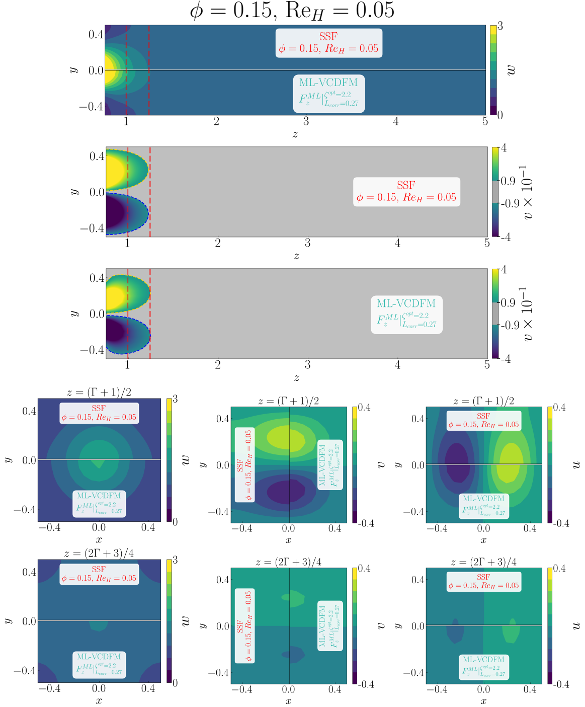
Figure D.62: Detailed comparison between the geometry-resolved small-scale flow (SSF) and ML-VCDFM using F_z^{ML} for the 1 \times 1 SRG at \phi = 0.15 and Re_H = 0.05 . The upper panels compare the streamwise velocity w and transverse velocity v in the central (z, y) -plane, restricted to the correction region. The lower panels compare the corresponding transverse (x, y) -plane distributions of w , v , and u , from left to right, at z = (\Gamma + 1)/2 in the first row and z = (2\Gamma + 3)/4 in the second row.
