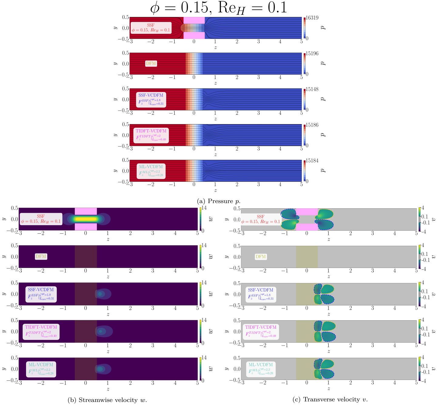
Figure D.64: Flow organization in the streamwise (z, y) -plane for the 1 \times 1 SRG at \phi = 0.15 , \text{Re}_H = 0.1 , and \alpha = 0^\circ . The blocks show (a) pressure p with streamlines, (b) streamwise velocity w , and (c) transverse velocity v . Within each block, the rows show, from top to bottom, the SSF, DFM, SSF-VCDFM, TIDFT-VCDFM, and ML-VCDFM. Pink shading marks the grid walls in the SSF; olive shading marks the equivalent porous zone in the model solutions.
