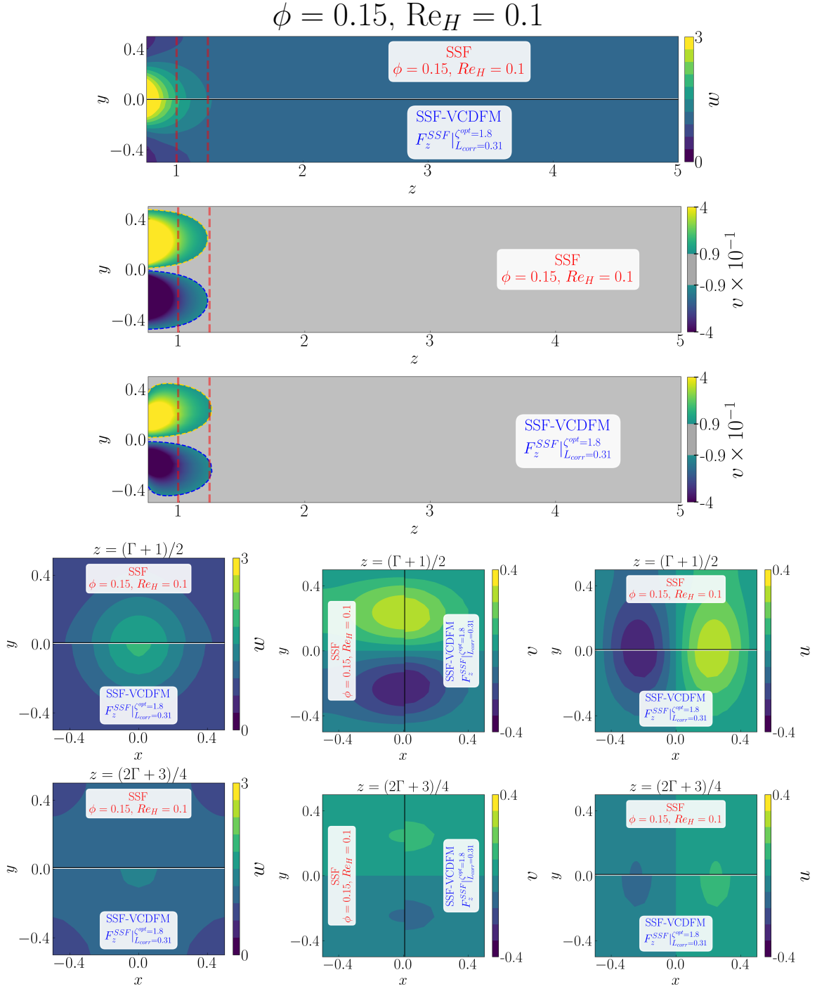
Figure D.66: Detailed comparison between the geometry-resolved small-scale flow (SSF) and SSF-VCDFM using F_z^{\text{SSF}} for the 1 \times 1 SRG at \phi = 0.15 and Re_H = 0.1 . The upper panels compare the streamwise velocity w and transverse velocity v in the central (z, y) -plane, restricted to the correction region. The lower panels compare the corresponding transverse (x, y) -plane distributions of w , v , and u , from left to right, at z = (\Gamma + 1)/2 in the first row and z = (2\Gamma + 3)/4 in the second row.
