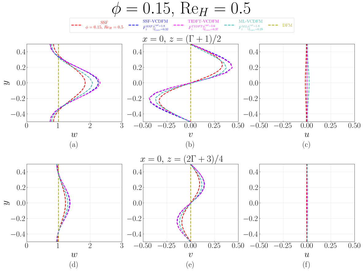
Figure D.71: Velocity profiles at x = 0 for the 1 \times 1 SRG at \phi = 0.15 and \text{Re}_H = 0.5 , comparing the SSF, DFM, SSF-VCDFM, TIDFT-VCDFM, and ML-VCDFM. Profiles of w(y) , v(y) , and u(y) are shown at z = (\Gamma + 1)/2 in (a–c) and z = (2\Gamma + 3)/4 in (d–f).
