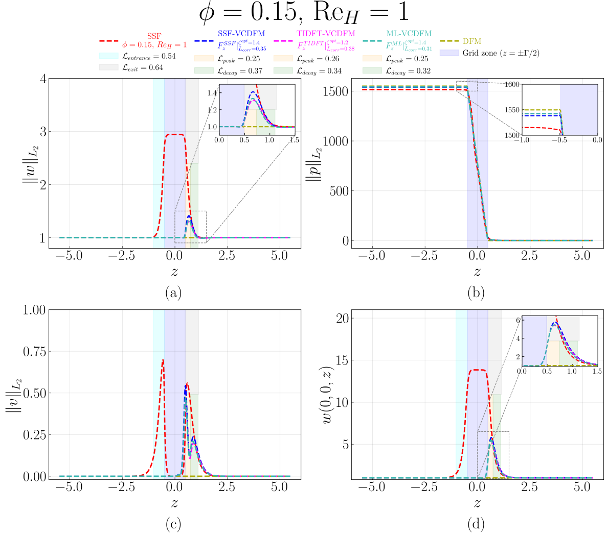
Figure D.75: Streamwise evolution of (a) \|w\|_{L_2} , (b) \|p\|_{L_2} , (c) \|v\|_{L_2} , and (d) centerline velocity w(0,0,z) for the 1 \times 1 SRG at \phi = 0.15 and \text{Re}_H = 1 . The figure compares the SSF, DFM, SSF-VCDFM, TIDFT-VCDFM, and ML-VCDFM. Shading marks the grid and the characteristic entrance, exit, peak, and decay regions. Only the SSF-based \mathcal{L}_{\text{peak}} and \mathcal{L}_{\text{decay}} are marked on the plot; the corresponding TIDFT-VCDFM and ML-VCDFM values appear in the legend.
