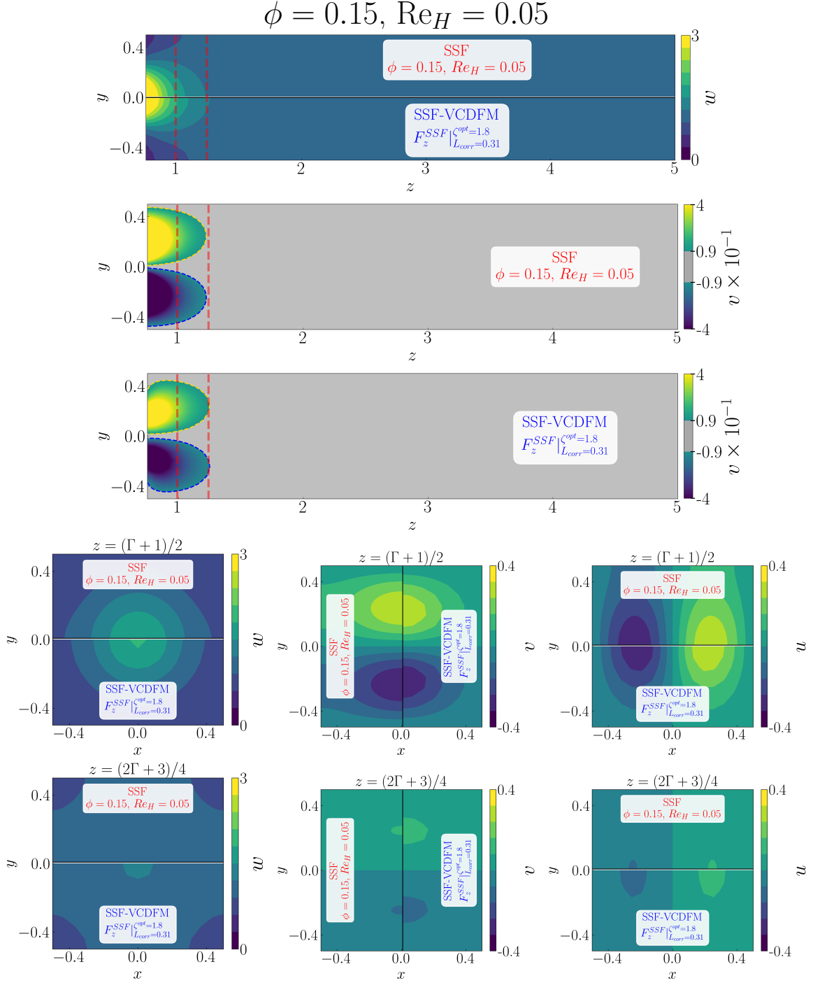
Figure D.60: Detailed comparison between the geometry-resolved small-scale flow (SSF) and SSF-VCDFM using F_z^{SSF} for the 1 \times 1 SRG at \phi = 0.15 and Re_H = 0.05 . The upper panels compare the streamwise velocity w and transverse velocity v in the central (z, y) -plane, restricted to the correction region. The lower panels compare the corresponding transverse (x, y) -plane distributions of w , v , and u , from left to right, at z = (\Gamma + 1)/2 in the first row and z = (2\Gamma + 3)/4 in the second row.
