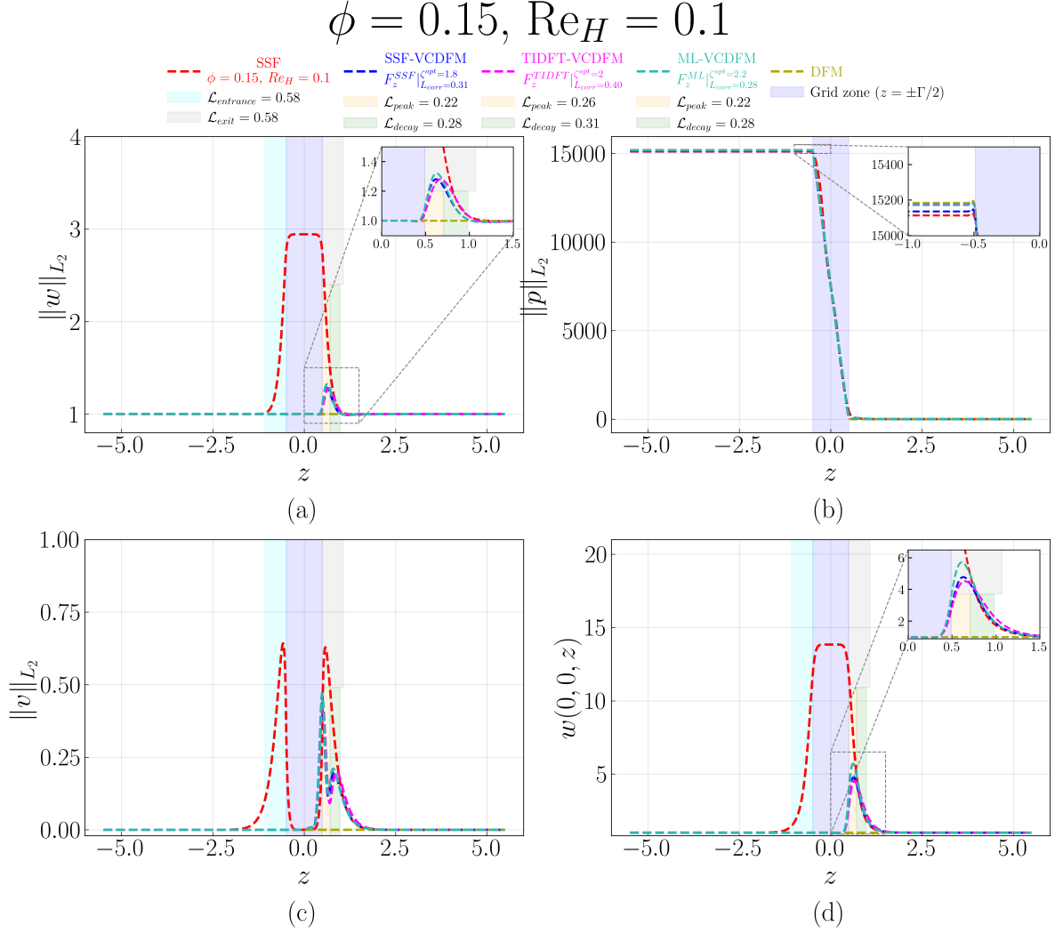
Figure D.63: Streamwise evolution of (a) \|w\|_{L_2} , (b) \|p\|_{L_2} , (c) \|v\|_{L_2} , and (d) centerline velocity w(0,0,z) for the 1 \times 1 SRG at \phi = 0.15 and \text{Re}_H = 0.1 . The figure compares the SSF, DFM, SSF-VCDFM, TIDFT-VCDFM, and ML-VCDFM. Shading marks the grid and the characteristic entrance, exit, peak, and decay regions. Only the SSF-based \mathcal{L}_{\text{peak}} and \mathcal{L}_{\text{decay}} are marked on the plot; the corresponding TIDFT-VCDFM and ML-VCDFM values appear in the legend.
