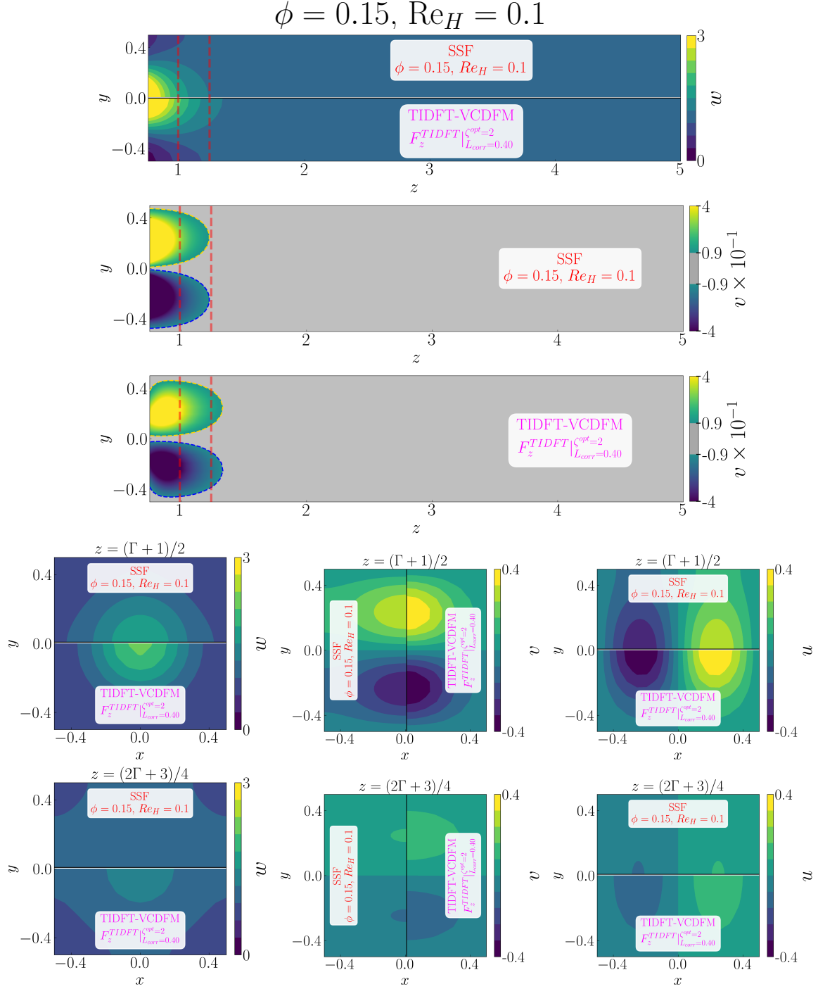
Figure D.67: Detailed comparison between the geometry-resolved small-scale flow (SSF) and TIDFT-VCDFM using F_z^{TIDFT} for the 1 \times 1 SRG at \phi = 0.15 and Re_H = 0.1 . The upper panels compare the streamwise velocity w and transverse velocity v in the central (z, y) -plane, restricted to the correction region. The lower panels compare the corresponding transverse (x, y) -plane distributions of w , v , and u , from left to right, at z = (\Gamma + 1)/2 in the first row and z = (2\Gamma + 3)/4 in the second row.
