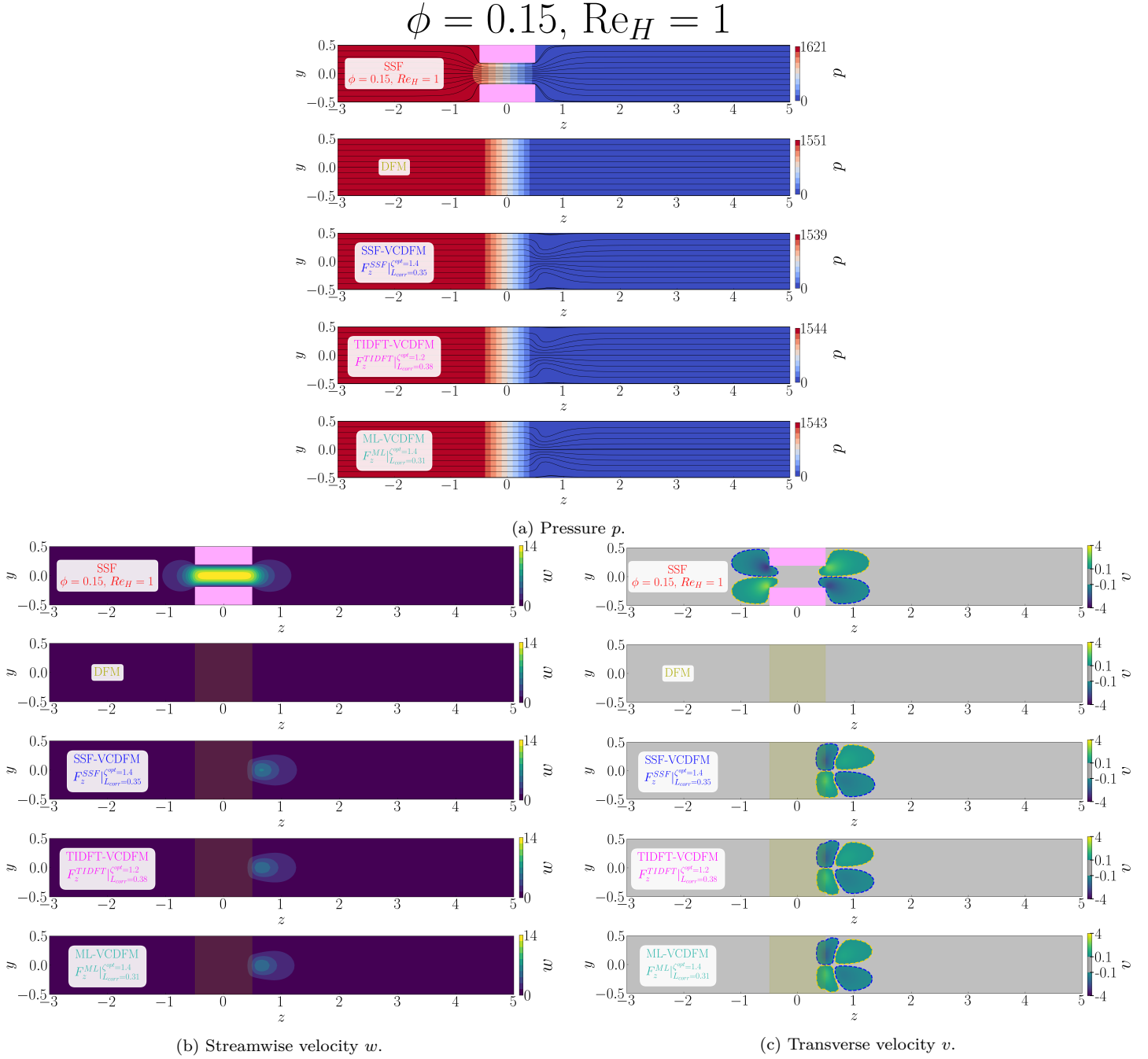
Figure D.76: Flow organization in the streamwise (z, y) -plane for the 1 \times 1 SRG at \phi = 0.15 , Re_H = 1 , and \alpha = 0^\circ . The blocks show (a) pressure p with streamlines, (b) streamwise velocity w , and (c) transverse velocity v . Within each block, the rows show, from top to bottom, the SSF, DFM, SSF-VCDFM, TIDFT-VCDFM, and ML-VCDFM. Pink shading marks the grid walls in the SSF; olive shading marks the equivalent porous zone in the model solutions.
