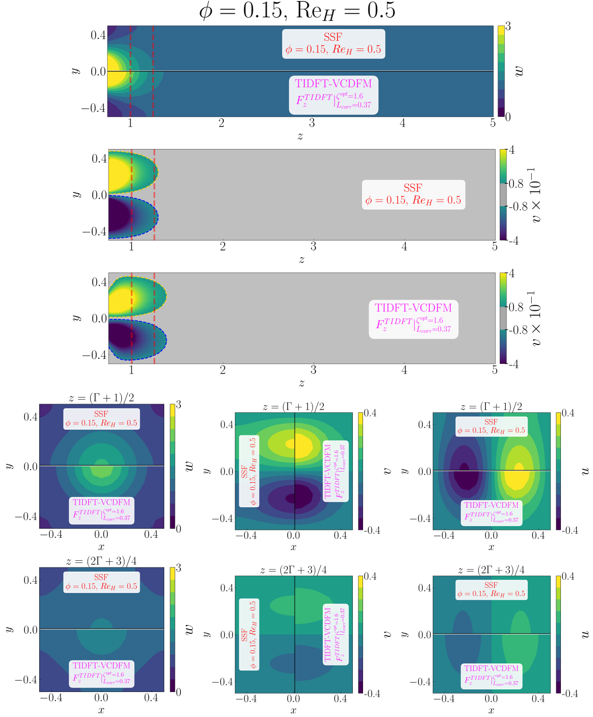
Figure D.73: Detailed comparison between the geometry-resolved small-scale flow (SSF) and TIDFT-VCDFM using F_z^{TIDFT} for the 1 \times 1 SRG at \phi = 0.15 and Re_H = 0.5 . The upper panels compare the streamwise velocity w and transverse velocity v in the central (z, y) -plane, restricted to the correction region. The lower panels compare the corresponding transverse (x, y) -plane distributions of w , v , and u , from left to right, at z = (\Gamma + 1)/2 in the first row and z = (2\Gamma + 3)/4 in the second row.
