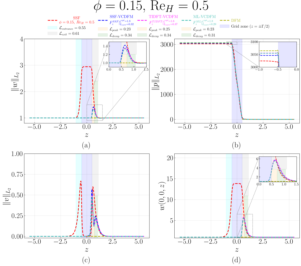
Figure D.69: Streamwise evolution of (a) \|w\|_{L_2} , (b) \|p\|_{L_2} , (c) \|v\|_{L_2} , and (d) centerline velocity w(0,0,z) for the 1 \times 1 SRG at \phi = 0.15 and \text{Re}_H = 0.5 . The figure compares the SSF, DFM, SSF-VCDFM, TIDFT-VCDFM, and ML-VCDFM. Shading marks the grid and the characteristic entrance, exit, peak, and decay regions. Only the SSF-based \mathcal{L}_{\text{peak}} and \mathcal{L}_{\text{decay}} are marked on the plot; the corresponding TIDFT-VCDFM and ML-VCDFM values appear in the legend.
