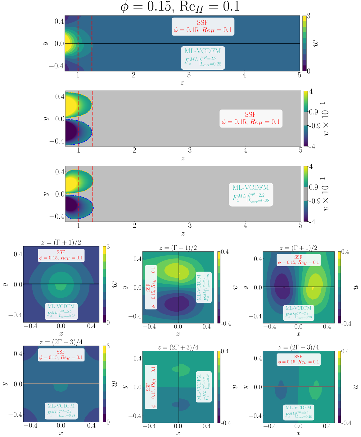
Figure D.68: Detailed comparison between the geometry-resolved small-scale flow (SSF) and ML-VCDFM using F_z^{\text{ML}} for the 1 \times 1 SRG at \phi = 0.15 and \text{Re}_H = 0.1 . The upper panels compare the streamwise velocity w and transverse velocity v in the central (z, y) -plane, restricted to the correction region. The lower panels compare the corresponding transverse (x, y) -plane distributions of w , v , and u , from left to right, at z = (\Gamma + 1)/2 in the first row and z = (2\Gamma + 3)/4 in the second row.
