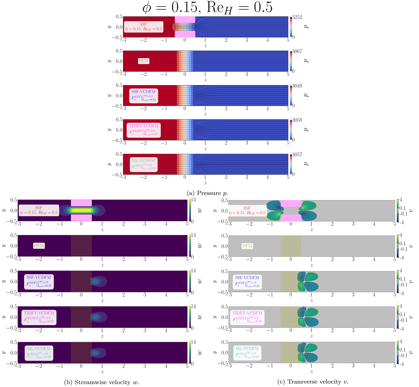
Figure D.70: Flow organization in the streamwise (z, y) -plane for the 1 \times 1 SRG at \phi = 0.15 , \text{Re}_H = 0.5 , and \alpha = 0^\circ . The blocks show (a) pressure p with streamlines, (b) streamwise velocity w , and (c) transverse velocity v . Within each block, the rows show, from top to bottom, the SSF, DFM, SSF-VCDFM, TIDFT-VCDFM, and ML-VCDFM. Pink shading marks the grid walls in the SSF; olive shading marks the equivalent porous zone in the model solutions.
