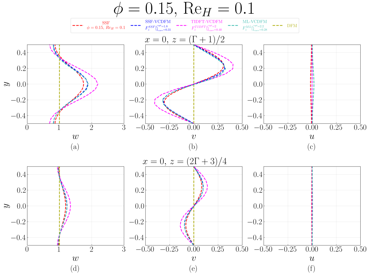
Figure D.65: Velocity profiles at x = 0 for the 1 \times 1 SRG at \phi = 0.15 and \text{Re}_H = 0.1 , comparing the SSF, DFM, SSF-VCDFM, TIDFT-VCDFM, and ML-VCDFM. Profiles of w(y) , v(y) , and u(y) are shown at z = (\Gamma + 1)/2 in (a–c) and z = (2\Gamma + 3)/4 in (d–f).
