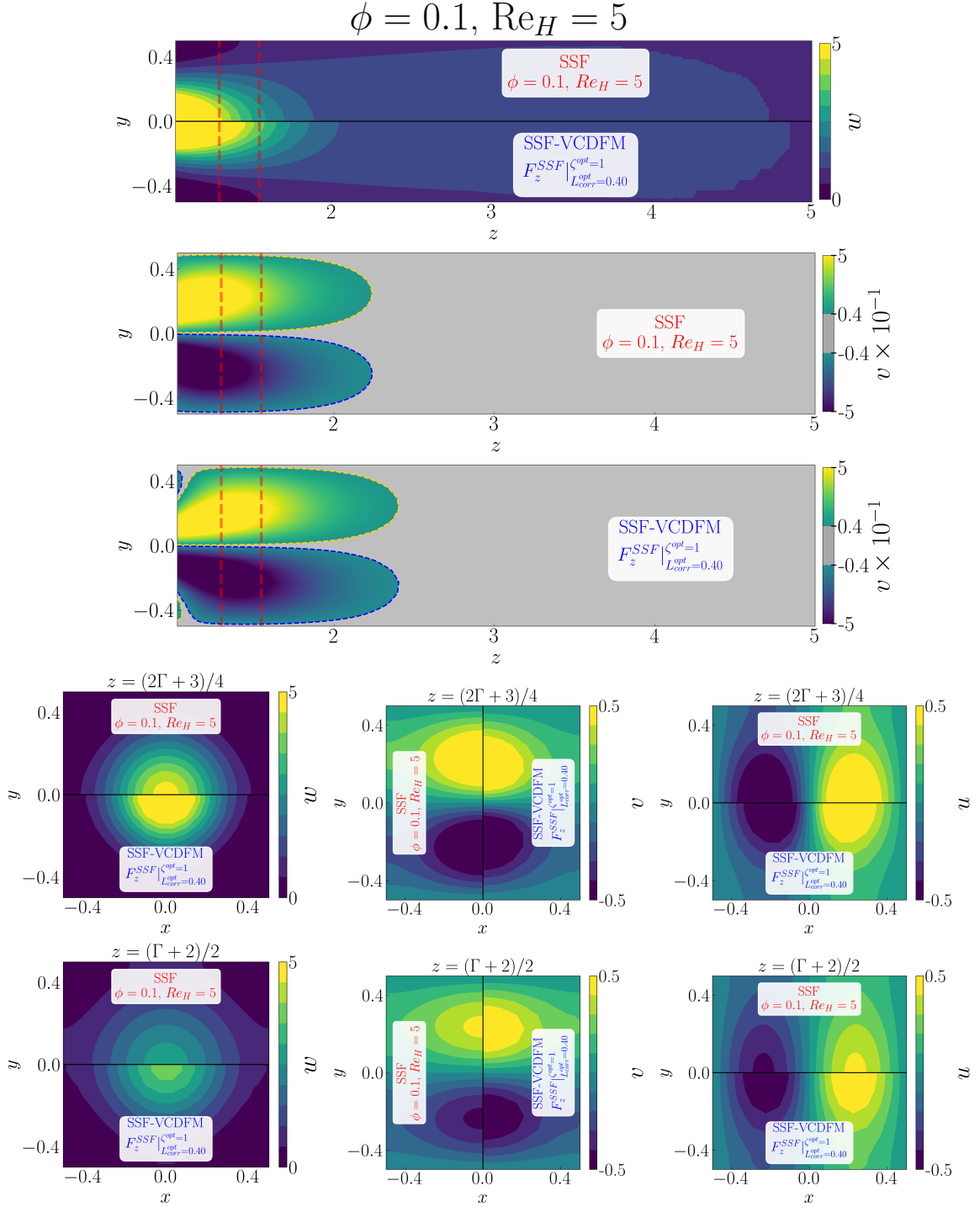
Figure D.42: Detailed comparison between the geometry-resolved small-scale flow (SSF) and SSF-VCDFM using F_z^{SSF} for the 1 \times 1 SRG at \phi = 0.1 and Re_H = 5 . The upper panels compare the streamwise velocity w and transverse velocity v in the central (z, y) -plane, restricted to the correction region. The lower panels compare the corresponding transverse (x, y) -plane distributions of w , v , and u , from left to right, at z = (2\Gamma + 3)/4 in the first row and z = (\Gamma + 2)/2 in the second row.
