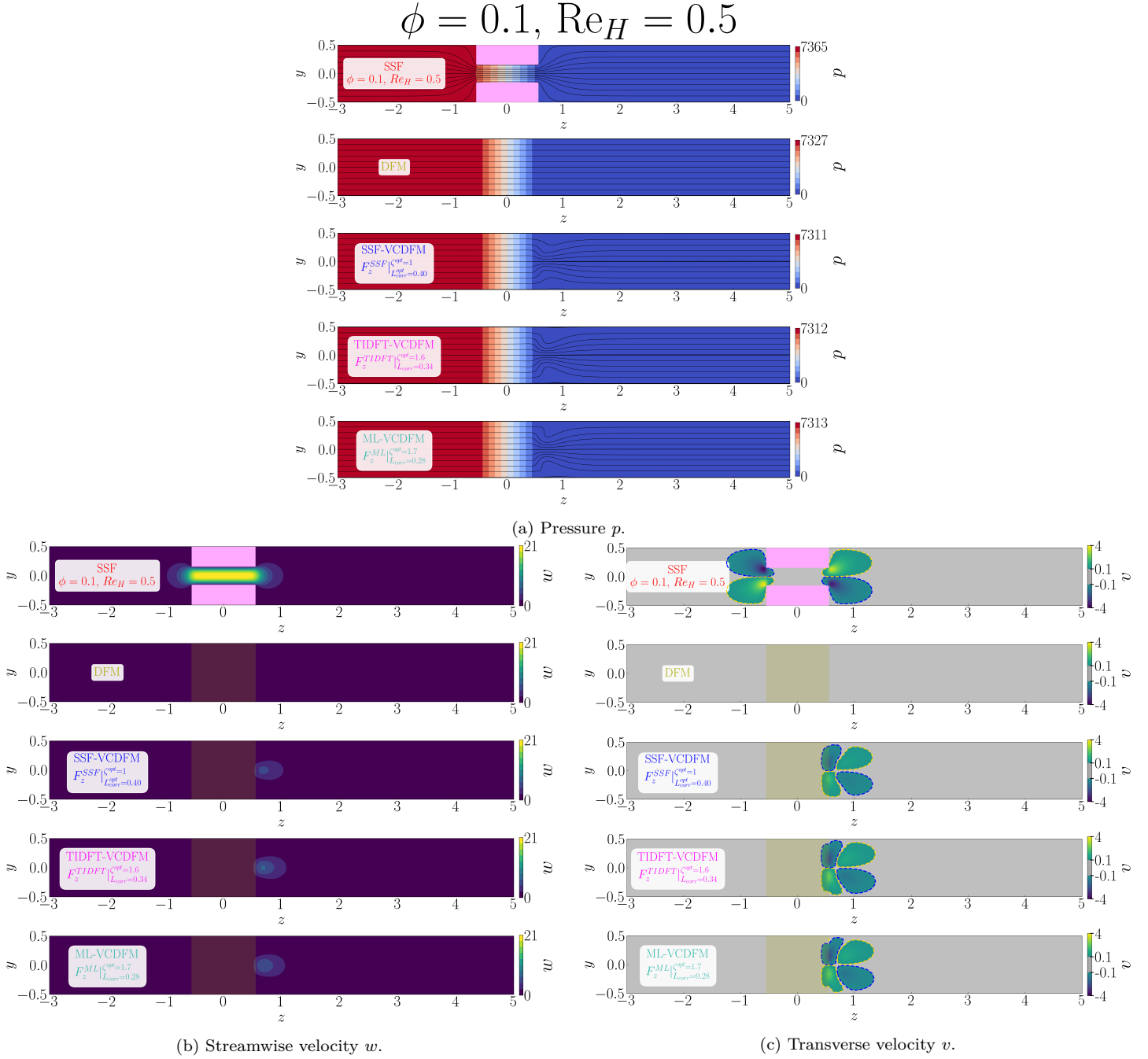
Figure D.28: Flow organization in the streamwise (z, y) -plane for the 1 \times 1 SRG at \phi = 0.1 , \text{Re}_H = 0.5 , and \alpha = 0^\circ . The blocks show (a) pressure p with streamlines, (b) streamwise velocity w , and (c) transverse velocity v . Within each block, the rows show, from top to bottom, the SSF, DFM, SSF-VCDFM, TIDFT-VCDFM, and ML-VCDFM. Pink shading marks the grid walls in the SSF; olive shading marks the equivalent porous zone in the model solutions.
