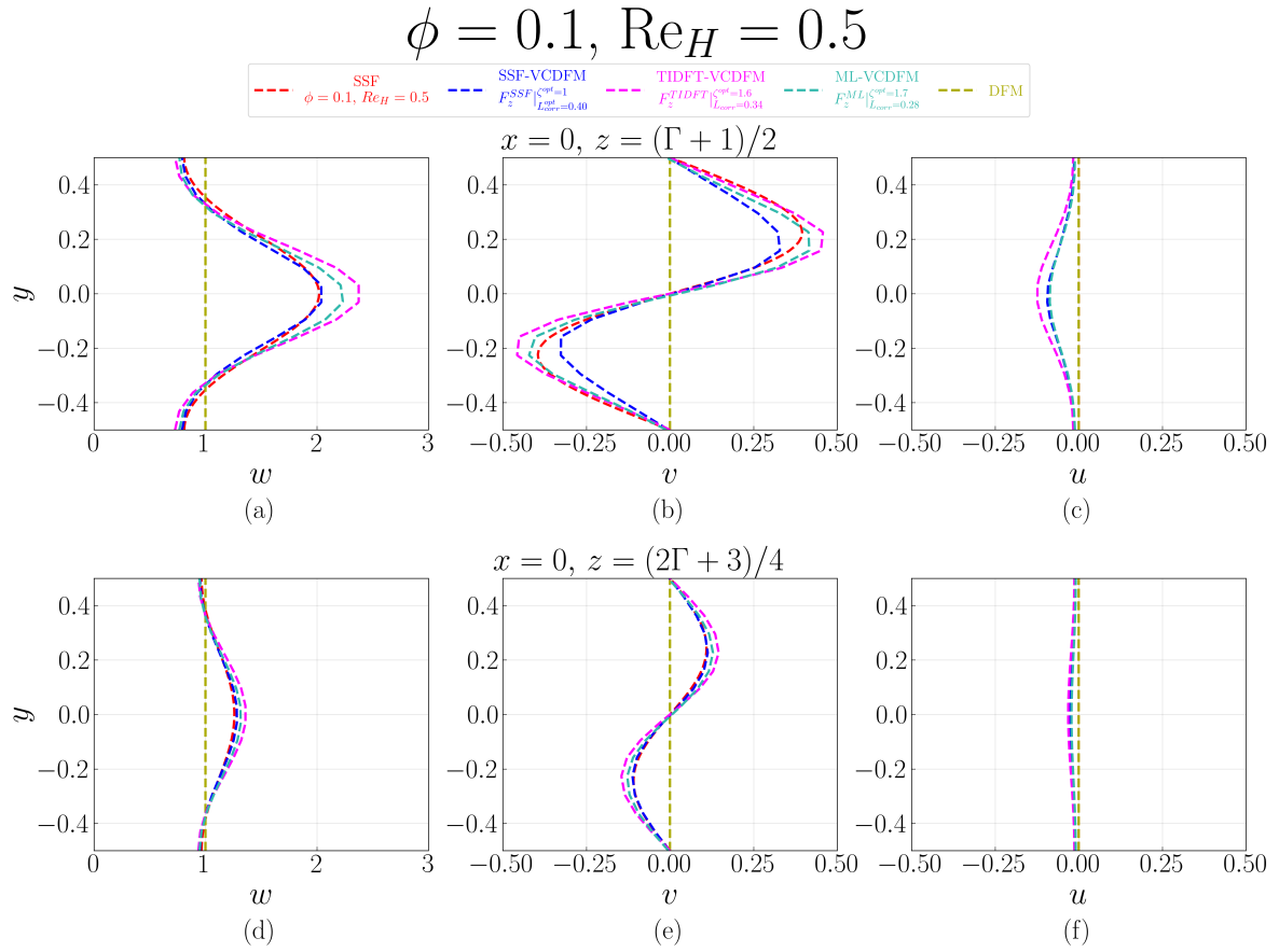
Figure D.29: Velocity profiles at x = 0 for the 1 \times 1 SRG at \phi = 0.1 and \text{Re}_H = 0.5 , comparing the SSF, DFM, SSF-VCDFM, TIDFT-VCDFM, and ML-VCDFM. Profiles of w(y) , v(y) , and u(y) are shown at z = (\Gamma + 1)/2 in (a–c) and z = (2\Gamma + 3)/4 in (d–f).
