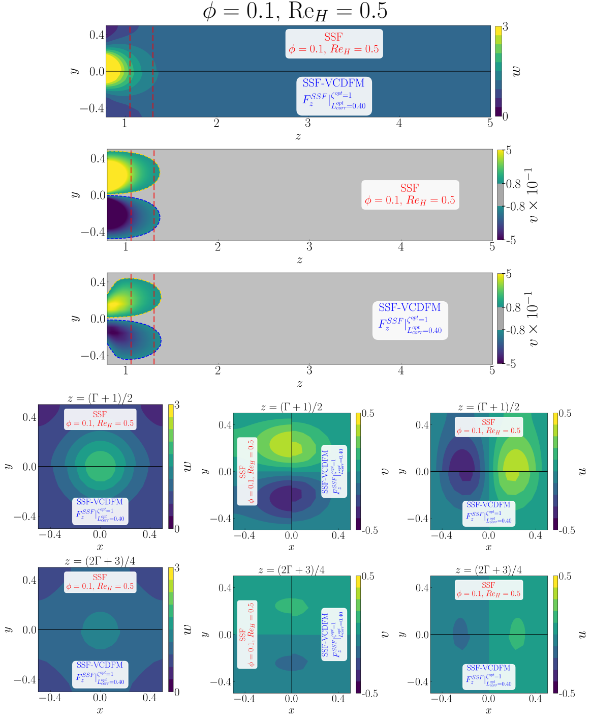
Figure D.30: Detailed comparison between the geometry-resolved small-scale flow (SSF) and SSF-VCDFM using F_z^{SSF} for the 1 \times 1 SRG at \phi = 0.1 and Re_H = 0.5 . The upper panels compare the streamwise velocity w and transverse velocity v in the central (z, y) -plane, restricted to the correction region. The lower panels compare the corresponding transverse (x, y) -plane distributions of w , v , and u , from left to right, at z = (\Gamma + 1)/2 in the first row and z = (2\Gamma + 3)/4 in the second row.
