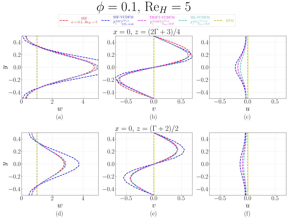
Figure D.41: Velocity profiles at x = 0 for the 1 \times 1 SRG at \phi = 0.1 and \text{Re}_H = 5 , comparing the SSF, DFM, SSF-VCDFM, TIDFT-VCDFM, and ML-VCDFM. Profiles of w(y) , v(y) , and u(y) are shown at z = (2\Gamma + 3)/4 in (a-c) and z = (\Gamma + 2)/2 in (d-f).
