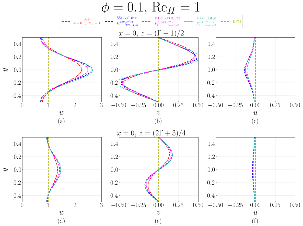
Figure D.35: Velocity profiles at x = 0 for the 1 \times 1 SRG at \phi = 0.1 and \text{Re}_H = 1 , comparing the SSF, DFM, SSF-VCDFM, TIDFT-VCDFM, and ML-VCDFM. Profiles of w(y) , v(y) , and u(y) are shown at z = (\Gamma + 1)/2 in (a–c) and z = (2\Gamma + 3)/4 in (d–f).
