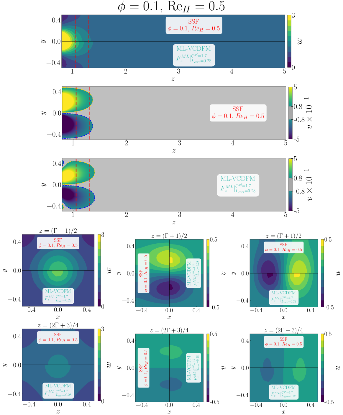
Figure D.32: Detailed comparison between the geometry-resolved small-scale flow (SSF) and ML-VCDFM using F_z^{ML} for the 1 \times 1 SRG at \phi = 0.1 and Re_H = 0.5 . The upper panels compare the streamwise velocity w and transverse velocity v in the central (z, y) -plane, restricted to the correction region. The lower panels compare the corresponding transverse (x, y) -plane distributions of w , v , and u , from left to right, at z = (\Gamma + 1)/2 in the first row and z = (2\Gamma + 3)/4 in the second row.
