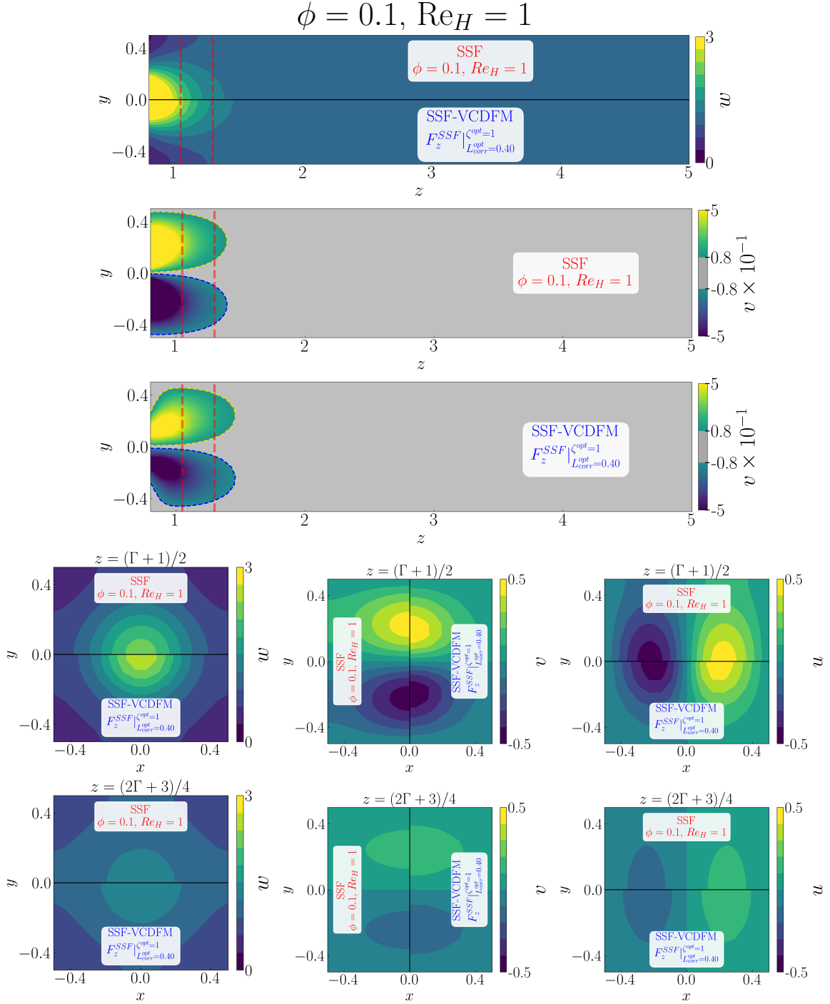
Figure D.36: Detailed comparison between the geometry-resolved small-scale flow (SSF) and SSF-VCDFM using F_z^{SSF} for the 1 \times 1 SRG at \phi = 0.1 and Re_H = 1 . The upper panels compare the streamwise velocity w and transverse velocity v in the central (z, y) -plane, restricted to the correction region. The lower panels compare the corresponding transverse (x, y) -plane distributions of w , v , and u , from left to right, at z = (\Gamma + 1)/2 in the first row and z = (2\Gamma + 3)/4 in the second row.
