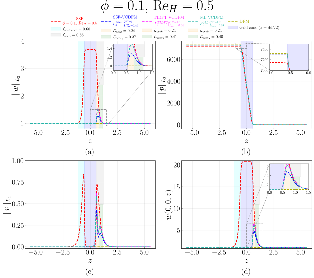
Figure D.27: Streamwise evolution of (a) \|w\|_{L_2} , (b) \|p\|_{L_2} , (c) \|v\|_{L_2} , and (d) centerline velocity w(0,0,z) for the 1 \times 1 SRG at \phi = 0.1 and \text{Re}_H = 0.5 . The figure compares the SSF, DFM, SSF-VCDFM, TIDFT-VCDFM, and ML-VCDFM. Shading marks the grid and the characteristic entrance, exit, peak, and decay regions. Only the SSF-based \mathcal{L}_{\text{peak}} and \mathcal{L}_{\text{decay}} are marked on the plot; the corresponding TIDFT-VCDFM and ML-VCDFM values appear in the legend.
