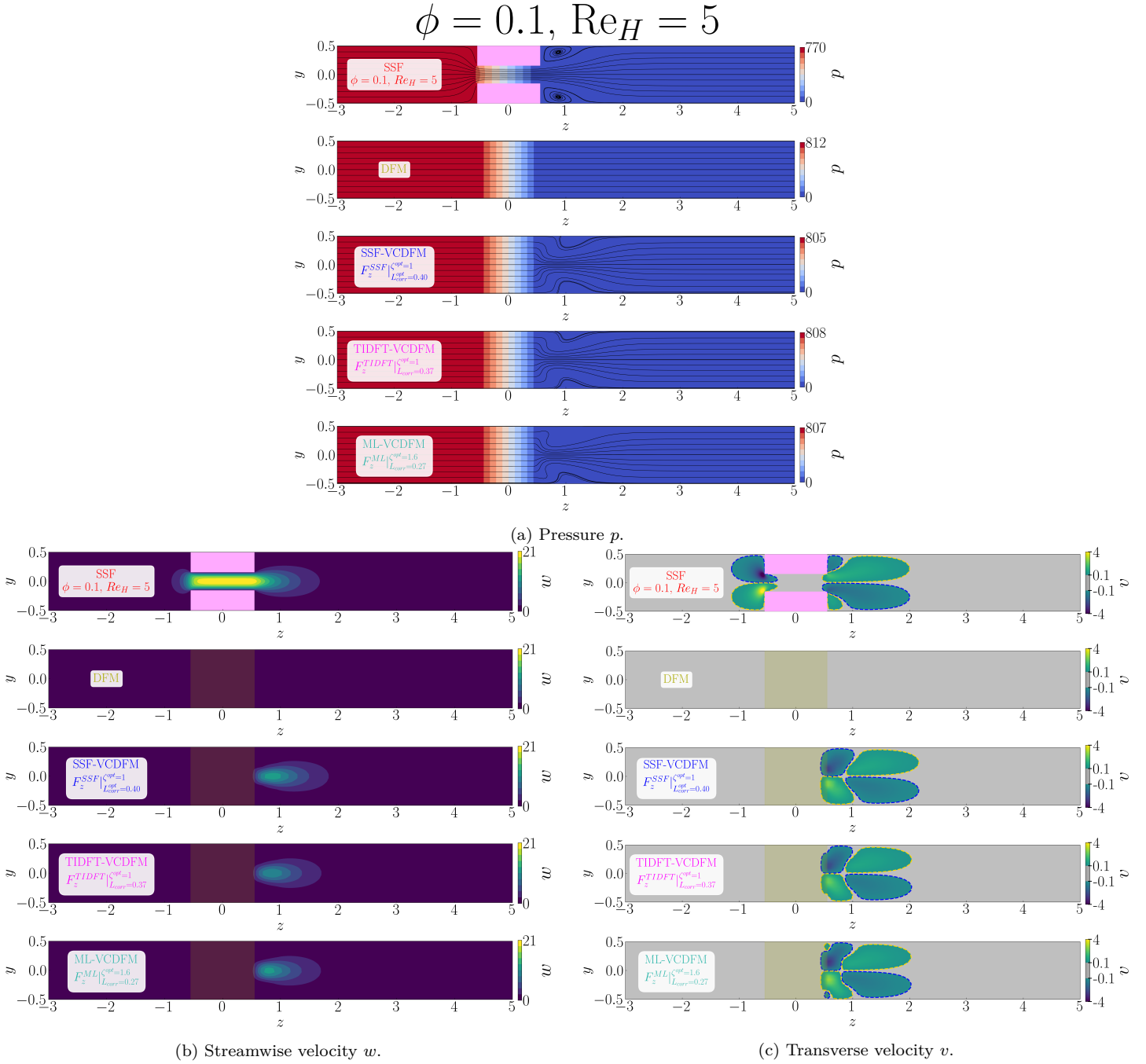
Figure D.40: Flow organization in the streamwise (z, y) -plane for the 1 \times 1 SRG at \phi = 0.1 , Re_H = 5 , and \alpha = 0^\circ . The blocks show (a) pressure p with streamlines, (b) streamwise velocity w , and (c) transverse velocity v . Within each block, the rows show, from top to bottom, the SSF, DFM, SSF-VCDFM, TIDFT-VCDFM, and ML-VCDFM. Pink shading marks the grid walls in the SSF; olive shading marks the equivalent porous zone in the model solutions.
