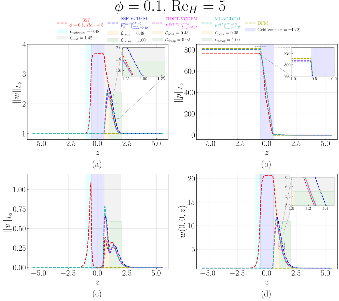
Figure D.39: Streamwise evolution of (a) \|w\|_{L_2} , (b) \|p\|_{L_2} , (c) \|v\|_{L_2} , and (d) centerline velocity w(0,0,z) for the 1 \times 1 SRG at \phi = 0.1 and \text{Re}_H = 5 . The figure compares the SSF, DFM, SSF-VCDFM, TIDFT-VCDFM, and ML-VCDFM. Shading marks the grid and the characteristic entrance, exit, peak, and decay regions. Only the SSF-based \mathcal{L}_{\text{peak}} and \mathcal{L}_{\text{decay}} are marked on the plot; the corresponding TIDFT-VCDFM and ML-VCDFM values appear in the legend.
