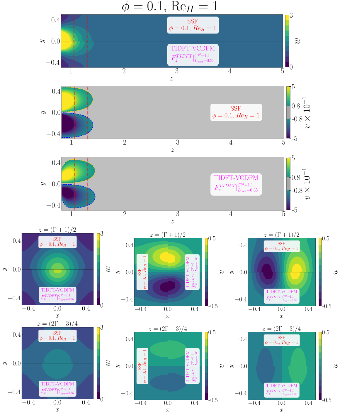
Figure D.37: Detailed comparison between the geometry-resolved small-scale flow (SSF) and TIDFT-VCDFM using F_z^{\text{TIDFT}} for the 1 \times 1 SRG at \phi = 0.1 and \text{Re}_H = 1 . The upper panels compare the streamwise velocity w and transverse velocity v in the central (z, y) -plane, restricted to the correction region. The lower panels compare the corresponding transverse (x, y) -plane distributions of w , v , and u , from left to right, at z = (\Gamma + 1)/2 in the first row and z = (2\Gamma + 3)/4 in the second row.
