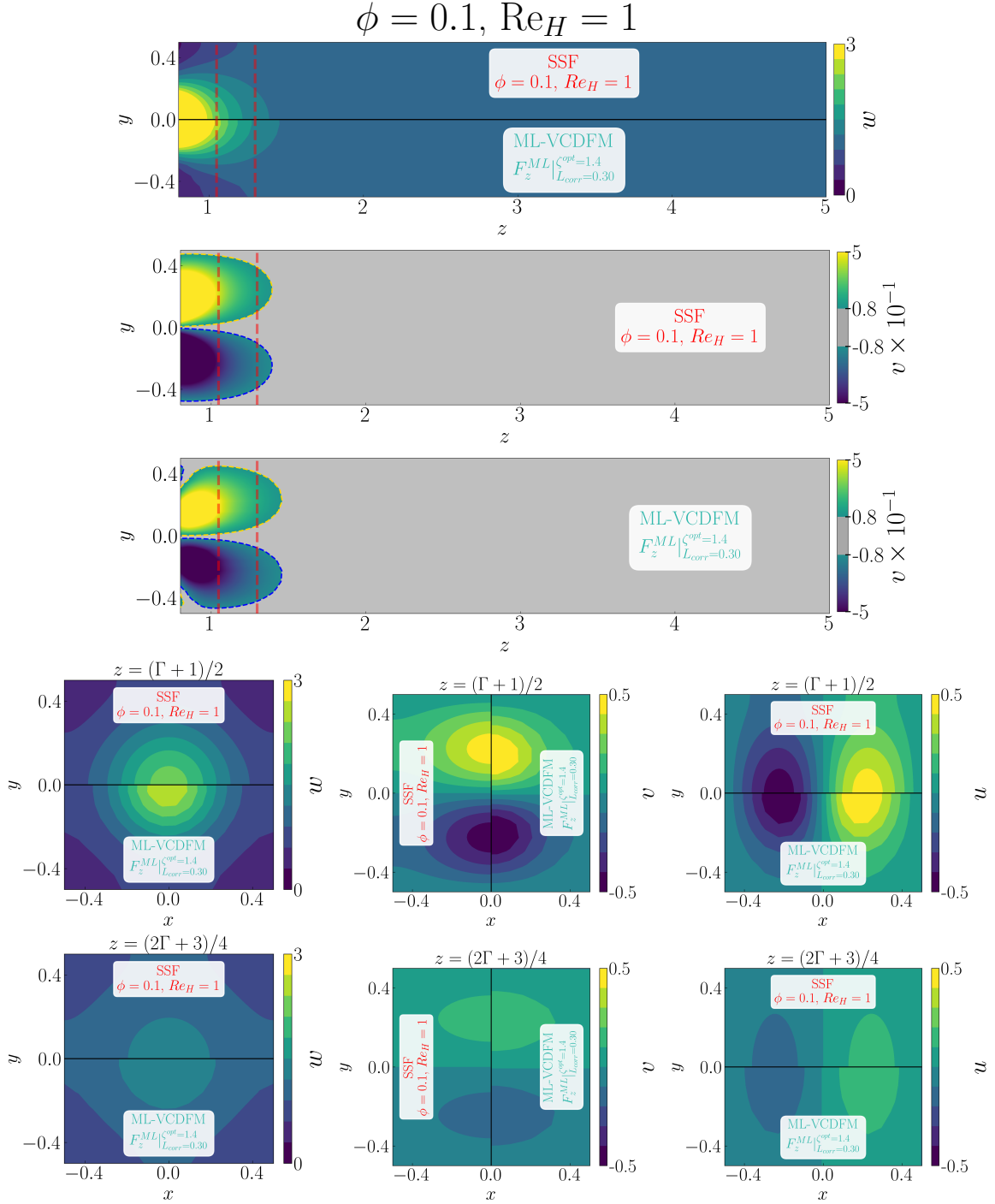
Figure D.38: Detailed comparison between the geometry-resolved small-scale flow (SSF) and ML-VCDFM using F_z^{ML} for the 1 \times 1 SRG at \phi = 0.1 and Re_H = 1 . The upper panels compare the streamwise velocity w and transverse velocity v in the central (z, y) -plane, restricted to the correction region. The lower panels compare the corresponding transverse (x, y) -plane distributions of w , v , and u , from left to right, at z = (\Gamma + 1)/2 in the first row and z = (2\Gamma + 3)/4 in the second row.
