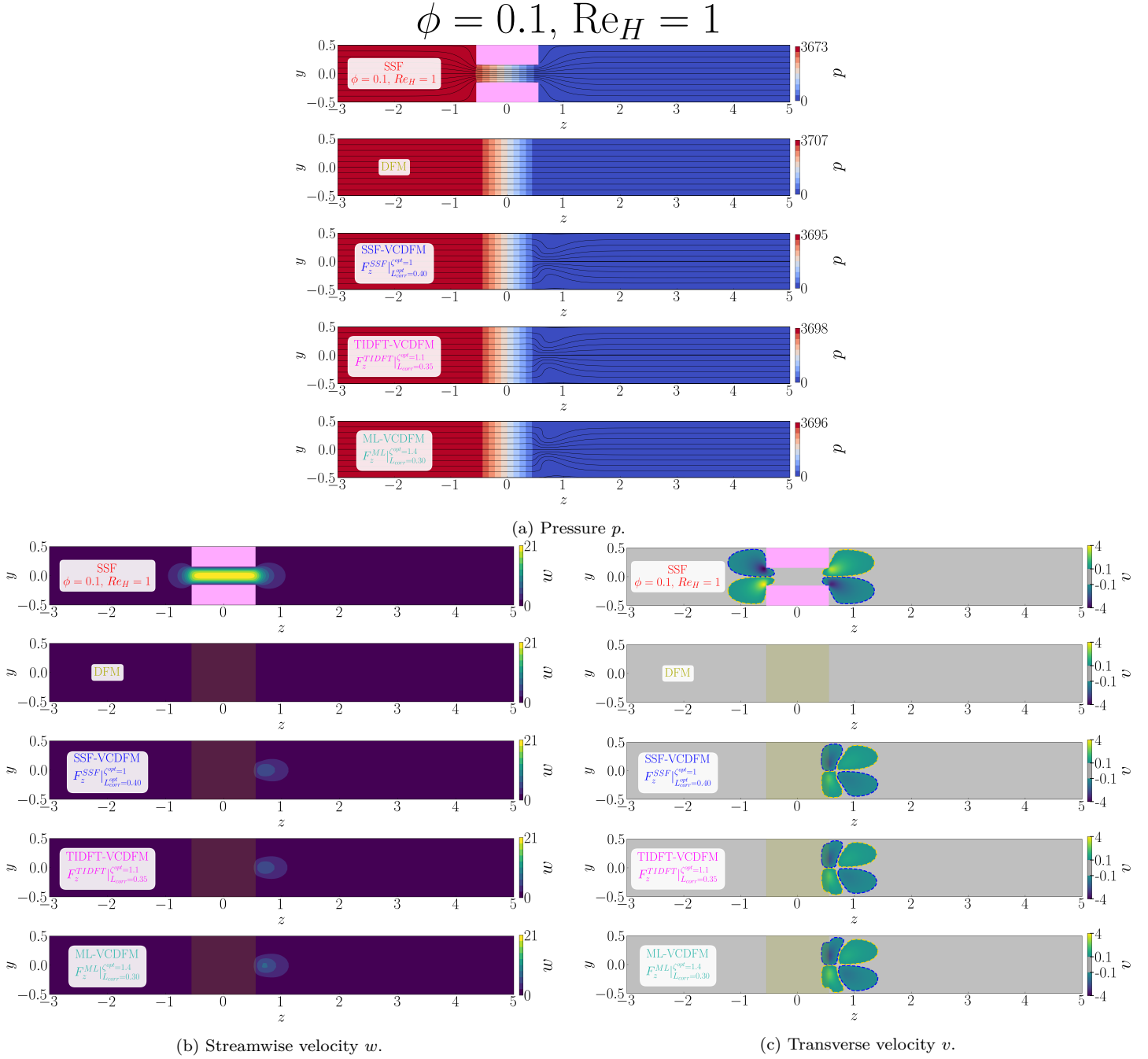
Figure D.34: Flow organization in the streamwise (z, y) -plane for the 1 \times 1 SRG at \phi = 0.1 , \text{Re}_H = 1 , and \alpha = 0^\circ . The blocks show (a) pressure p with streamlines, (b) streamwise velocity w , and (c) transverse velocity v . Within each block, the rows show, from top to bottom, the SSF, DFM, SSF-VCDFM, TIDFT-VCDFM, and ML-VCDFM. Pink shading marks the grid walls in the SSF; olive shading marks the equivalent porous zone in the model solutions.
