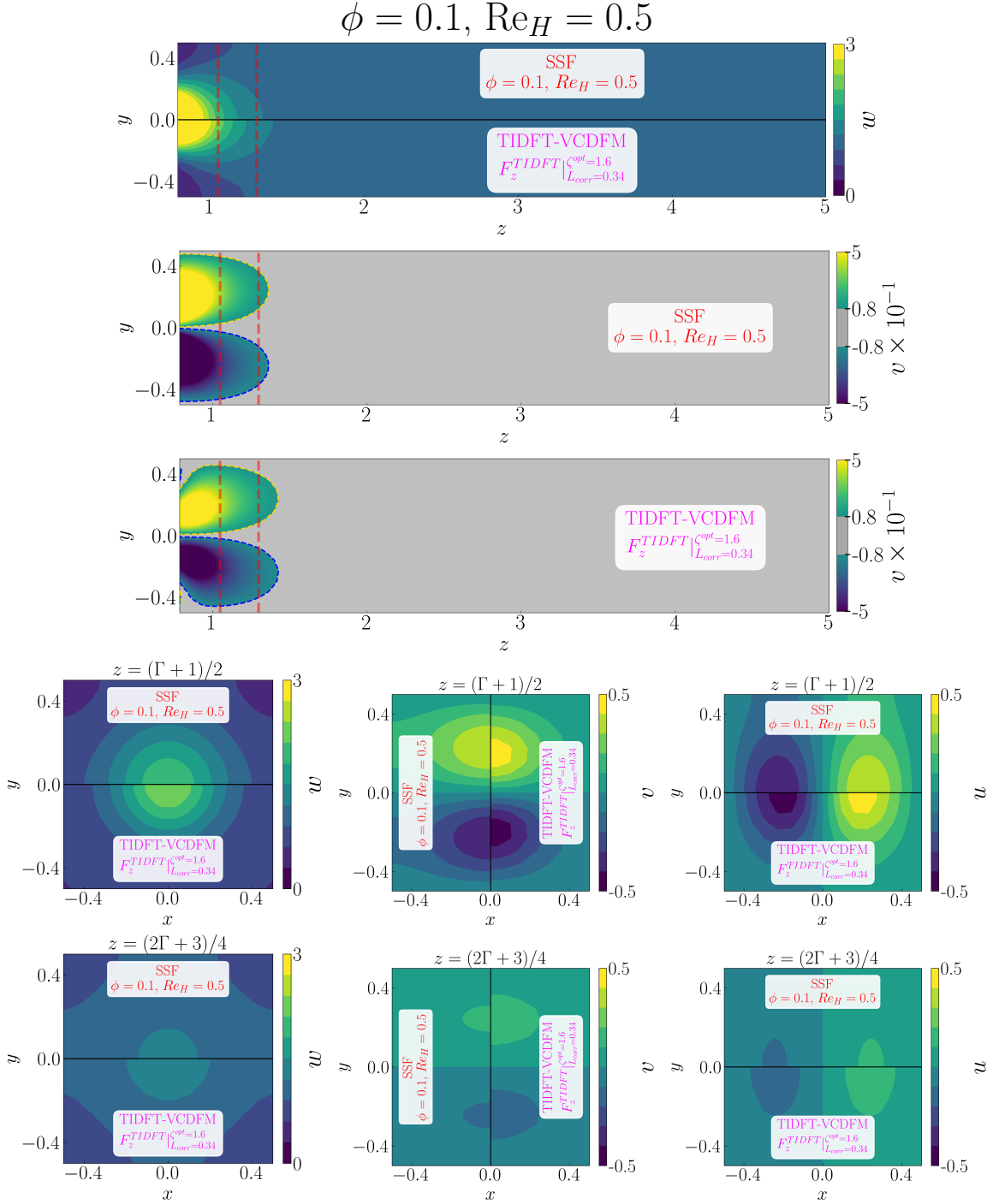
Figure D.31: Detailed comparison between the geometry-resolved small-scale flow (SSF) and TIDFT-VCDFM using F_z^{TIDFT} for the 1 \times 1 SRG at \phi = 0.1 and Re_H = 0.5 . The upper panels compare the streamwise velocity w and transverse velocity v in the central (z, y) -plane, restricted to the correction region. The lower panels compare the corresponding transverse (x, y) -plane distributions of w , v , and u , from left to right, at z = (\Gamma + 1)/2 in the first row and z = (2\Gamma + 3)/4 in the second row.
