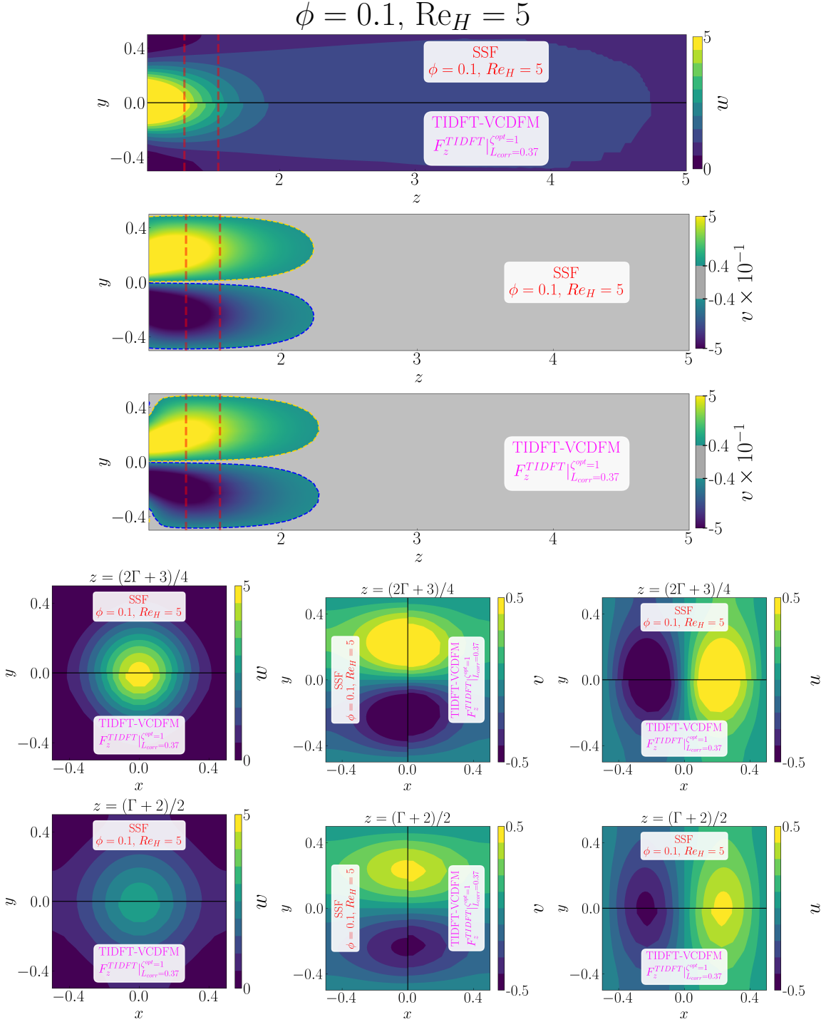
Figure D.43: Detailed comparison between the geometry-resolved small-scale flow (SSF) and TIDFT-VCDFM using F_z^{TIDFT} for the 1 \times 1 SRG at \phi = 0.1 and Re_H = 5 . The upper panels compare the streamwise velocity w and transverse velocity v in the central (z, y) -plane, restricted to the correction region. The lower panels compare the corresponding transverse (x, y) -plane distributions of w , v , and u , from left to right, at z = (2\Gamma + 3)/4 in the first row and z = (\Gamma + 2)/2 in the second row.
