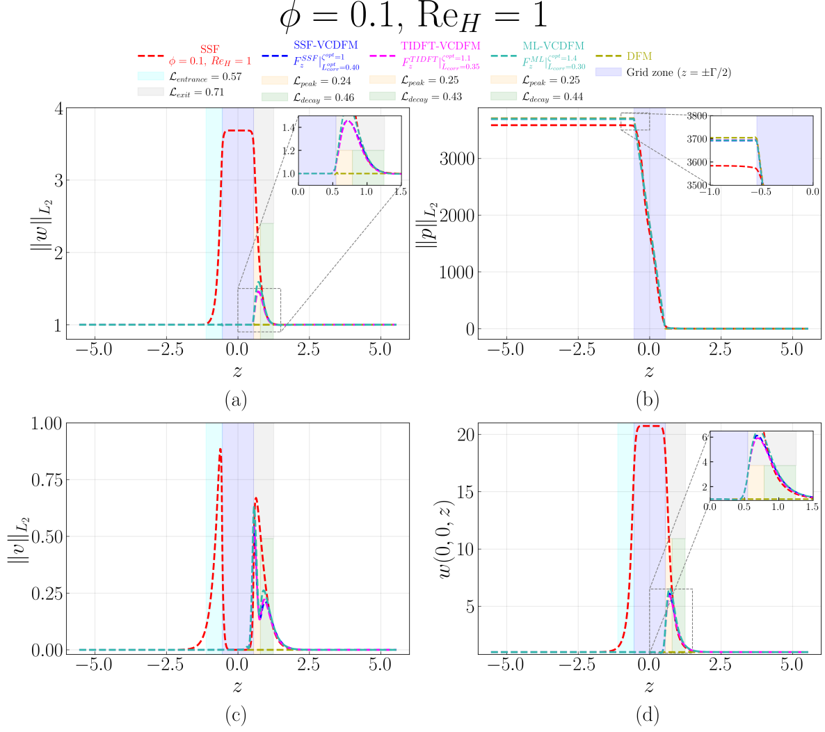
Figure D.33: Streamwise evolution of (a) \|w\|_{L_2} , (b) \|p\|_{L_2} , (c) \|v\|_{L_2} , and (d) centerline velocity w(0,0,z) for the 1 \times 1 SRG at \phi = 0.1 and \text{Re}_H = 1 . The figure compares the SSF, DFM, SSF-VCDFM, TIDFT-VCDFM, and ML-VCDFM. Shading marks the grid and the characteristic entrance, exit, peak, and decay regions. Only the SSF-based \mathcal{L}_{\text{peak}} and \mathcal{L}_{\text{decay}} are marked on the plot; the corresponding TIDFT-VCDFM and ML-VCDFM values appear in the legend.
