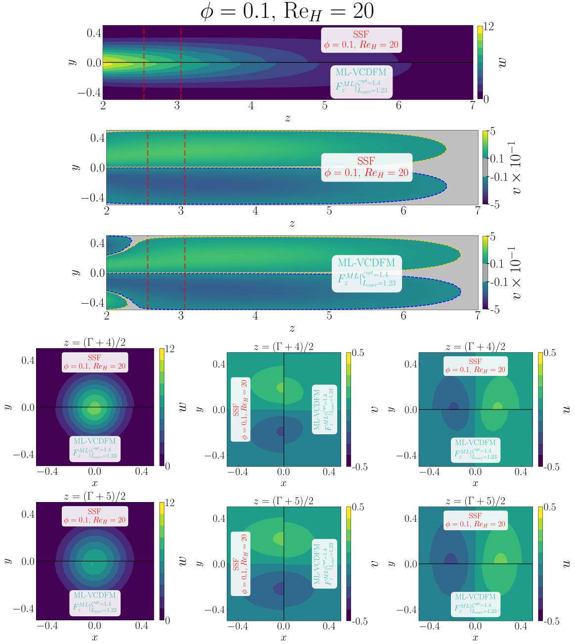
Figure D.56: Detailed comparison between the geometry-resolved small-scale flow (SSF) and ML-VCDFM using F_z^{\text{ML}} for the 1 × 1 SRG at \phi = 0.1 and \text{Re}_H = 20 . The upper panels compare the streamwise velocity w and transverse velocity v in the central (z, y) -plane, restricted to the correction region. The lower panels compare the corresponding transverse (x, y) -plane distributions of w , v , and u , from left to right, at z = (\Gamma + 4)/2 in the first row and z = (\Gamma + 5)/2 in the second row.
