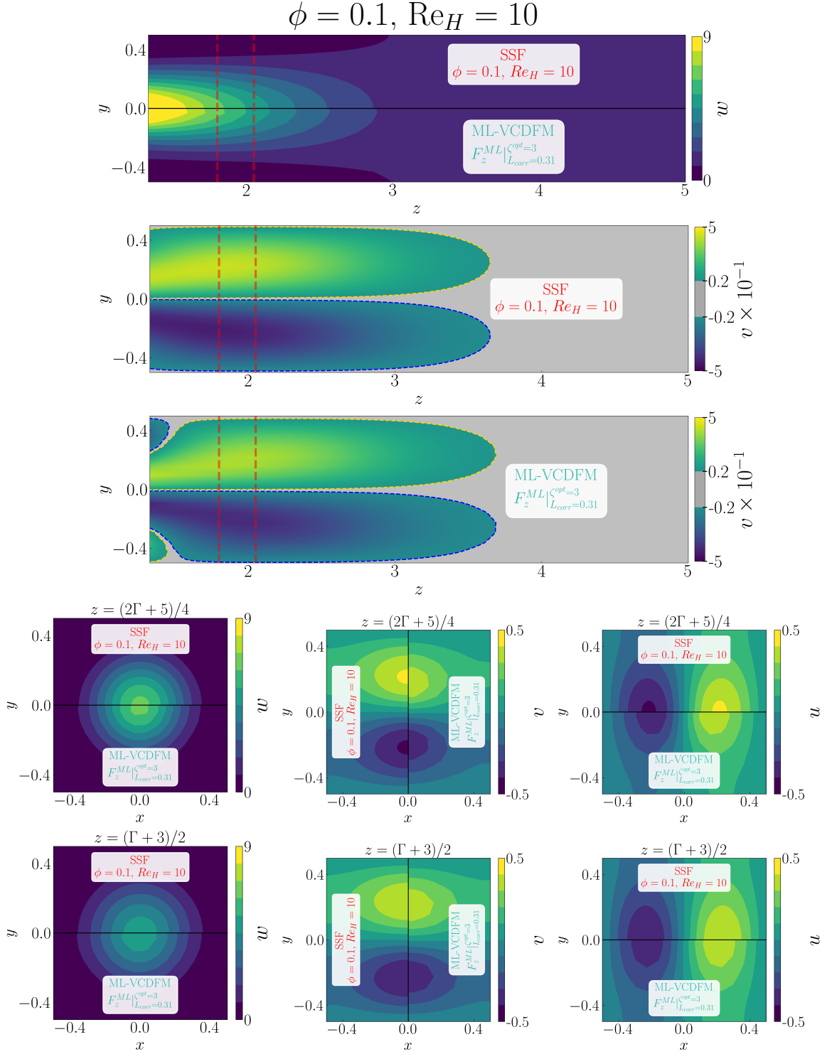
Figure D.50: Detailed comparison between the geometry-resolved small-scale flow (SSF) and ML-VCDFM using F_z^{ML} for the 1 \times 1 SRG at \phi = 0.1 and Re_H = 10 . The upper panels compare the streamwise velocity w and transverse velocity v in the central (z, y) -plane, restricted to the correction region. The lower panels compare the corresponding transverse (x, y) -plane distributions of w , v , and u , from left to right, at z = (2\Gamma + 5)/4 in the first row and z = (\Gamma + 3)/2 in the second row.
