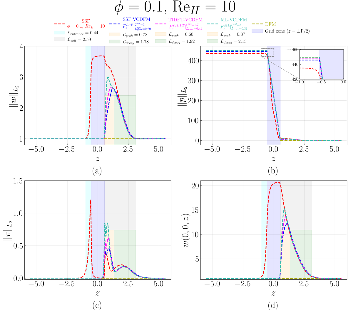
Figure D.45: Streamwise evolution of (a) \|w\|_{L_2} , (b) \|p\|_{L_2} , (c) \|v\|_{L_2} , and (d) centerline velocity w(0,0,z) for the 1 \times 1 SRG at \phi = 0.1 and \text{Re}_H = 10 . The figure compares the SSF, DFM, SSF-VCDFM, TIDFT-VCDFM, and ML-VCDFM. Shading marks the grid and the characteristic entrance, exit, peak, and decay regions. Only the SSF-based \mathcal{L}_{\text{peak}} and \mathcal{L}_{\text{decay}} are marked on the plot; the corresponding TIDFT-VCDFM and ML-VCDFM values appear in the legend.
