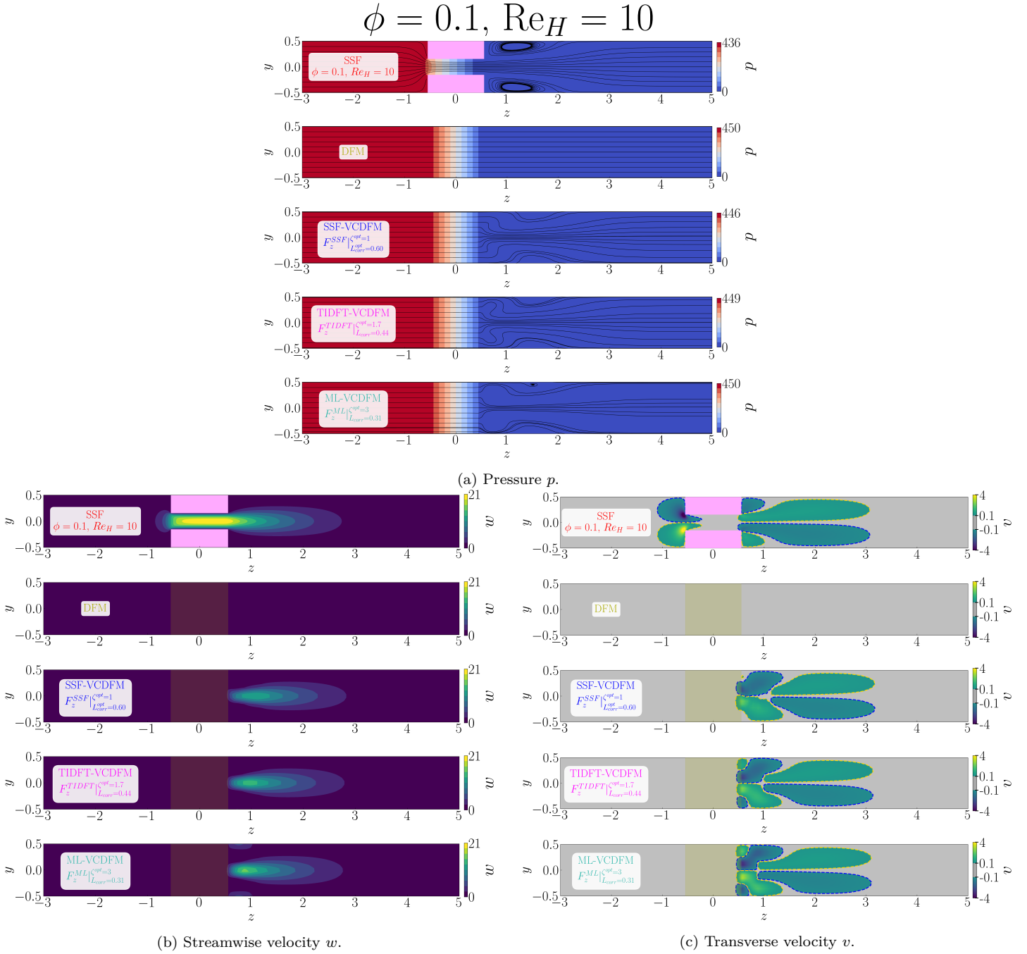
Figure D.46: Flow organization in the streamwise (z, y) -plane for the 1 \times 1 SRG at \phi = 0.1 , Re_H = 10 , and \alpha = 0^\circ . The blocks show (a) pressure p with streamlines, (b) streamwise velocity w , and (c) transverse velocity v . Within each block, the rows show, from top to bottom, the SSF, DFM, SSF-VCDFM, TIDFT-VCDFM, and ML-VCDFM. Pink shading marks the grid walls in the SSF; olive shading marks the equivalent porous zone in the model solutions.
