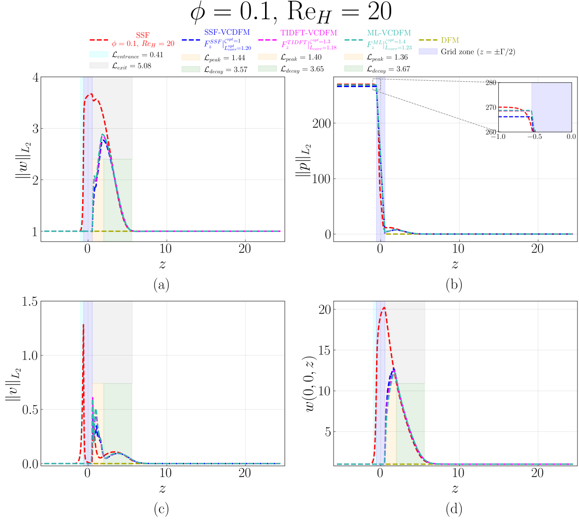
Figure D.51: Streamwise evolution of (a) \|w\|_{L_2} , (b) \|p\|_{L_2} , (c) \|v\|_{L_2} , and (d) centerline velocity w(0,0,z) for the 1 \times 1 SRG at \phi = 0.1 and Re_H = 20 . The figure compares the SSF, DFM, SSF-VCDFM, TIDFT-VCDFM, and ML-VCDFM. Shading marks the grid and the characteristic entrance, exit, peak, and decay regions. Only the SSF-based \mathcal{L}_{peak} and \mathcal{L}_{decay} are marked on the plot; the corresponding TIDFT-VCDFM and ML-VCDFM values appear in the legend.
