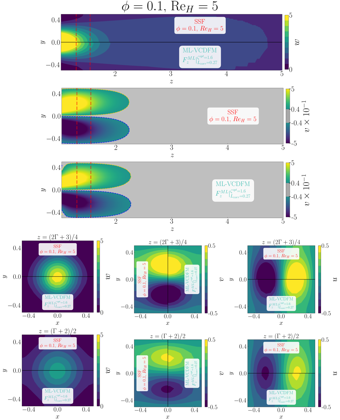
Figure D.44: Detailed comparison between the geometry-resolved small-scale flow (SSF) and ML-VCDFM using F_z^{ML} for the 1 \times 1 SRG at \phi = 0.1 and Re_H = 5 . The upper panels compare the streamwise velocity w and transverse velocity v in the central (z, y) -plane, restricted to the correction region. The lower panels compare the corresponding transverse (x, y) -plane distributions of w , v , and u , from left to right, at z = (2\Gamma + 3)/4 in the first row and z = (\Gamma + 2)/2 in the second row.
