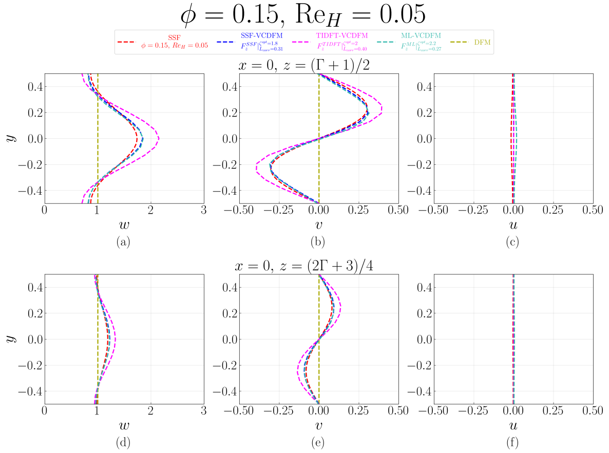
Figure D.59: Velocity profiles at x = 0 for the 1 \times 1 SRG at \phi = 0.15 and \text{Re}_H = 0.05 , comparing the SSF, DFM, SSF-VCDFM, TIDFT-VCDFM, and ML-VCDFM. Profiles of w(y) , v(y) , and u(y) are shown at z = (\Gamma + 1)/2 in (a–c) and z = (2\Gamma + 3)/4 in (d–f).
