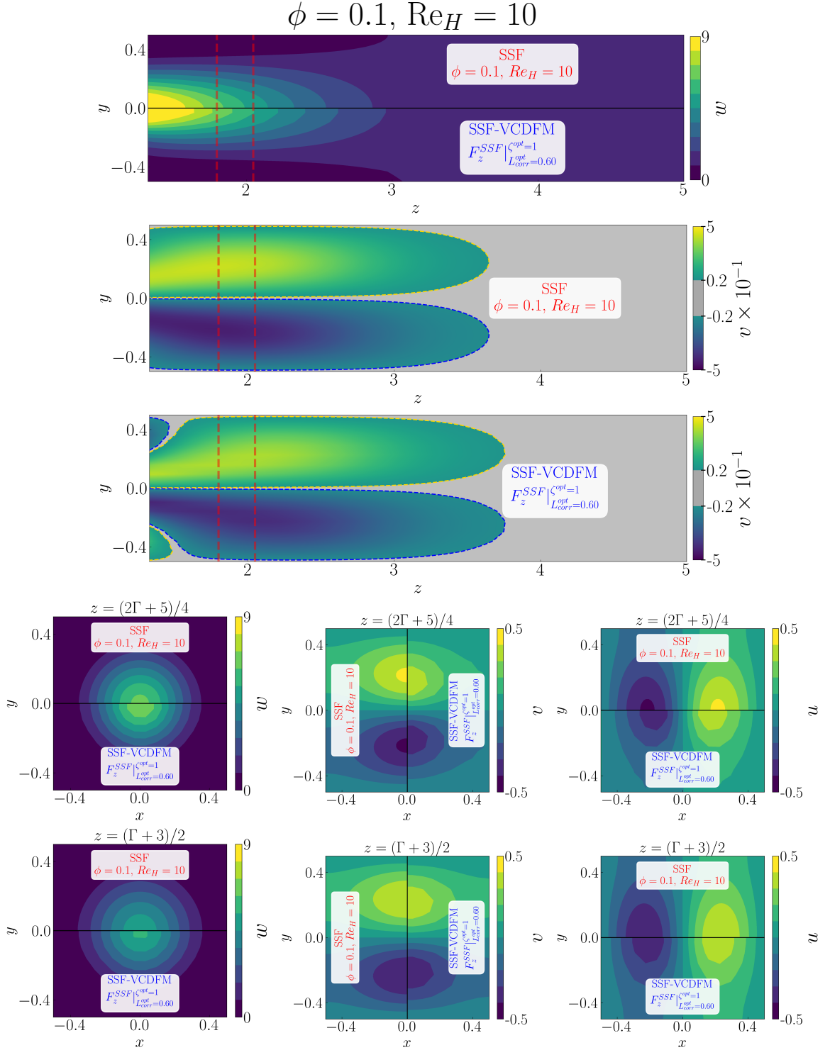
Figure D.48: Detailed comparison between the geometry-resolved small-scale flow (SSF) and SSF-VCDFM using F_z^{SSF} for the 1 \times 1 SRG at \phi = 0.1 and Re_H = 10 . The upper panels compare the streamwise velocity w and transverse velocity v in the central (z, y) -plane, restricted to the correction region. The lower panels compare the corresponding transverse (x, y) -plane distributions of w , v , and u , from left to right, at z = (2\Gamma + 5)/4 in the first row and z = (\Gamma + 3)/2 in the second row.
