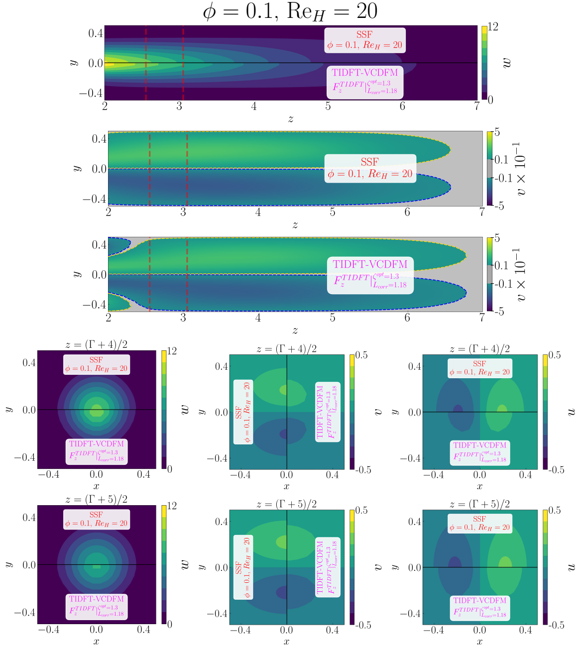
Figure D.55: Detailed comparison between the geometry-resolved small-scale flow (SSF) and TIDFT-VCDFM using F_z^{TIDFT} for the 1 \times 1 SRG at \phi = 0.1 and Re_H = 20 . The upper panels compare the streamwise velocity w and transverse velocity v in the central (z, y) -plane, restricted to the correction region. The lower panels compare the corresponding transverse (x, y) -plane distributions of w , v , and u , from left to right, at z = (\Gamma + 4)/2 in the first row and z = (\Gamma + 5)/2 in the second row.
