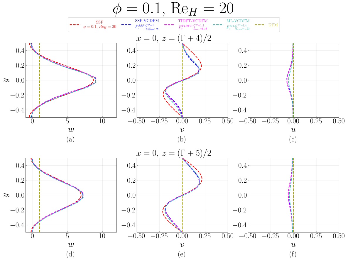
Figure D.53: Velocity profiles at x = 0 for the 1 \times 1 SRG at \phi = 0.1 and \text{Re}_H = 20 , comparing the SSF, DFM, SSF-VCDFM, TIDFT-VCDFM, and ML-VCDFM. Profiles of w(y) , v(y) , and u(y) are shown at z = (\Gamma + 4)/2 in (a–c) and z = (\Gamma + 5)/2 in (d–f).
