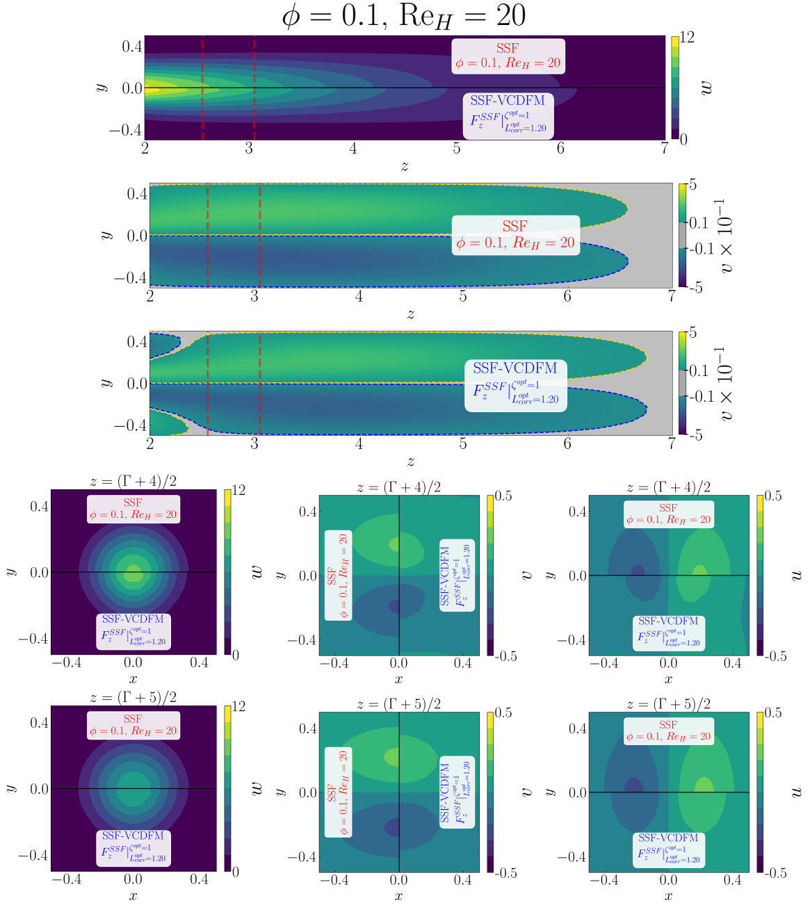
Figure D.54: Detailed comparison between the geometry-resolved small-scale flow (SSF) and SSF-VCDFM using F_z^{SSF} for the 1 \times 1 SRG at \phi = 0.1 and Re_H = 20 . The upper panels compare the streamwise velocity w and transverse velocity v in the central (z, y) -plane, restricted to the correction region. The lower panels compare the corresponding transverse (x, y) -plane distributions of w , v , and u , from left to right, at z = (\Gamma + 4)/2 in the first row and z = (\Gamma + 5)/2 in the second row.
