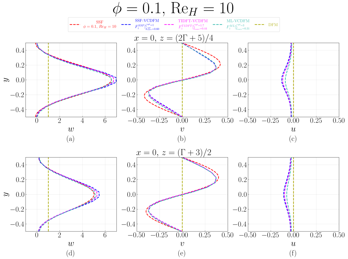
Figure D.47: Velocity profiles at x = 0 for the 1 \times 1 SRG at \phi = 0.1 and \text{Re}_H = 10 , comparing the SSF, DFM, SSF-VCDFM, TIDFT-VCDFM, and ML-VCDFM. Profiles of w(y) , v(y) , and u(y) are shown at z = (2\Gamma + 5)/4 in (a–c) and z = (\Gamma + 3)/2 in (d–f).
