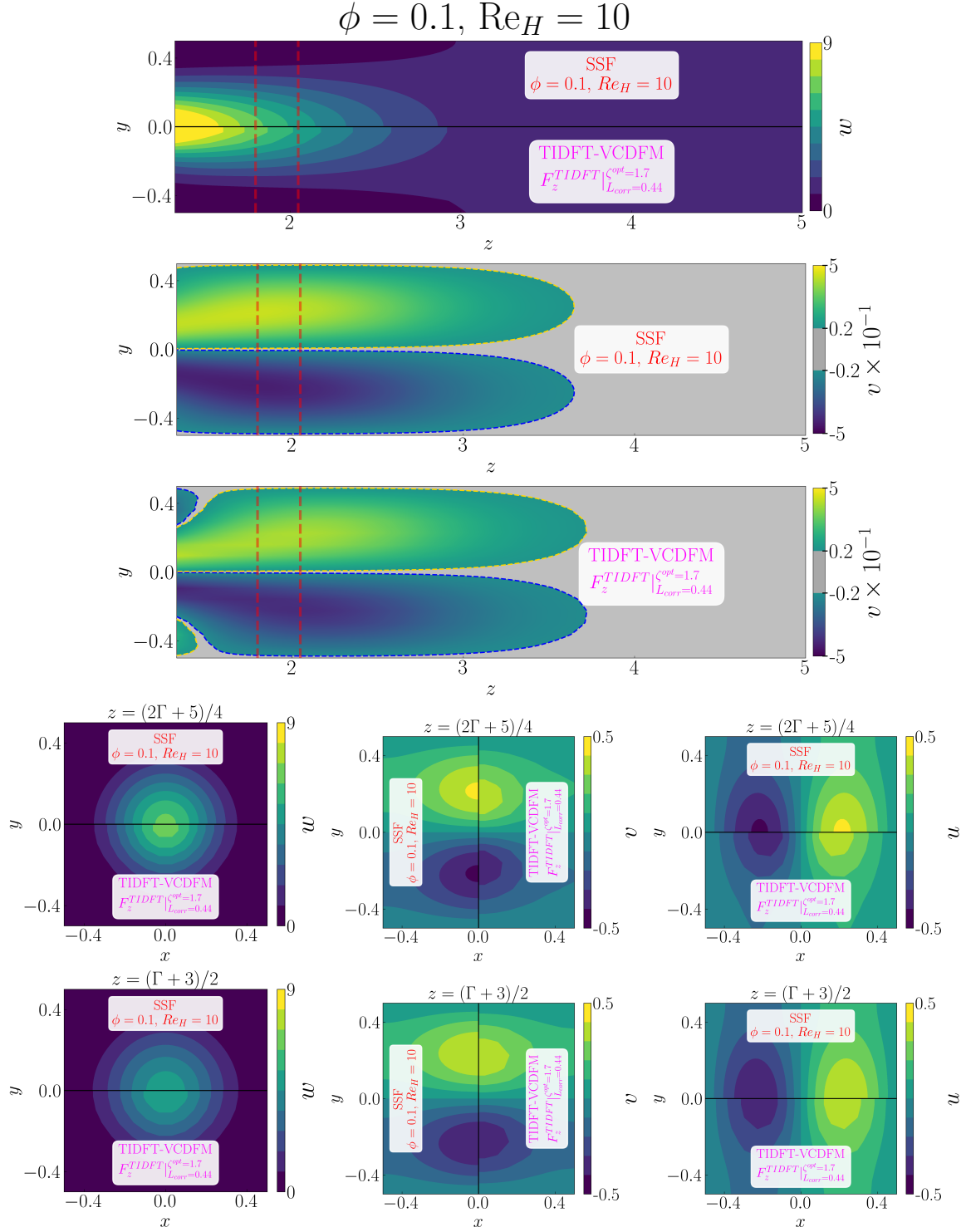
Figure D.49: Detailed comparison between the geometry-resolved small-scale flow (SSF) and TIDFT-VCDFM using F_z^{TIDFT} for the 1 \times 1 SRG at \phi = 0.1 and Re_H = 10 . The upper panels compare the streamwise velocity w and transverse velocity v in the central (z, y) -plane, restricted to the correction region. The lower panels compare the corresponding transverse (x, y) -plane distributions of w , v , and u , from left to right, at z = (2\Gamma + 5)/4 in the first row and z = (\Gamma + 3)/2 in the second row.
