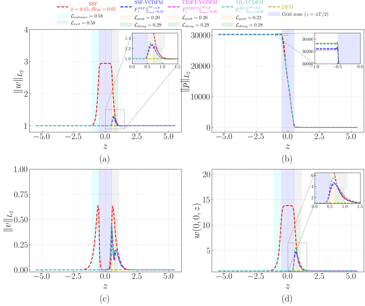
Figure D.57: Streamwise evolution of (a) \|w\|_{L_2} , (b) \|p\|_{L_2} , (c) \|v\|_{L_2} , and (d) centerline velocity w(0,0,z) for the 1 \times 1 SRG at \phi = 0.15 and \text{Re}_H = 0.05 . The figure compares the SSF, DFM, SSF-VCDFM, TIDFT-VCDFM, and ML-VCDFM. Shading marks the grid and the characteristic entrance, exit, peak, and decay regions. Only the SSF-based \mathcal{L}_{\text{peak}} and \mathcal{L}_{\text{decay}} are marked on the plot; the corresponding TIDFT-VCDFM and ML-VCDFM values appear in the legend.
