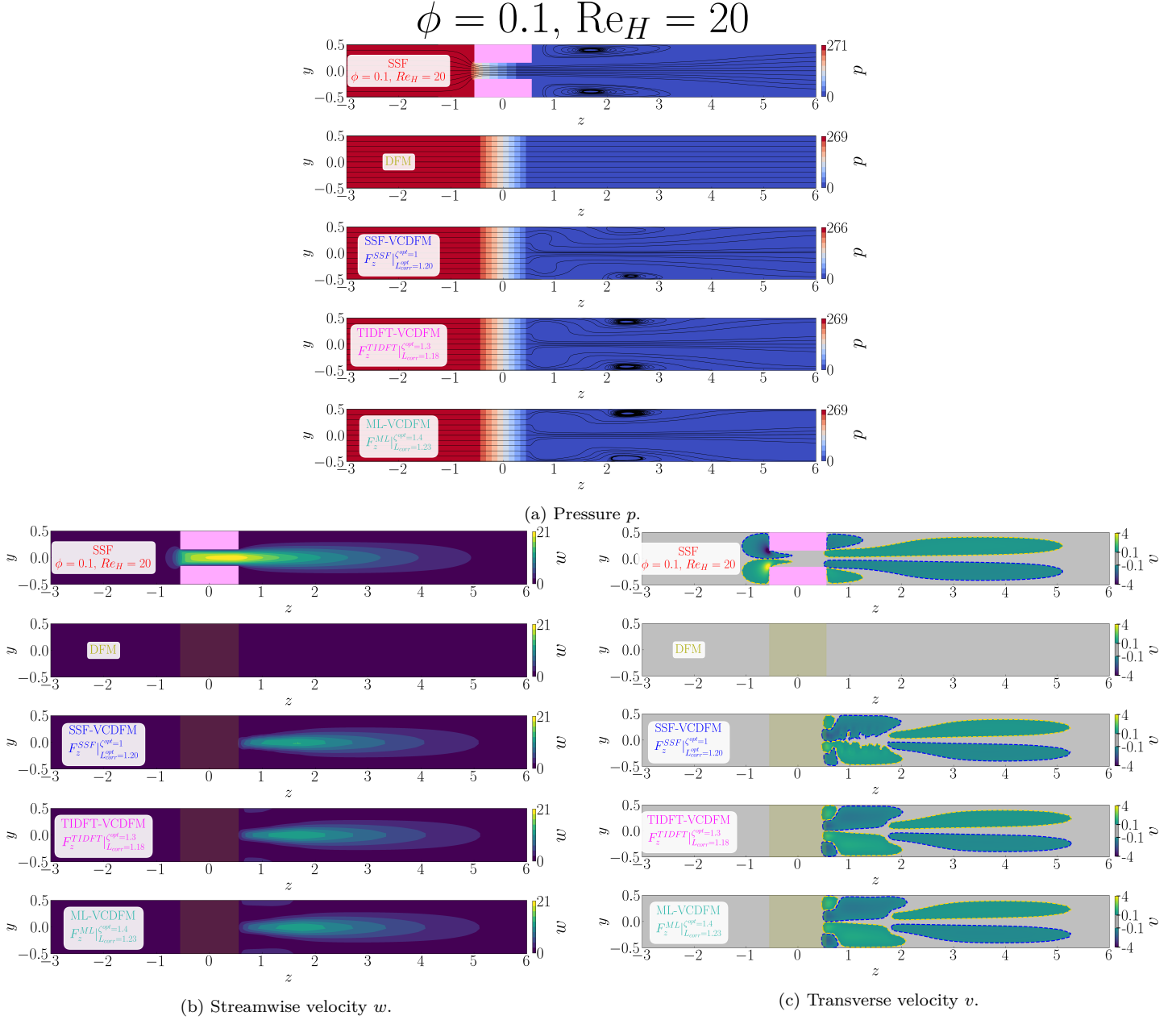
Figure D.52: Flow organization in the streamwise (z, y) -plane for the 1 \times 1 SRG at \phi = 0.1 , \text{Re}_H = 20 , and \alpha = 0^\circ . The blocks show (a) pressure p with streamlines, (b) streamwise velocity w , and (c) transverse velocity v . Within each block, the rows show, from top to bottom, the SSF, DFM, SSF-VCDFM, TIDFT-VCDFM, and ML-VCDFM. Pink shading marks the grid walls in the SSF; olive shading marks the equivalent porous zone in the model solutions.
