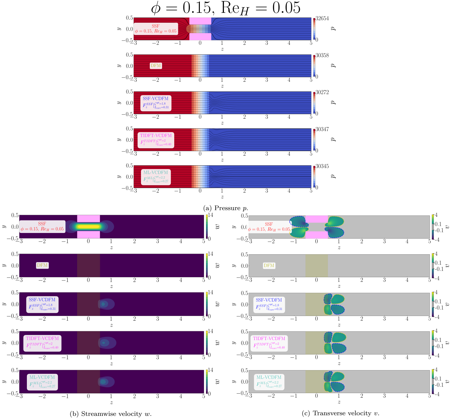
Figure D.58: Flow organization in the streamwise (z, y) -plane for the 1 \times 1 SRG at \phi = 0.15 , \text{Re}_H = 0.05 , and \alpha = 0^\circ . The blocks show (a) pressure p with streamlines, (b) streamwise velocity w , and (c) transverse velocity v . Within each block, the rows show, from top to bottom, the SSF, DFM, SSF-VCDFM, TIDFT-VCDFM, and ML-VCDFM. Pink shading marks the grid walls in the SSF; olive shading marks the equivalent porous zone in the model solutions.
