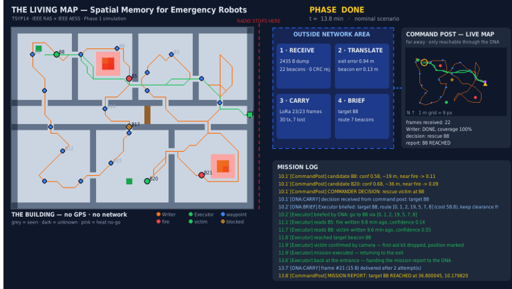
Figure 6: Simulator (Pygame) at the end of the nominal mission: building with the Writer’s (orange) and Executor’s (green) trails, beacons, the ONA’s 4 roles, the command-post live map and the mission log.
