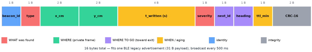
Figure 3: 16-byte beacon packet (little-endian, CRC-16/CCITT). Position is in the Writer’s private frame, in cm.
