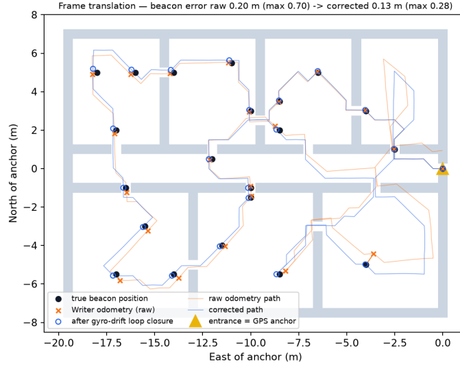
Figure 4: True vs. raw vs. corrected beacon positions (ENU around the anchor), nominal run.
