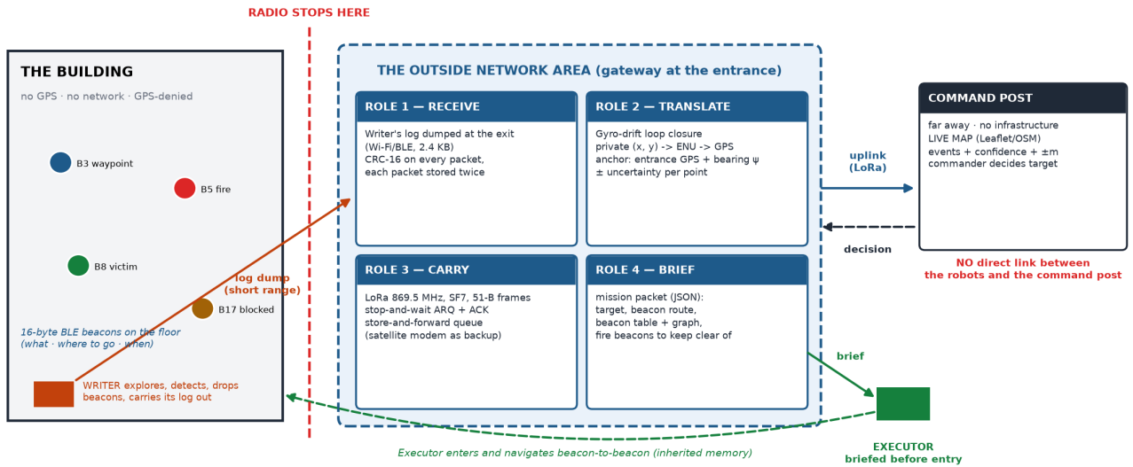
Figure 1: Architecture. All inside↔outside traffic goes through the ONA; robots never talk to the command post (this is checked by test_no_direct_robot_to_command_post_link ).
