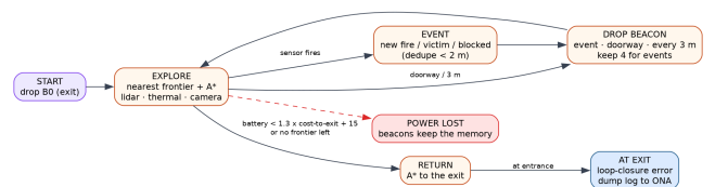
Figure 2: Writer decision state machine.
