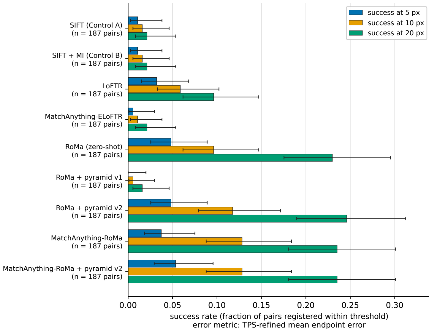
Registration success on the Amalgamatch benchmark all 187 pairs; error bars are 95 % Wilson score intervals
