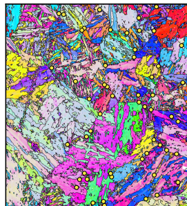
Narrow: EBSD orientation map 25 % of the wide image's area 54 annotated points
