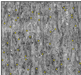
Narrow: SEM, backscattered electrons 99 % of the wide image's area 47 annotated points
