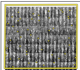
Wide: EBSD pattern-sharpness map
