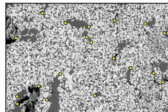
Narrow: SEM, backscattered electrons 4.9 % of the wide image's area 19 annotated points
