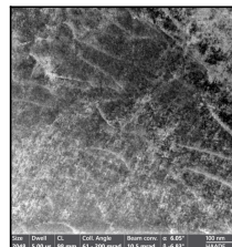
STEM, annular dark field 2048 x 2192 px
