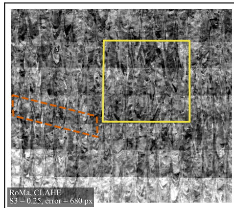
Flagged: CoNi-AM90 SEM-DIC EBSD SlipPartitioning
