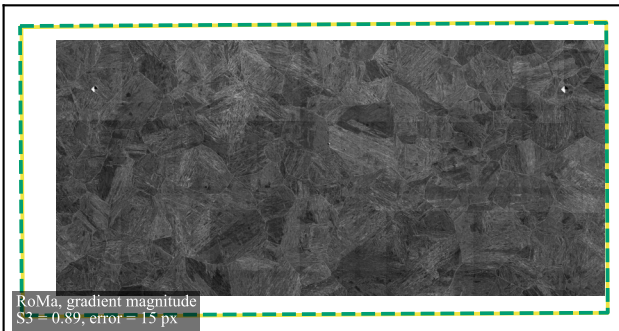
Accepted: AF9628-Martensitic SEM-SE-Stitch EBSD SameSlice
