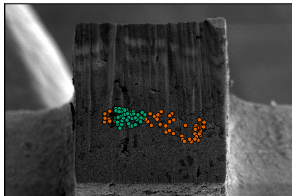
wide image: SEM, secondary electrons
