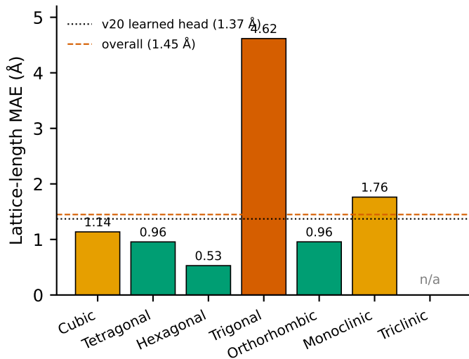
(b) Per-system lattice error
