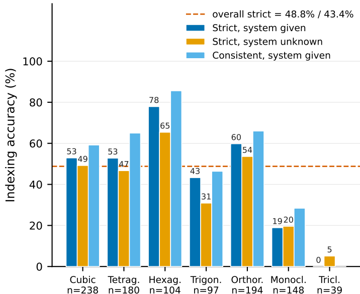
(a) Per-system match rate
