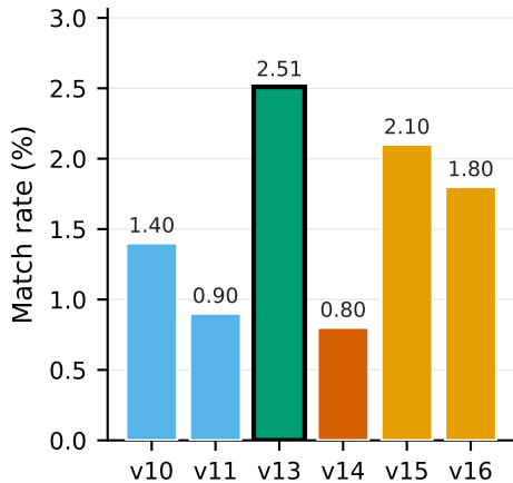
(a) StructureMatcher
