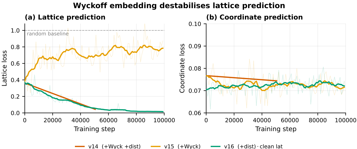
Figure 5: Figure 5. Wyckoff embedding destabilises lattice prediction. Lattice (a) and coordinate (b) training-loss curves for the distance-aux run (v16) vs the Wyckoff-embedding run (v15). Adding the Wyckoff embedding inflates the lattice loss by an order of magnitude ( \sim 0.6 vs \sim 0.02 ) while leaving the coordinate loss largely unchanged; the failure is localised to the lattice channel.
