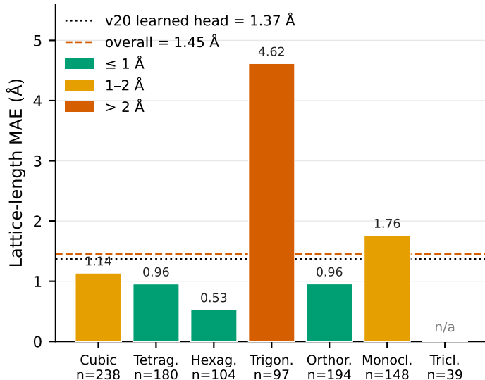
(b) Per-system lattice error
