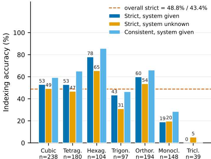
(a) Per-system match rate
