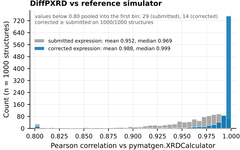
Figure 1: Figure 1. Differentiable-simulator validation. Distribution of Pearson correlation between the PyTorch DiffPXRd module and pymatgen.XRD Calculator over the first 1000 MP-20 test structures, with the corrected form factor (mean 0.988, median 0.999) and with the form factor of the submitted version (mean 0.952, median 0.969). The correction improves every structure. The residual lower tail is dominated by layered structures with strong texture in the reference.
