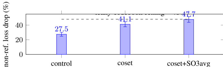
Figure 1: Deployable coset conditioning recovers two-thirds of the way from the no-coset control to the leaky-codebook ceiling; the SO(3) -averaged objective closes the rest. Three-seed mean, error bars s.d.
