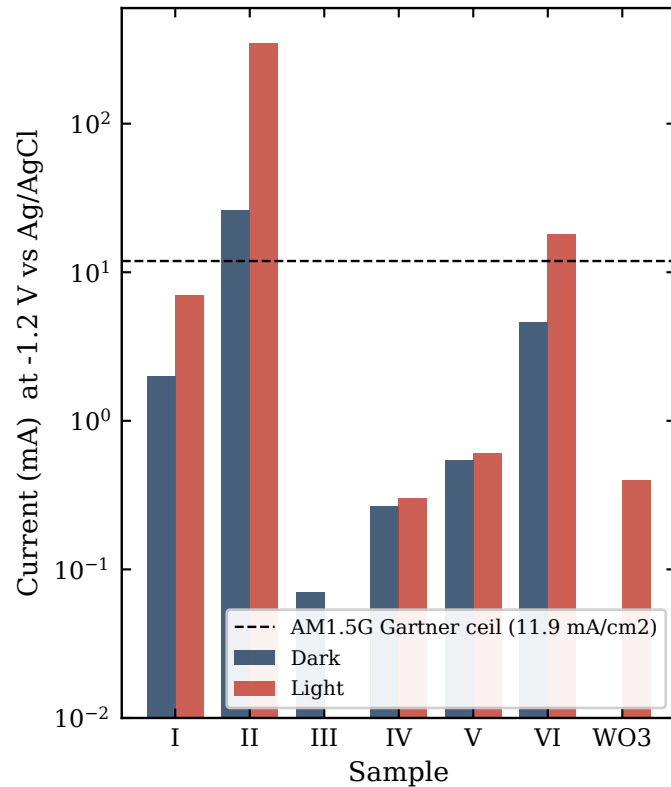
(c) Full sample comparison 0.5 M KOH, 395 nm torch, 1 cm 2
