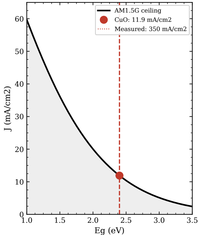
(a) AM1.5G ceiling (benchmark - not actual conditions)
