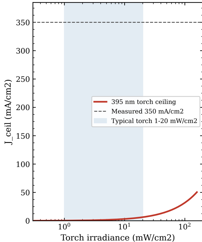
Gartner Analysis + Sample Comparison Measure torch irradiance for quantitative roughness factor (b) 395 nm torch Gartner ceiling ACTUAL measurement conditions
