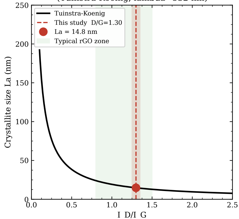
(b) Crystallite size from D/G (Tuinstra-Koenig, \lambda=532 nm)
