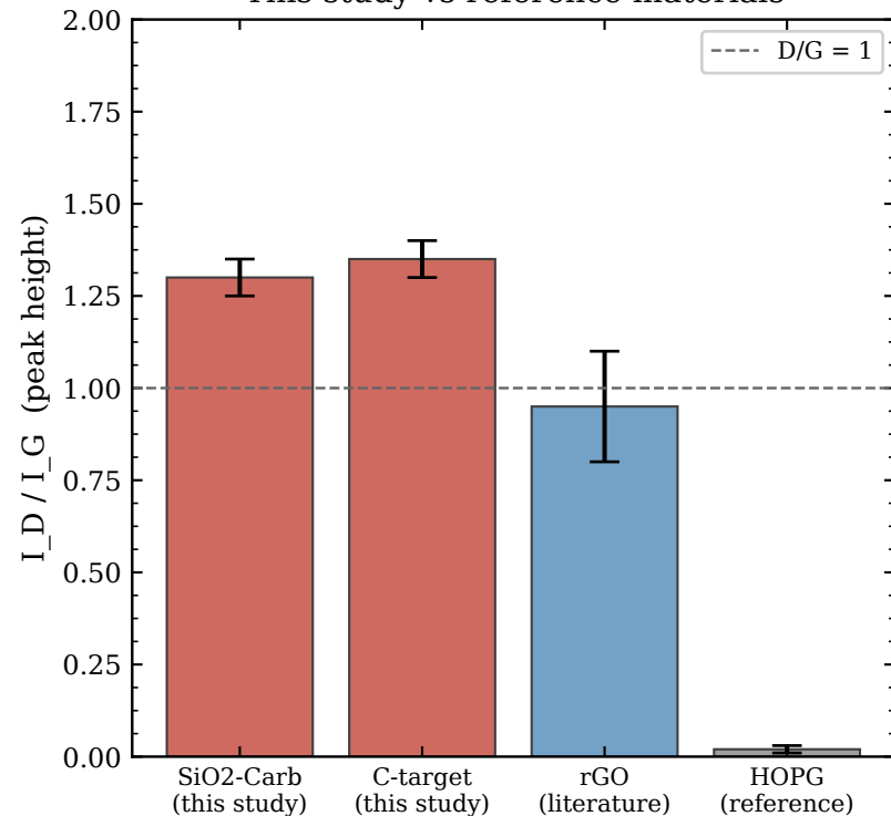
(a) Raman D/G ratio This study vs reference materials
