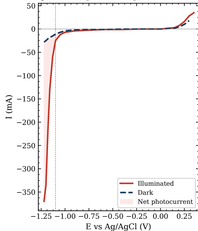
(a) LSV vs Ag/AgCl (digitised - replace with potentiostat CSV)
