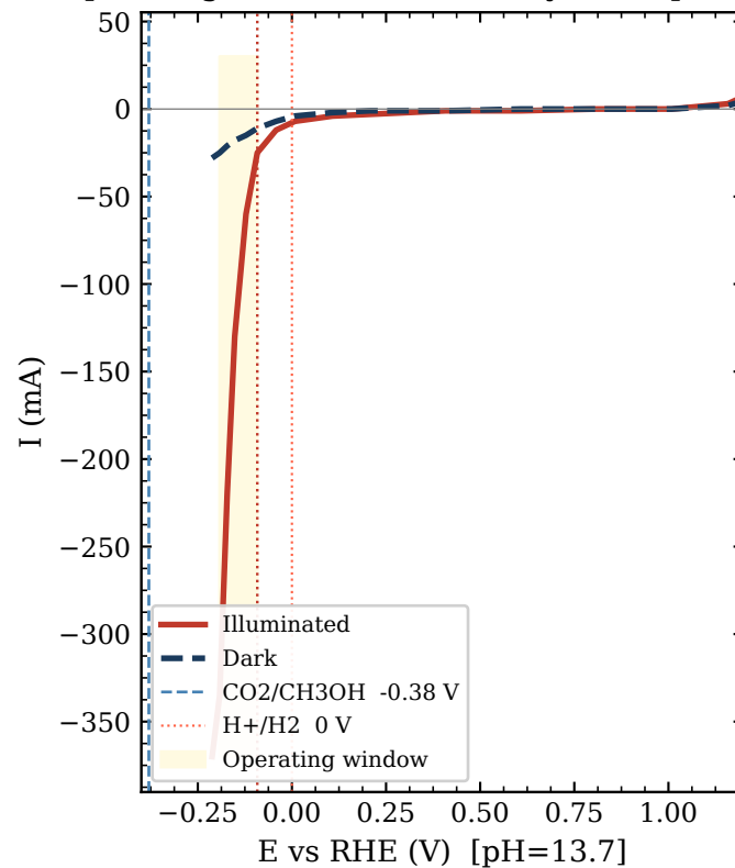
(b) LSV vs RHE Operating window vs thermodynamic potentials
