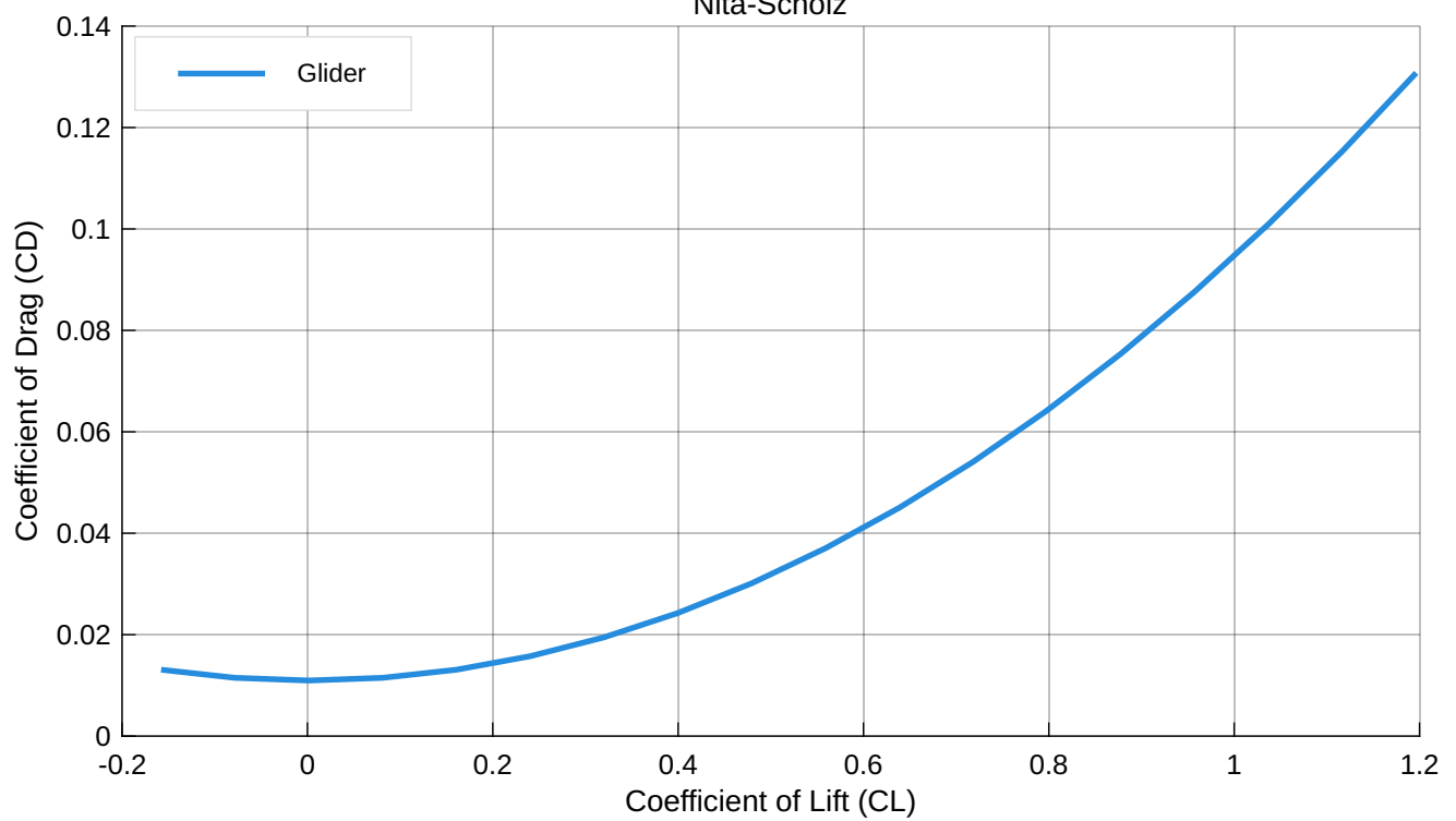
Drag Polar Configuration Comparison - Nita-Scholz
