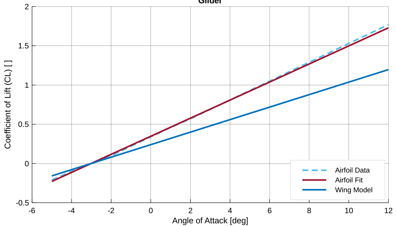
Lift Curve Slope Modeling - Configuration Glider
