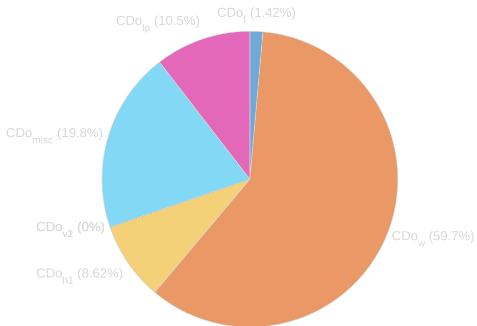
Parasite Drag Breakdown in Drag Counts: Glider
