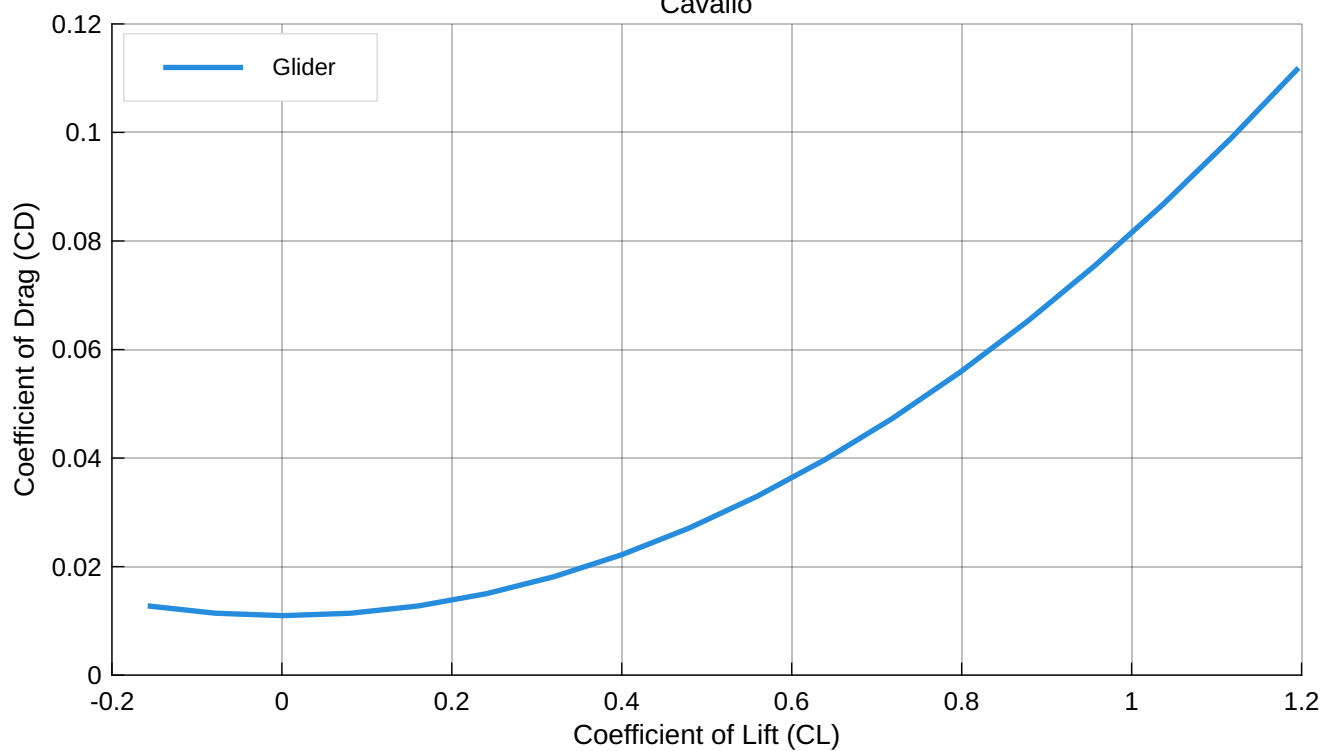
Drag Polar Configuration Comparison - Cavallo
