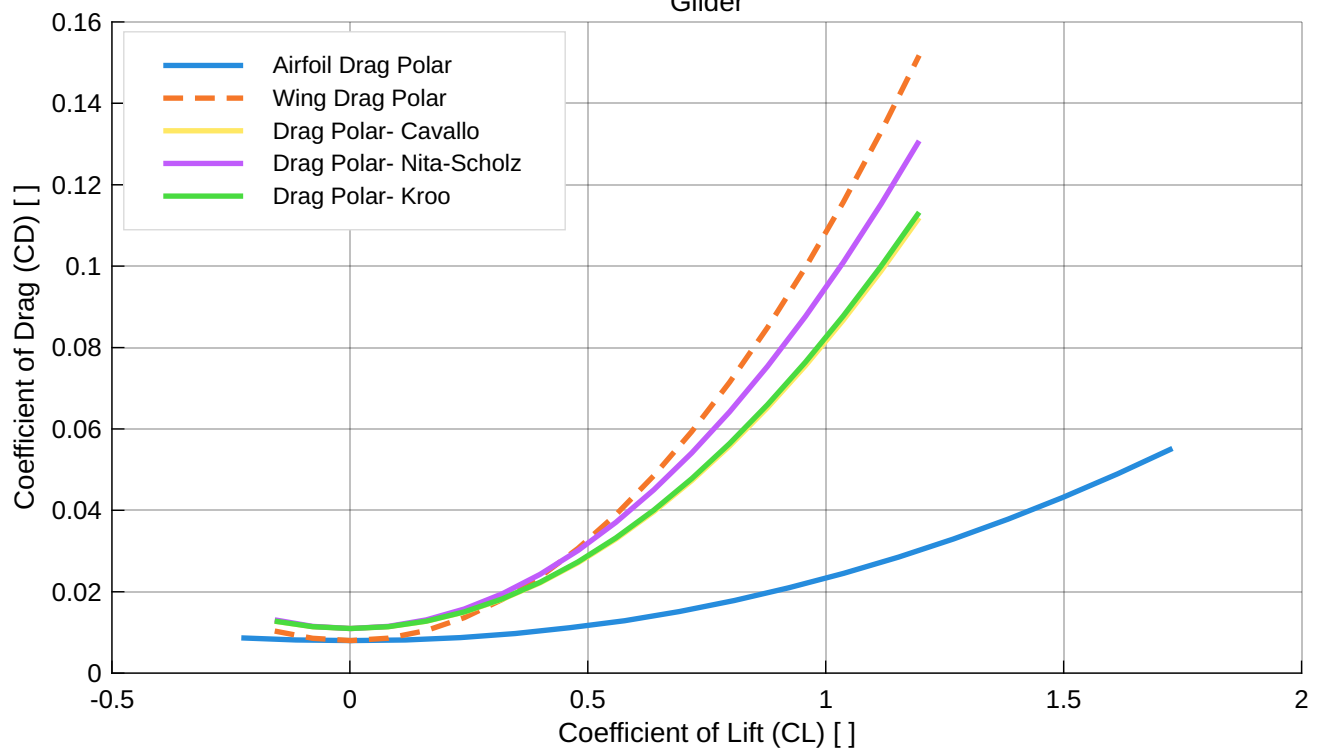
Drag Polar Model Comparison Config:
