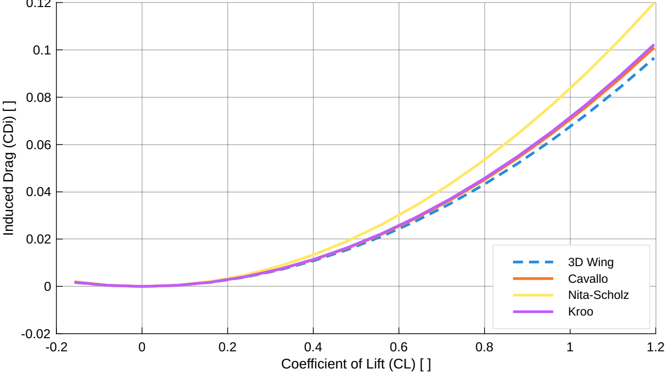
Induced Drag (CDi) Modeling Config: Glider
