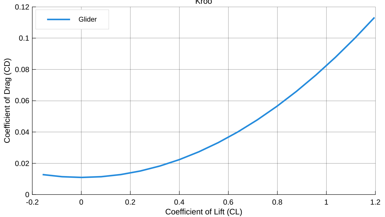
Drag Polar Configuration Comparison -
