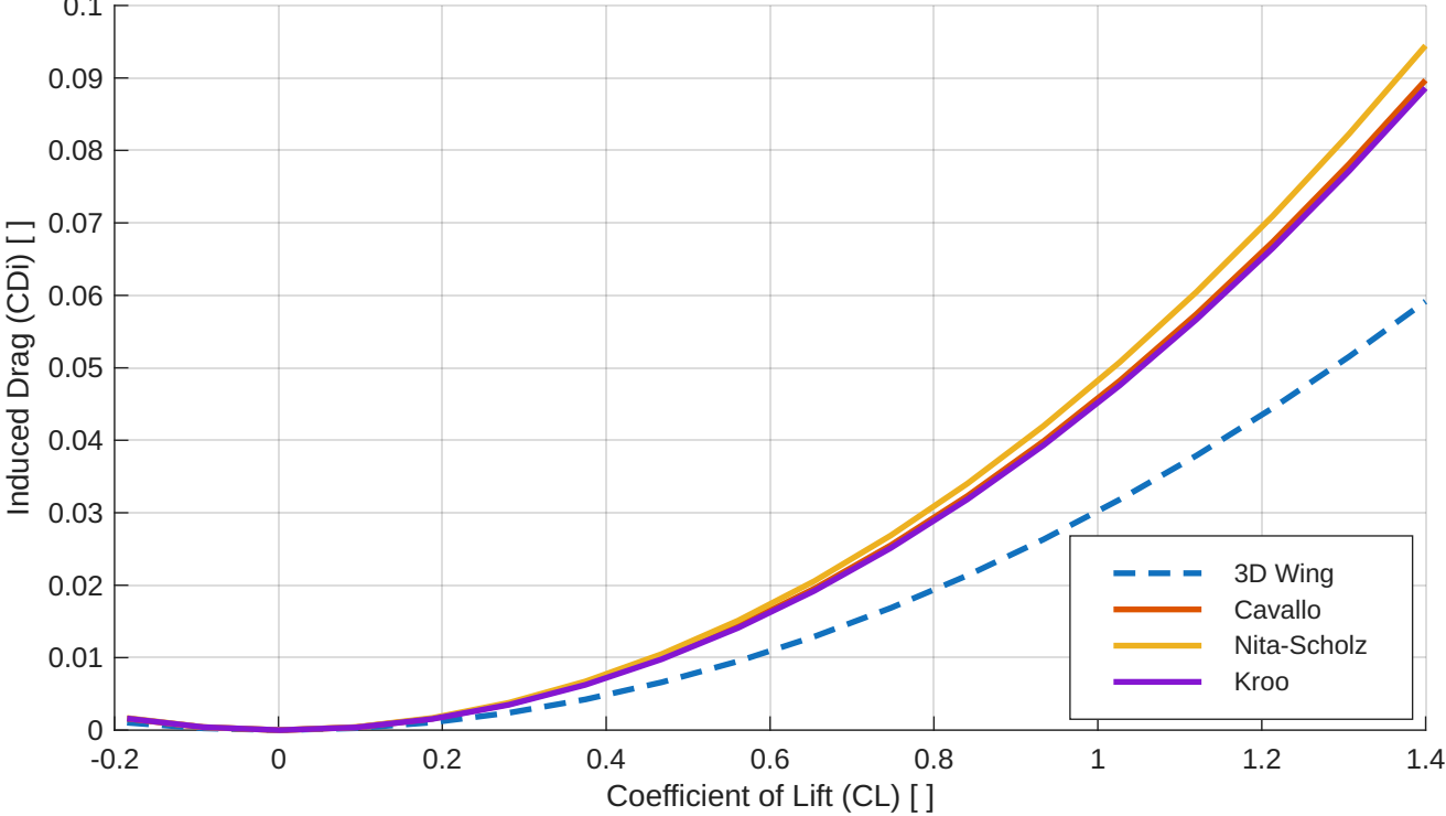
Induced Drag (CDi) Modeling Config: Owen
