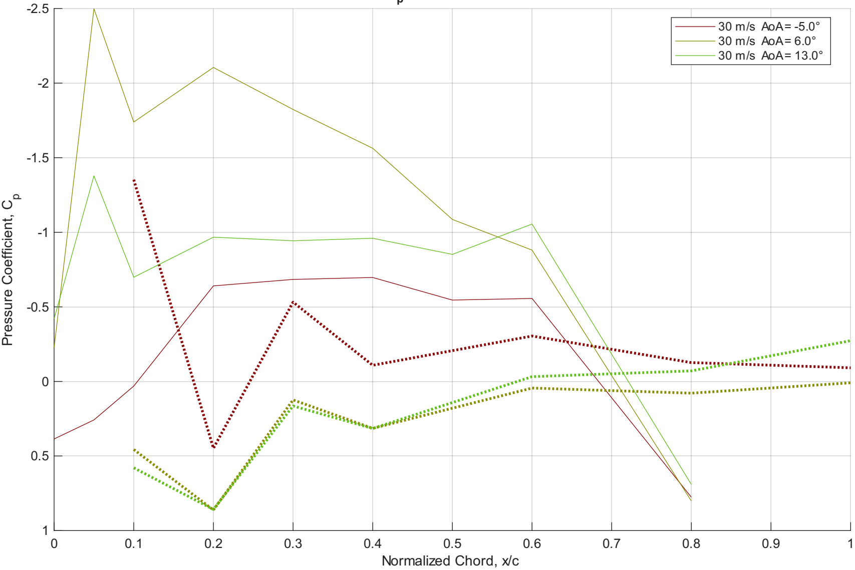
C_p vs x/c for 30 m/s
