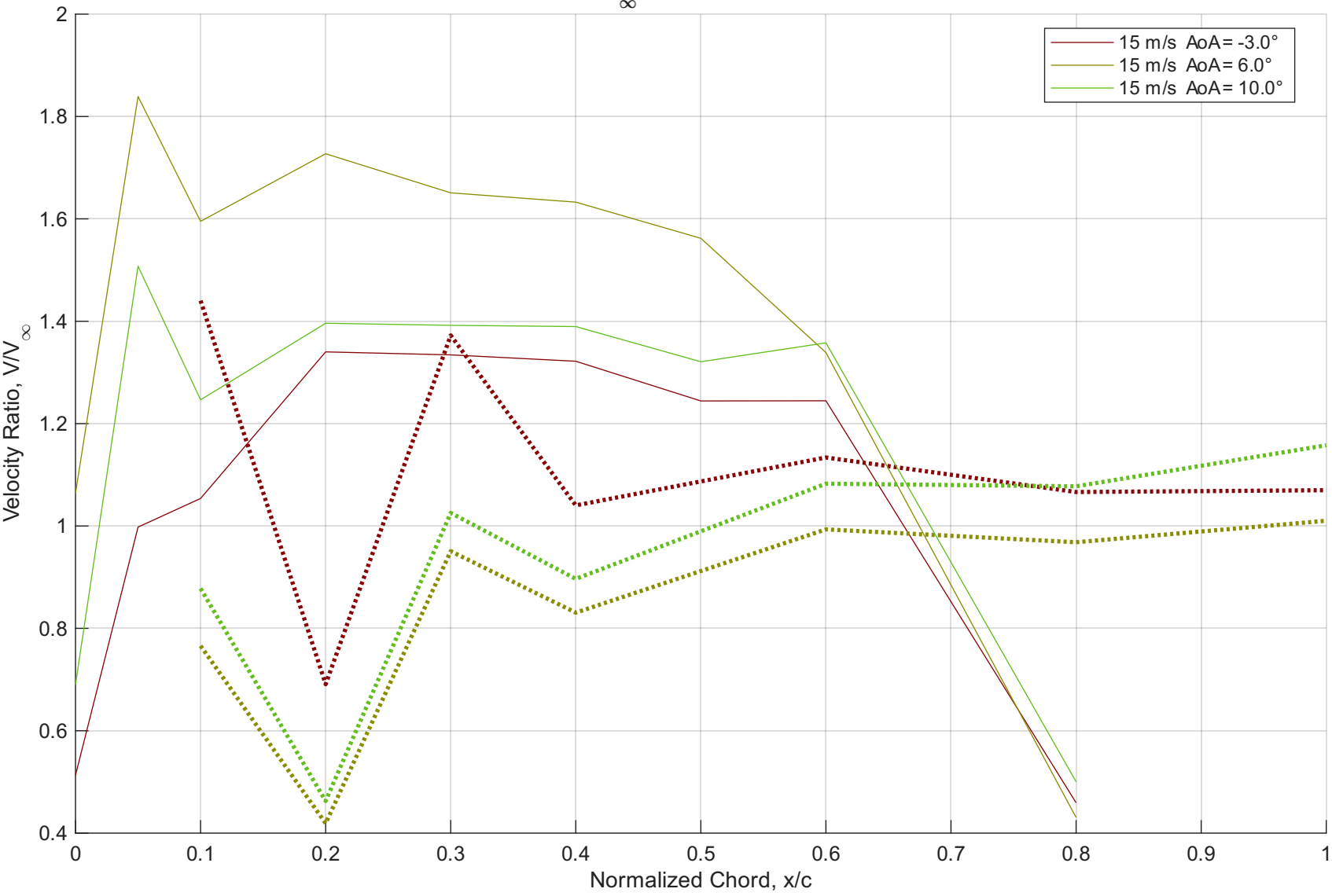
V/V_\infty vs x/c for 15 m/s
