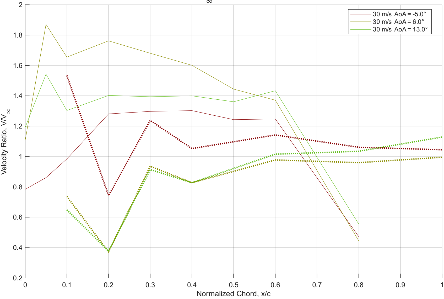
V/V_\infty vs x/c for 30 m/s
