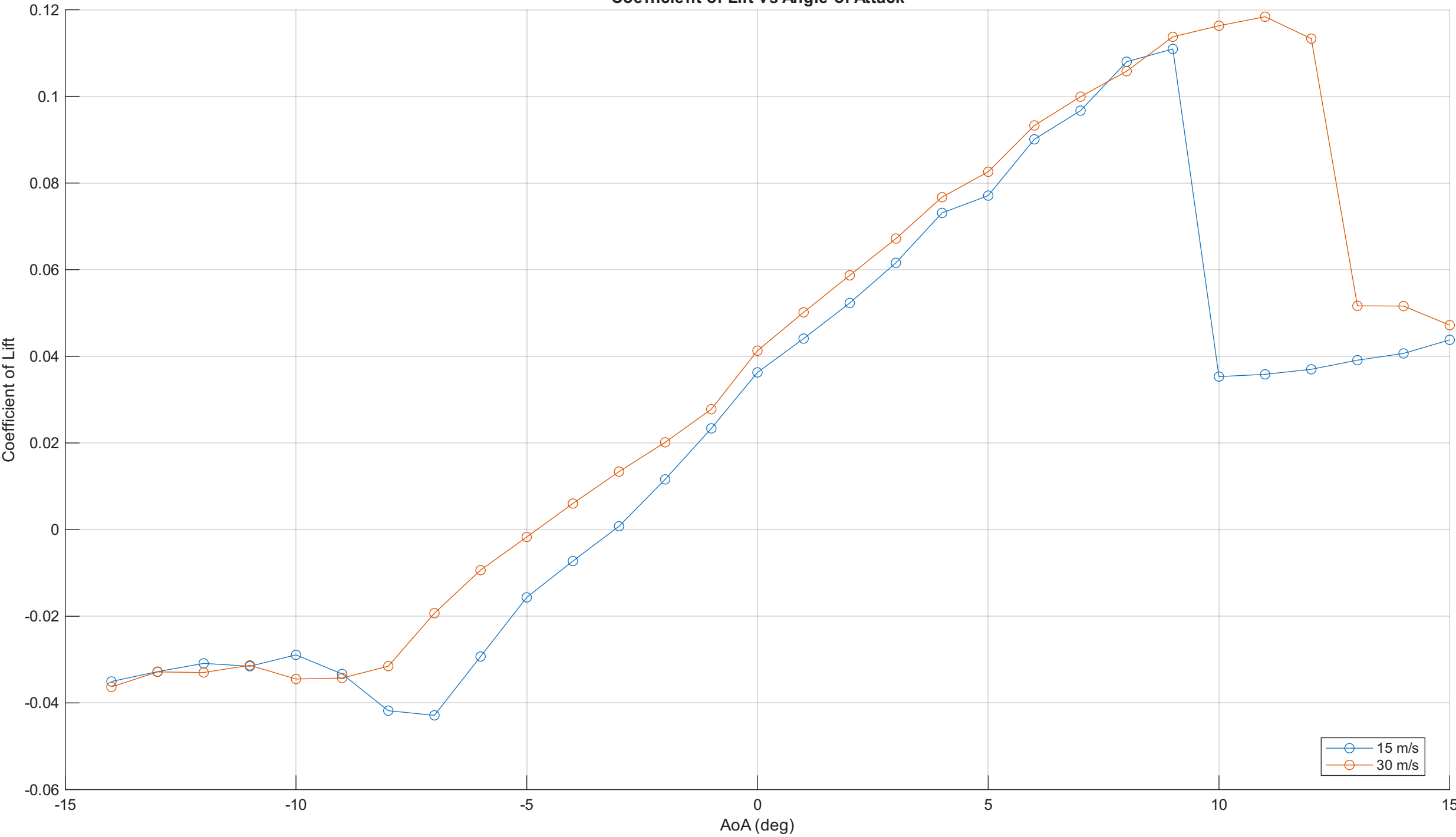
Coefficient of Lift vs Angle of Attack
