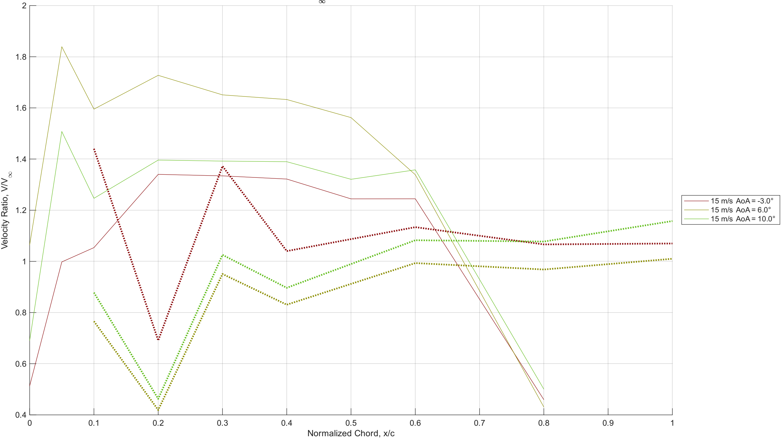
V/V_\infty vs x/c for 15 m/s
