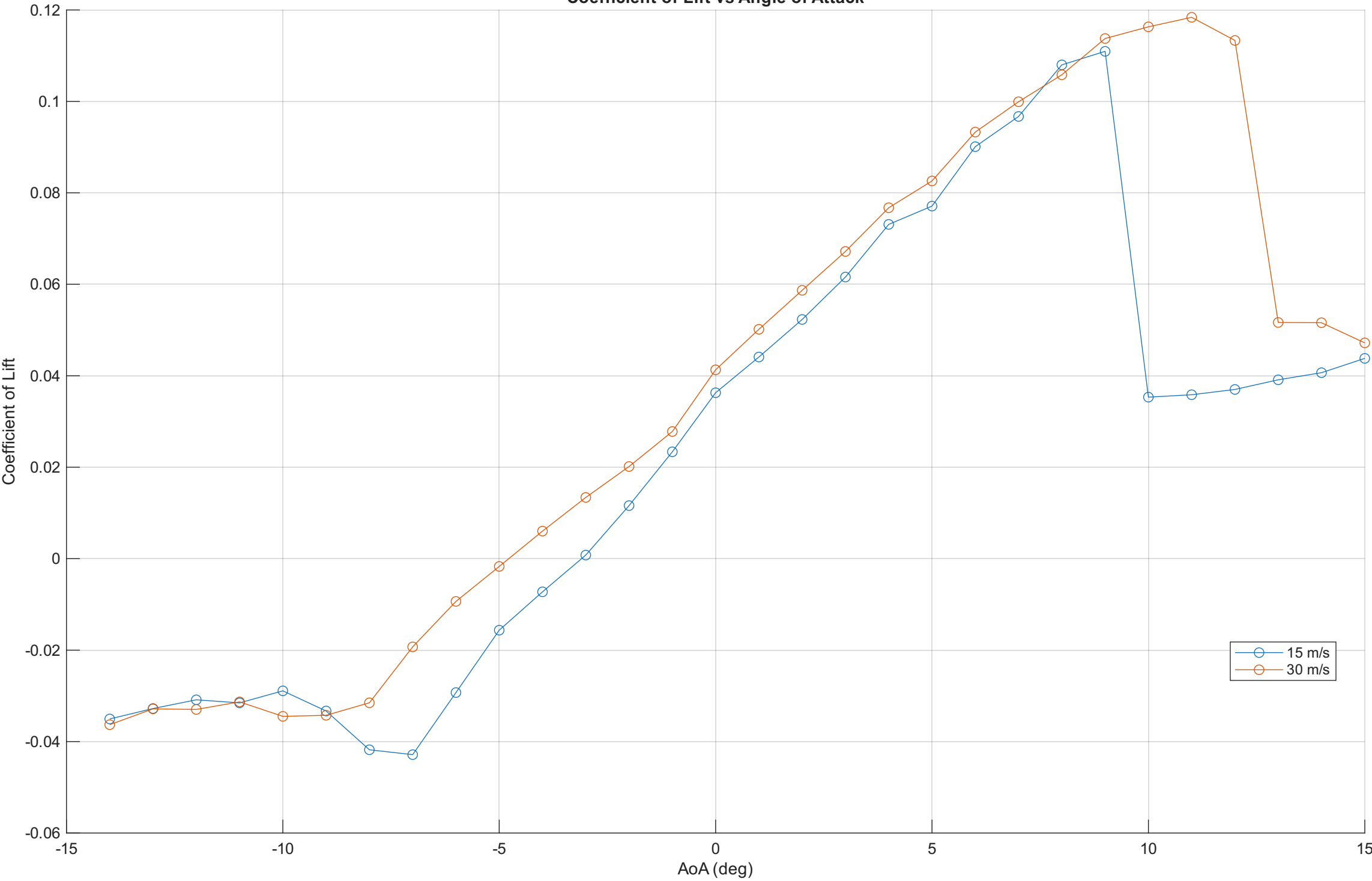
Coefficient of Lift vs Angle of Attack
