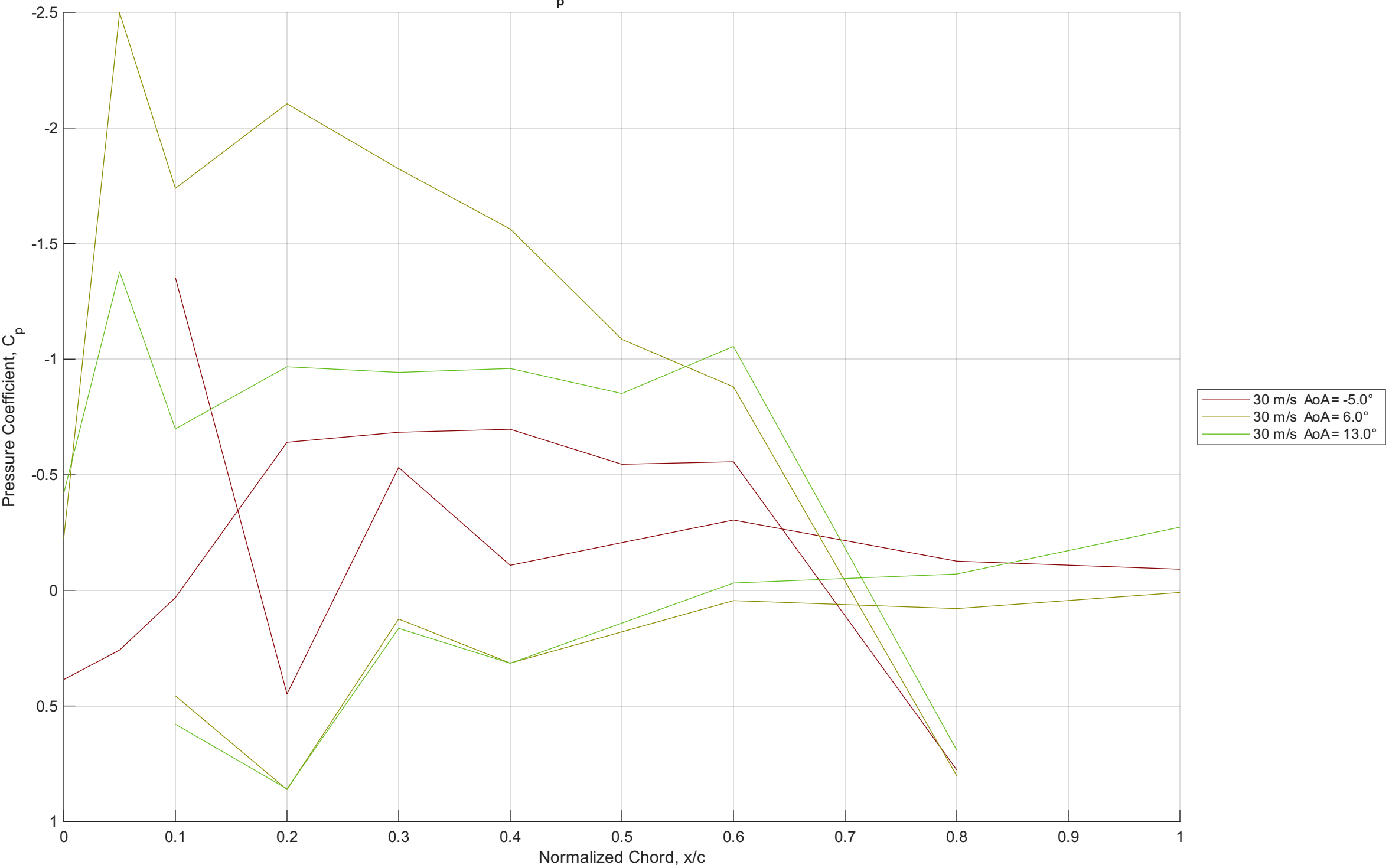
C_p vs x/c for 30 m/s
