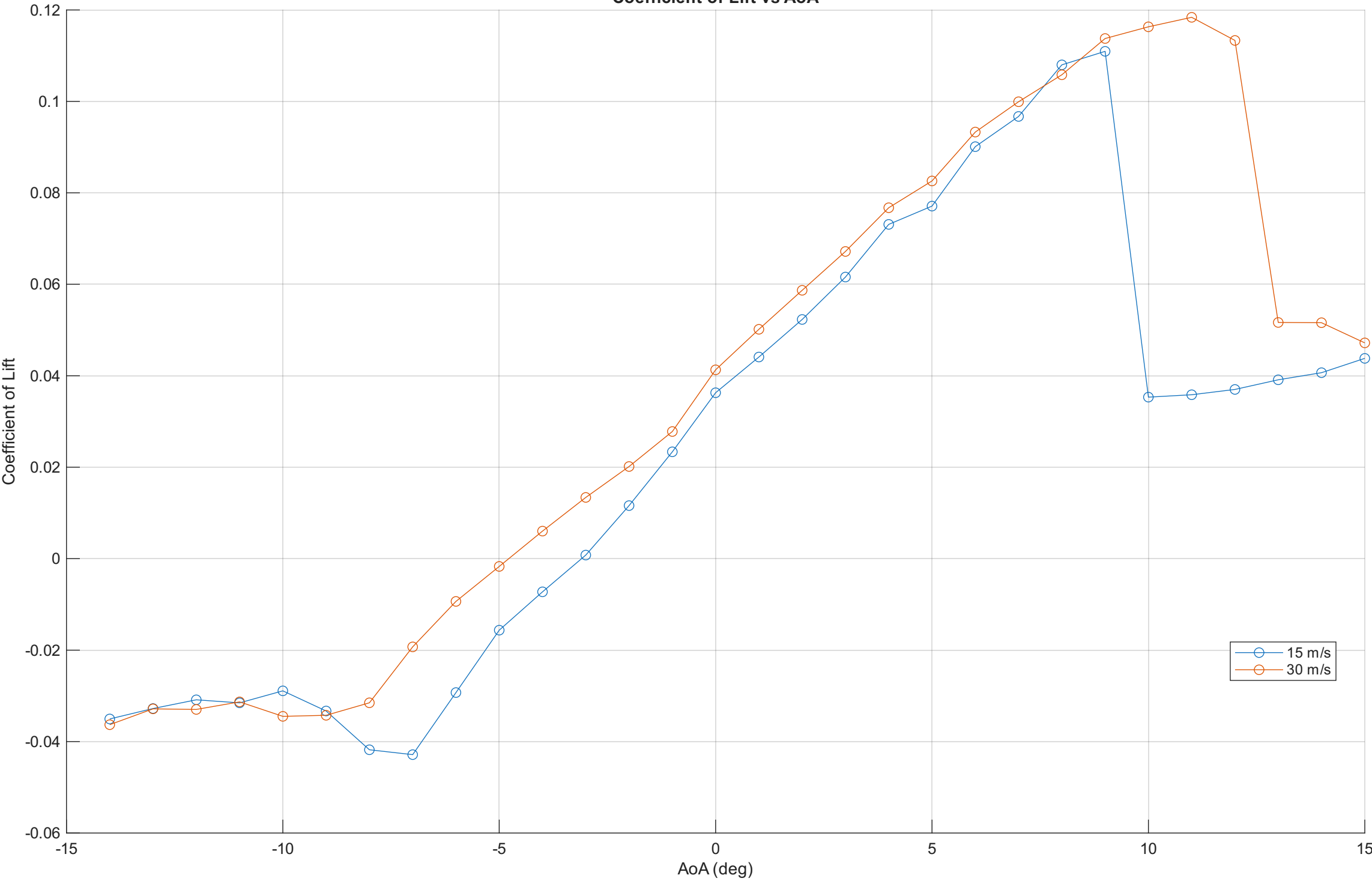
Coefficient of Lift vs AoA
