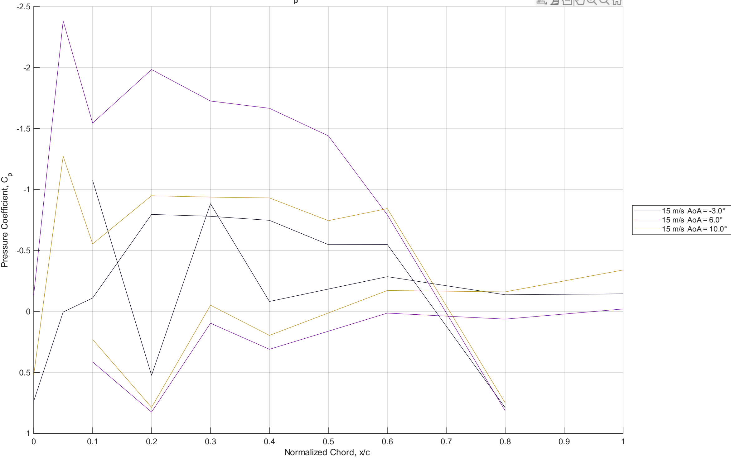
C_p vs x/c for 15 m/s
