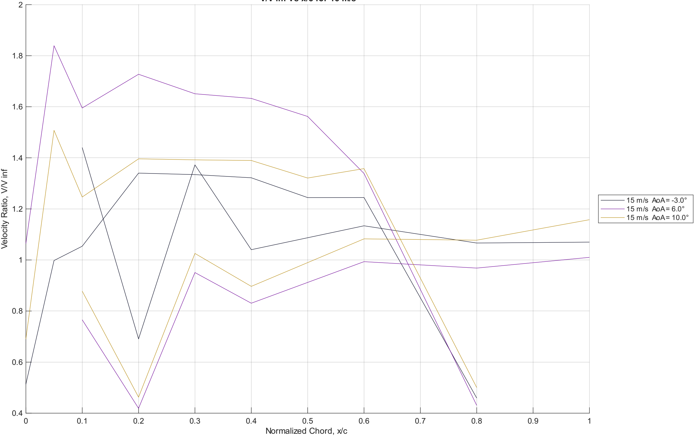
V/V inf vs x/c for 15 m/s
