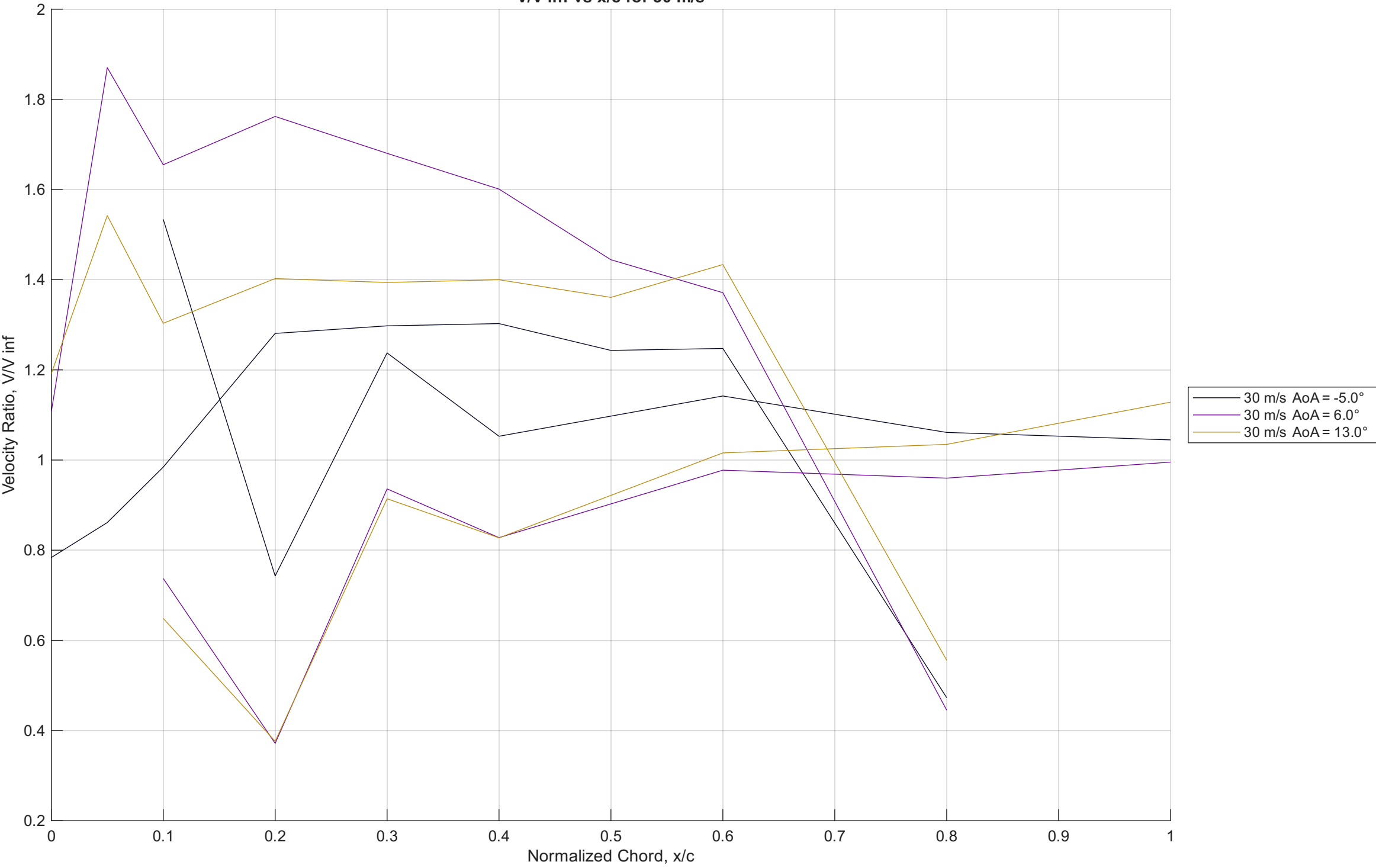
V/V inf vs x/c for 30 m/s
