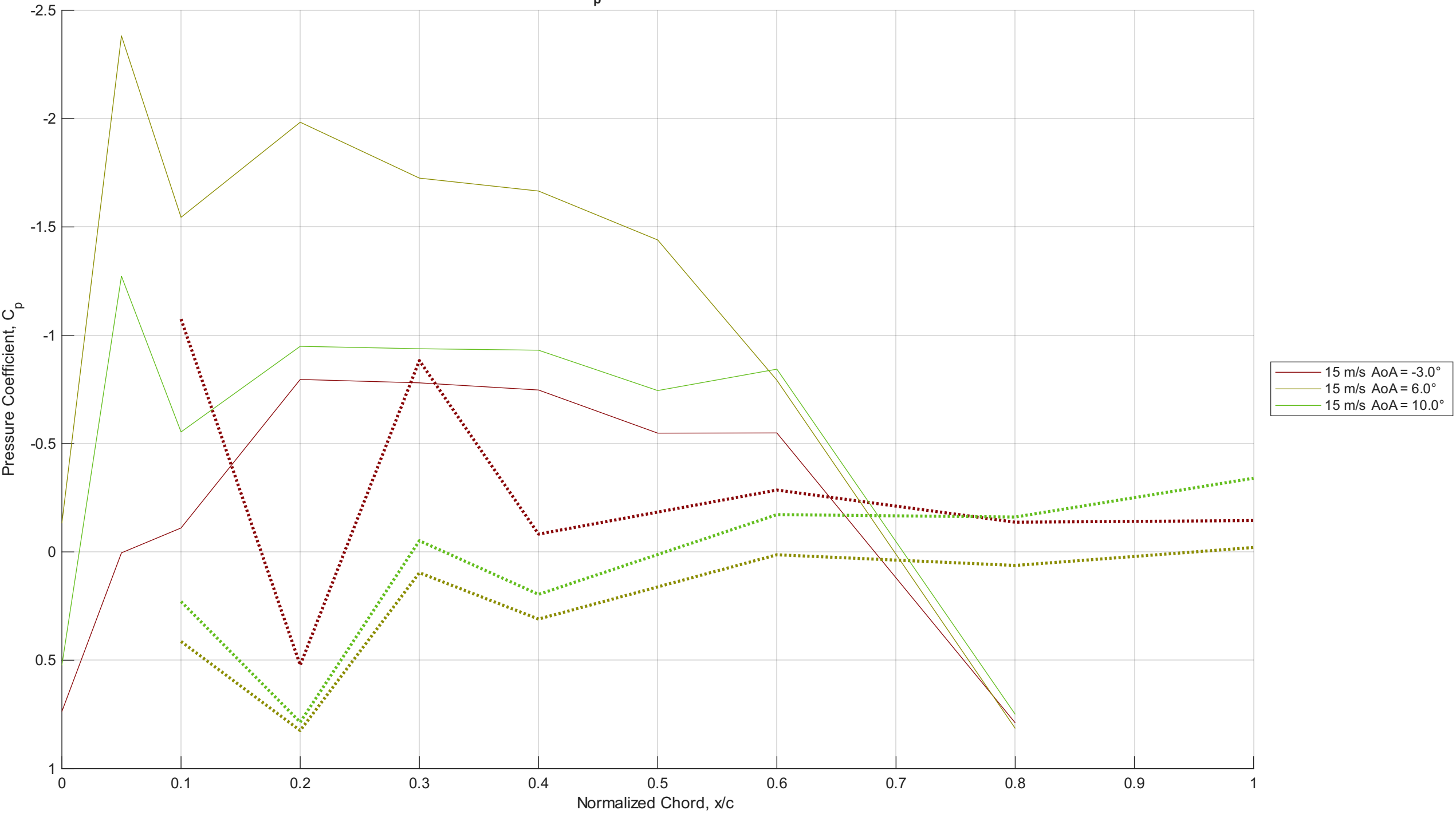
C_p vs x/c for 15 m/s
