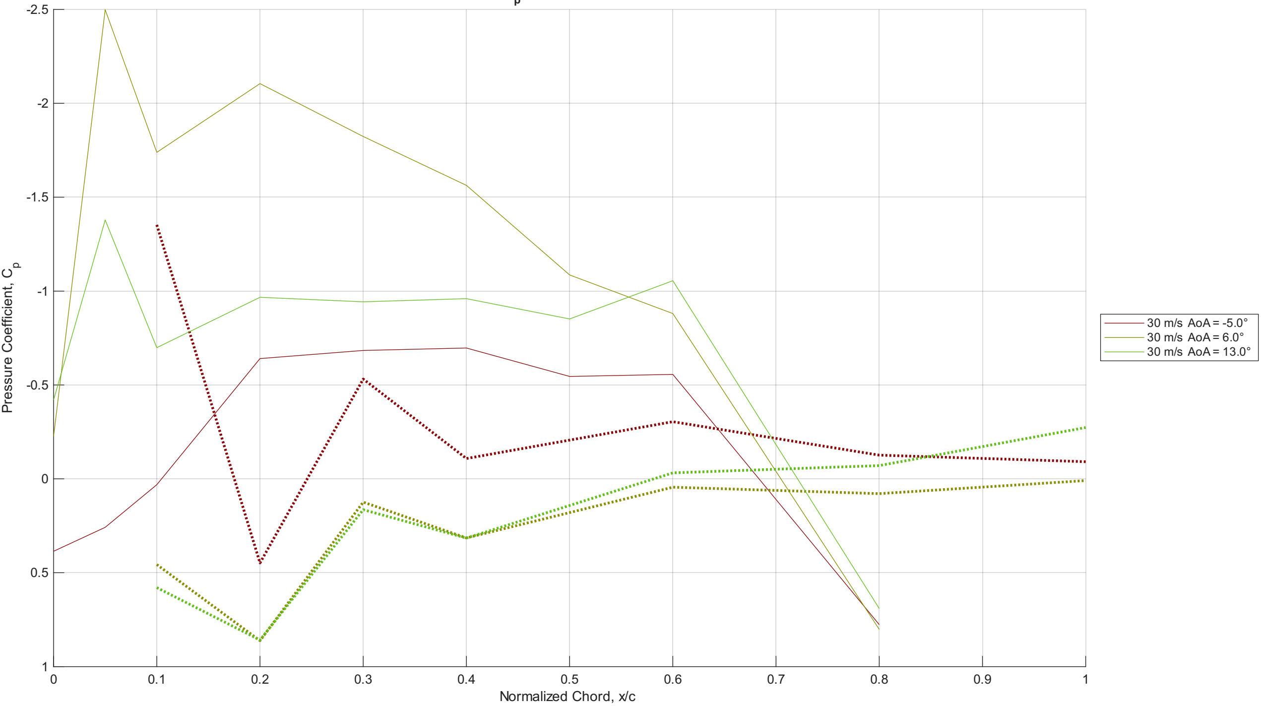
C_p vs x/c for 30 m/s
