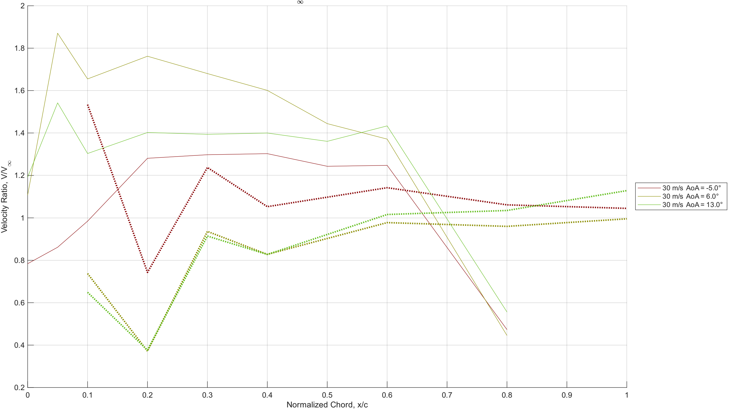
V/V_\infty vs x/c for 30 m/s
