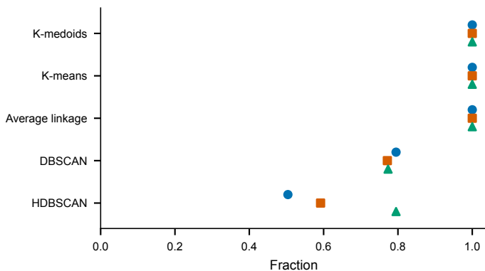
c Assigned fraction
