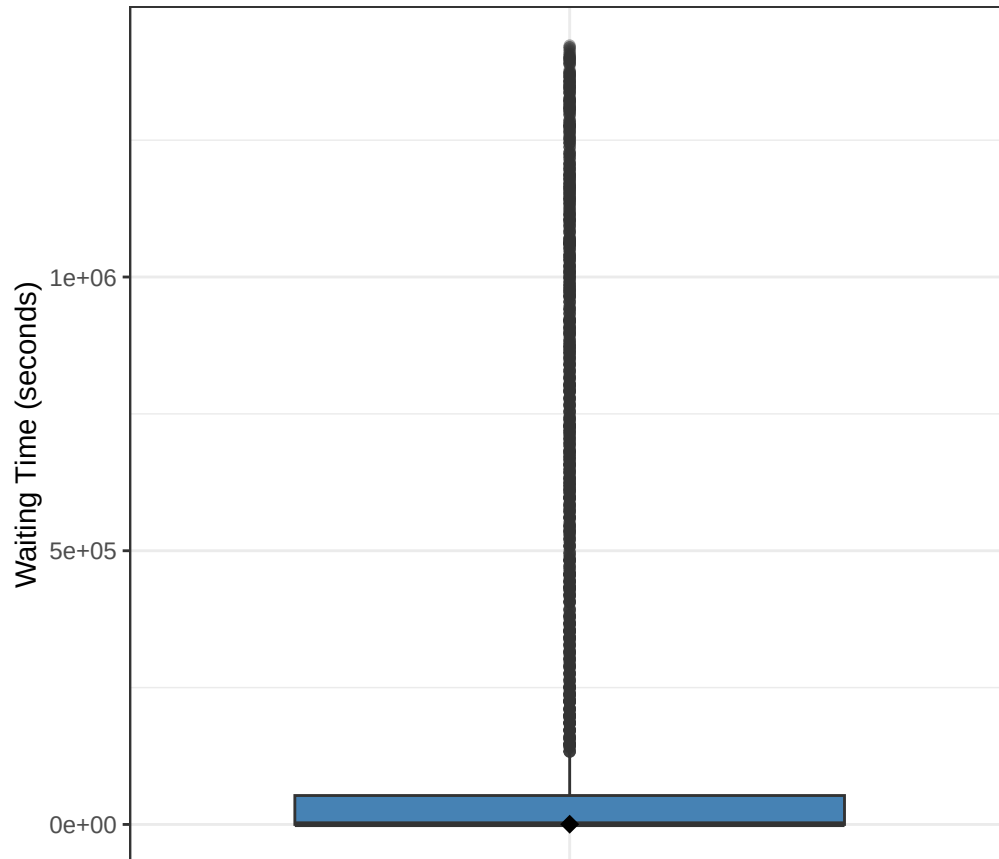
Waiting Time
