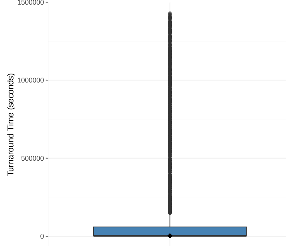
Turnaround Time
