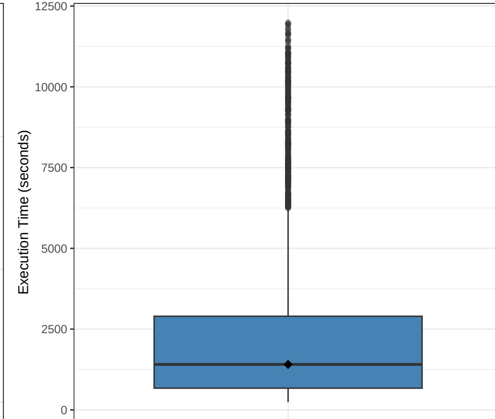
Execution Time
