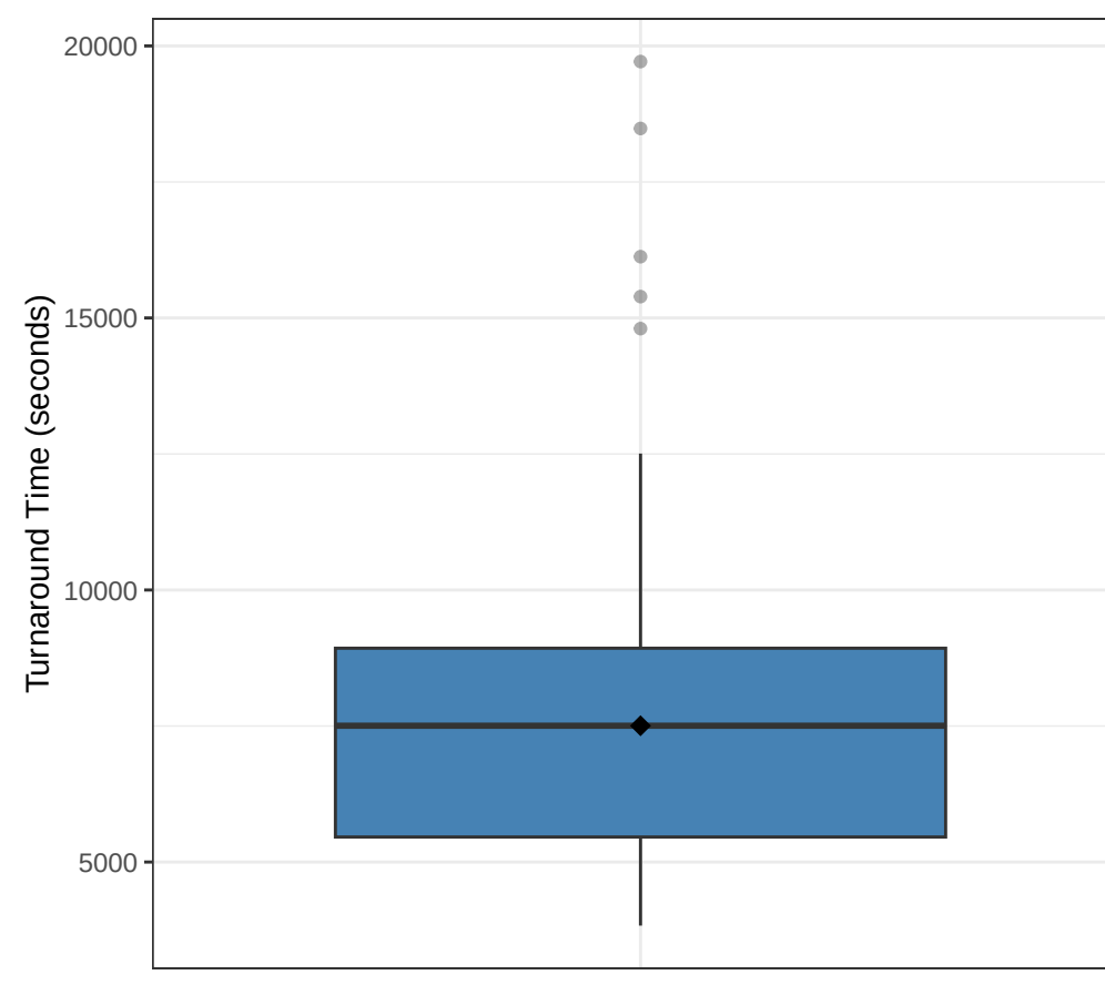
Turnaround Time
