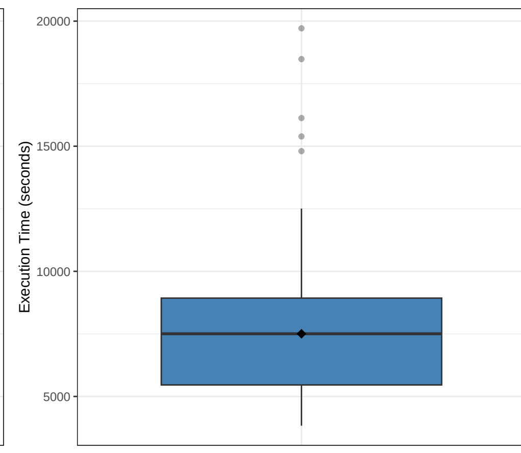
Execution Time
