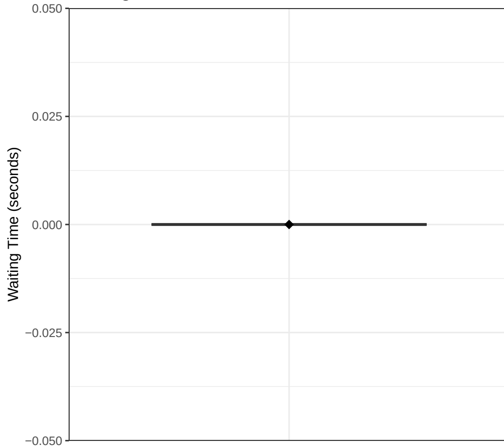
Waiting Time
