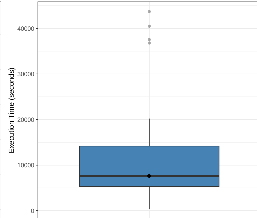
Execution Time
