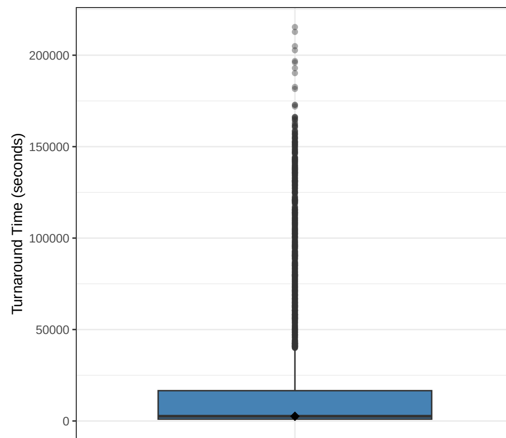
Turnaround Time
