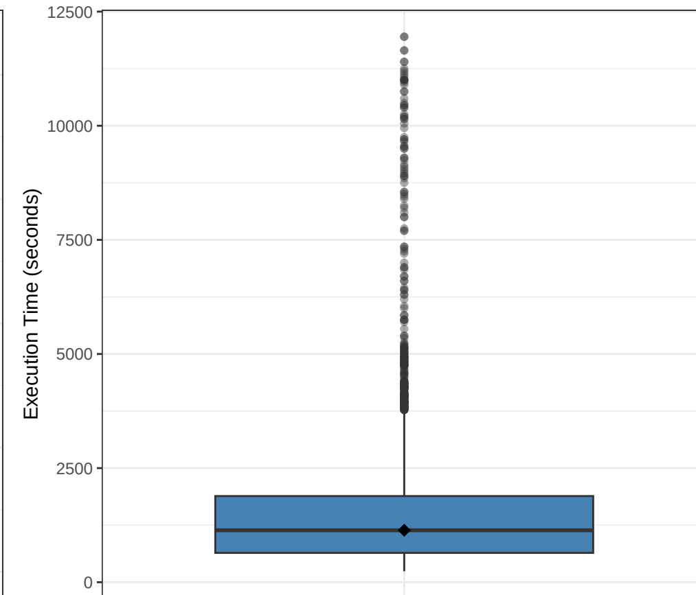
Execution Time
