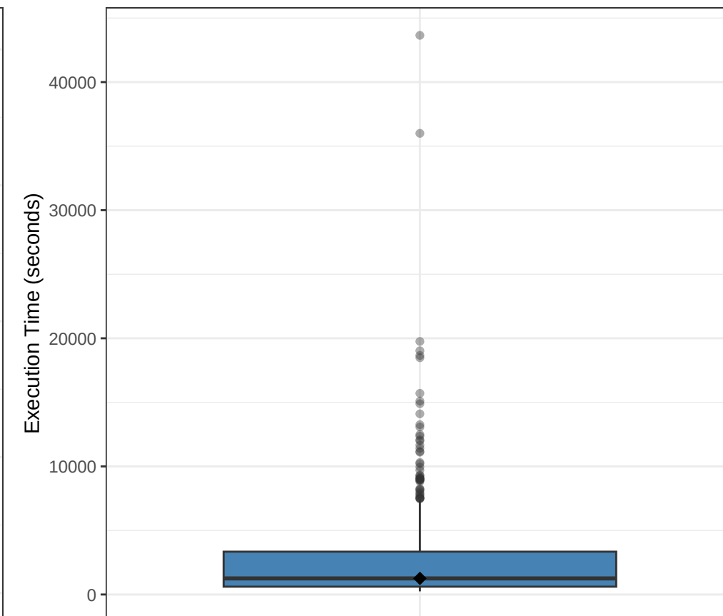
Execution Time
