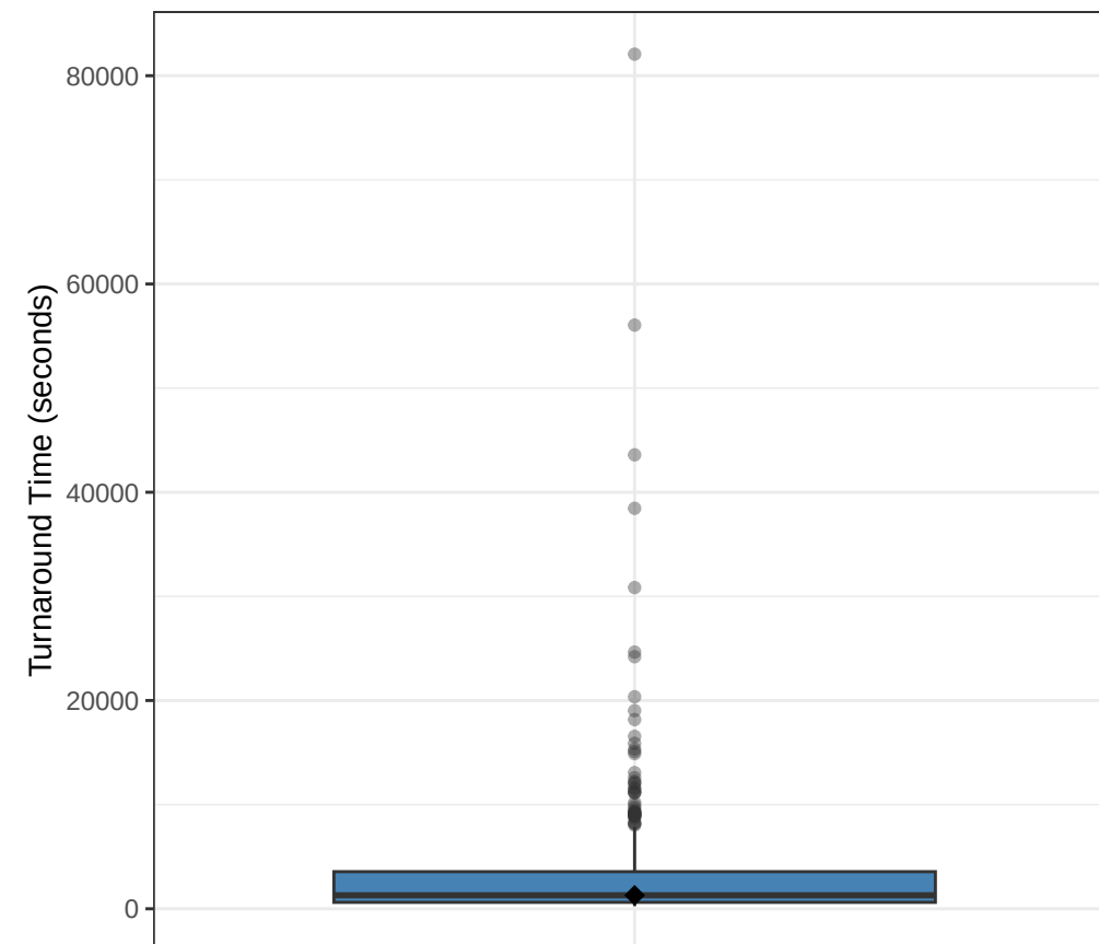
Turnaround Time
