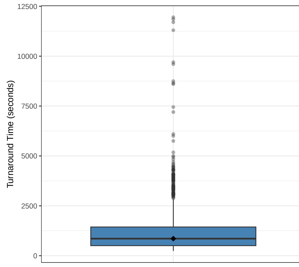
Turnaround Time
