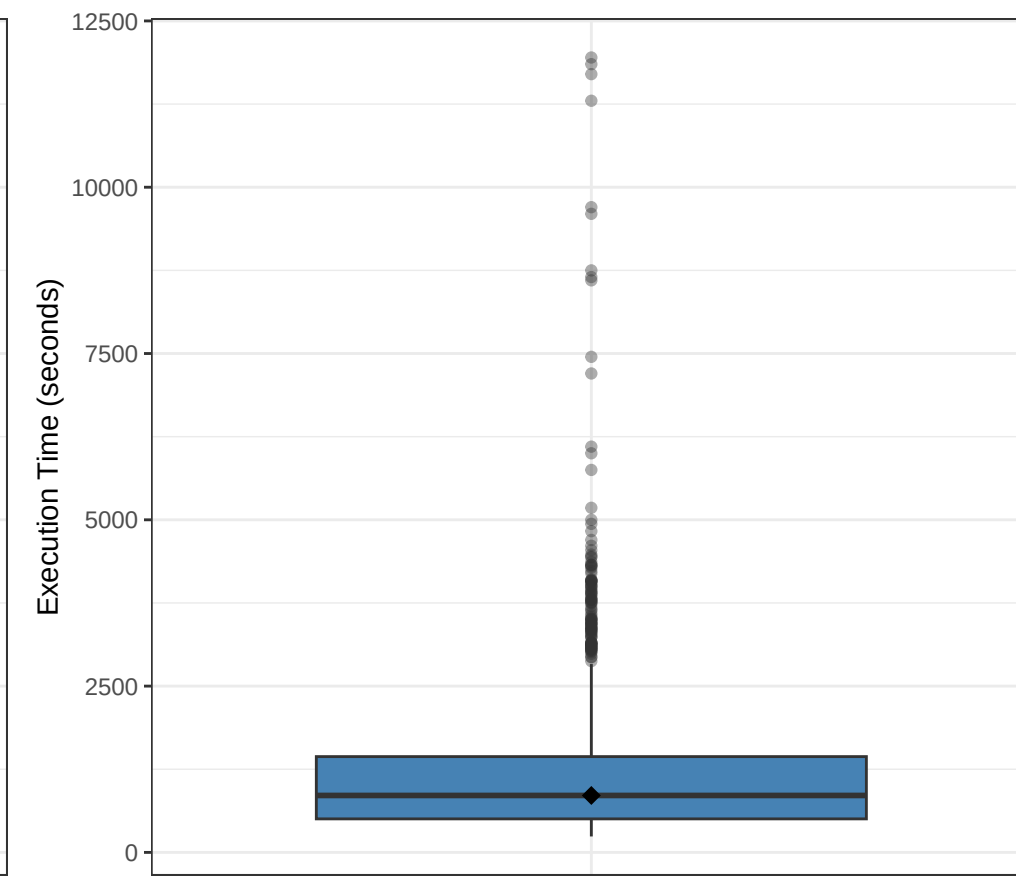
Execution Time
