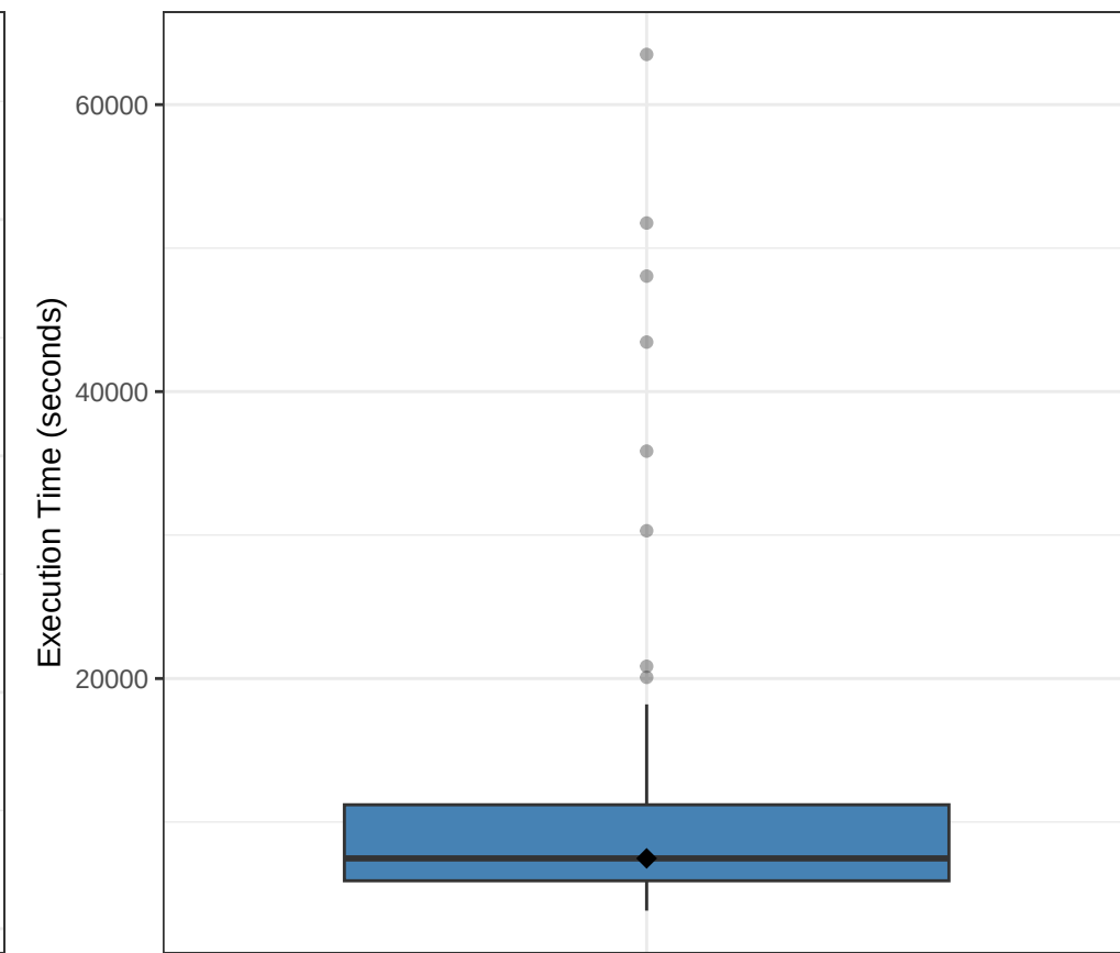
Execution Time
