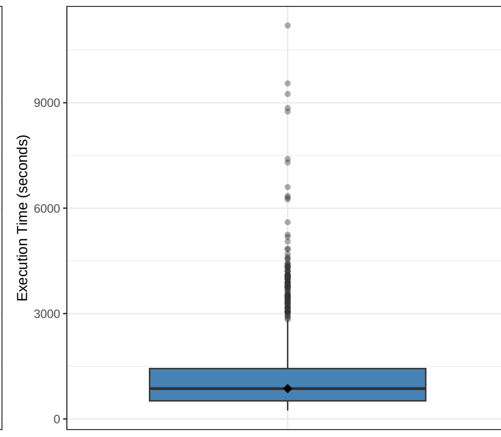
Execution Time
