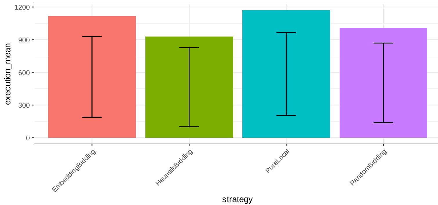
Mean Execution - business_mixed_20_80_67
